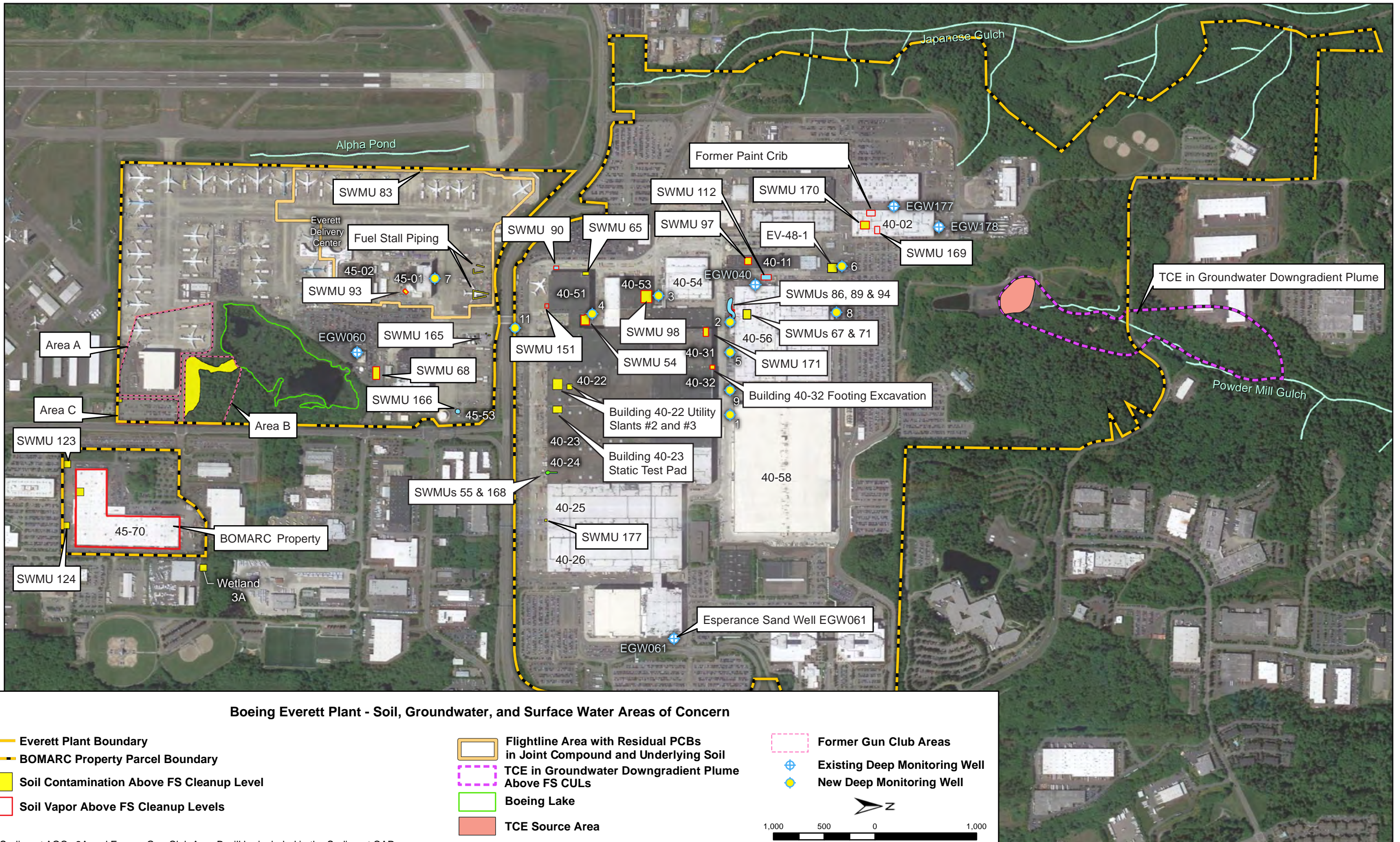
Figure 1-2 Site Plan – Boeing Everett Plant
