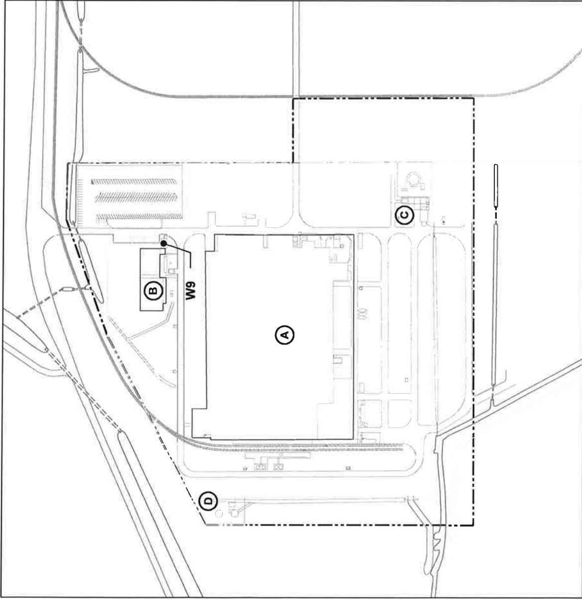
Former Reynolds Plant Building Demolition Northwest Alloys - Longview
