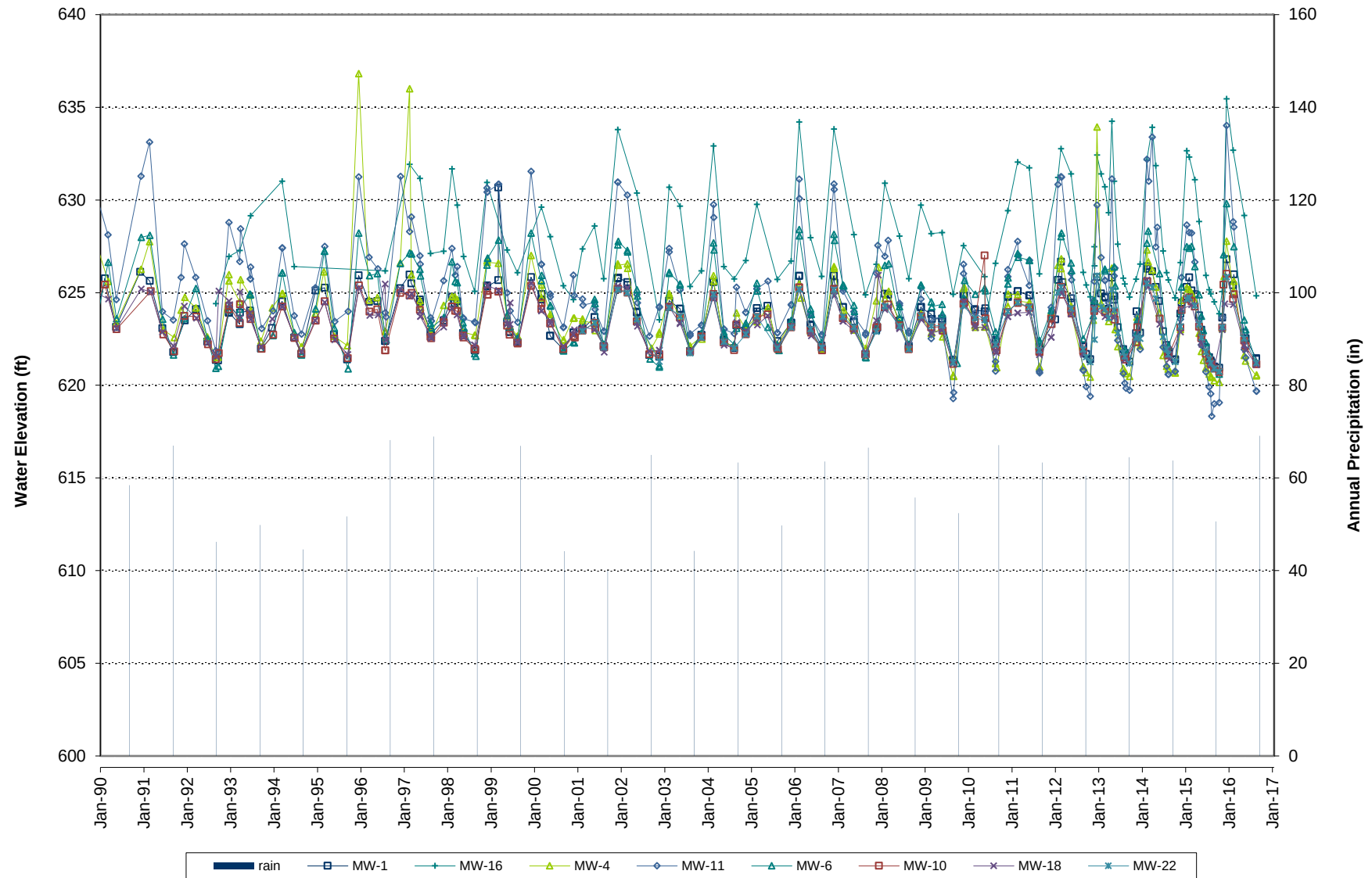
FIGURE 5. HOBART LANDFILL SHALLOW GROUNDWATER ELEVATIONS
