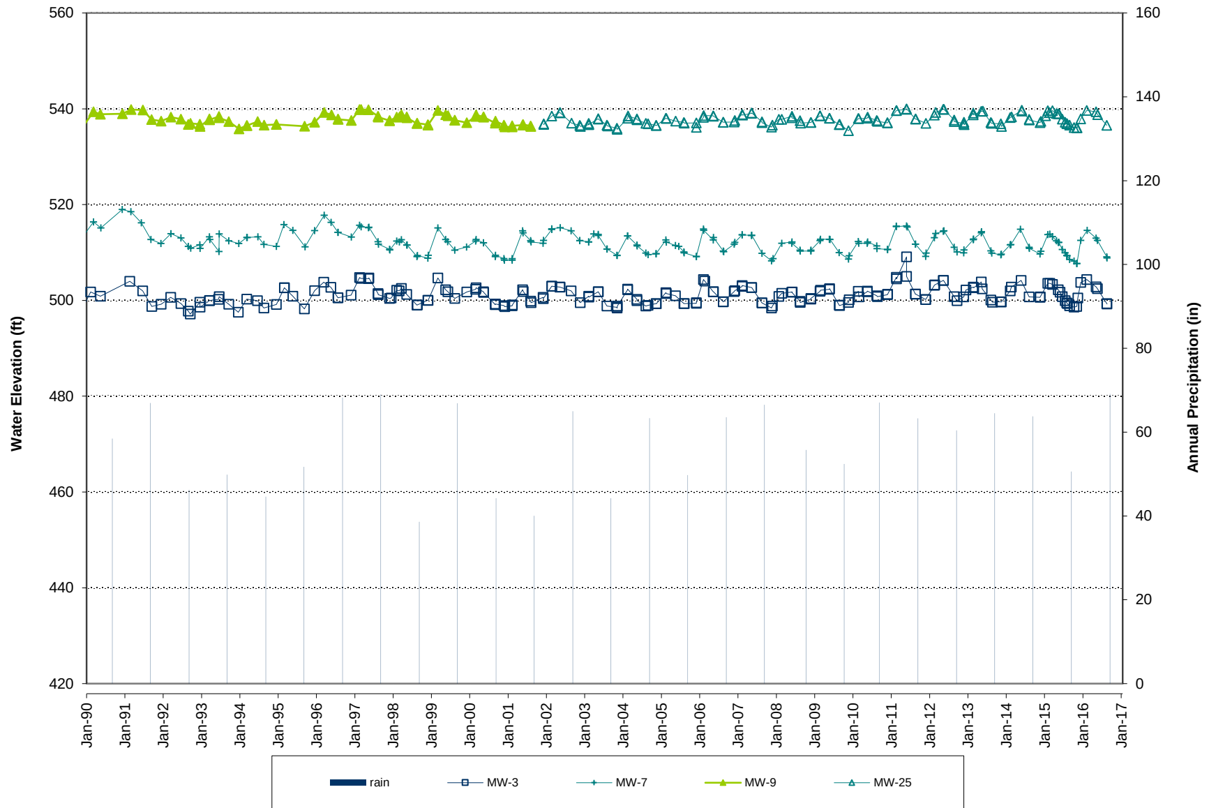
FIGURE 6. HOBART LANDFILL DEEP GROUNDWATER ELEVATIONS
