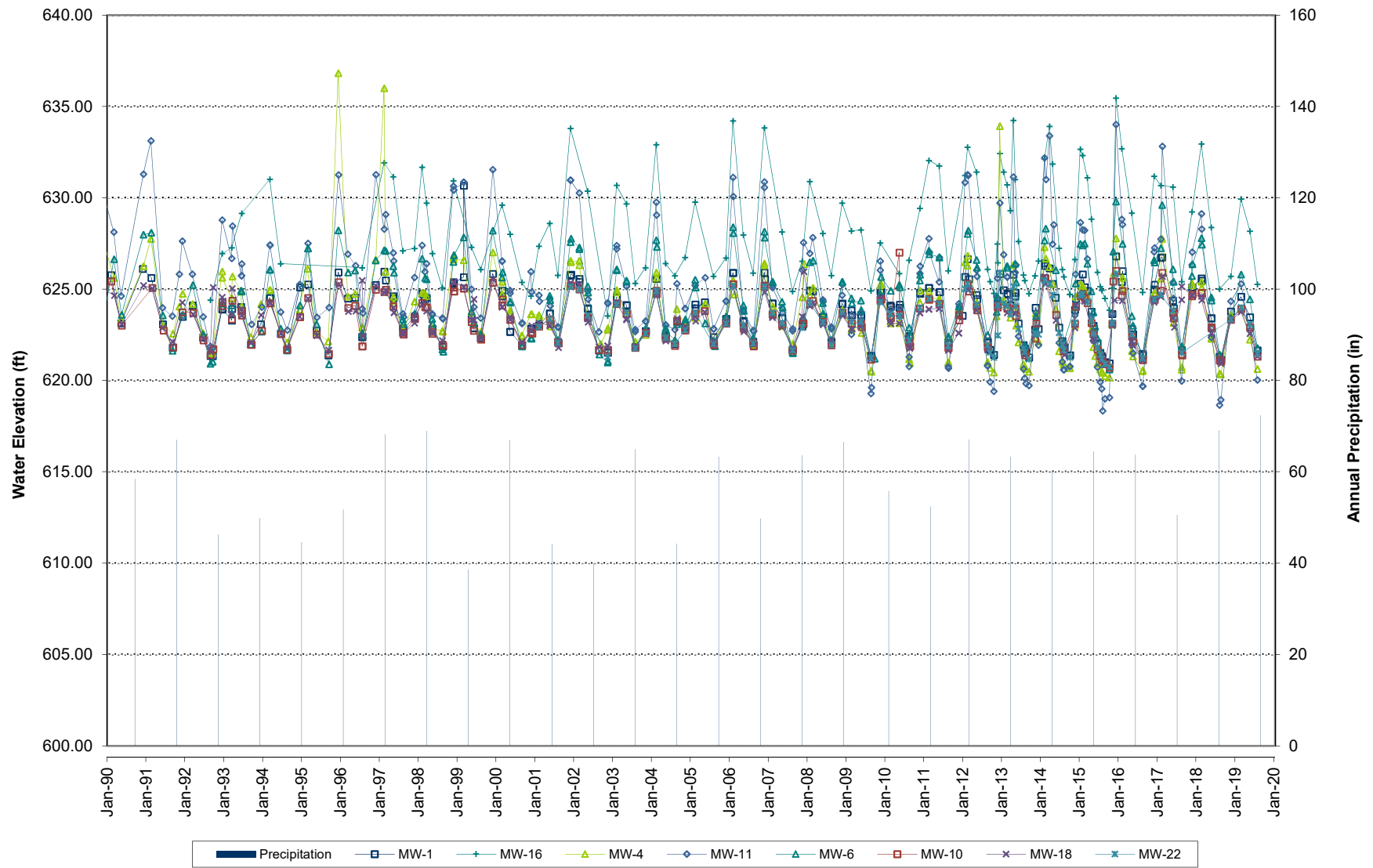
HOBART CLOSED LANDFILL FIGURE 6. SHALLOW AQUIFER HYDROGRAPH
