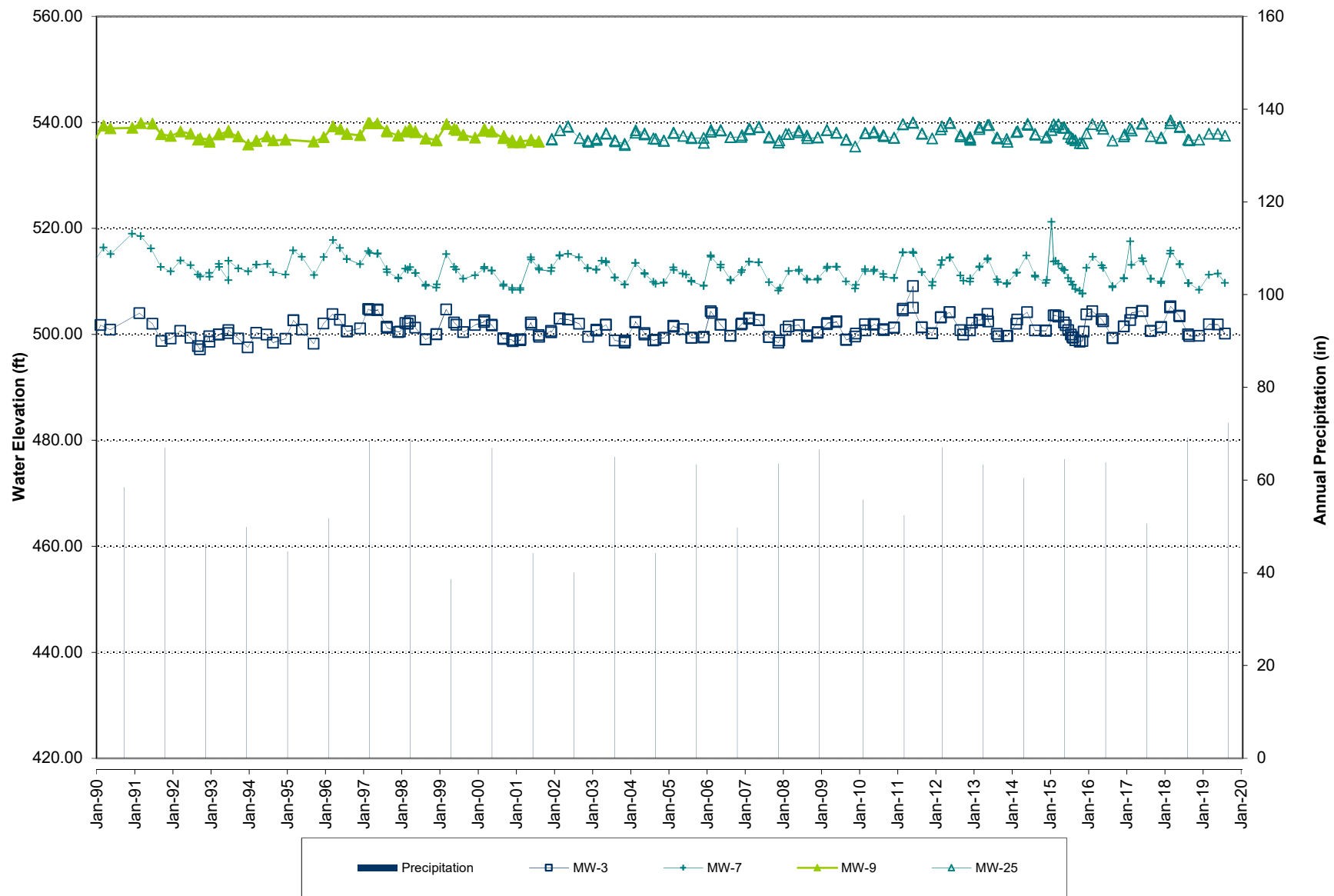
HOBART CLOSED LANDFILL FIGURE 7. DEEP AQUIFER HYDROGRAPH
