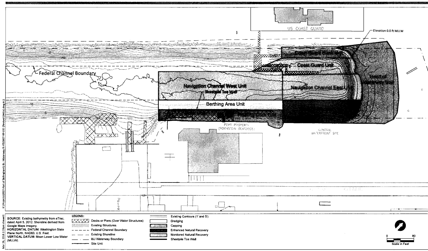
Figure 4-2 Alternative 2 Cleanup Action Plan I & J Waterway Site Port of Bellingham
