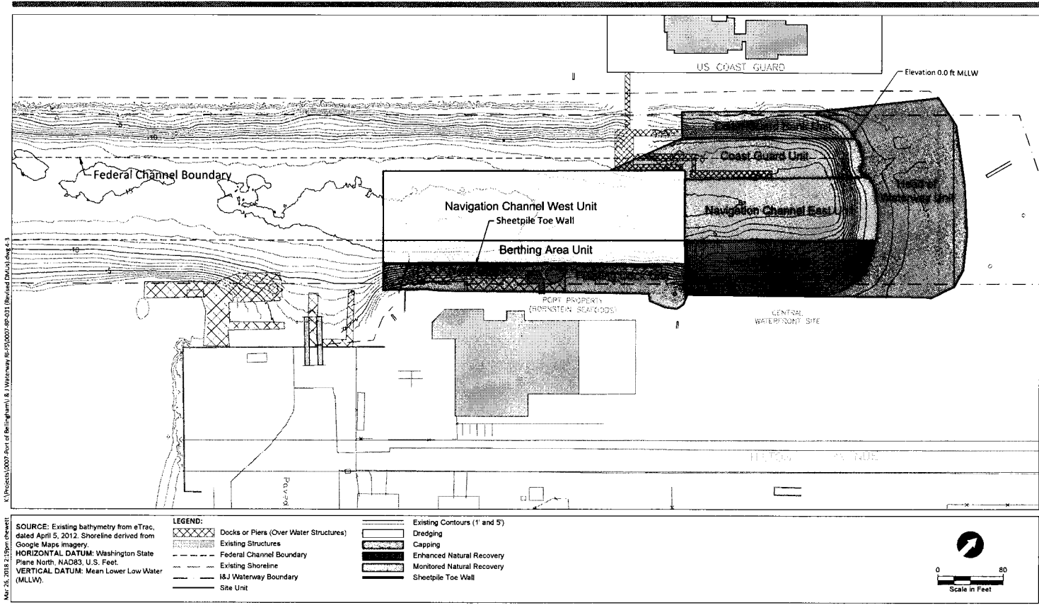
Figure 4-3 Alternative 3 Cleanup Action Plan I & J Waterway Site Port of Bellingham
