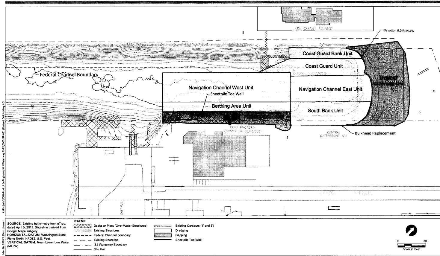
Figure 4-5 Alternative 5 Cleanup Action Plan I & J Waterway Site Port of Bellingham
