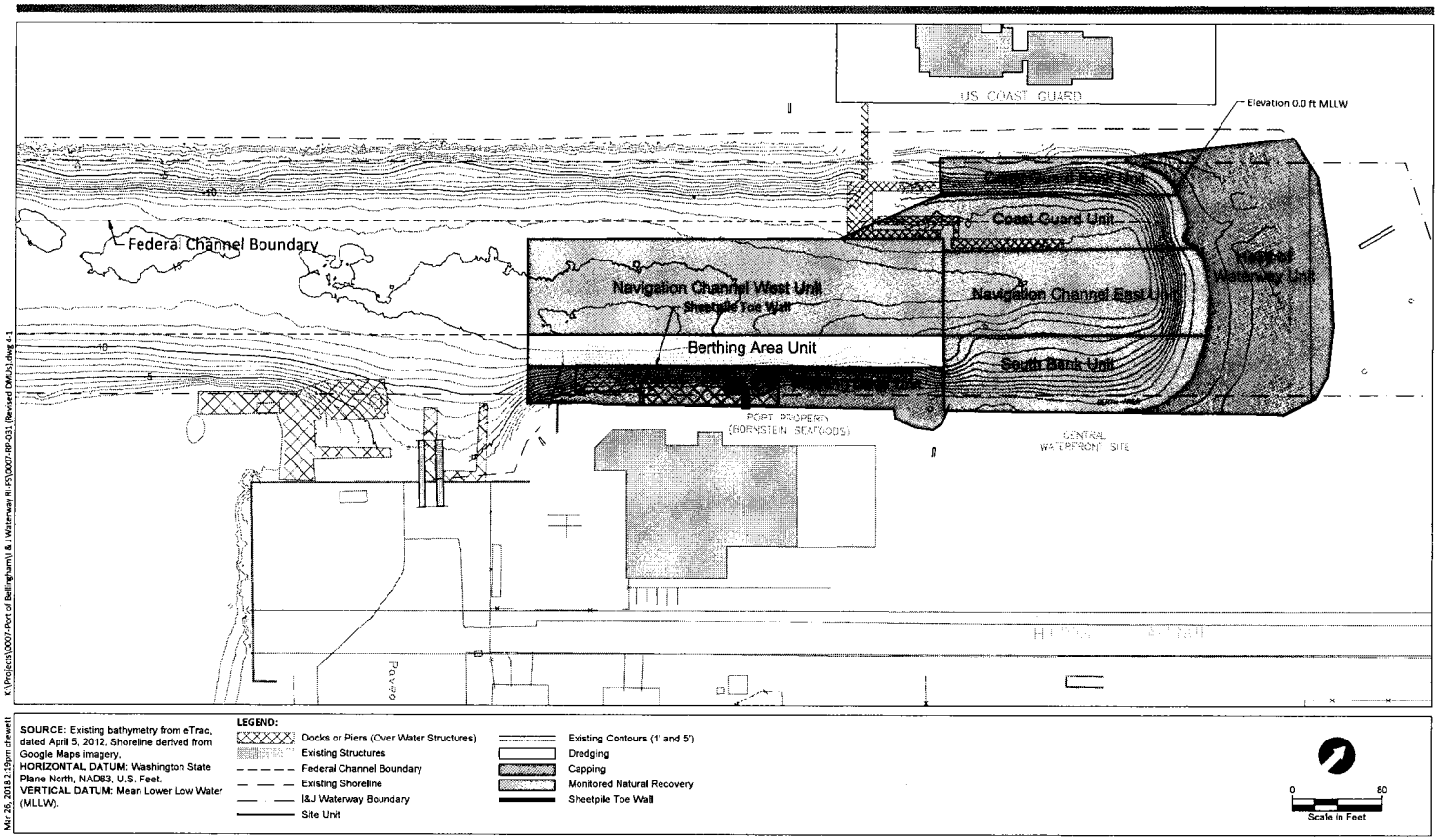
Figure 4-1 Alternative 1 Cleanup Action Plan I&J Waterway Site Port of Bellingham
