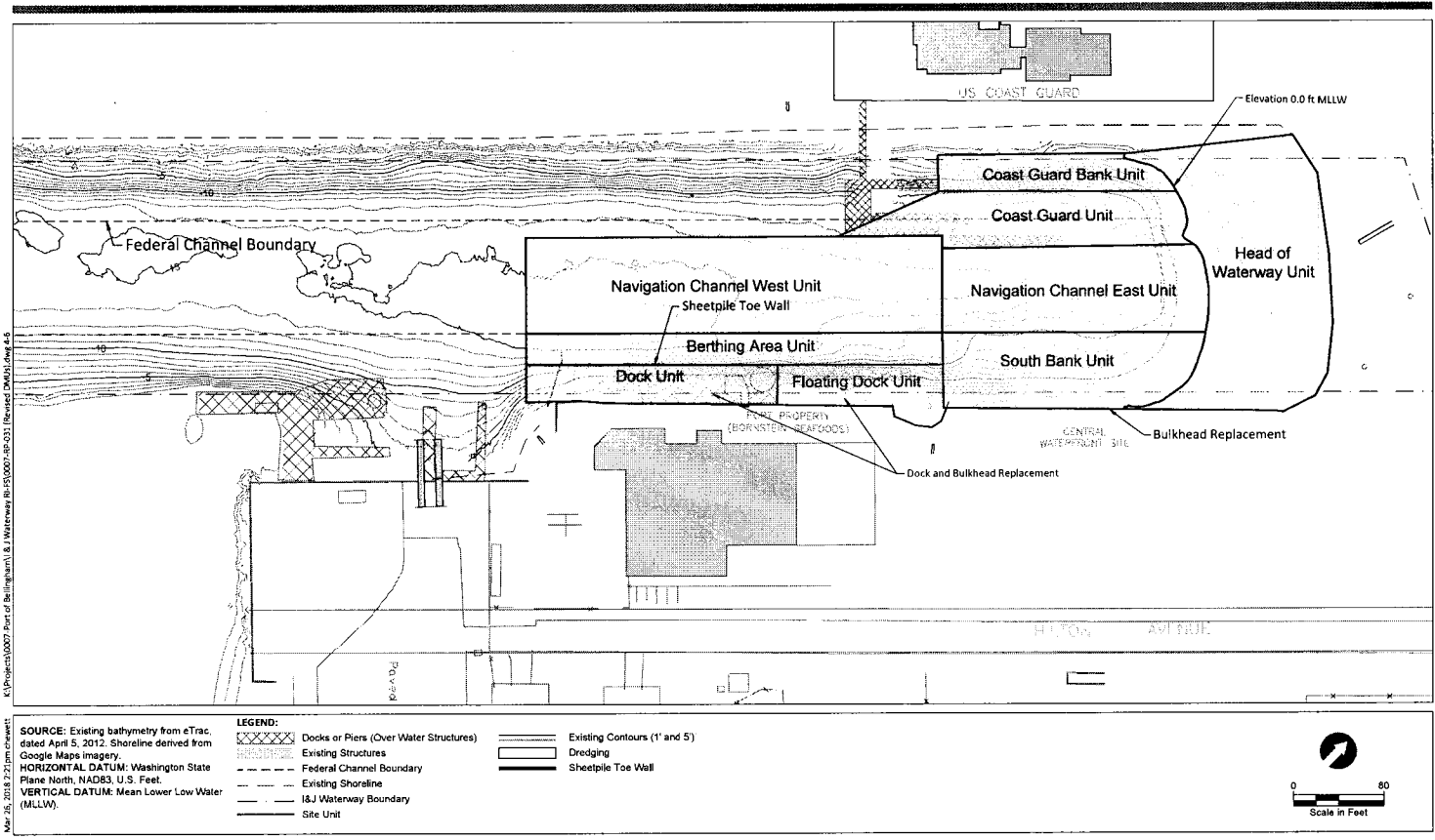
Figure 4-6 Alternative 6 Cleanup Action Plan I&J Waterway Site Port of Bellingham
