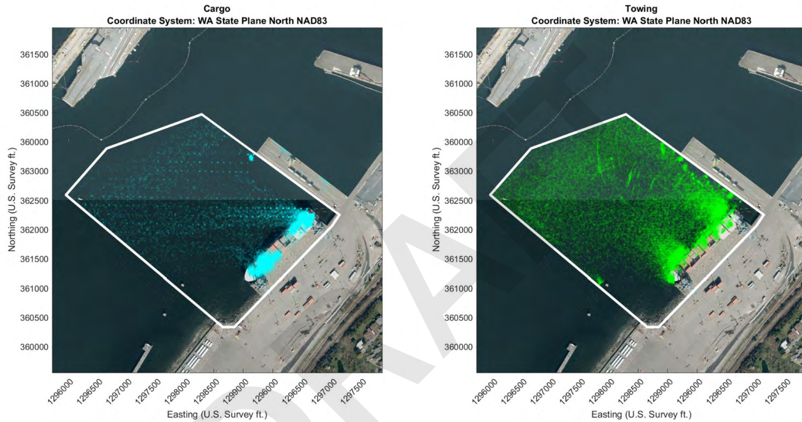
Figure 8. AIS Vessel Tracking Data for Cargo and Tugs (while towing/pushing vessel) at Pacific Terminal
