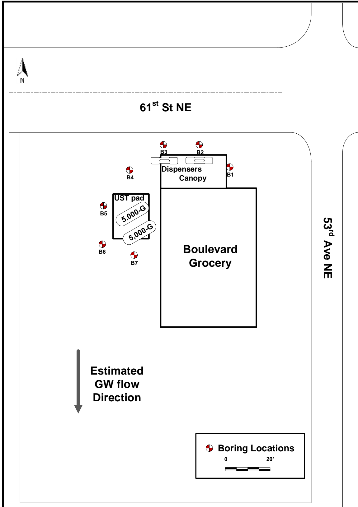
Figure 2. Site Plan
