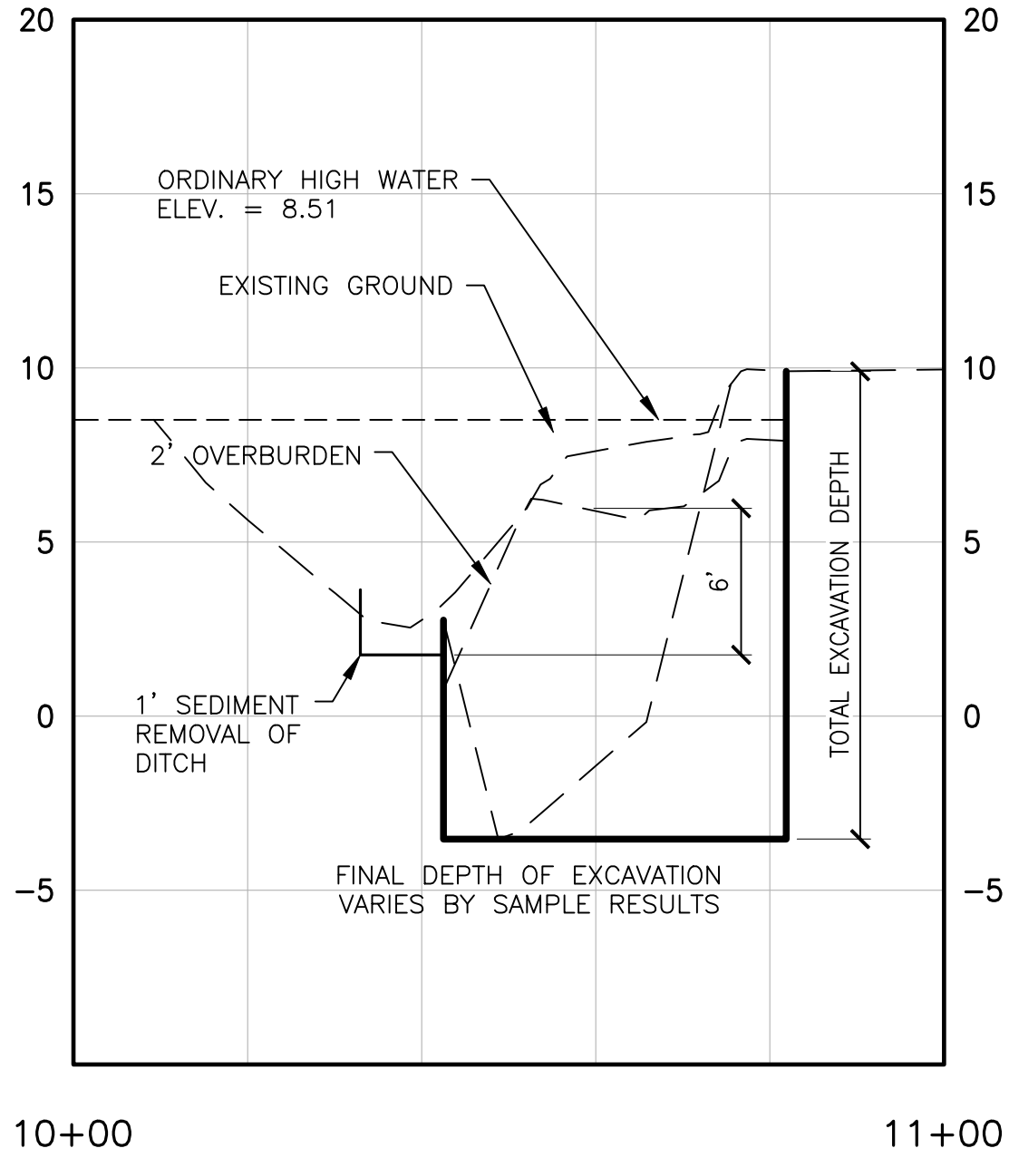
TYPICAL EXCAVATION CROSS-SECTION A-A
