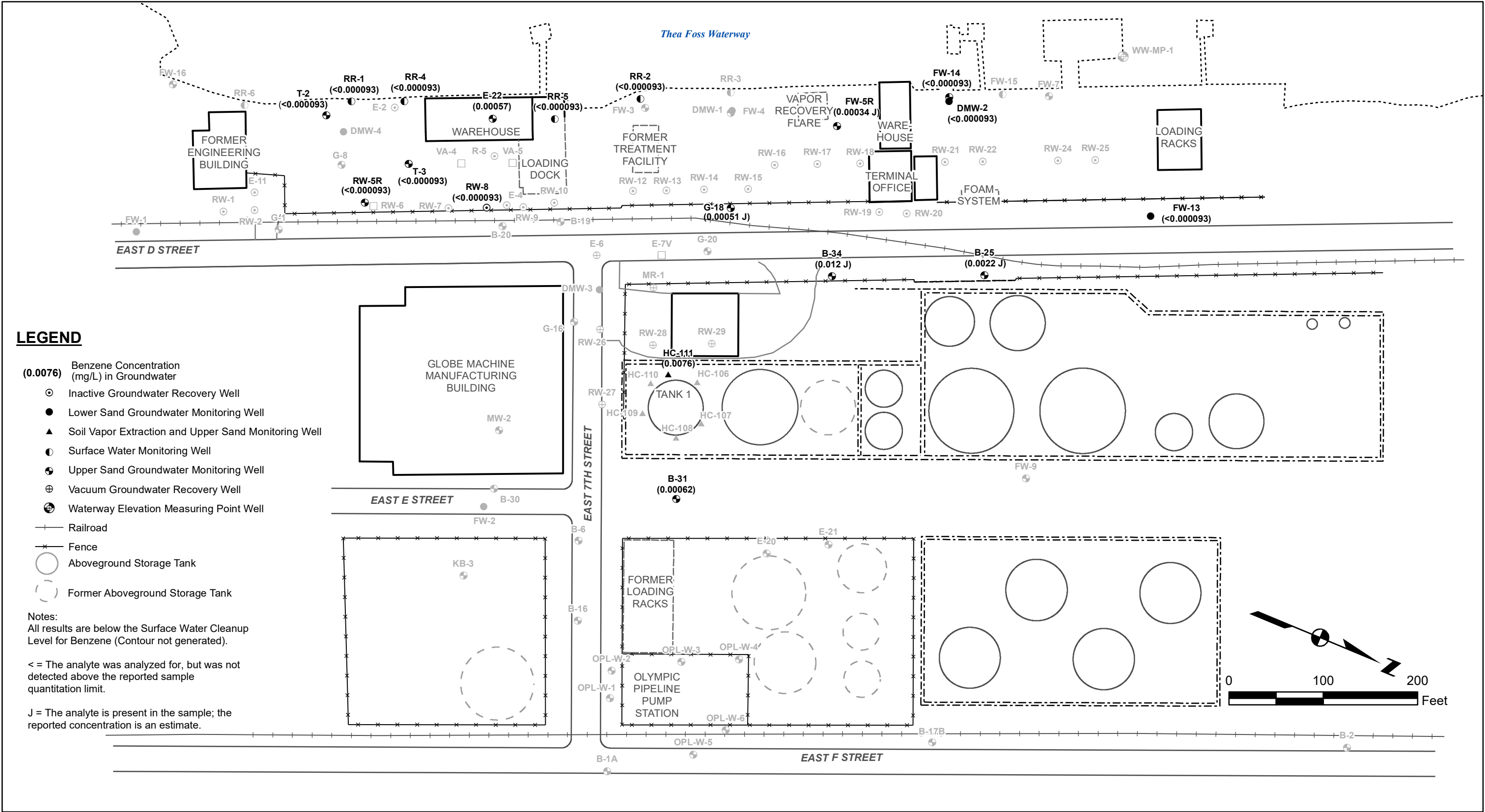
BENZENE CONCENTRATIONS IN GROUNDWATER (UPPER SAND UNIT), MAY 2024
