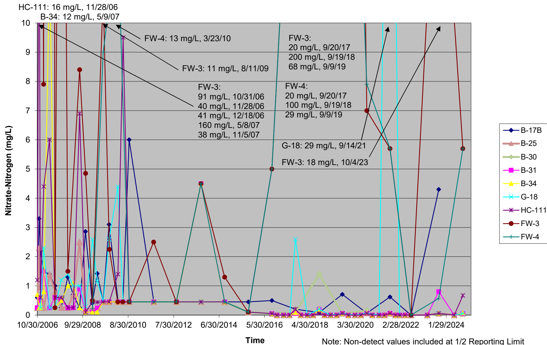
Graph 8 Nitrate-Nitrogen Time Series - HC-111 Plume
