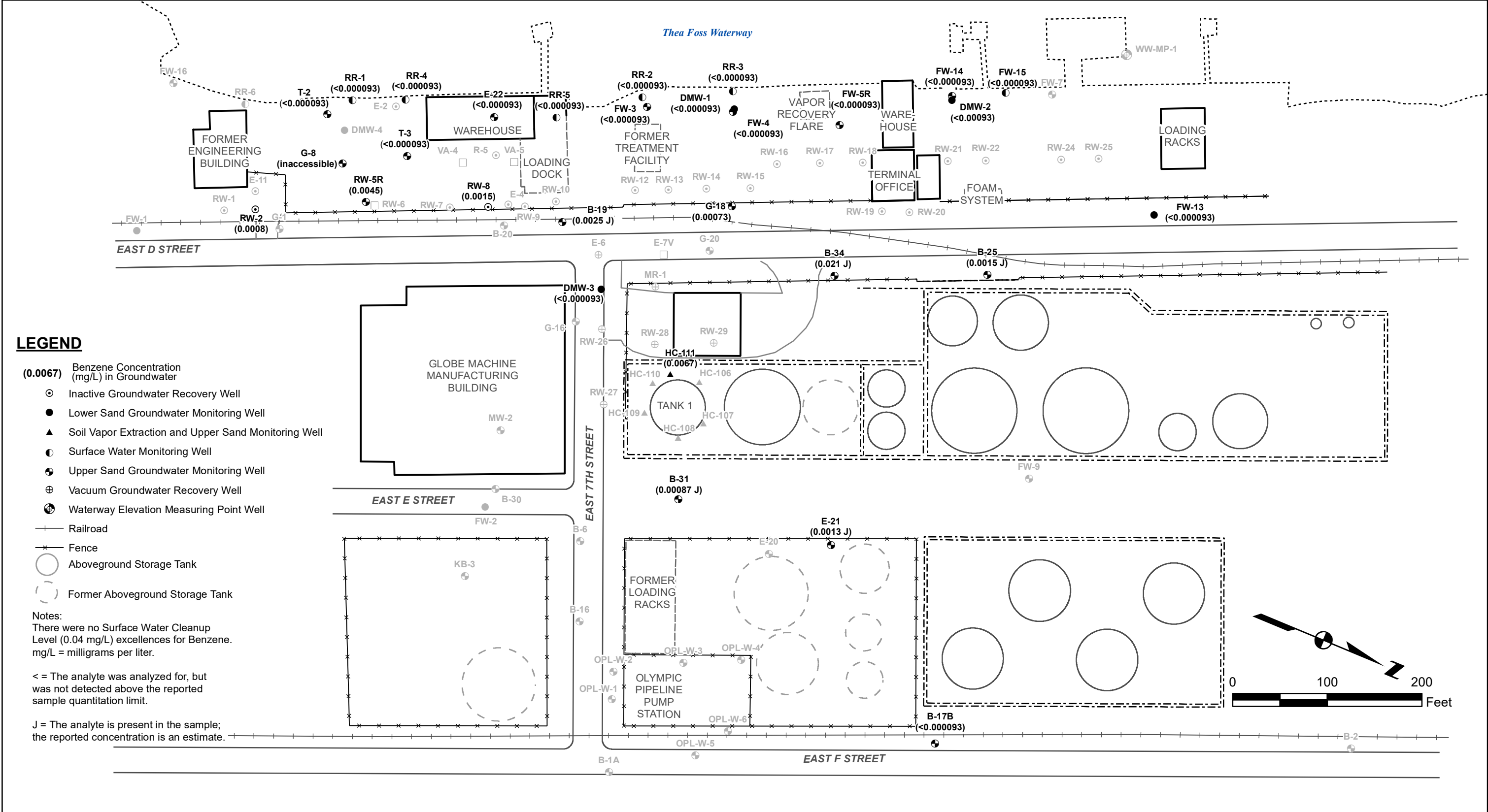
Source: Landau Associates, 2009. Maul Foster & Alongi, Inc. 2002. USGS, 2009. BENZENE CONCENTRATIONS IN GROUNDWATER (UPPER SAND UNIT), OCTOBER 2024
