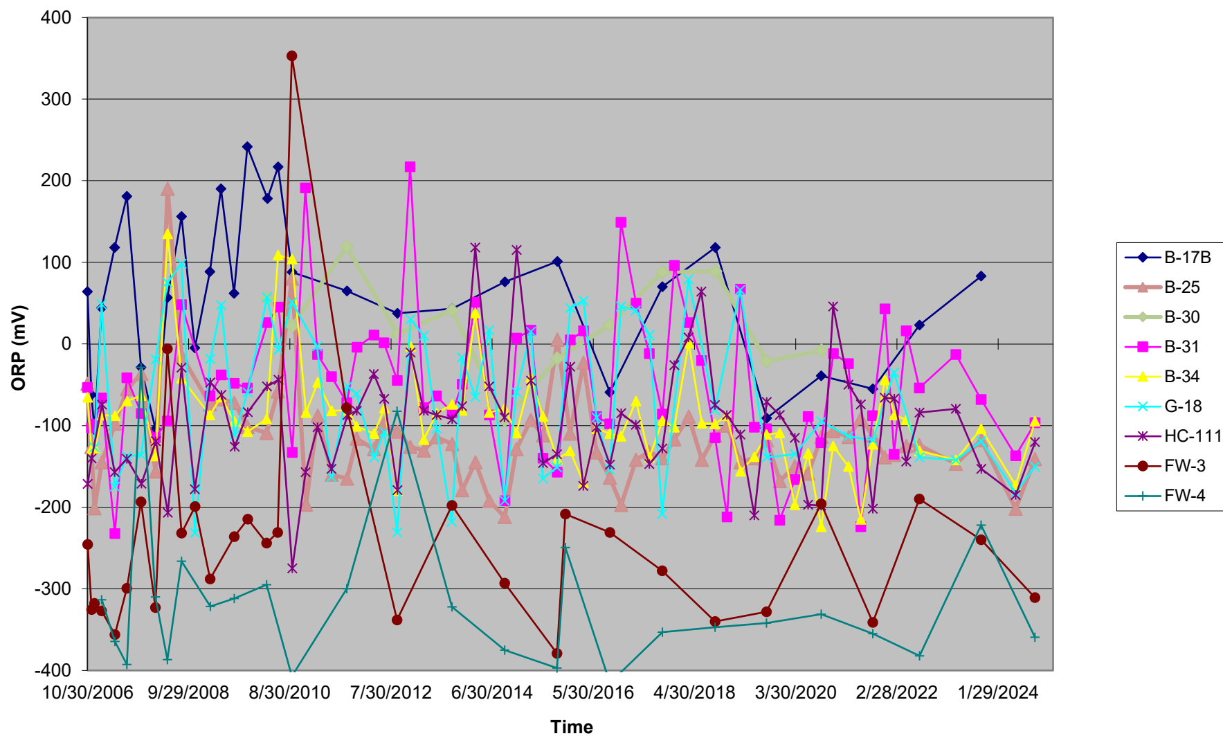
Graph 6 ORP Time Series - HC-111 Plume
