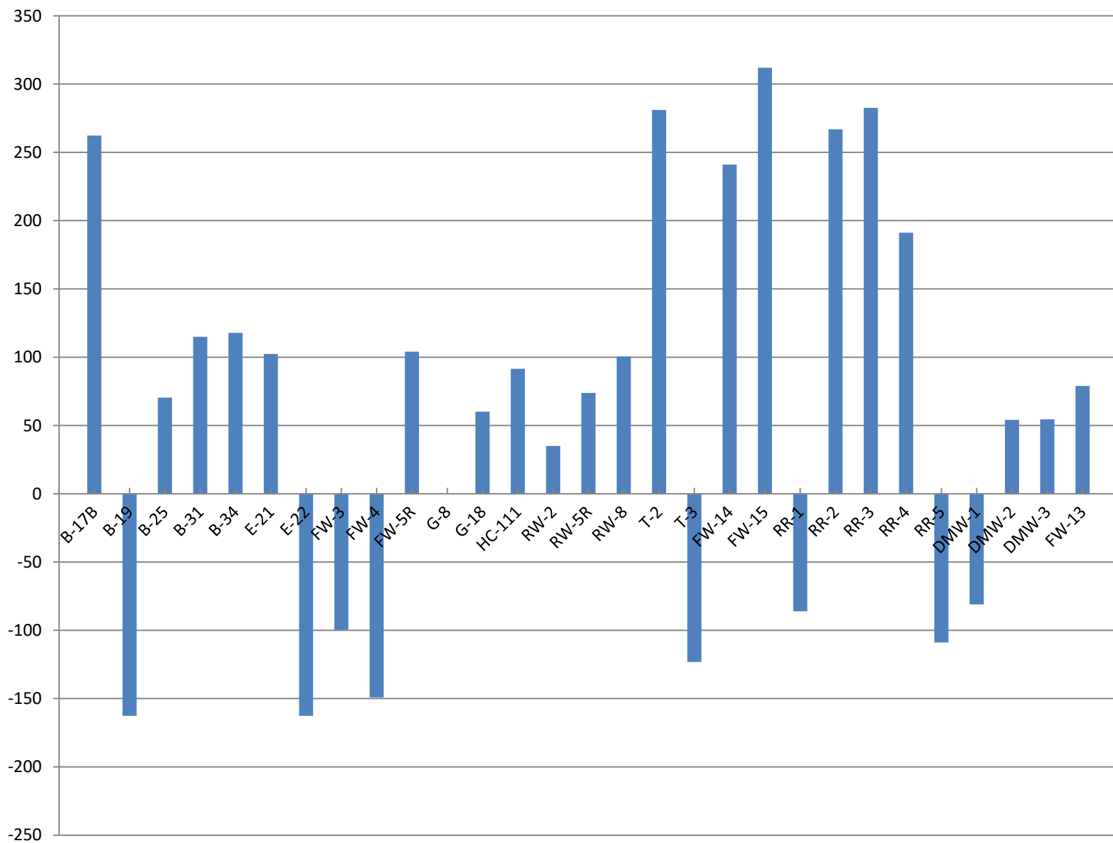
Graph 17 Summary of Redox Values ( E_H , in mV), October 2024
