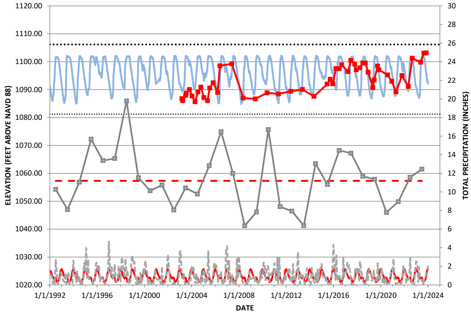
Groundwater Elevation Hydrograph: Monitoring Well MW-23
