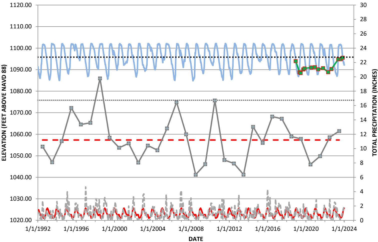
Groundwater Elevation Hydrograph: Monitoring Well RW-1
