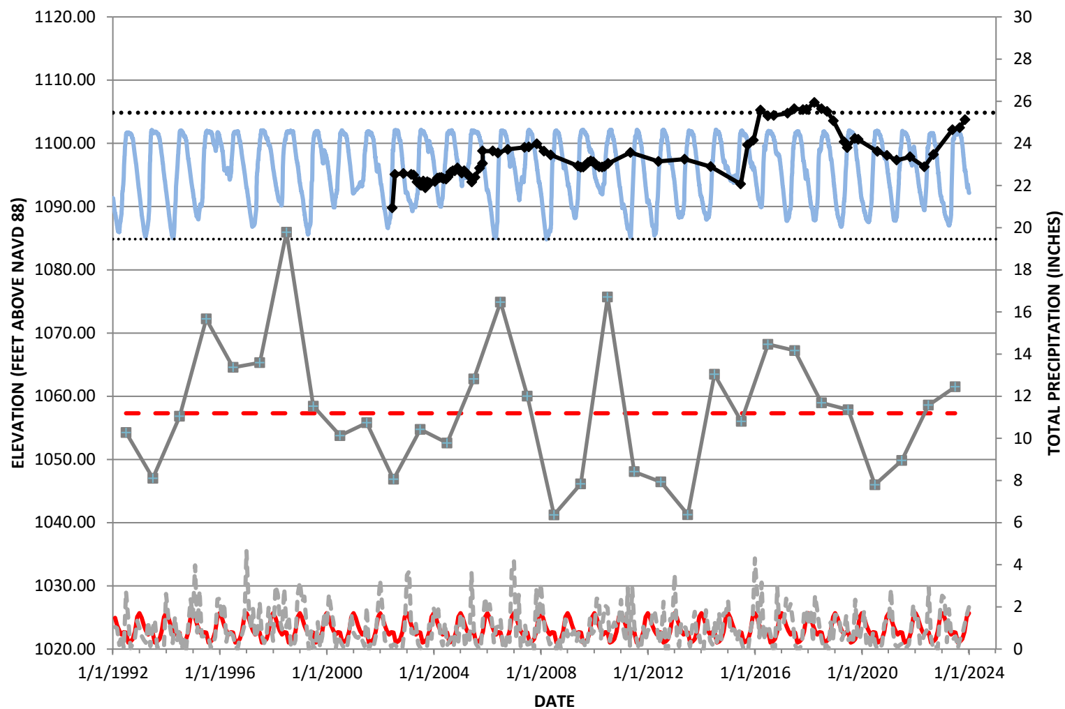
Groundwater Elevation Hydrograph: Monitoring Well MW-18
