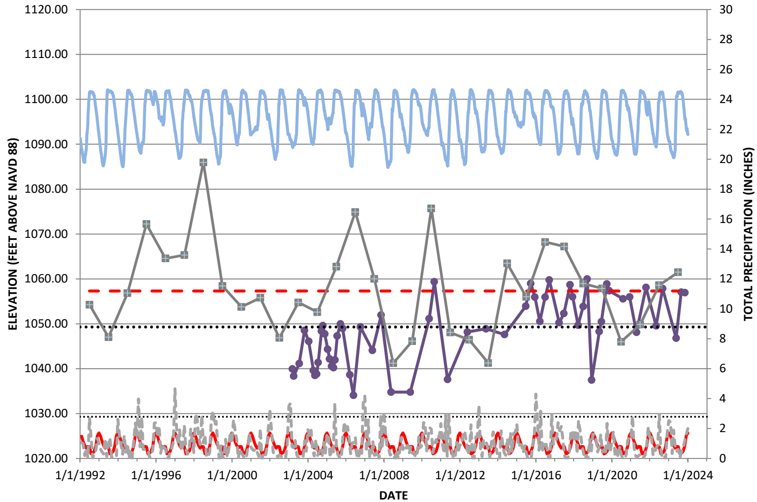
Groundwater Elevation Hydrograph: Monitoring Well MW-30
