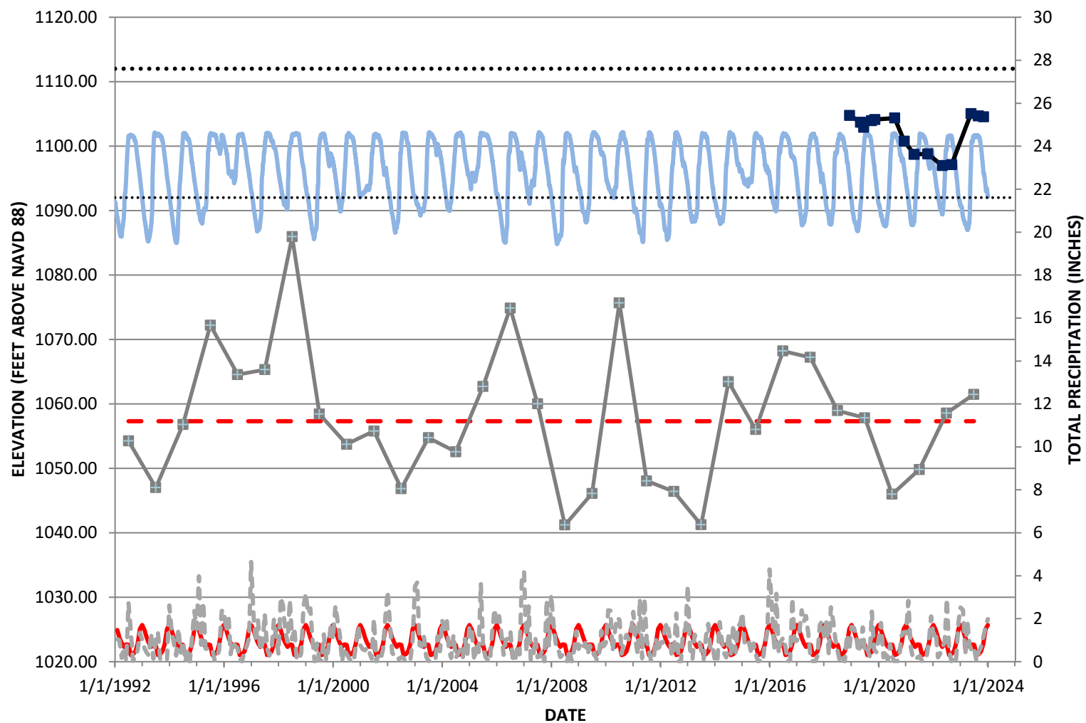
Groundwater Elevation Hydrograph: Monitoring Well MW-41
