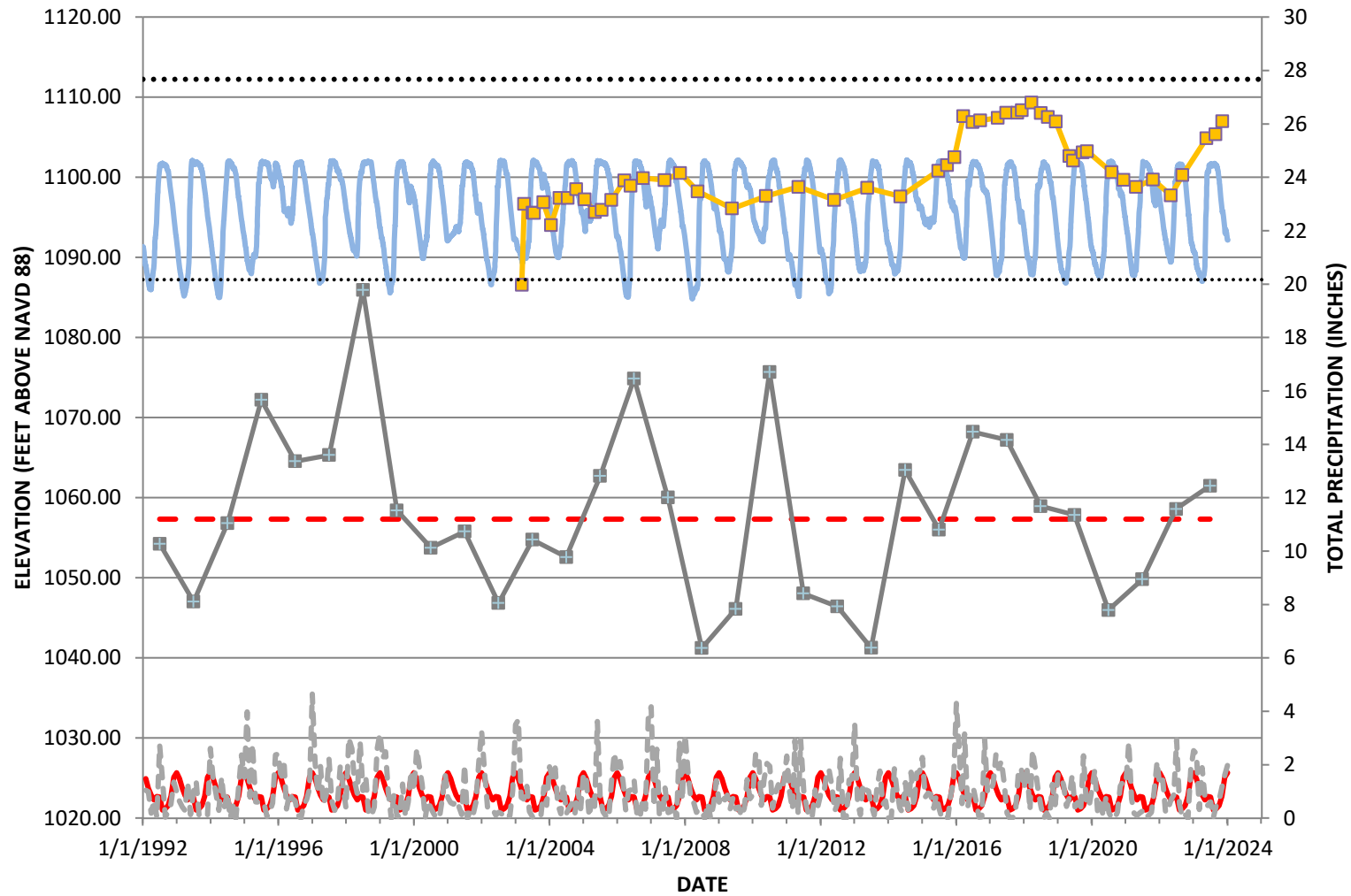
Groundwater Elevation Hydrograph: Monitoring Well MW-28
