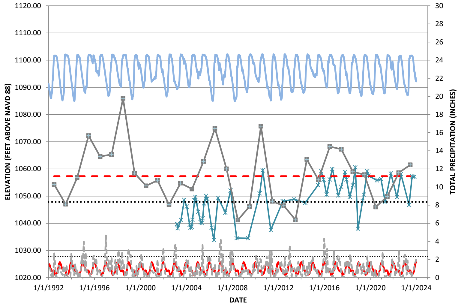
Groundwater Elevation Hydrograph: Monitoring Well MW-31
