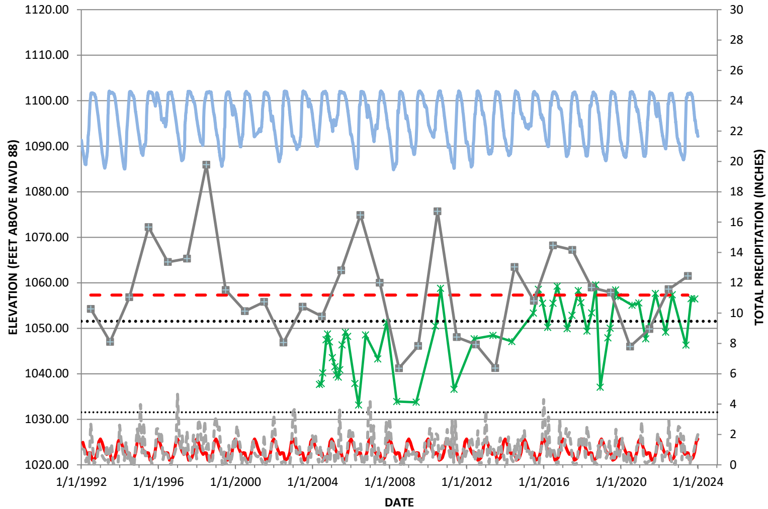
Groundwater Elevation Hydrograph: Monitoring Well MW-37
