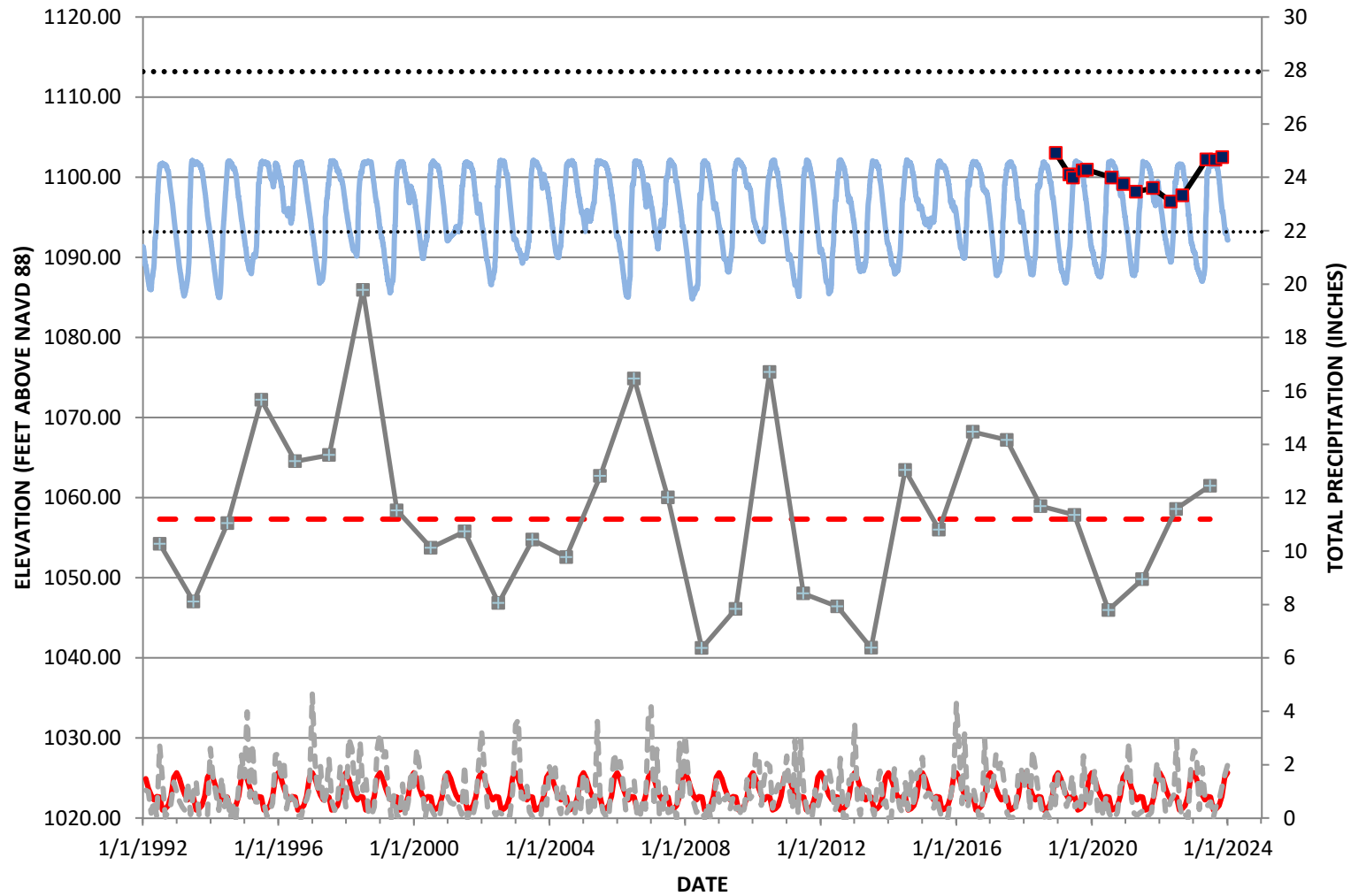
Groundwater Elevation Hydrograph: Monitoring Well MW-45
