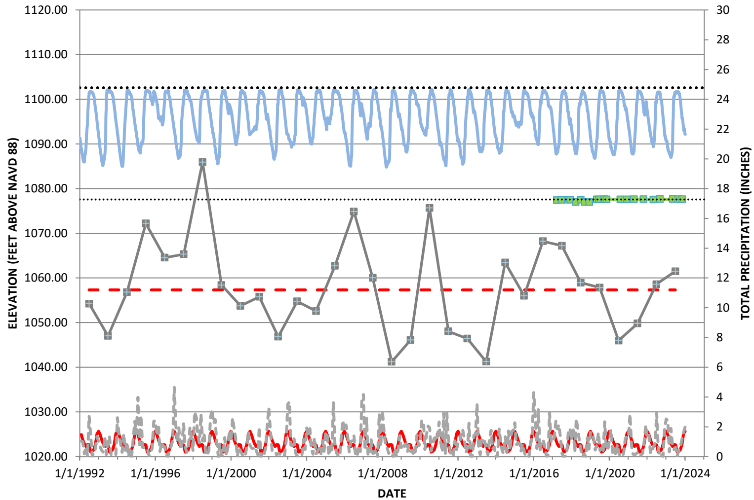
Groundwater Elevation Hydrograph: Monitoring Well MW-38
