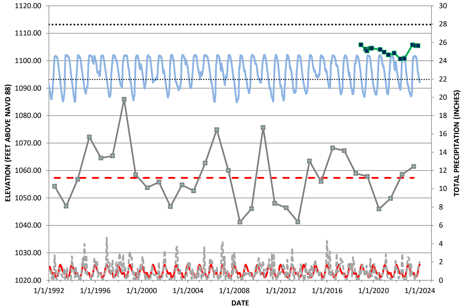
Groundwater Elevation Hydrograph: Monitoring Well MW-43
