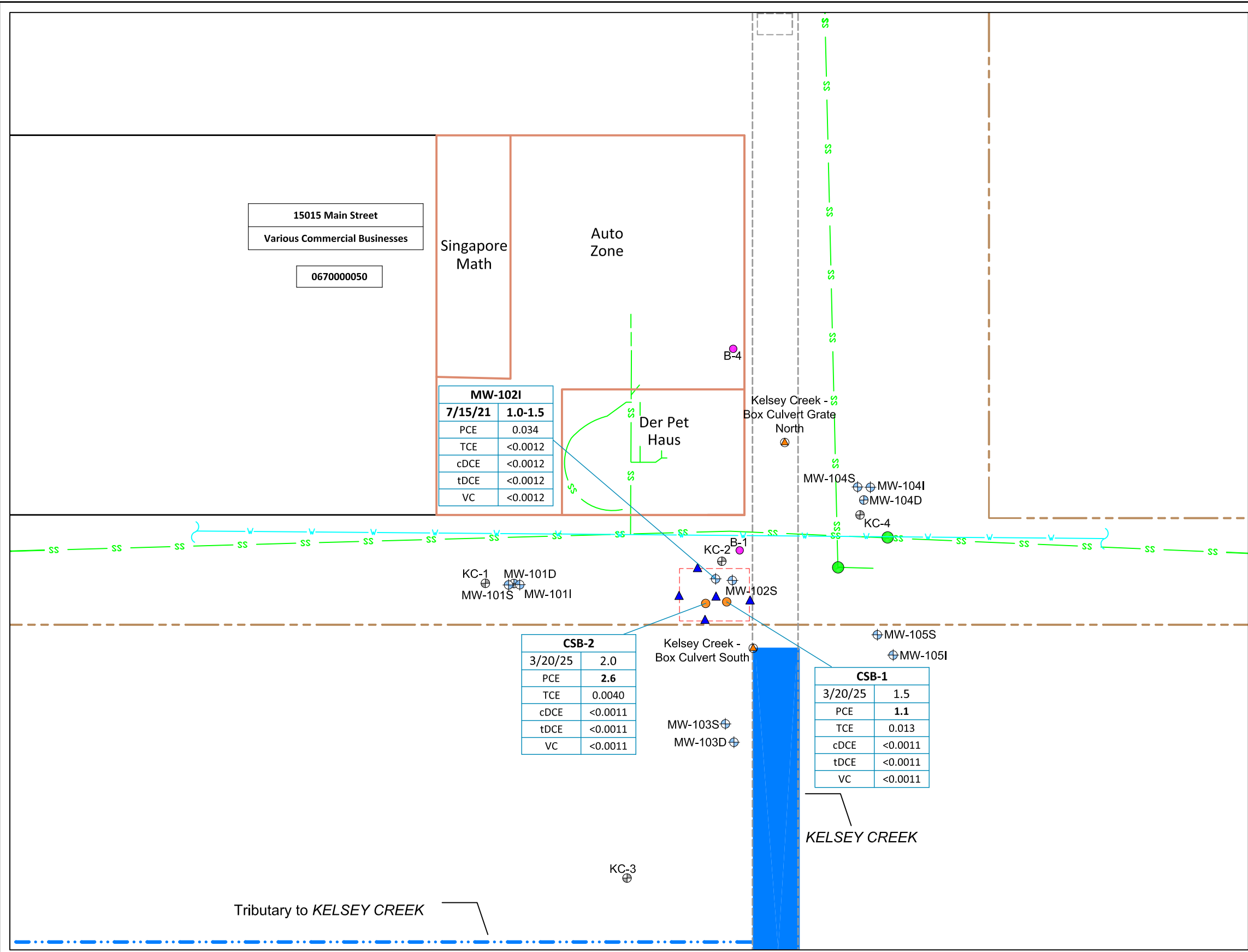
Figure 1 Site Plan
