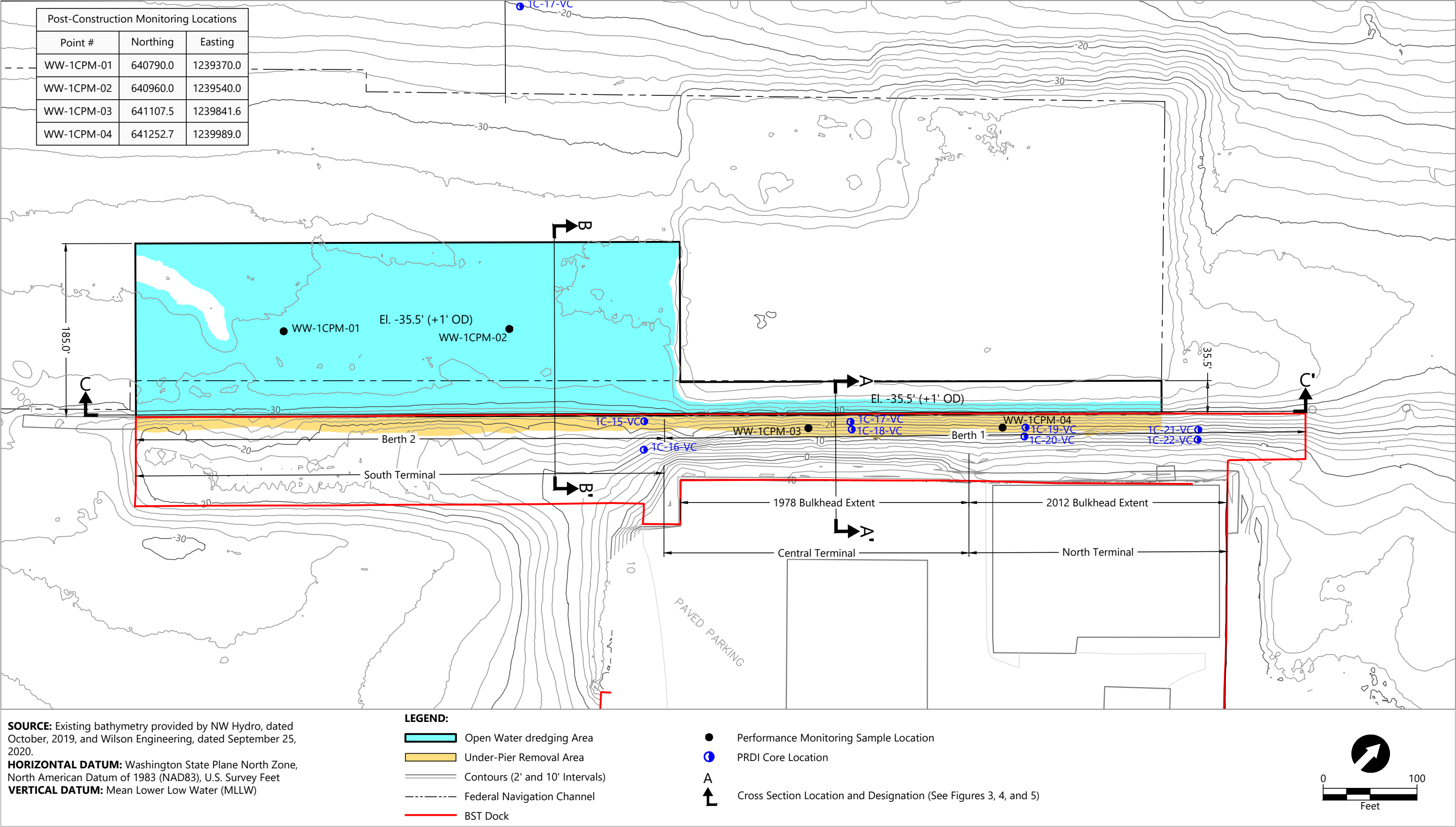
Figure 2 Unit 1C Dredging - Plan View EDR for Unit 1C Dredging Whatcom Waterway Cleanup
