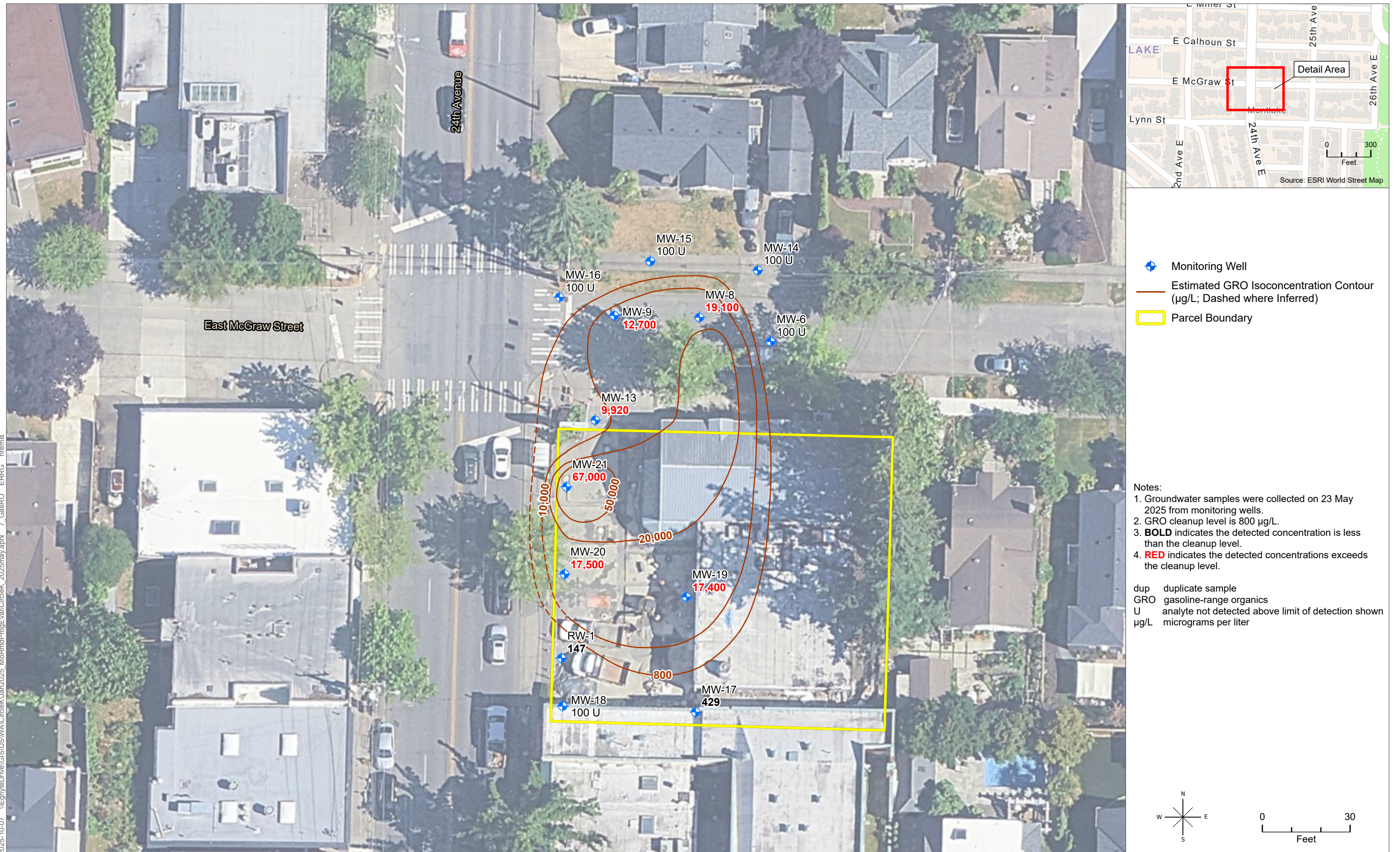
Figure 7. Groundwater Gasoline-Range Organics Contours, May 2025 Second Quarter 2025 Remedial Progress Evaluation Report for Former Circle K 1461 Seattle, WA
