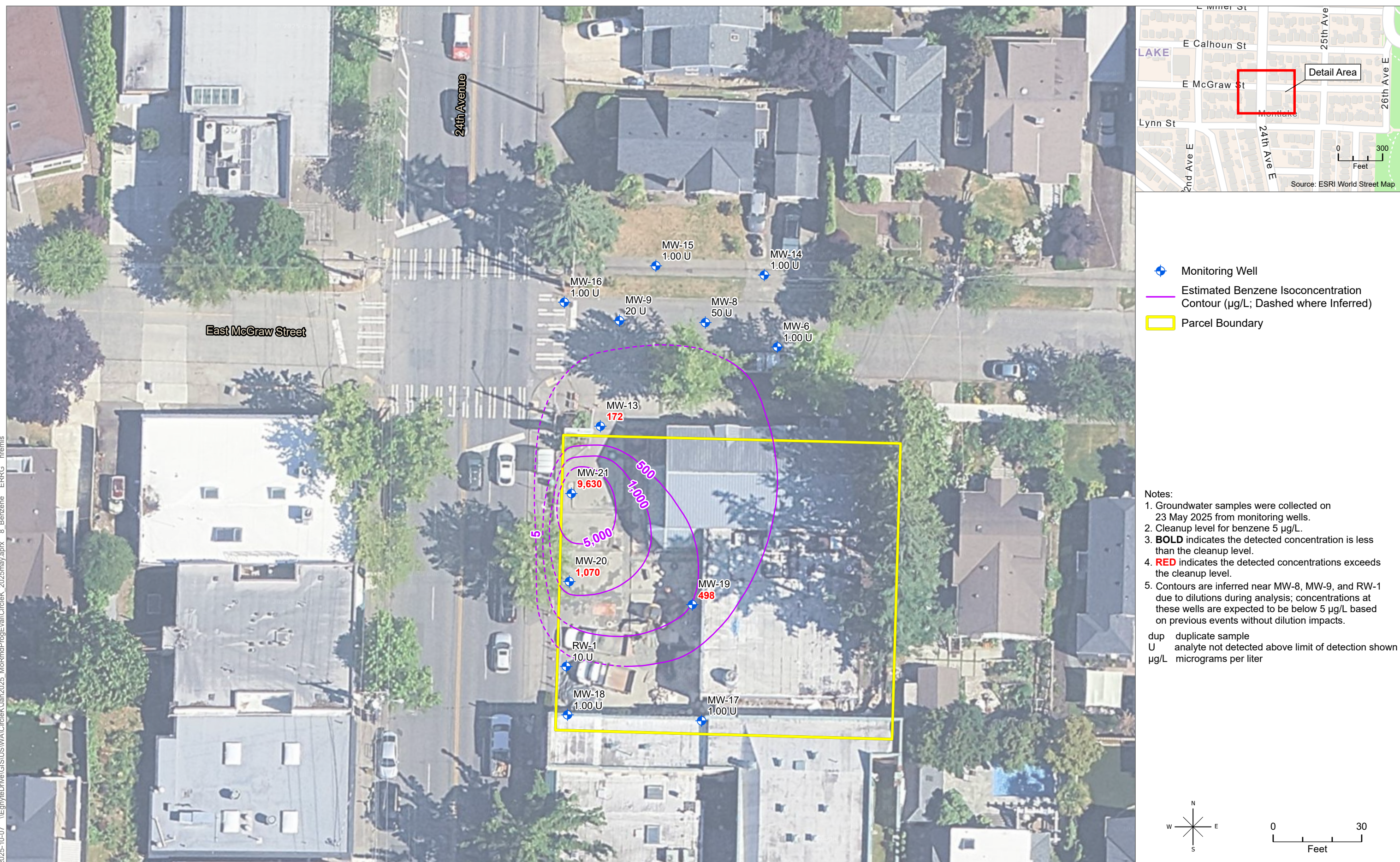
Figure 8. Groundwater Benzene Concentration Contours, May 2025 Second Quarter 2025 Remedial Progress Evaluation Report for Former Circle K 1461 Seattle, WA
