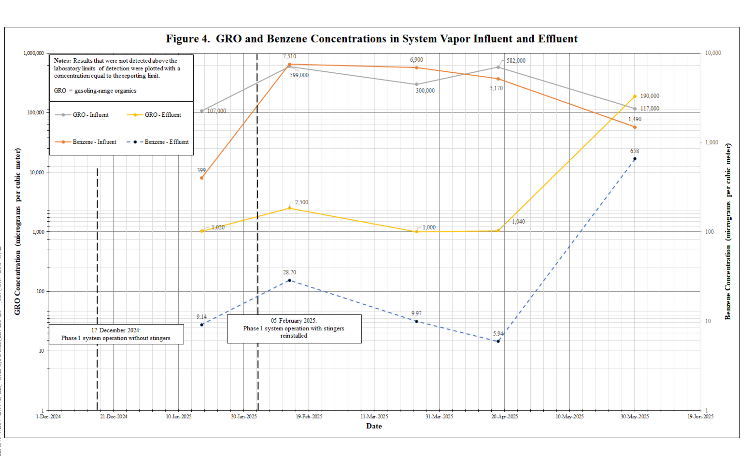
Figure 4. GRO and Benzene Concentrations in System Vapor Influent and Effluent Second Quarter 2025 Remedial Progress Evaluation Report for Former Circle K 1461 Seattle, WA
