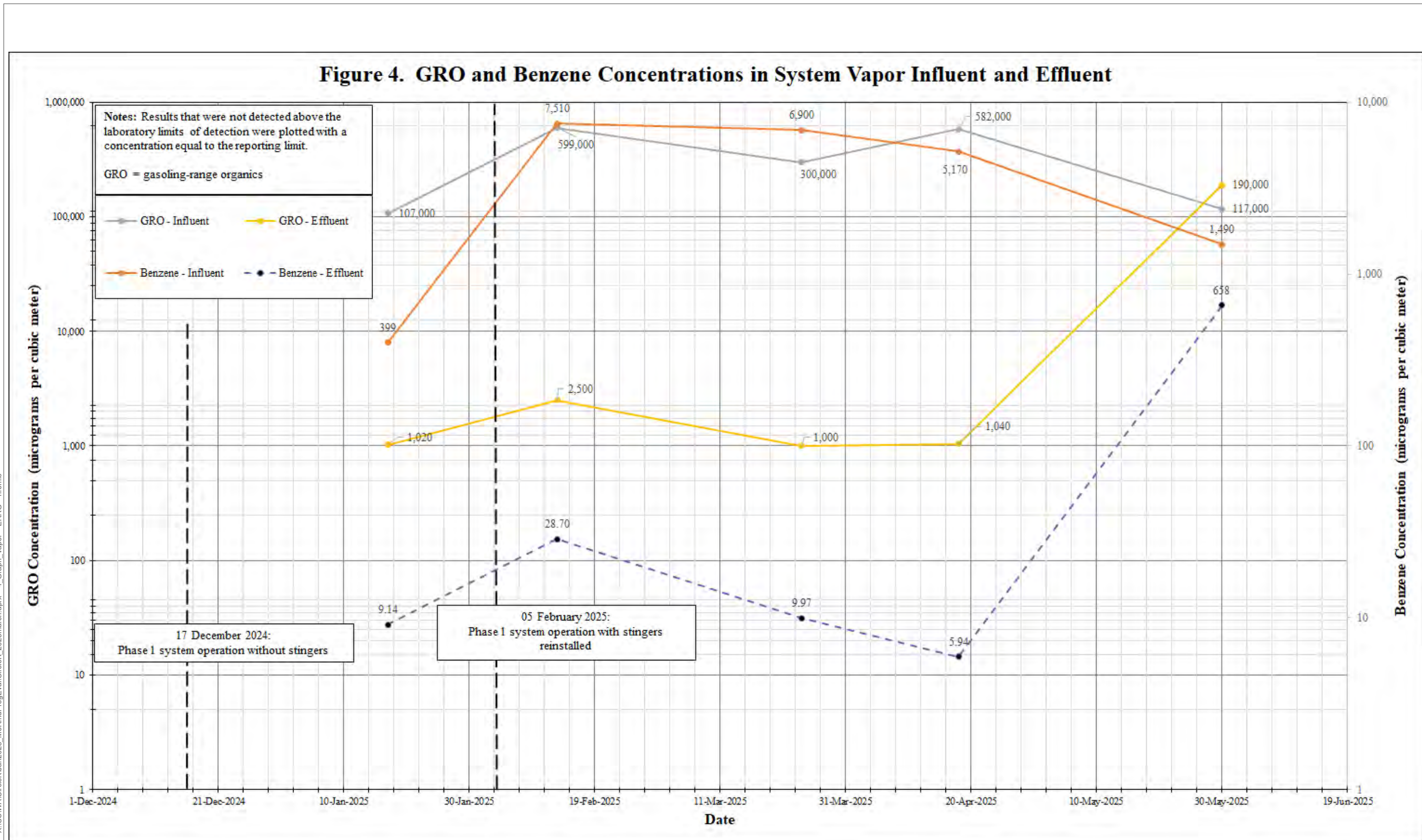
Figure 4. GRO and Benzene Concentrations in System Vapor Influent and Effluent Second Quarter 2025 Remedial Progress Evaluation Report for Former Circle K 1461 Seattle, WA
