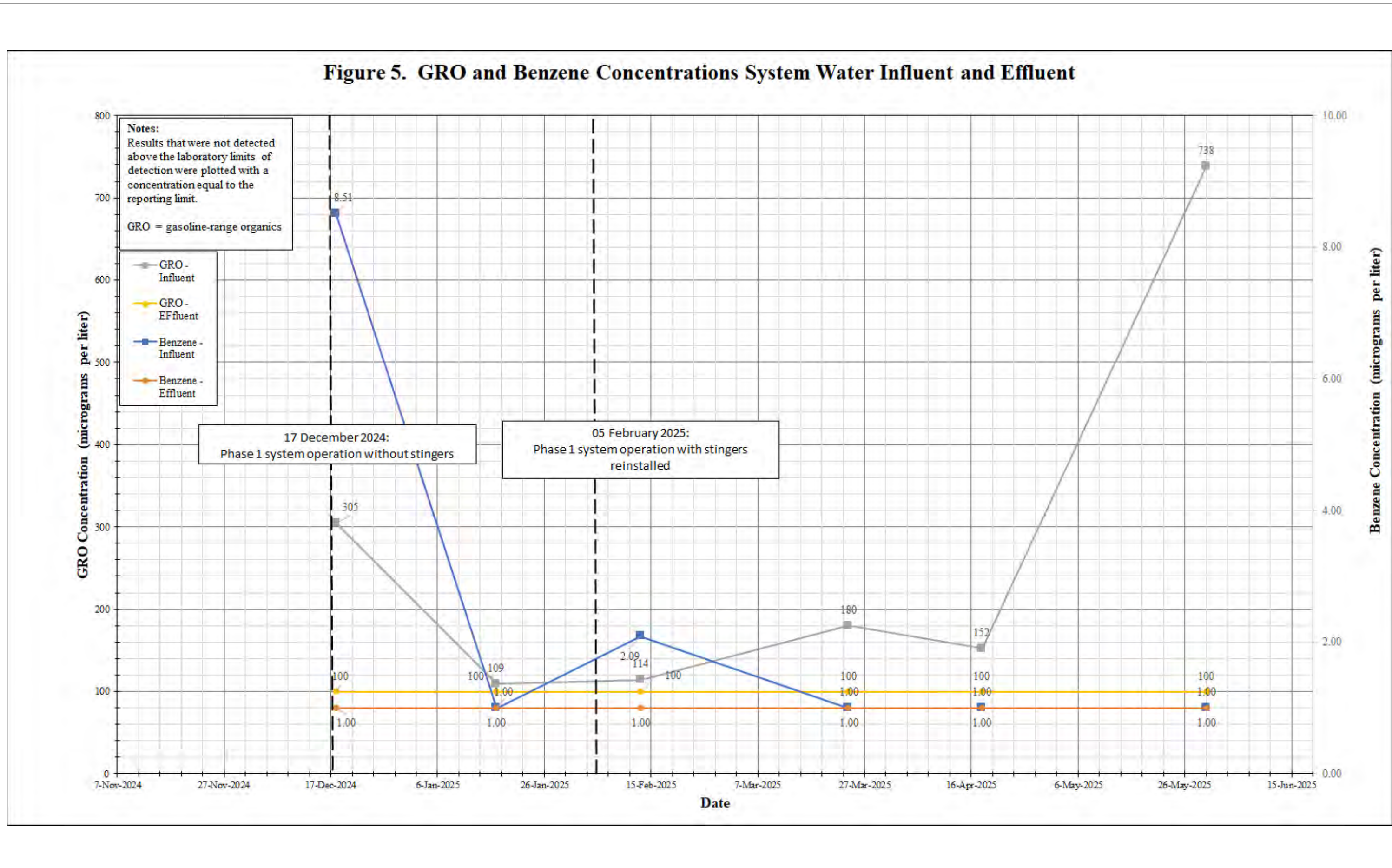
Figure 5. GRO and Benzene Concentrations in System Water Influent and Effluent Second Quarter 2025 Remedial Progress Evaluation Report for Former Circle K 1461 Seattle, WA
