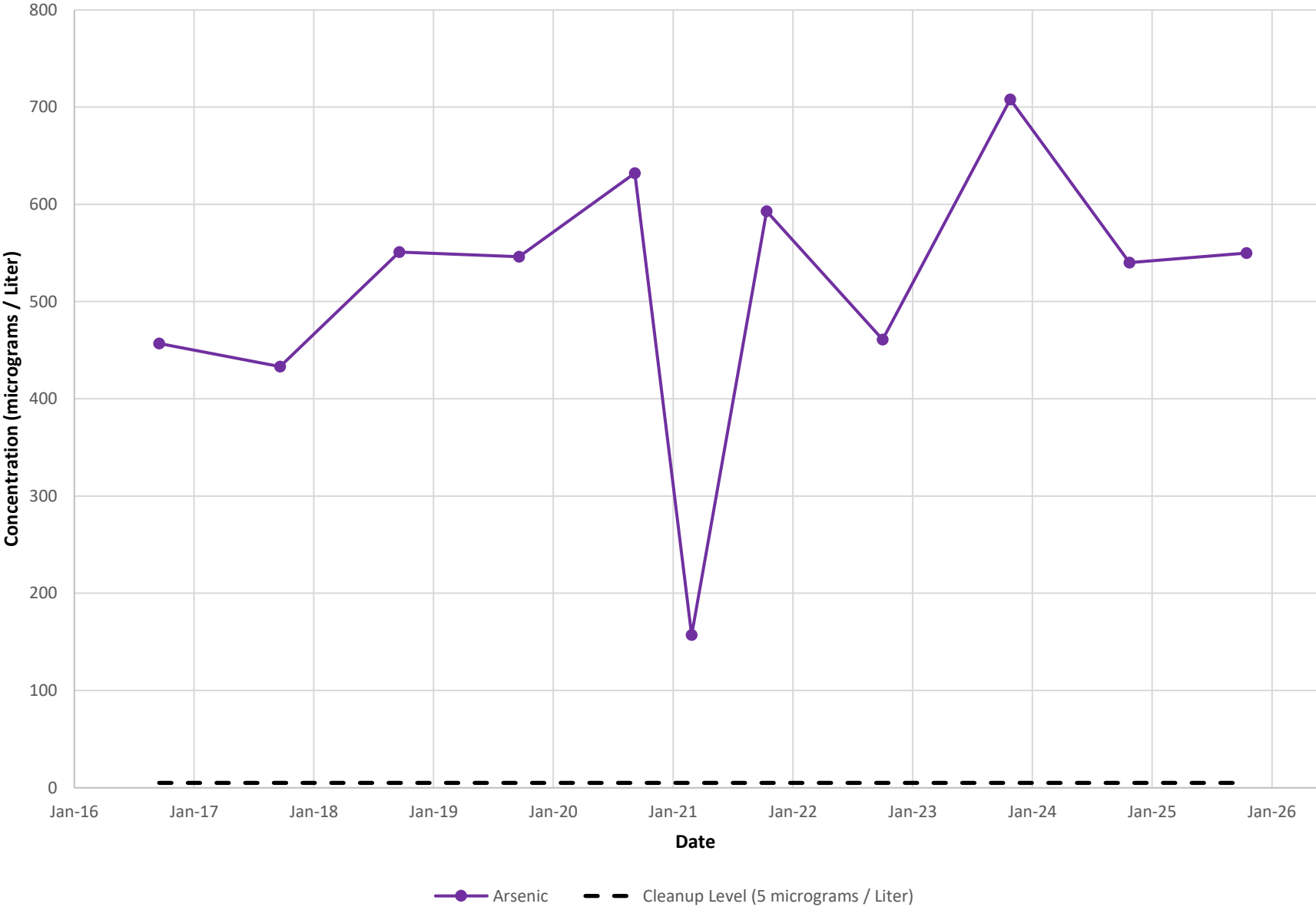
Figure 8 Groundwater Quality Trends for PZ-3A Arsenic Former Mill E / Koppers Facility Everett, Washington
