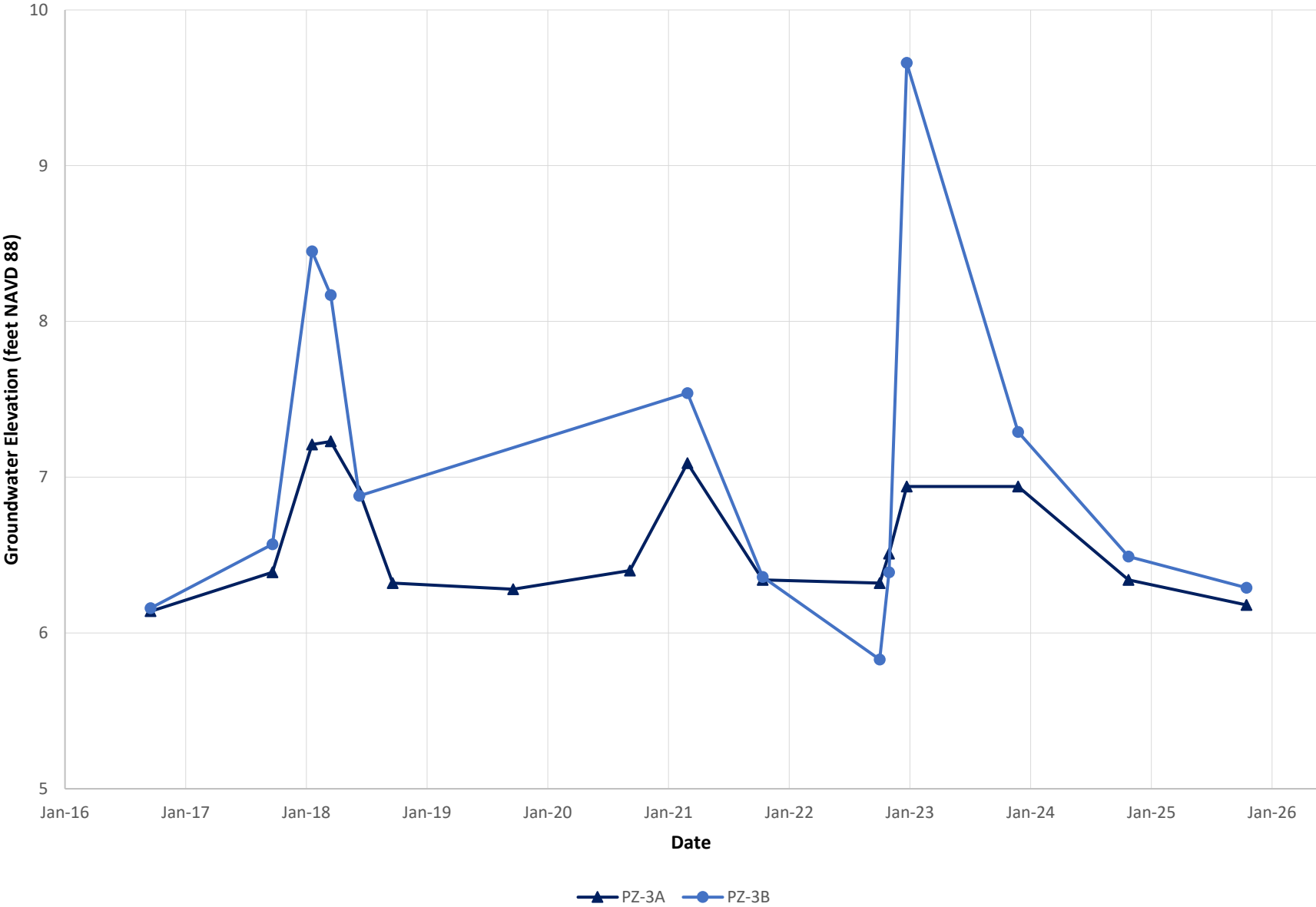
Figure 5 Groundwater Elevation Trends PZ-3A and PZ-3B Former Mill E / Koppers Facility Everett, Washington
