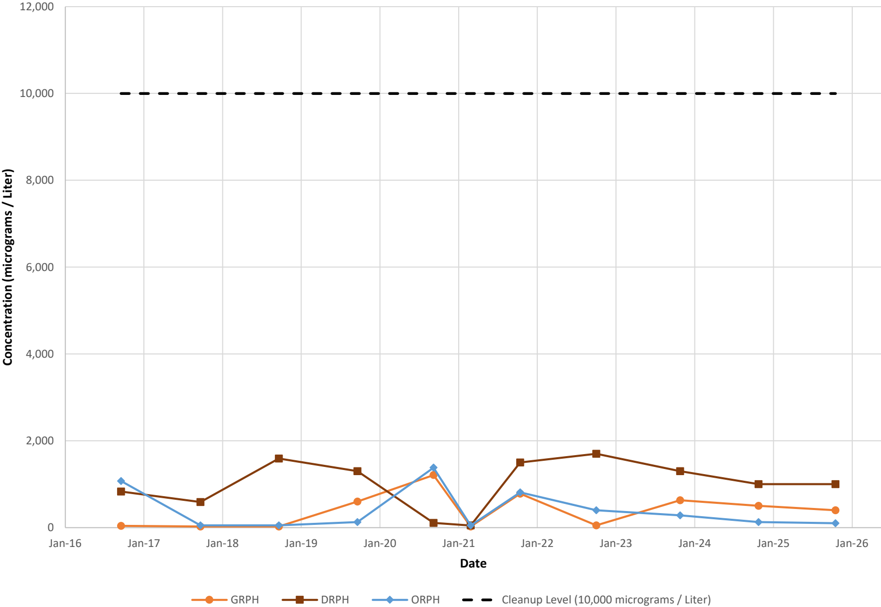
Figure 6 Groundwater Quality Trends for PZ-3A Total Petroleum Hydrocarbons Former Mill E / Koppers Facility Everett, Washington
