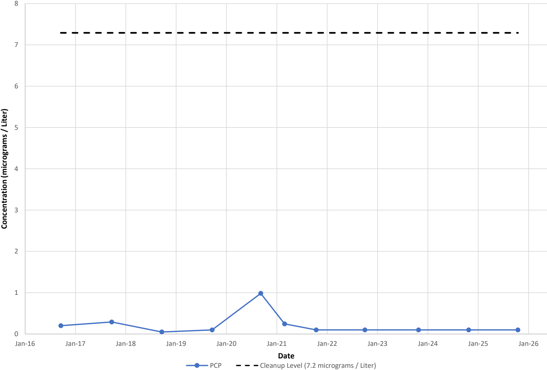
Figure 7 Groundwater Quality Trends for PZ-3A Pentachlorophenol Former Mill E / Koppers Facility Everett, Washington
