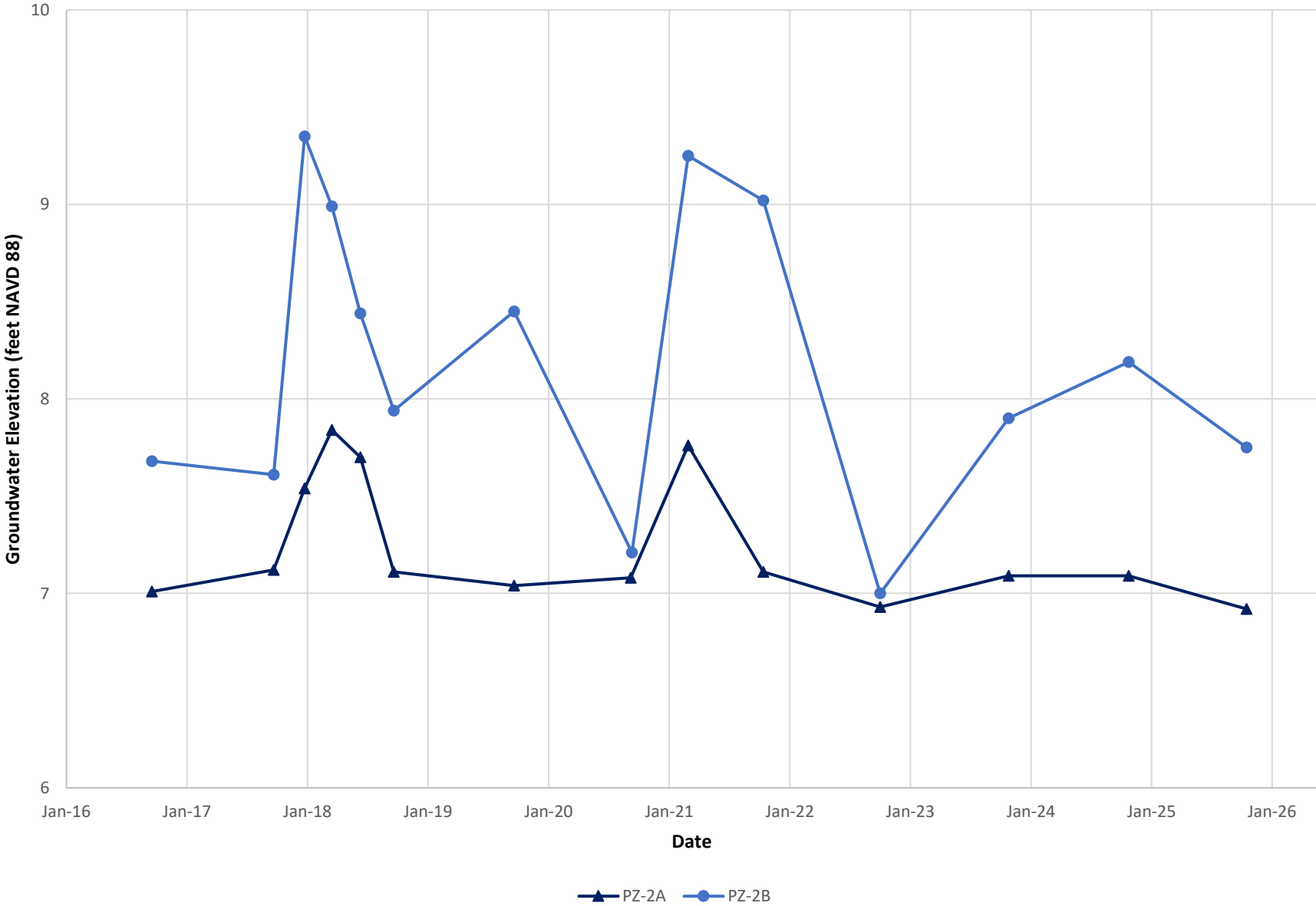
Figure 4 Groundwater Elevation Trends PZ-2A and PZ-2B Former Mill E / Koppers Facility Everett, Washington
