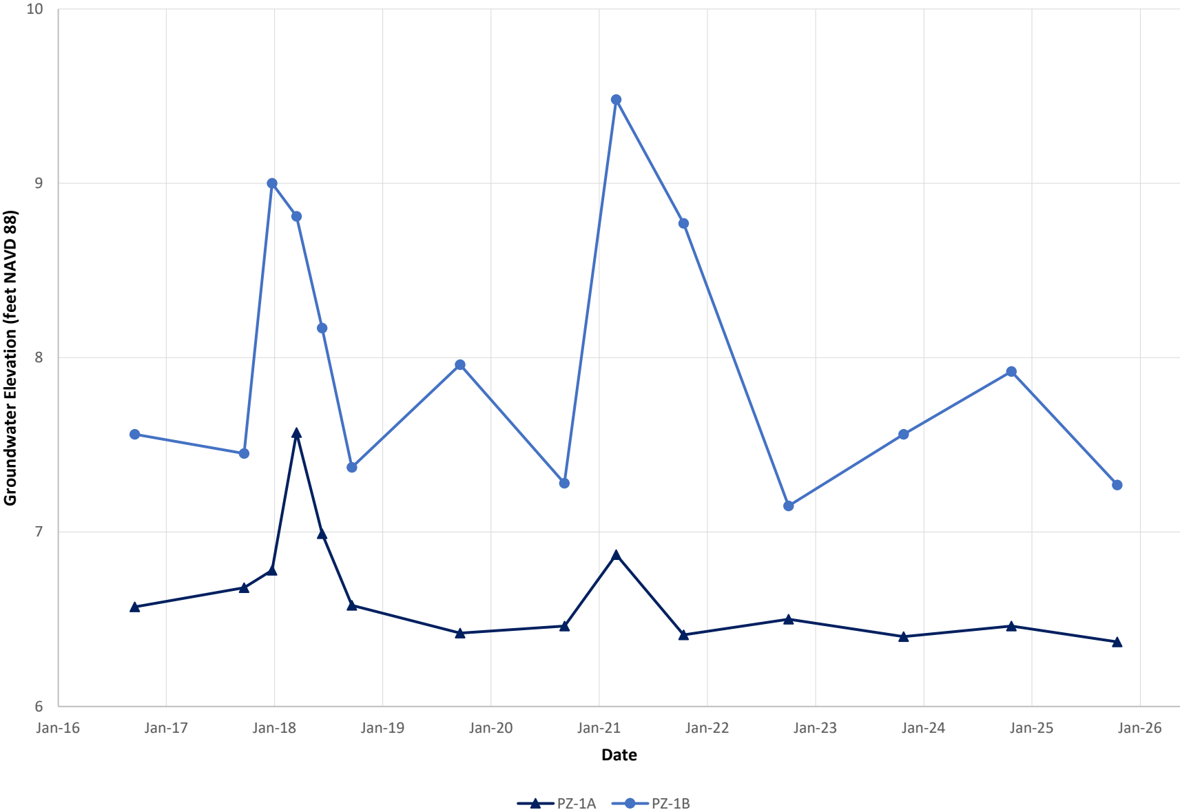
Figure 3 Groundwater Elevation Trends PZ-1A and PZ-1B Former Mill E / Koppers Facility Everett, Washington
