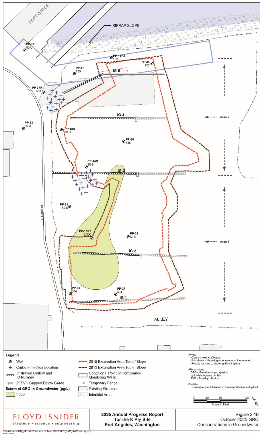
Figure 8. GRO in Groundwater – October 2025 (Floyd|Snider 2026)
