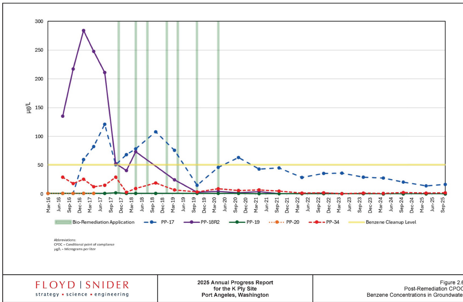
Figure 15: Post-Remediation Benzene Concentrations in Groundwater (Floyd|Snider 2026)
