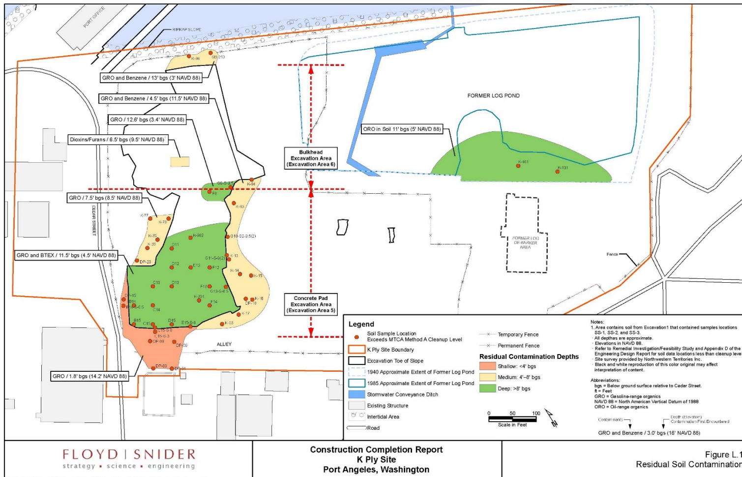
Figure 2: Site Plan (Floyd|Snider 2016)
