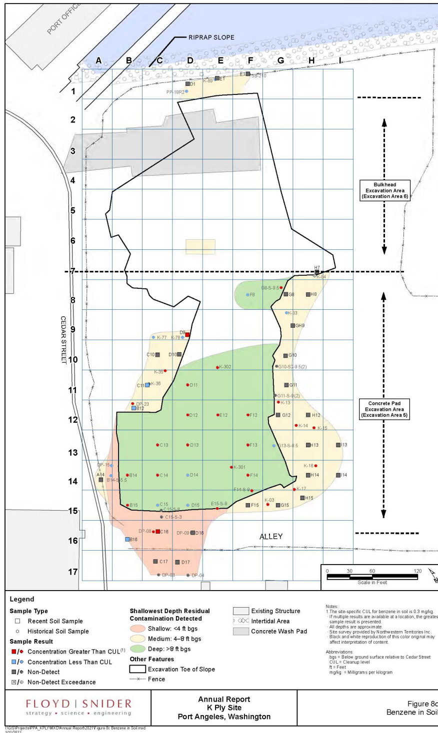
Figure 6: Benzene in soil – Results of 5-year soil monitoring (Floyd|Snider 2022)
