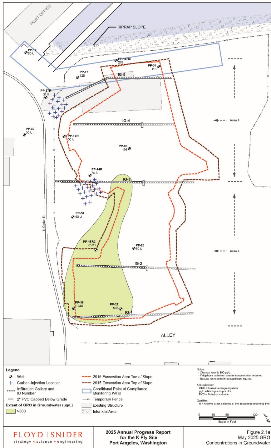
Figure 7: GRO in Groundwater – May 2025 (Floyd|Snider 2026)
