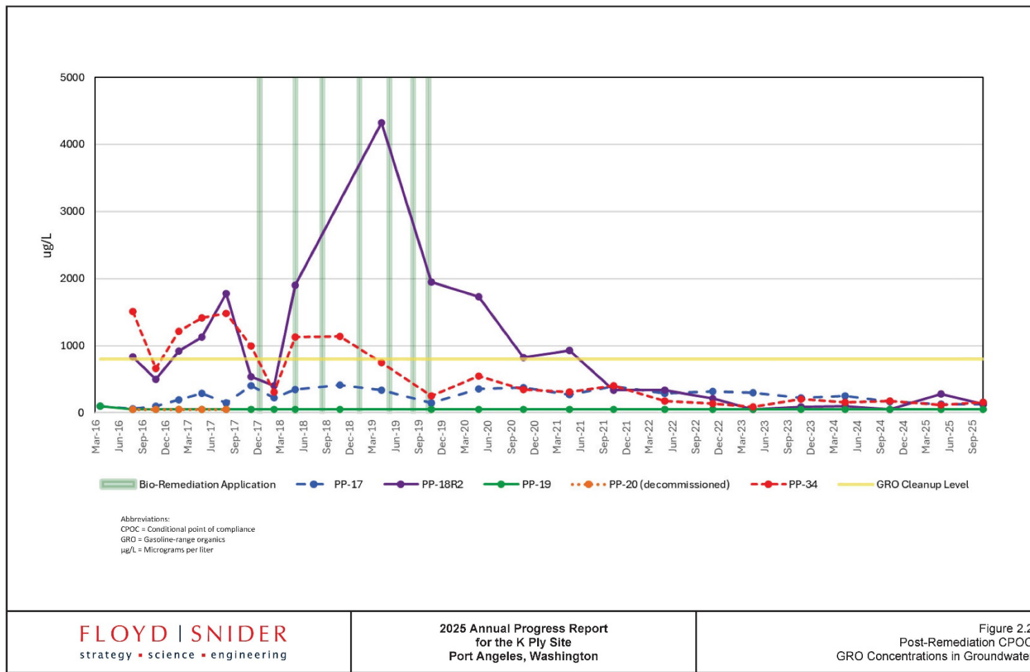
Figure 13: Post-Remediation GRO Concentrations in Groundwater (Floyd|Snider 2026)
