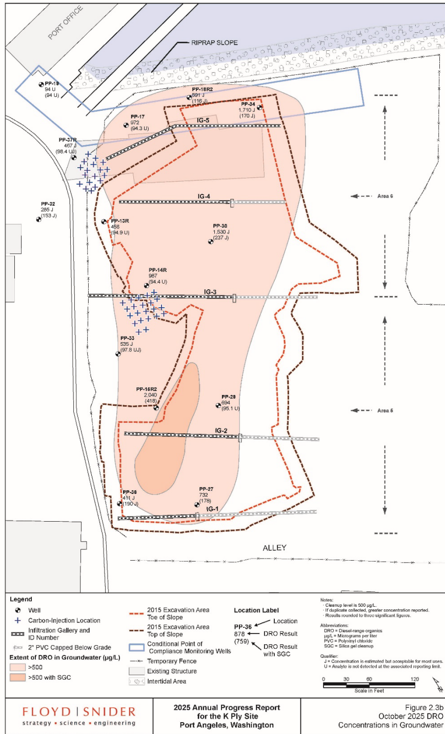
Figure 10: DRO in Groundwater – October 2025 (Floyd|Snider 2026)
