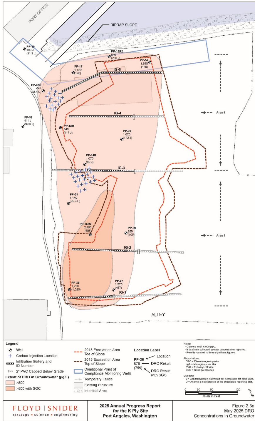
Figure 9: DRO in Groundwater – May 2025 (Floyd|Snider 2026)
