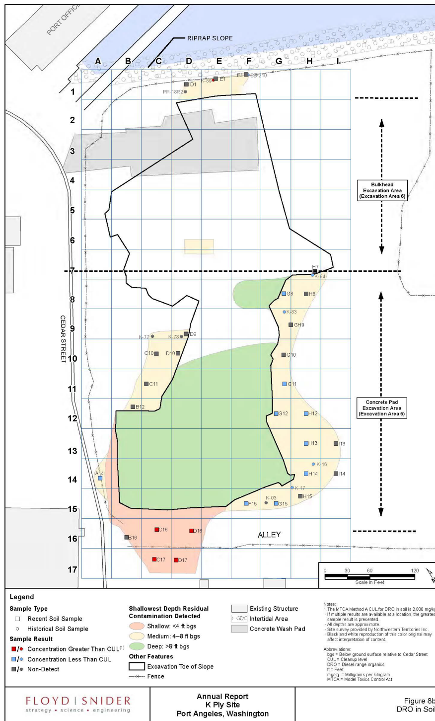
Figure 5: DRO in soil – Results of 5-year soil monitoring (Floyd|Snider 2022)
