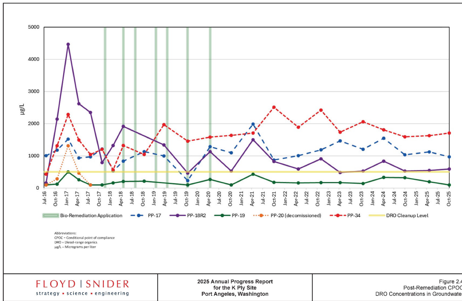
Figure 14: Post-Remediation DRO Concentrations in Groundwater (Floyd|Snider 2026)
