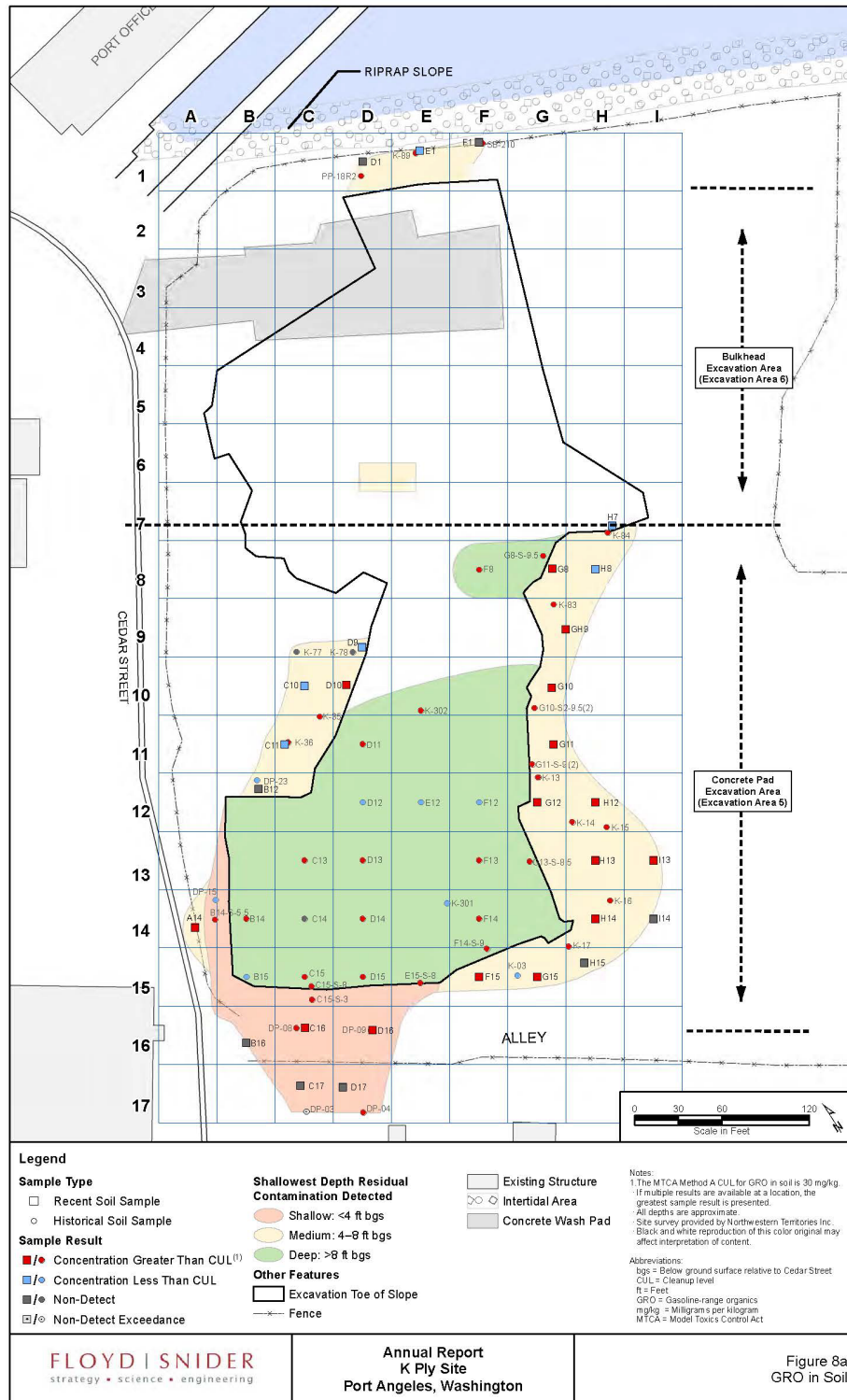
Figure 4: GRO in soil – Results of 5-year soil monitoring (Floyd|Snider 2022)
