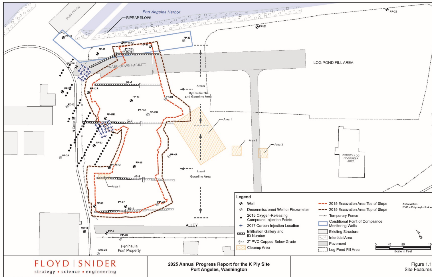
Figure 1: Site Features (Floyd|Snider 2026)
