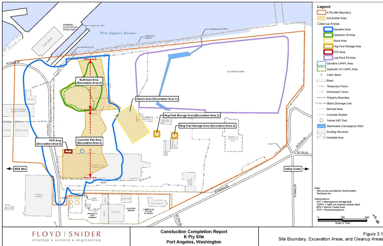
Figure 3: Site Boundary, Excavation Areas, and Cleanup Areas (Floyd|Snider 2016)
