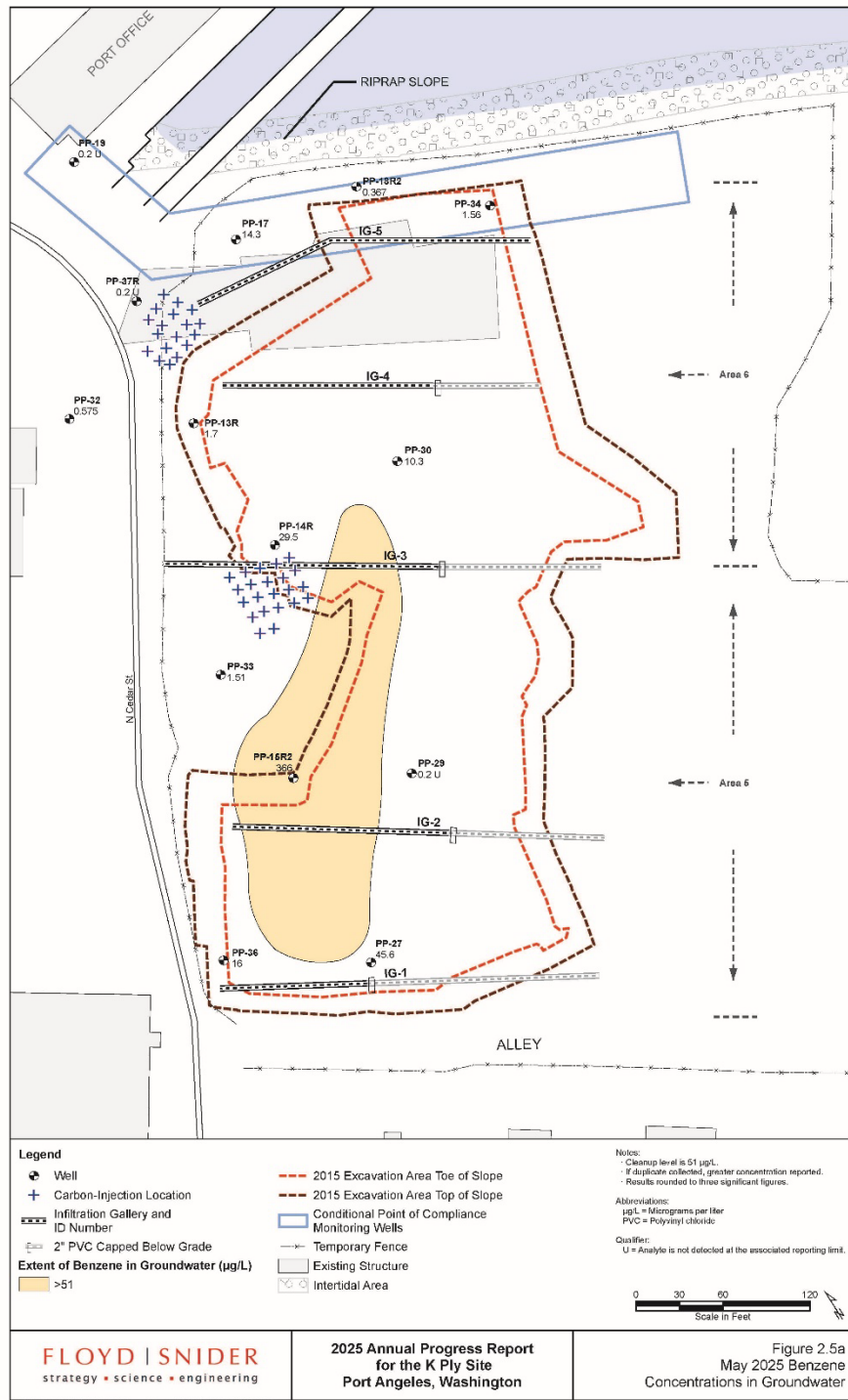
Figure 11: Benzene in Groundwater – May 2025 (Floyd|Snider 2026)
