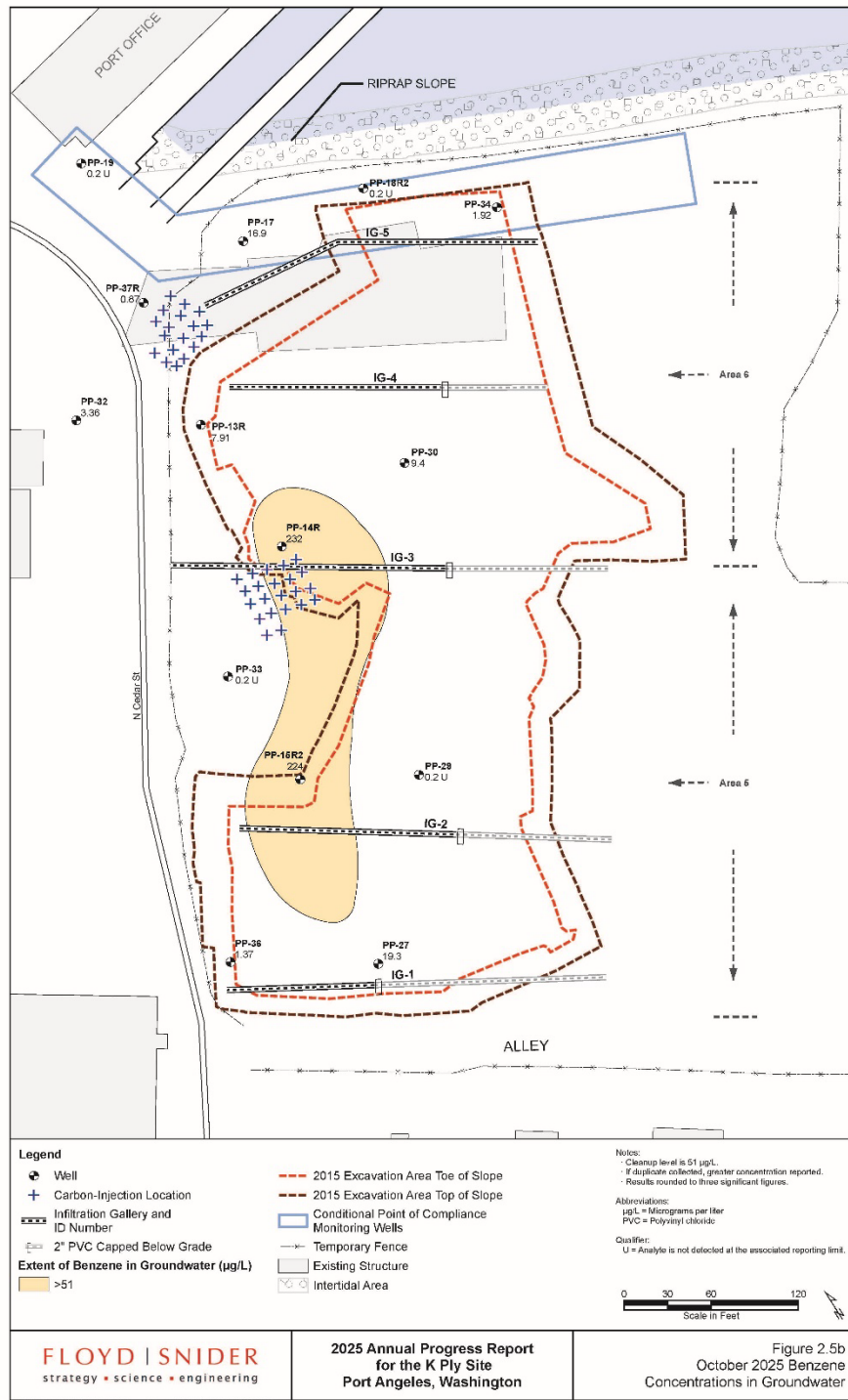
Figure 12: Benzene in Groundwater – October 2025 (Floyd|Snider 2026)
