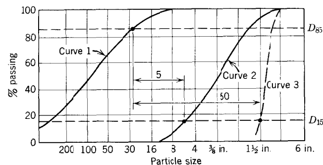
FIG. 5.6 Segregated filter materials also cause problems. D_{15} of unsegregated filter aggregate (curve 2) is five times D_{85} of soil (curve 1), but D_{15} of segregated pockets of coarse filter material (curve 3) is fifty times D_{85} of soil.
