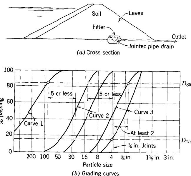
FIG. 5.3 Design of graded filter to protect soil (curve 1) from washing into \frac{1}{4} in. joints in drain pipe [fine material (curve 2) adjacent to soil; coarse material (curve 3) surrounds pipe].
