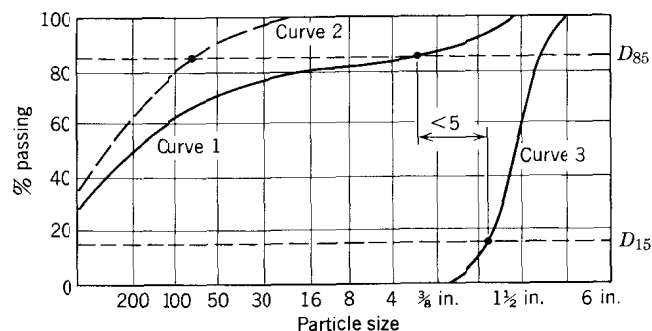
FIG. 5.5 Problems are caused by gap-graded soils. D_{15} size of filter (curve 3) is less than five times D_{85} size of rocky or gravelly soil (curve 1), but fine soil matrix (curve 2) may still migrate through filter.
