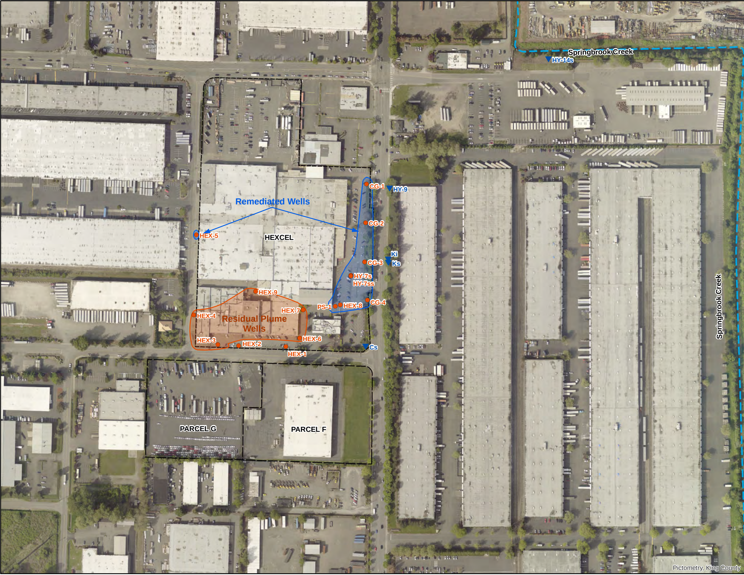
FIGURE 6 Compliance Monitoring Network
