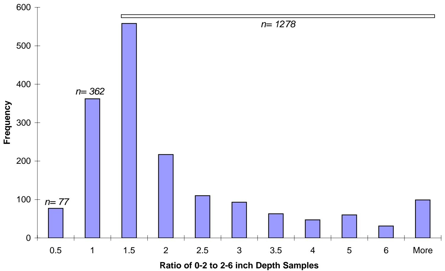
Figure 37 Histogram of Lead Depth Profile Ratios
