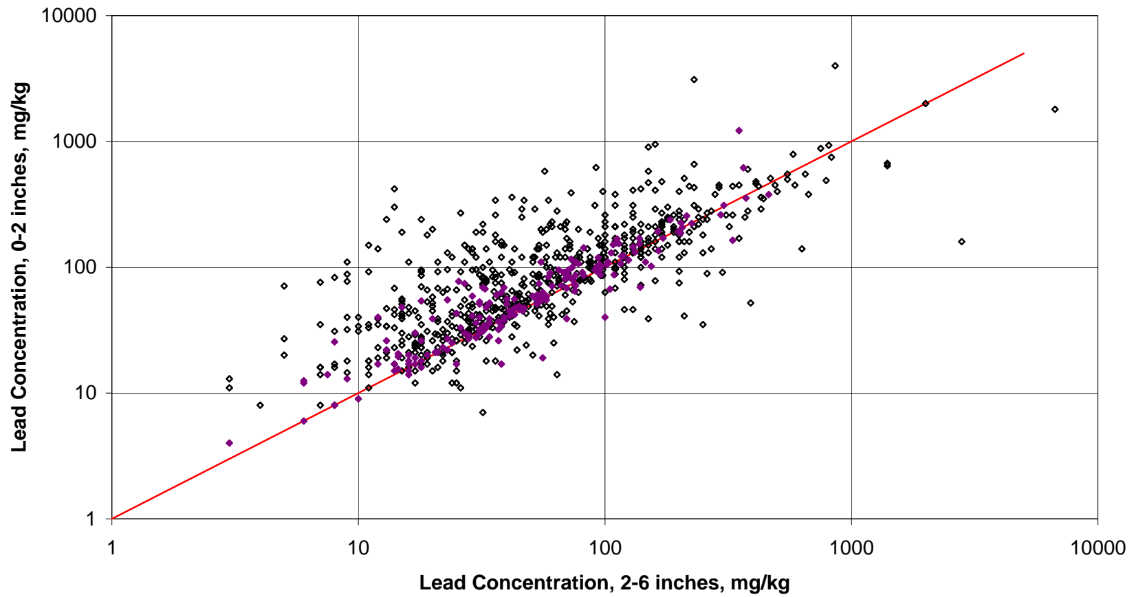
Figure 34 Lead Depth Profile Summary: Pierce County
