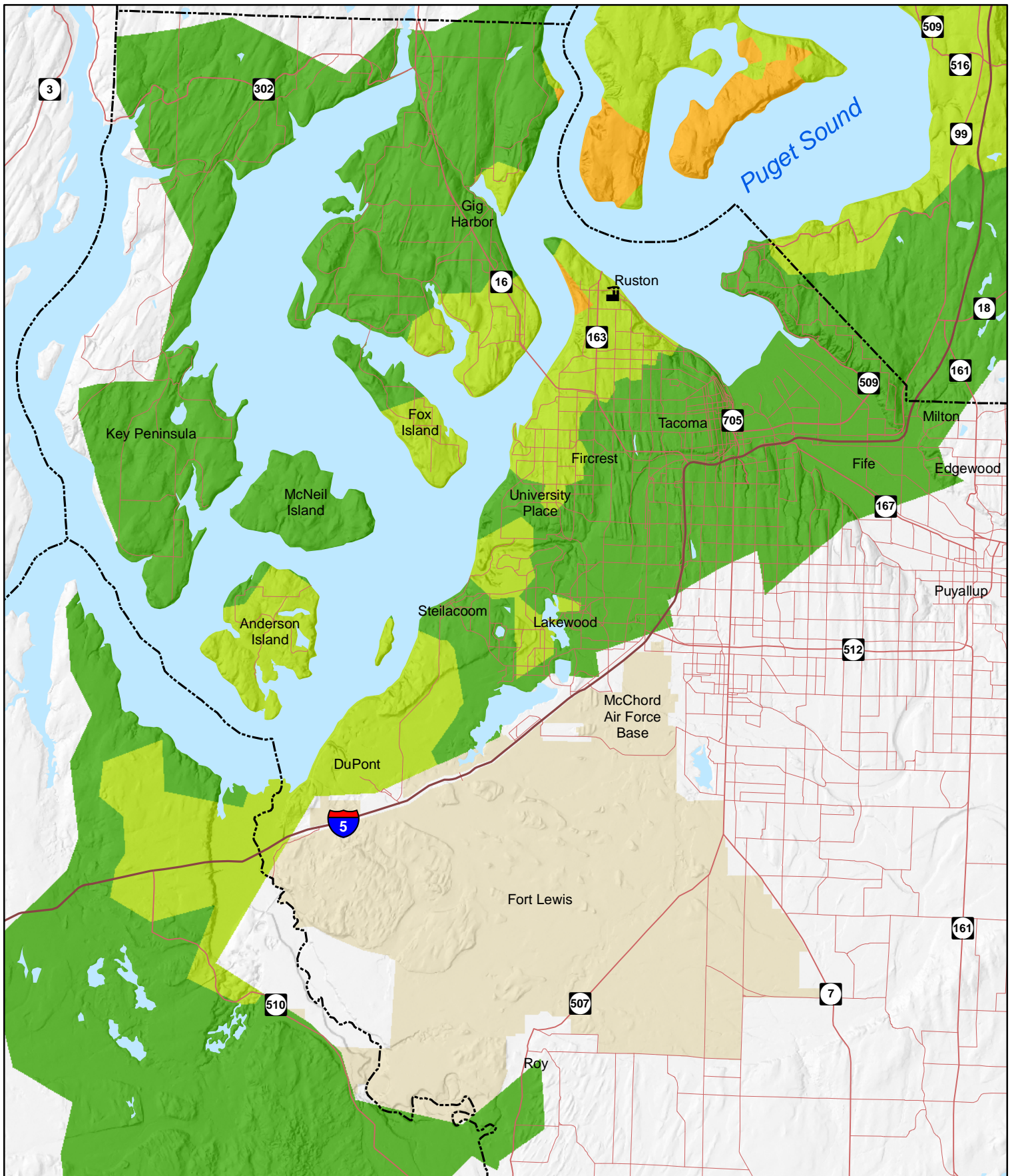
Figure D-4 Arsenic Concentrations In Soil, Median, 0-6 inches, Pierce County
