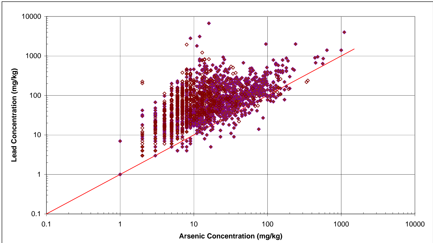
Figure 26 Arsenic vs. Lead: Pierce County
