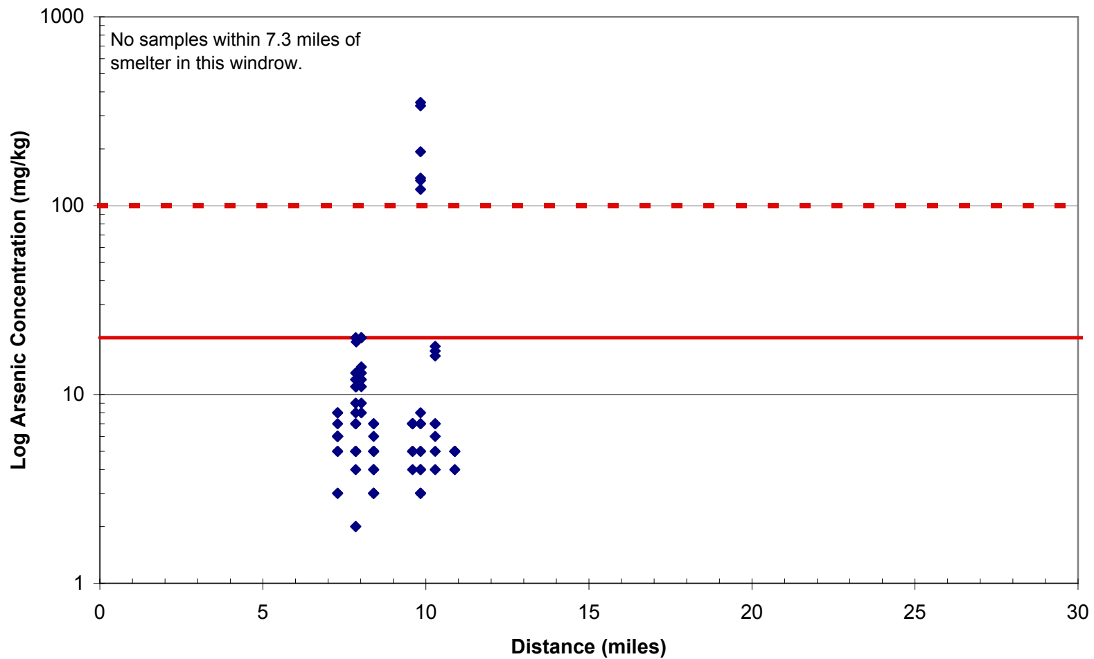
Figure 19 Arsenic Distribution: East-Southeast
