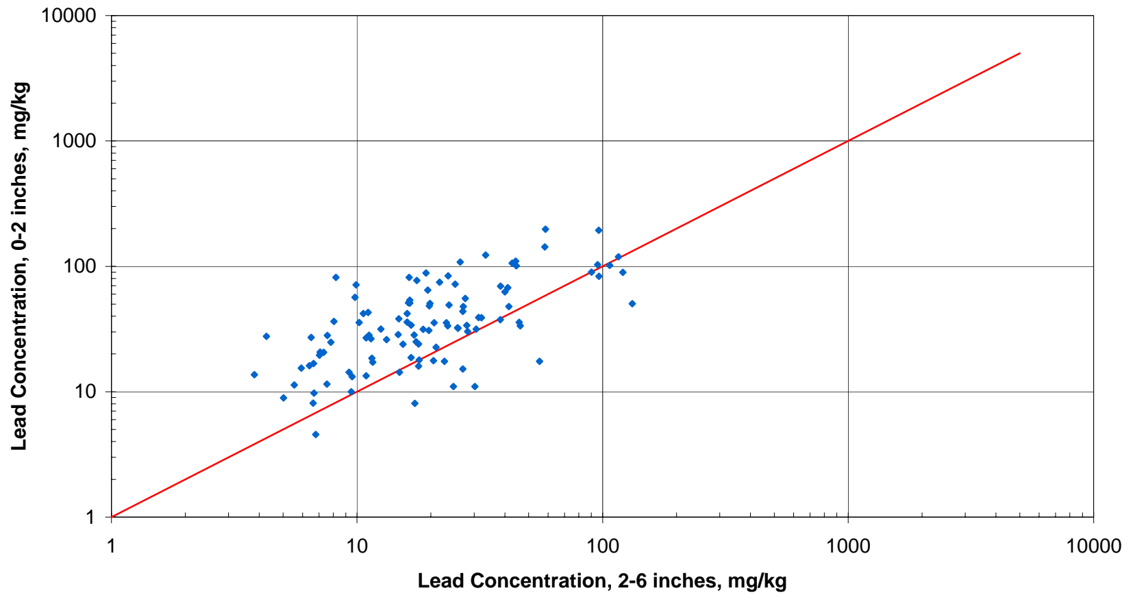
Figure 33 Lead Depth Profile Summary: Kitsap County
