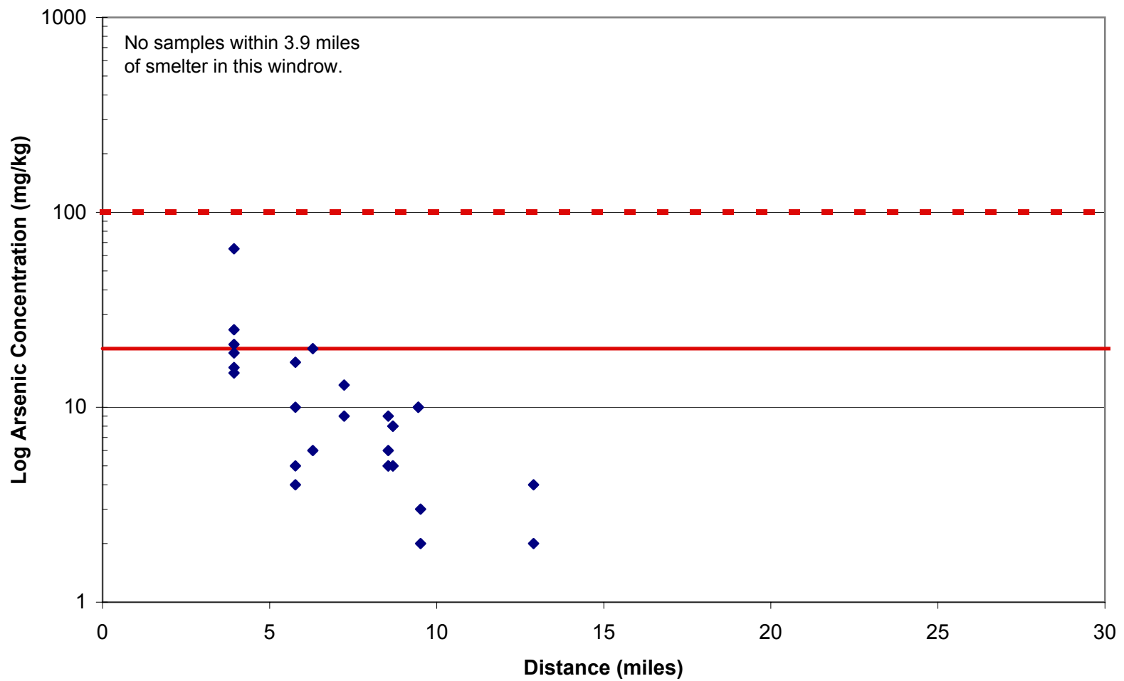
Figure 10 Arsenic Distribution: Northwest
