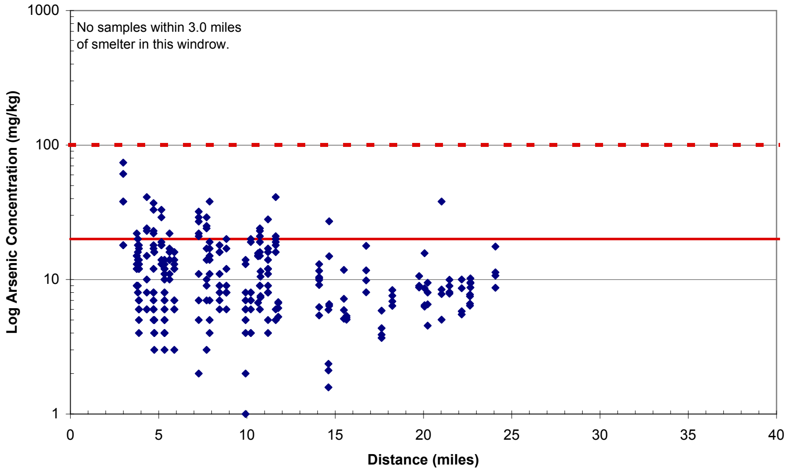
Figure 20 Arsenic Distribution: East
