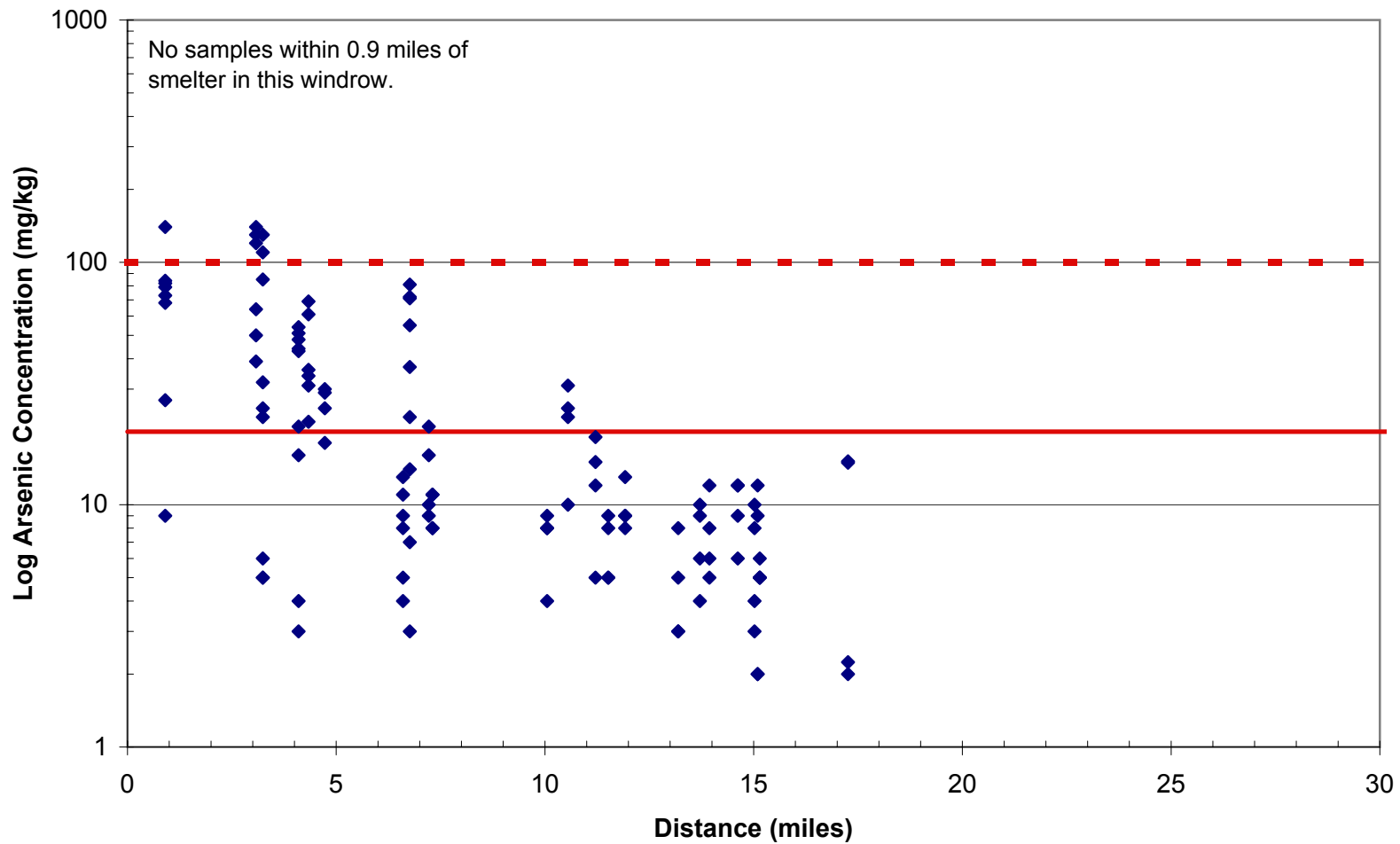
Figure 13 Arsenic Distribution: West-Southwest
