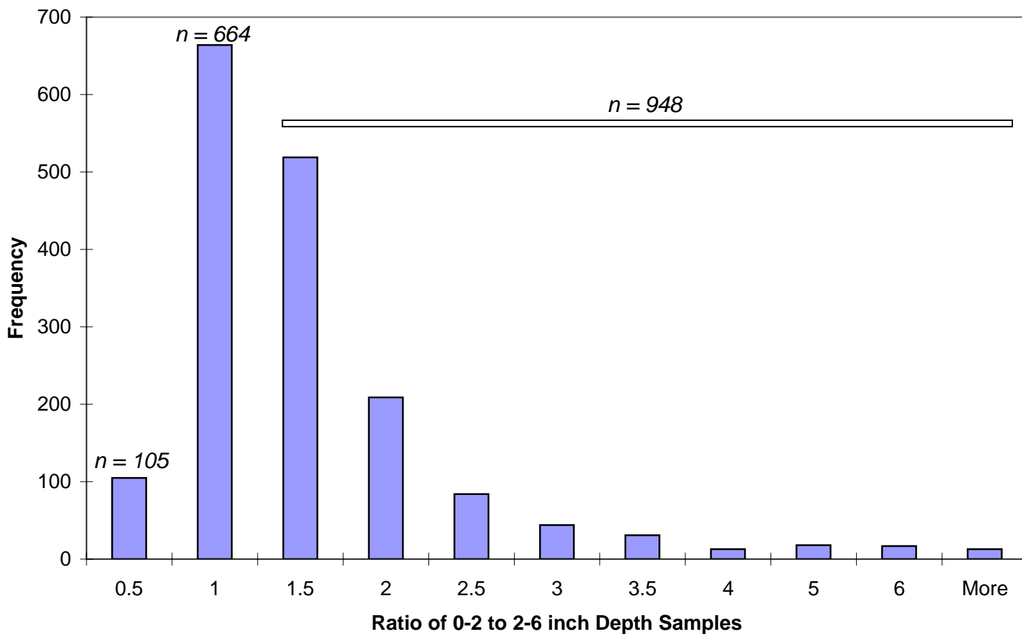
Figure 36 Histogram of Arsenic Depth Profile Ratios
