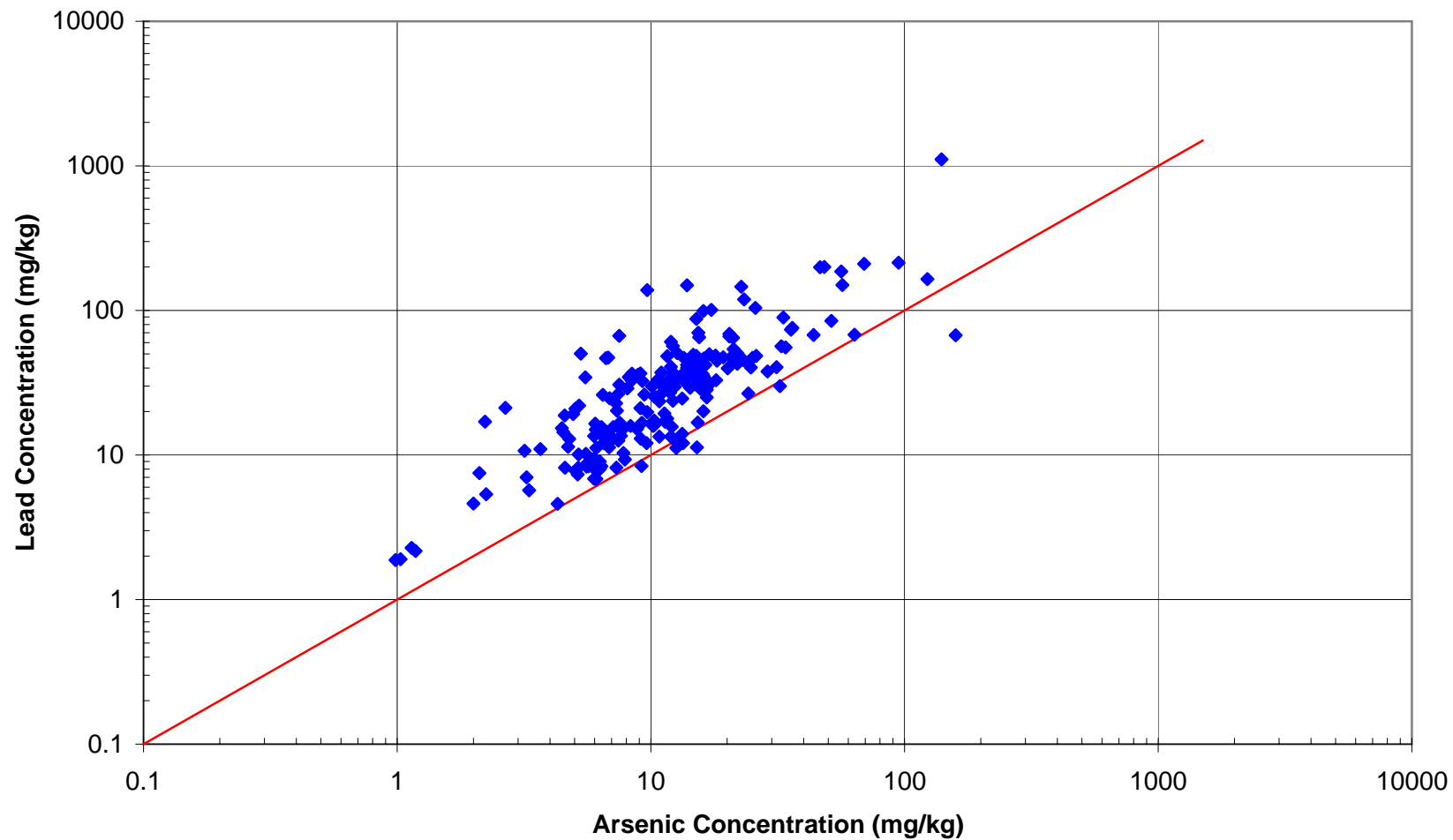
Figure 27 Arsenic vs. Lead: Thurston County
