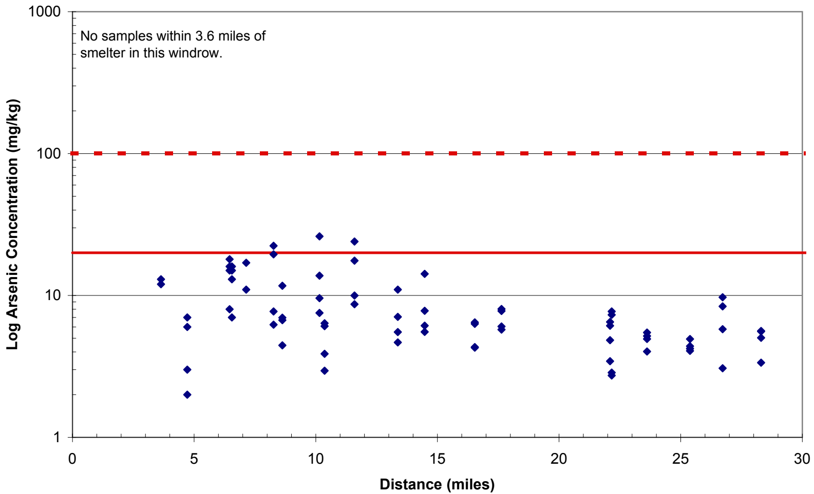
Figure 9 Arsenic Distribution: North-Northwest. Tacoma Smelter Plume Project
