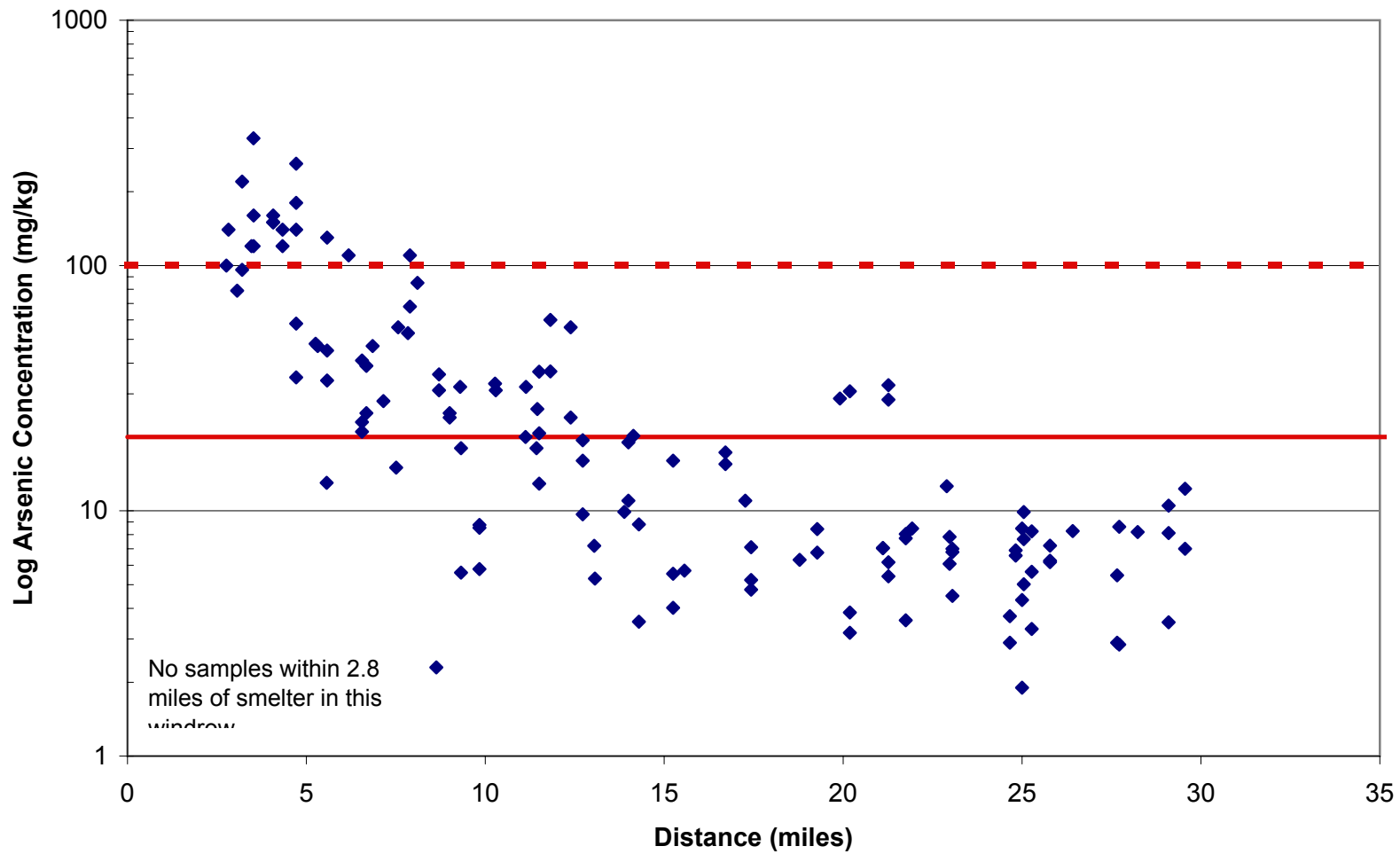
Figure 8 Arsenic Distribution: North Tacoma Smelter Plume Project
