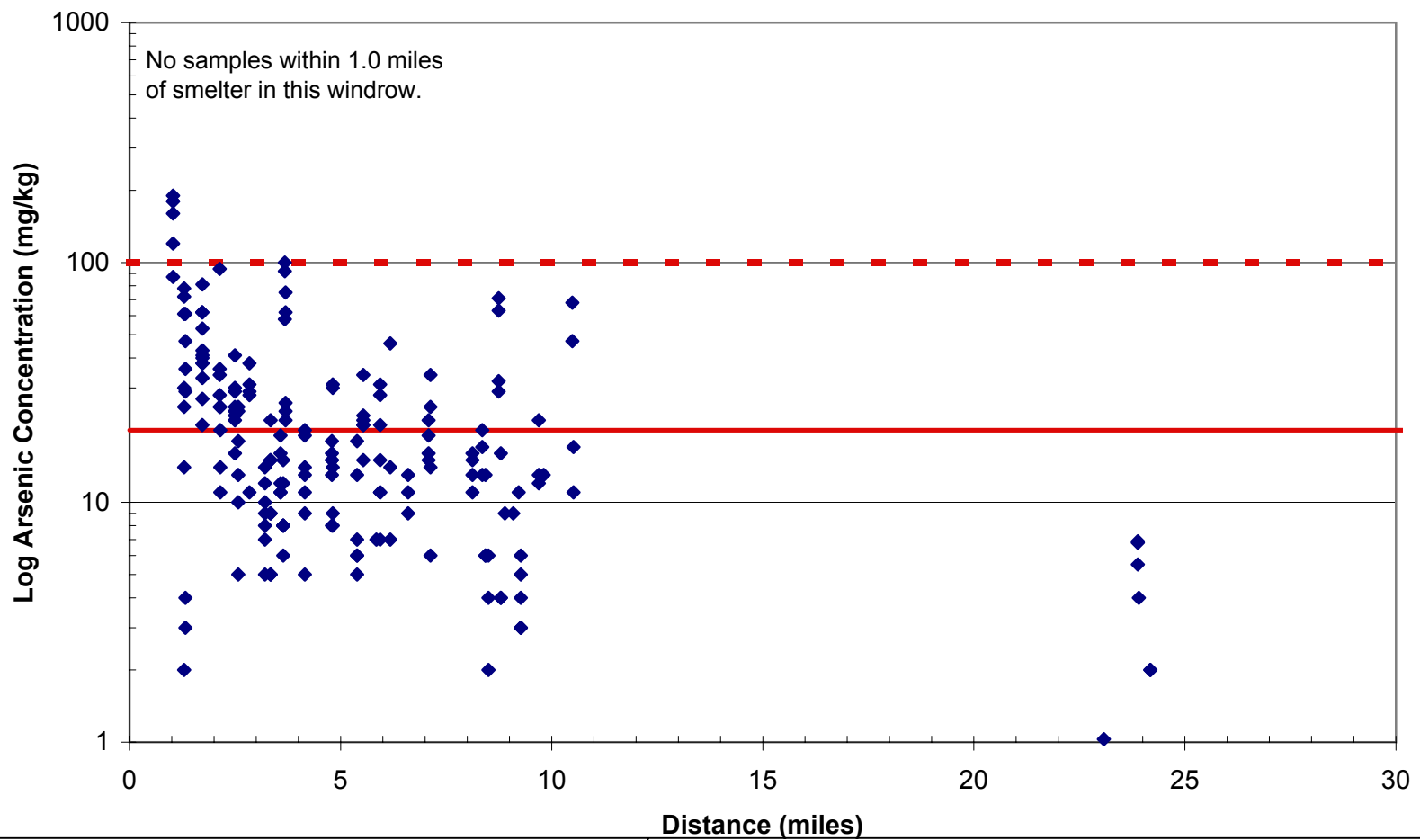
Figure 16 Arsenic Distribution: South
