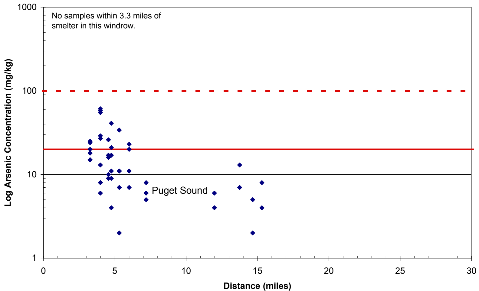
Figure 11 Arsenic Distribution: West-Northwest
