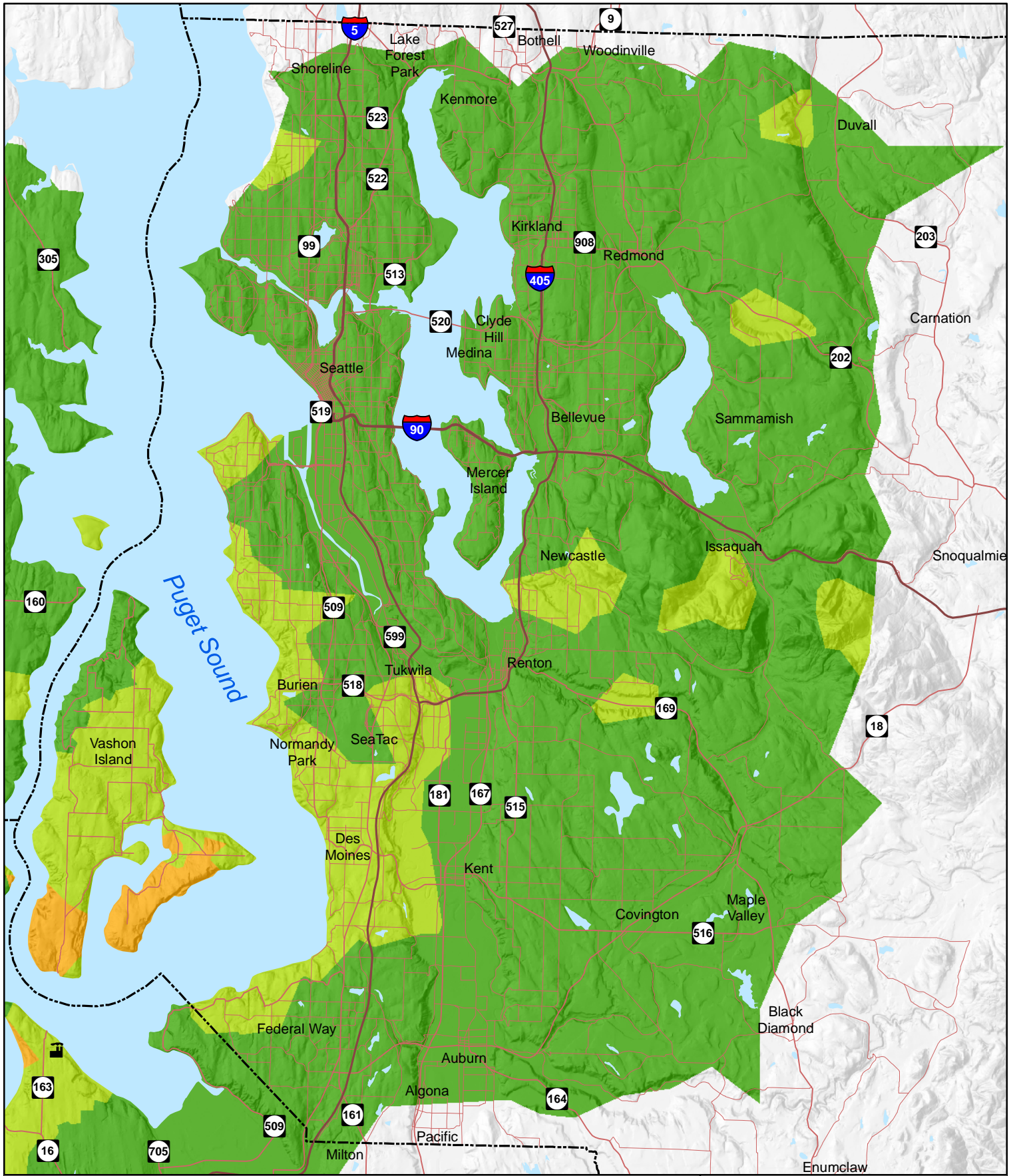
Figure B-4 Arsenic Concentrations In Soil, Median, 0-6 inches, King County
