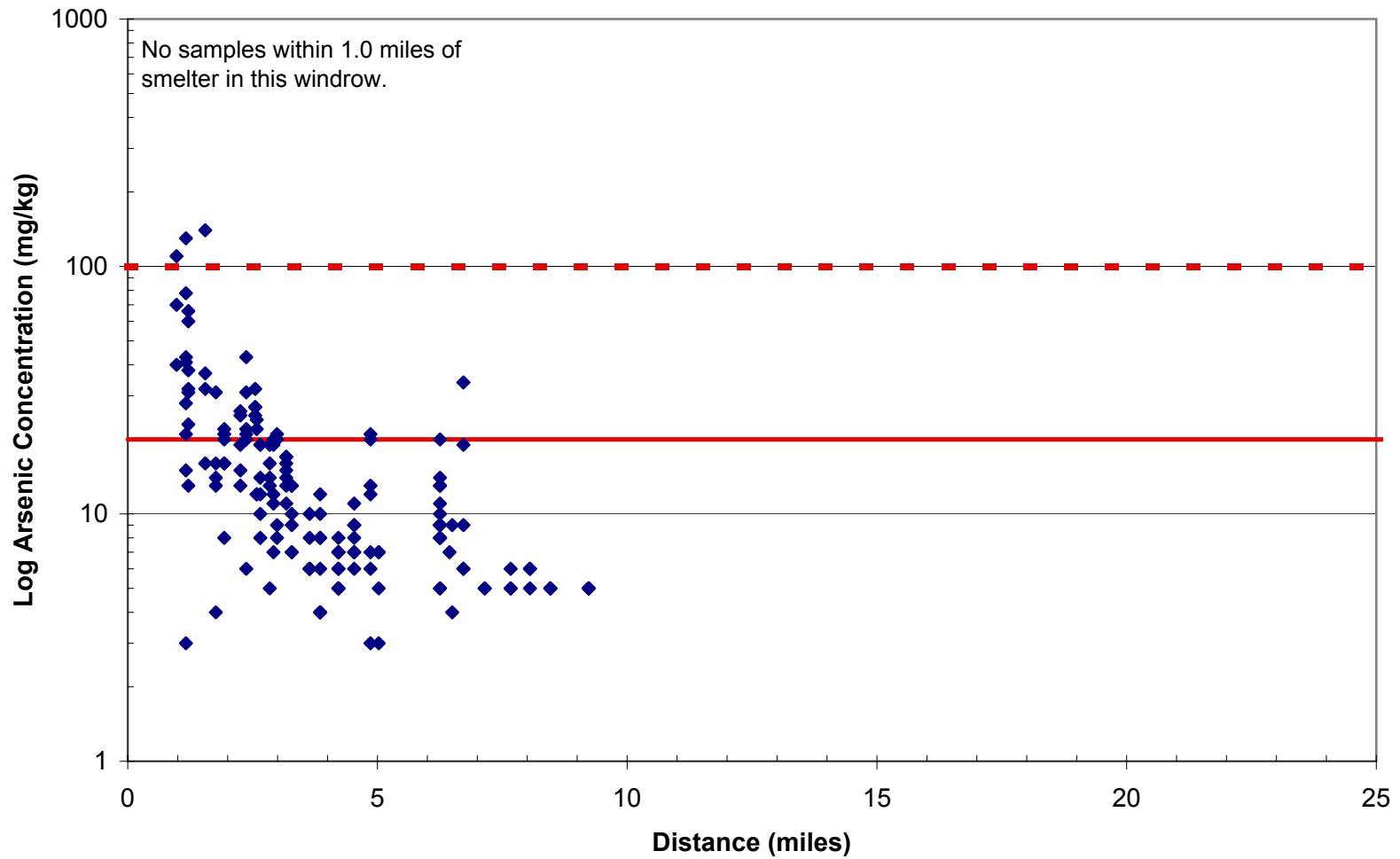
Figure 17 Arsenic Distribution: South-Southeast
