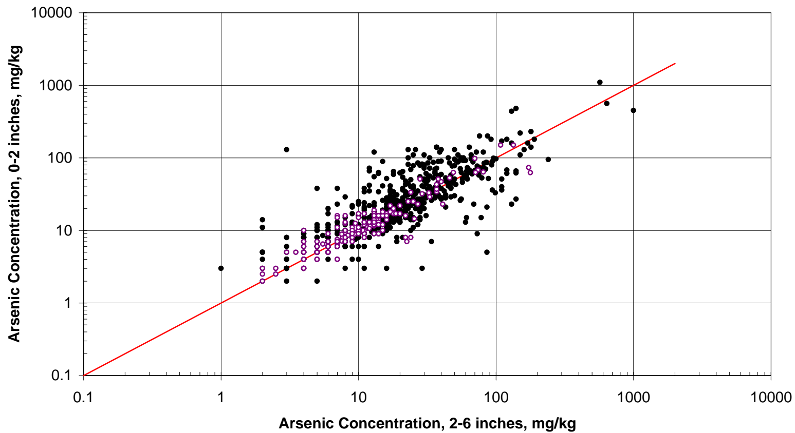
Figure 30 Arsenic Depth Profile Summary: Pierce County
