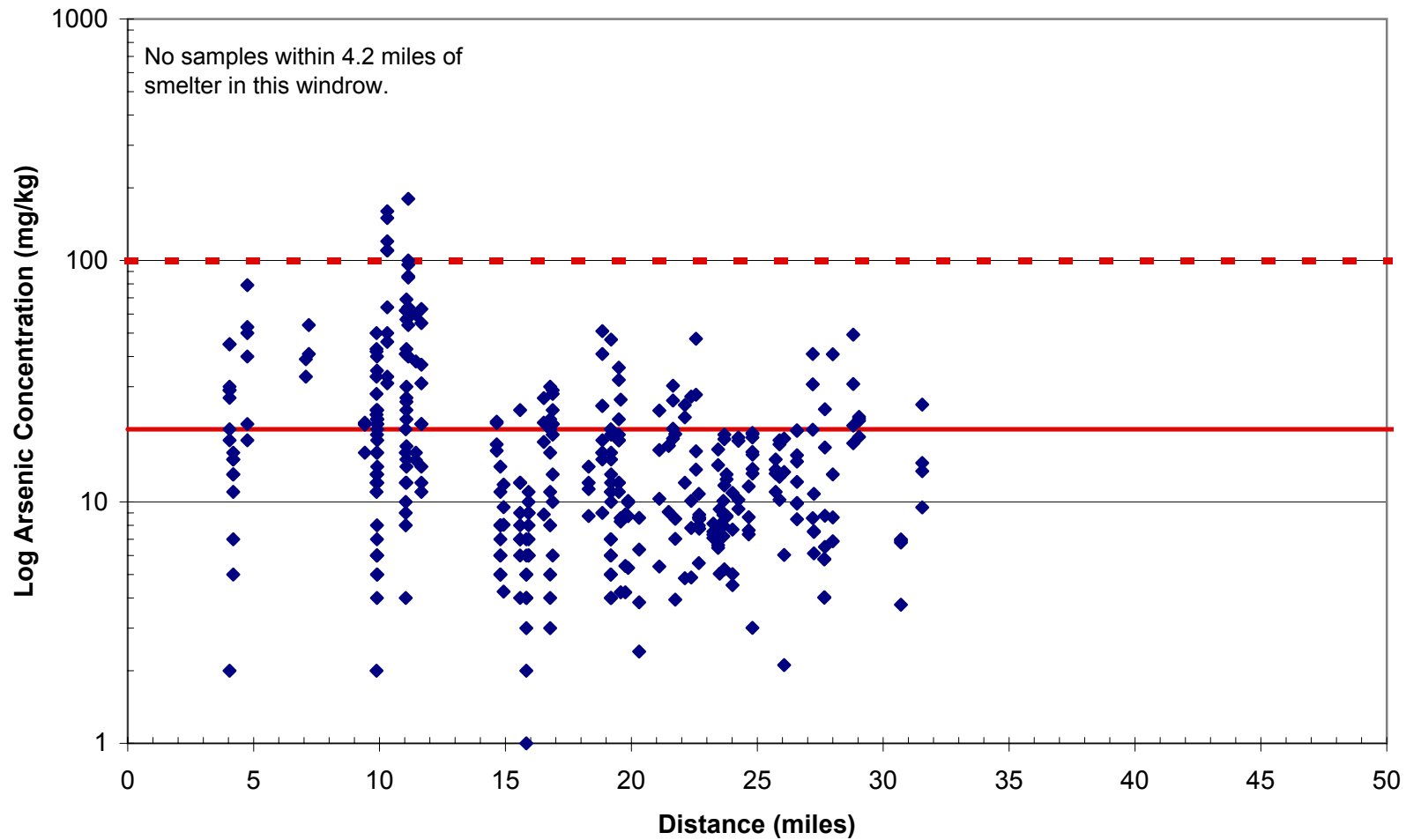
Figure 21 Arsenic Distribution: East-Northeast
