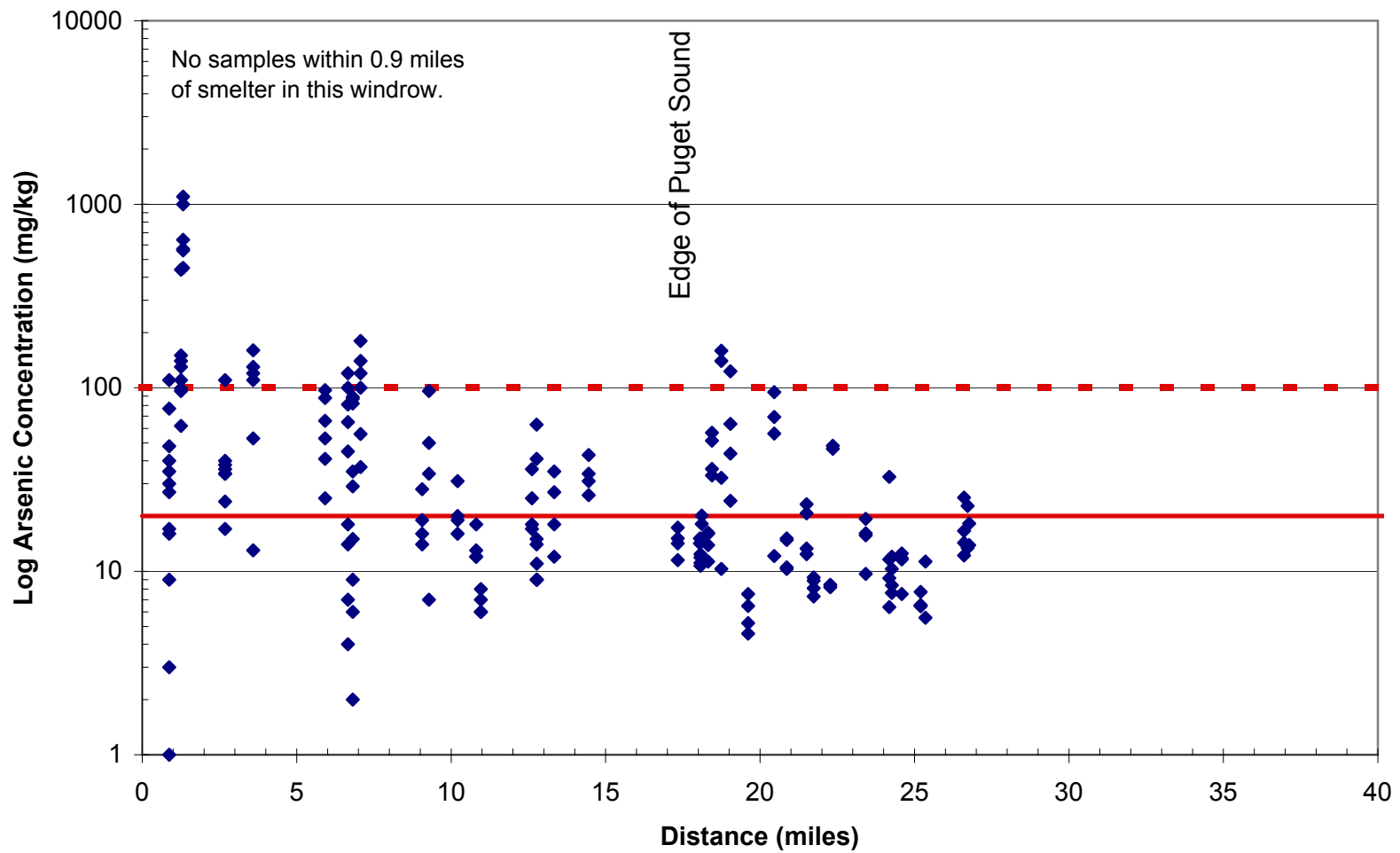
Figure 14 Arsenic Distribution: Southwest
