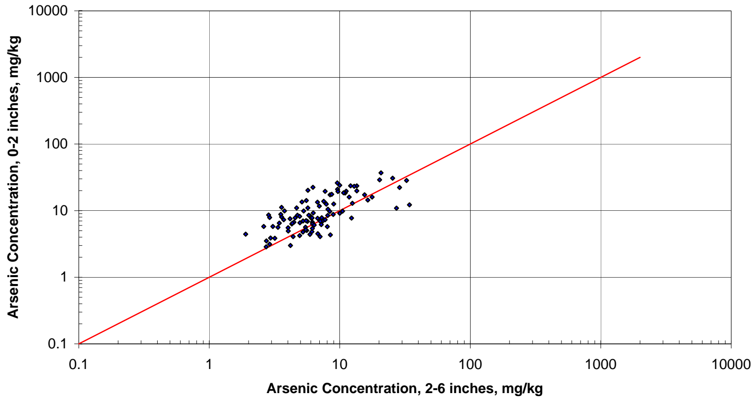
Figure 29 Arsenic Depth Profile Summary: Kitsap County
