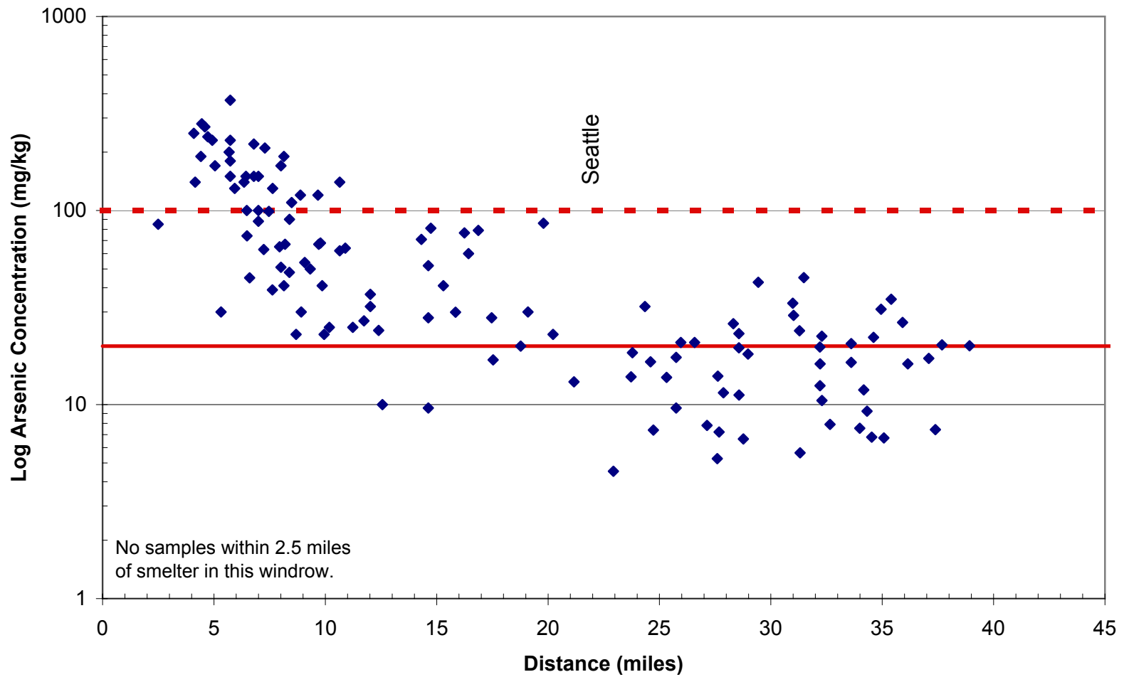
Figure 23 Arsenic Distribution: North-Northeast
