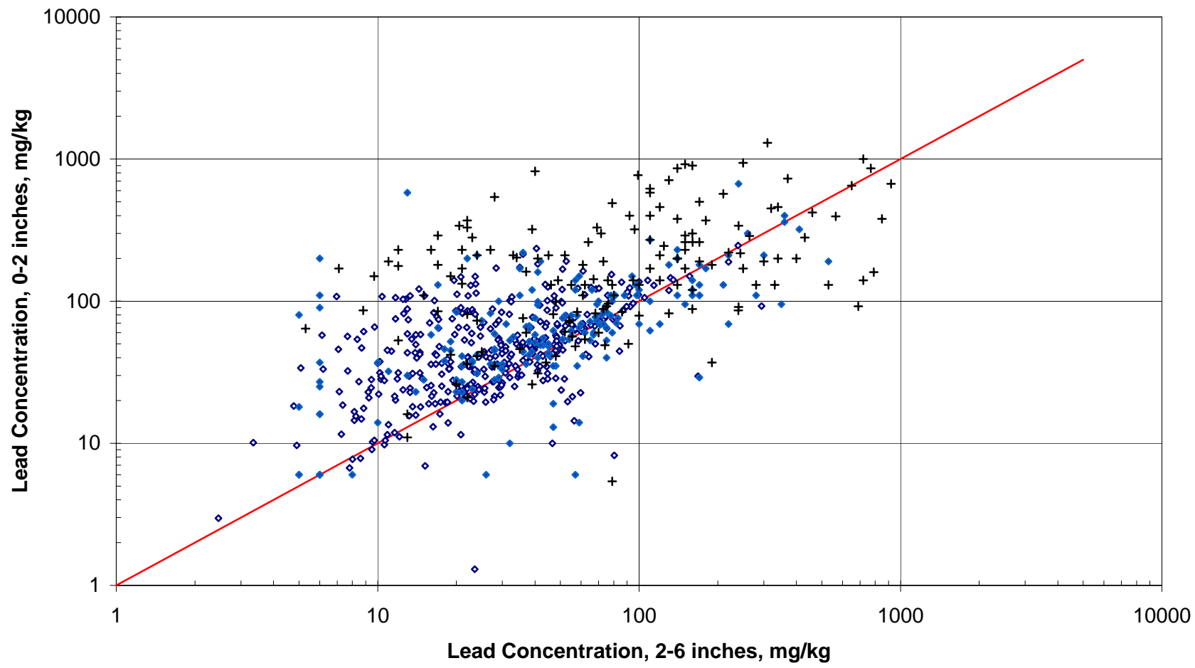
Figure 32 Lead Depth Profile Summary: King County
