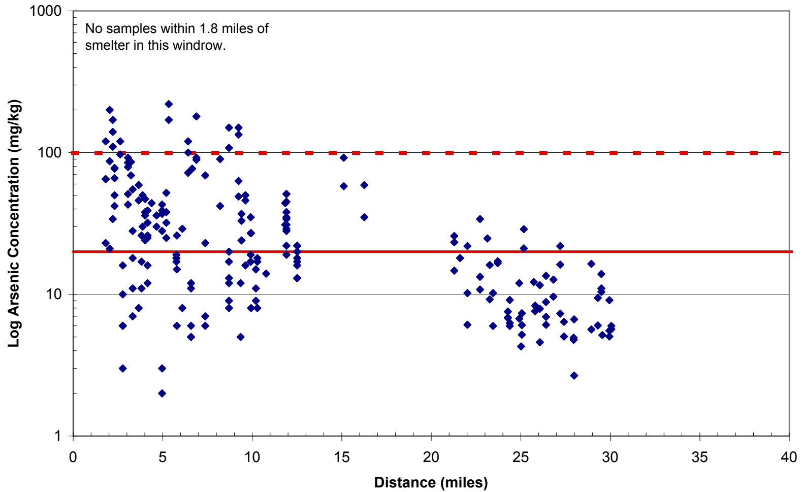
Figure 15 Arsenic Distribution: South-Southwest
