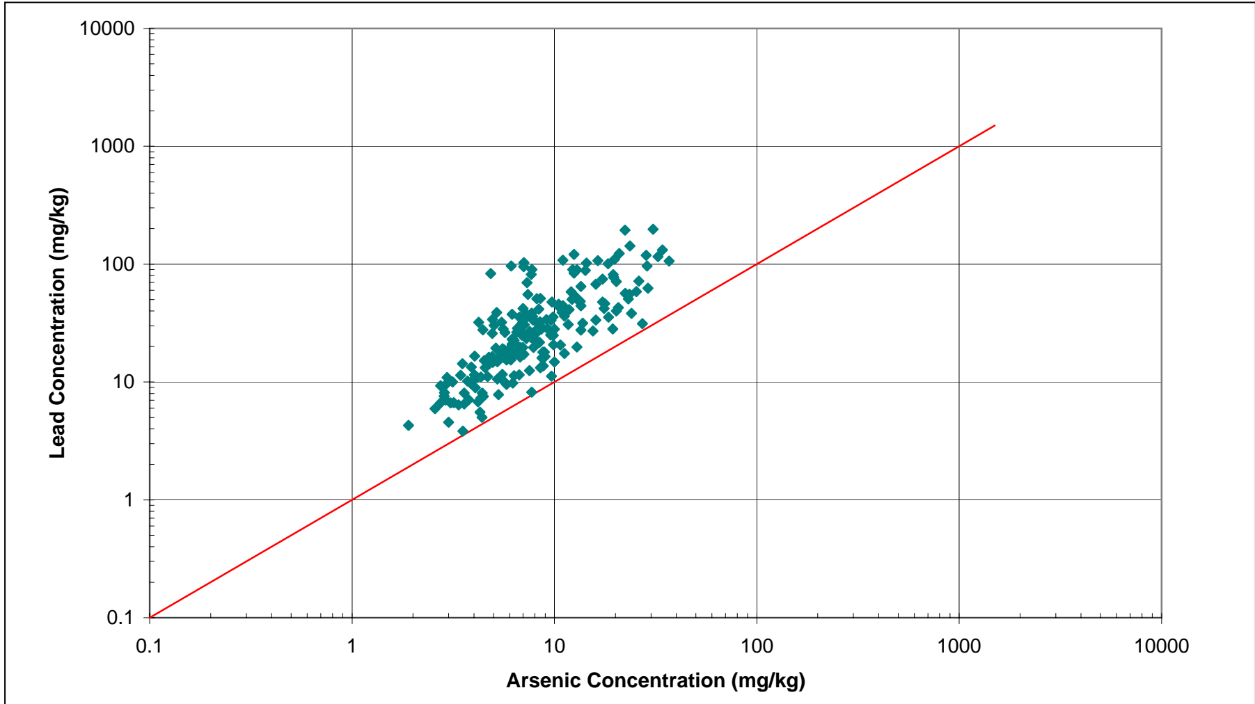
Figure 25 Arsenic vs. Lead : Kitsap County
