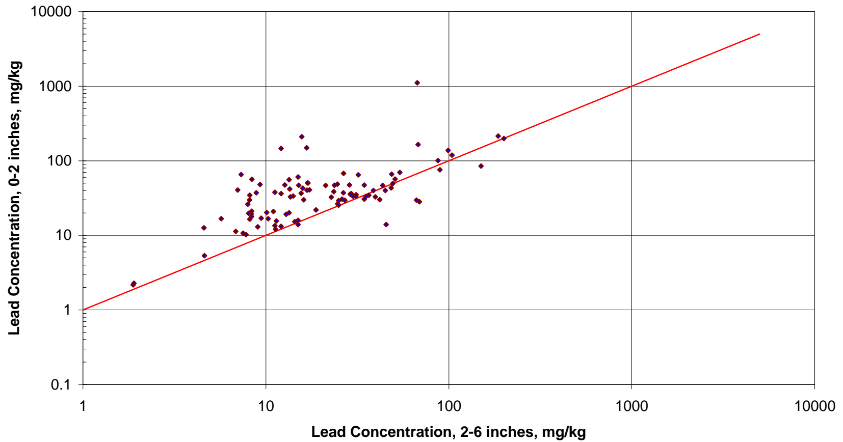
Figure 35 Lead Depth Profile Summary: Thurston County
