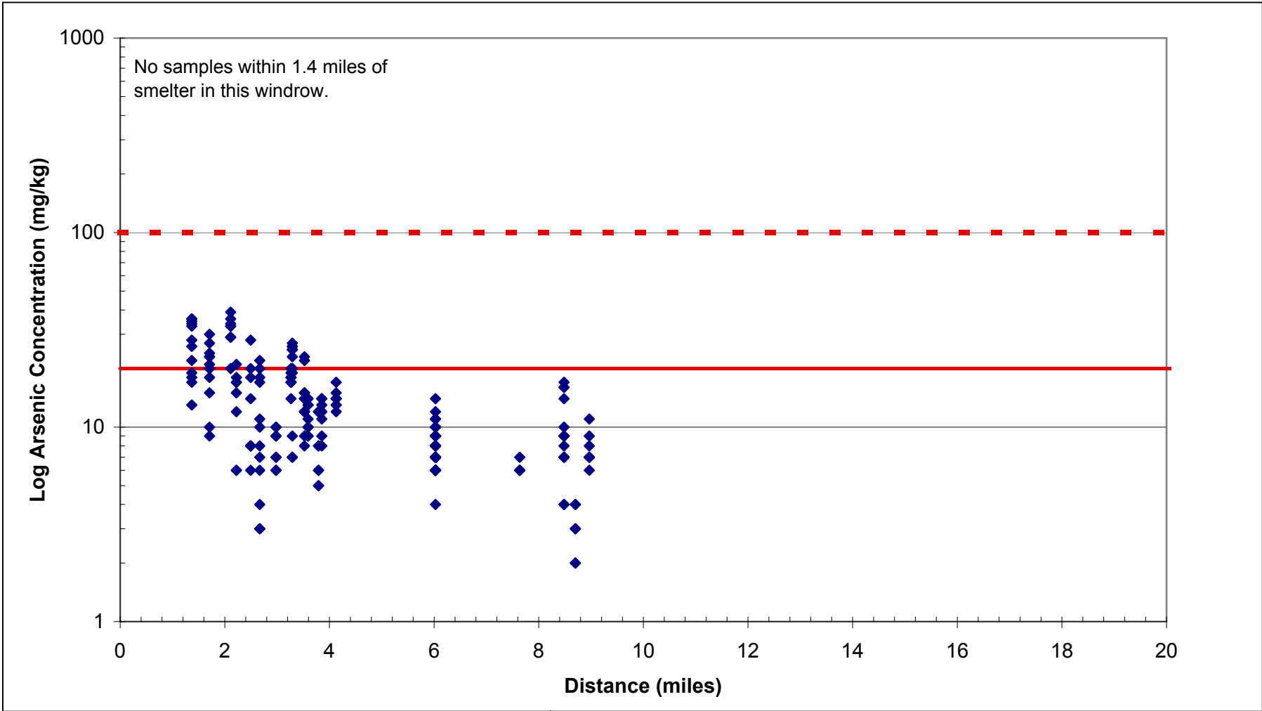
Figure 18 Arsenic Distribution: Southeast
