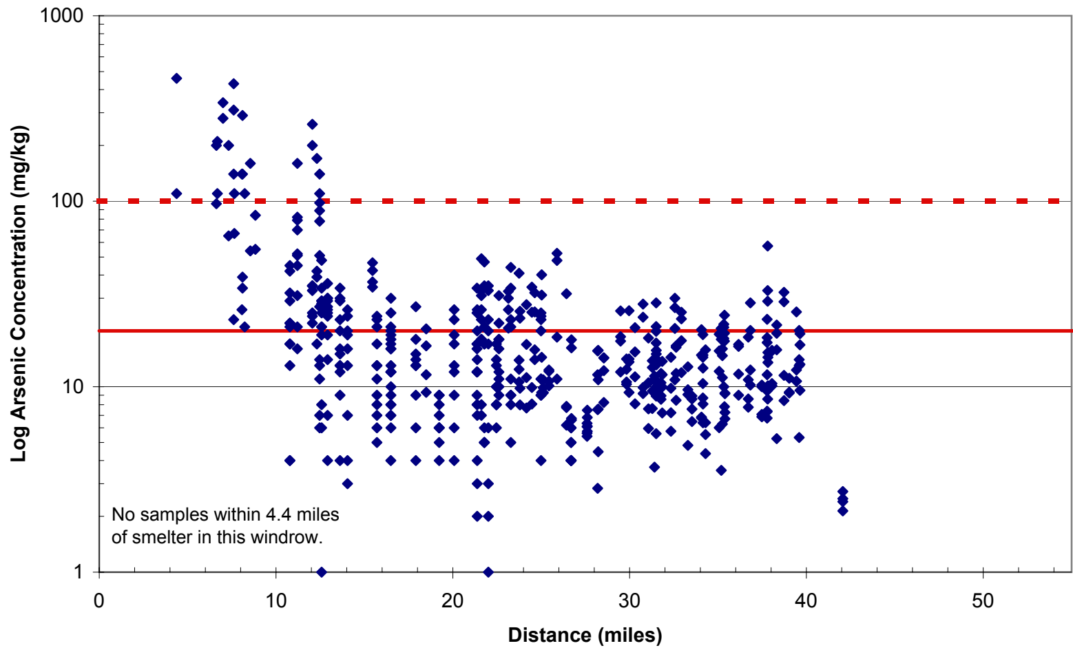
Figure 22 Arsenic Distribution: Northeast
