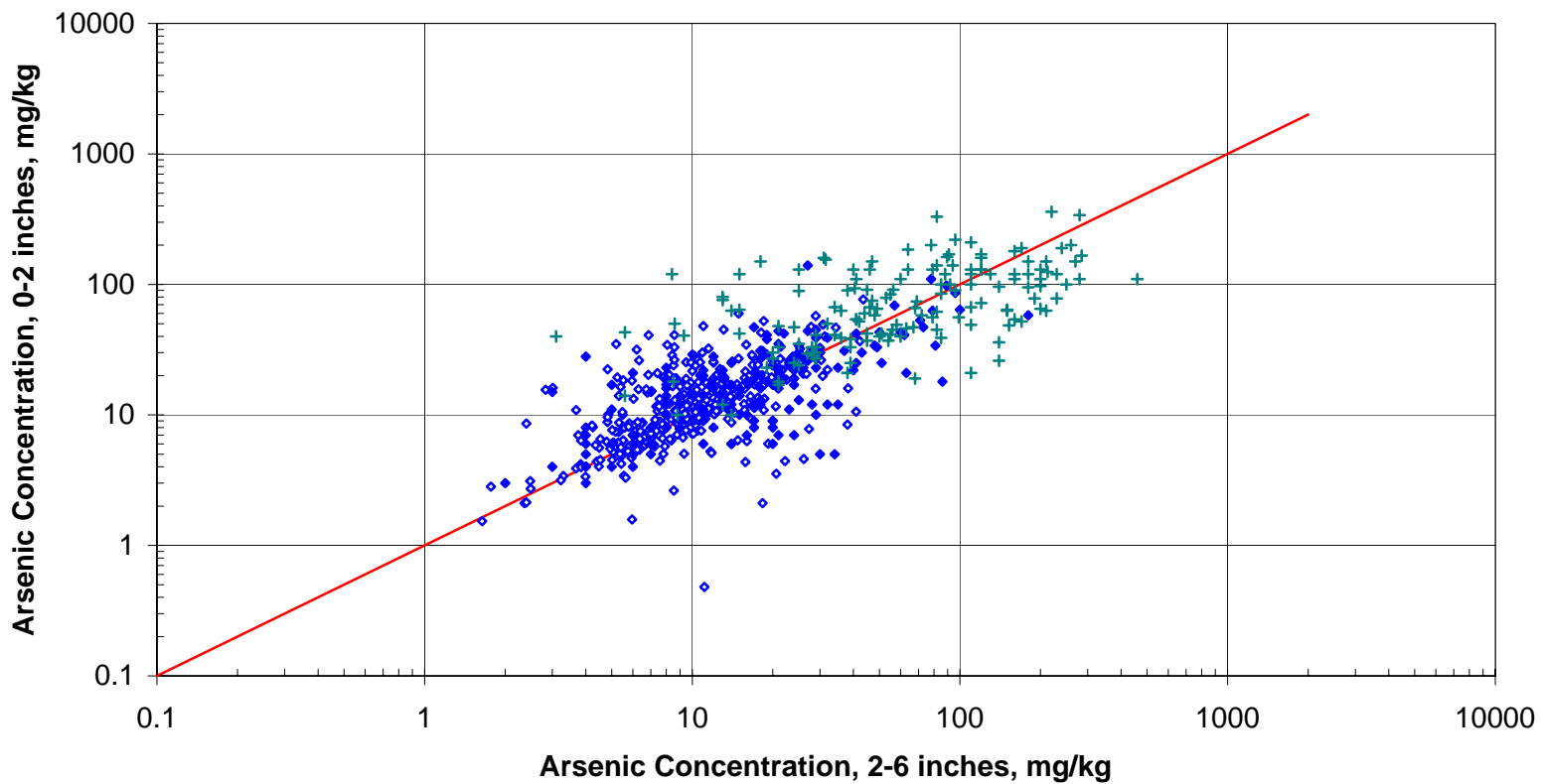
Figure 28 Arsenic Depth Profile Summary: King County
