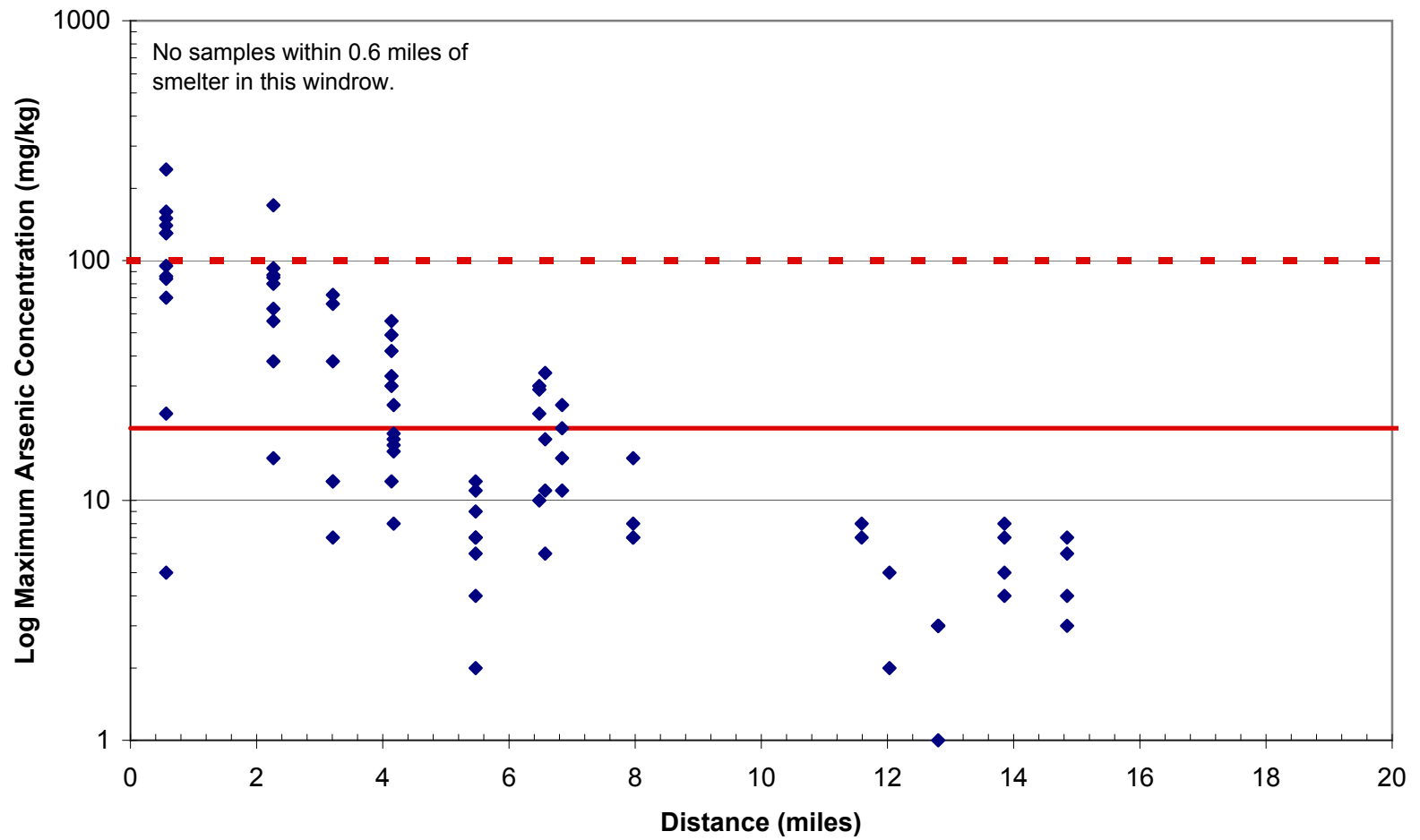
Figure 12 Arsenic Distribution: West
