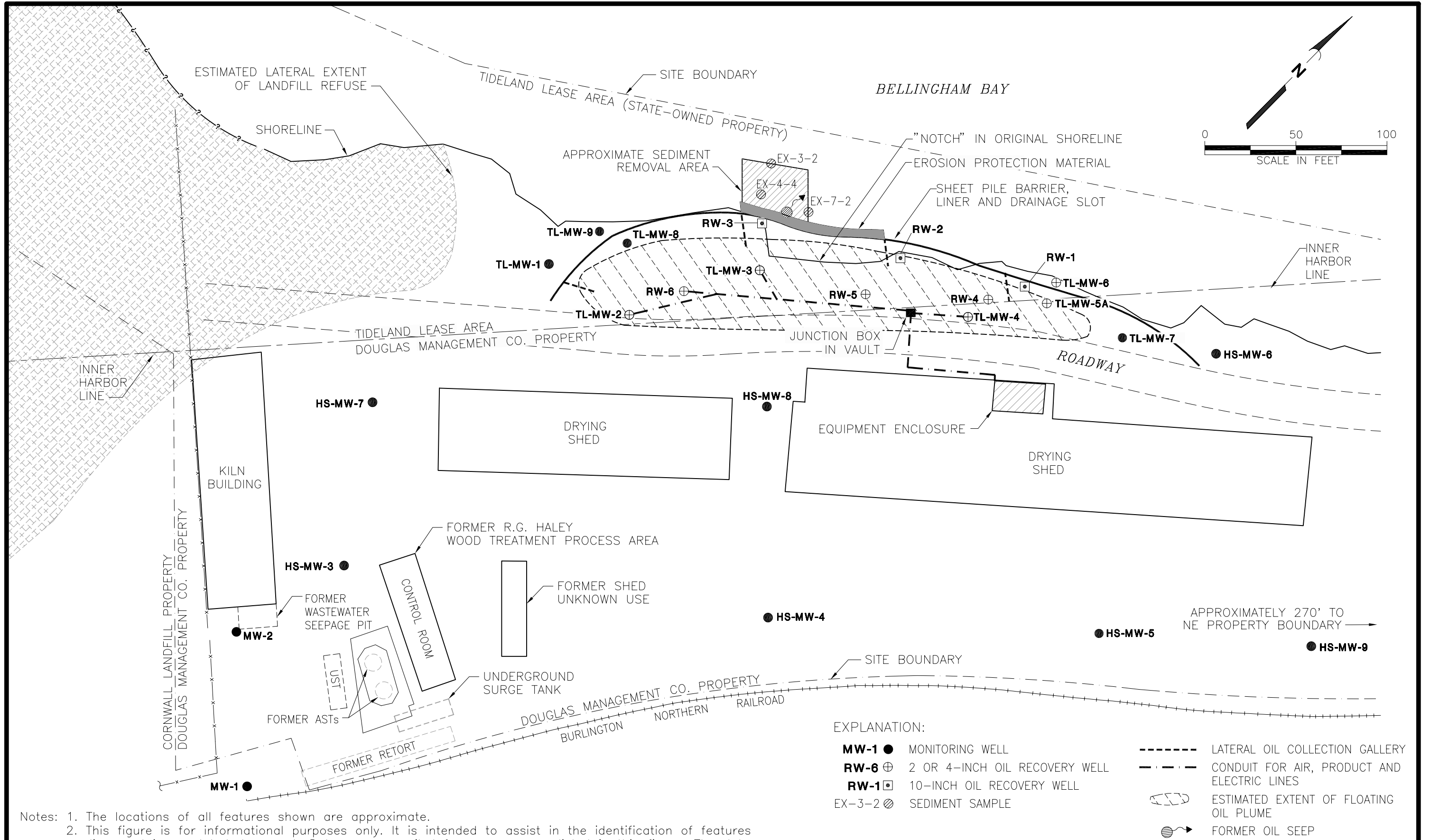
SITE PLAN INTERIM CLEANUP ACTION COMPONENTS FIGURE 10
