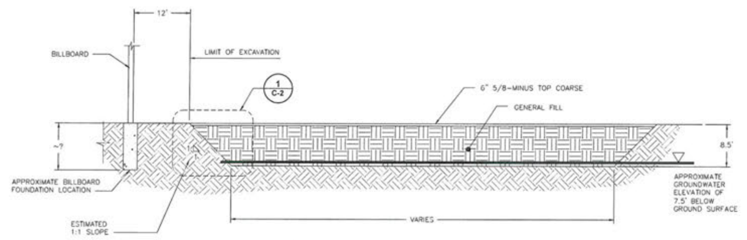
A C-2 EXCAVATION AREA CROSS SECTION NOT TO SCALE
