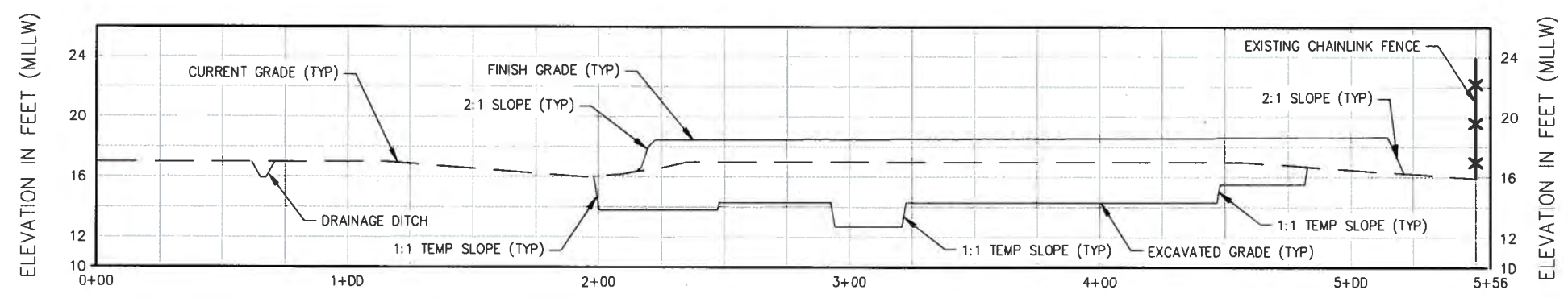
B CROSS SECTION C3.1, C3.3 SCALE: HORIZ- 1" = 30' VERT- 1" = 5'
