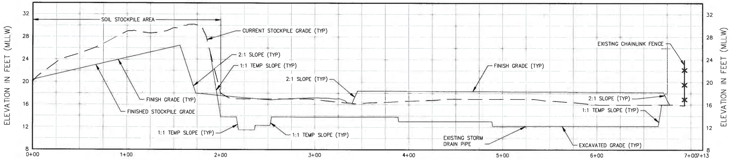
A CROSS SECTION C3.1, C3.3 SCALE: HORIZ- 1" = 30' VERT- 1" = 5'
