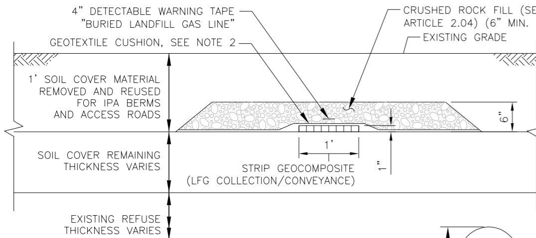
1 LFG COLLECTION/CONVEYANCE LINE DETAIL SCALE: NTS
