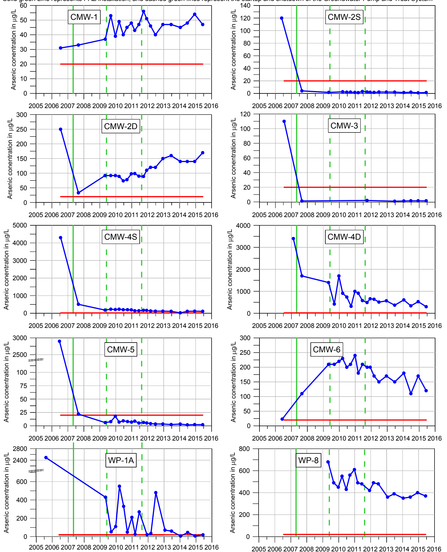
Figure 4 - Trends in Arsenic Concentrations in Groundwater at Monitoring Wells
