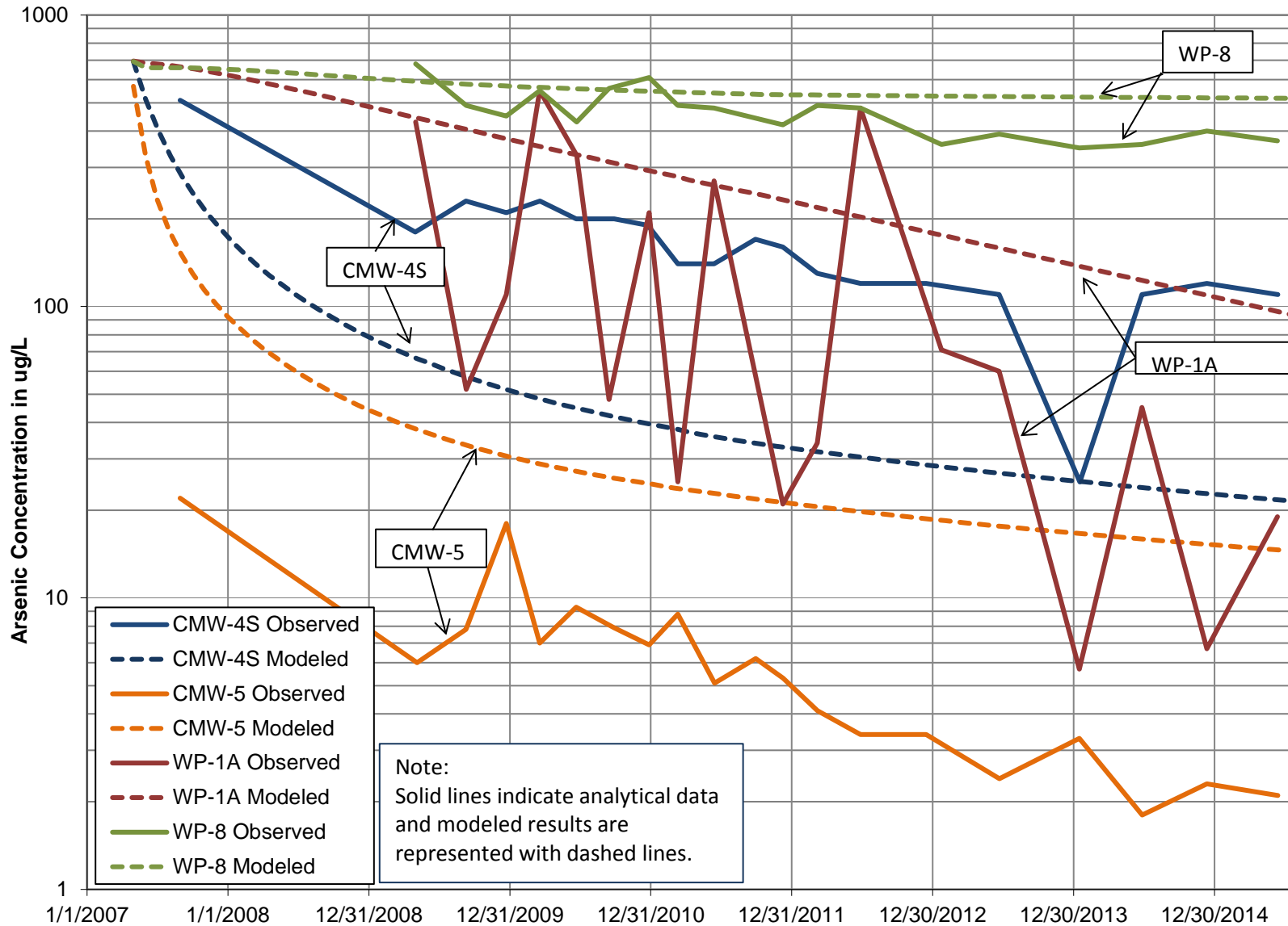
Comparison of Observed and Model-Predicted Arsenic Concentrations Downgradient of PAZ
