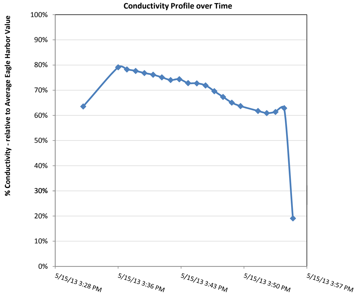
Figure 9E Conductivity Profiles and Drawdown for Seam Pumping conducted May 2013 - Seam 5 Wyckoff Sheet Pile Wall Evaluation Wyckoff/Eagle Harbor Superfund Site
