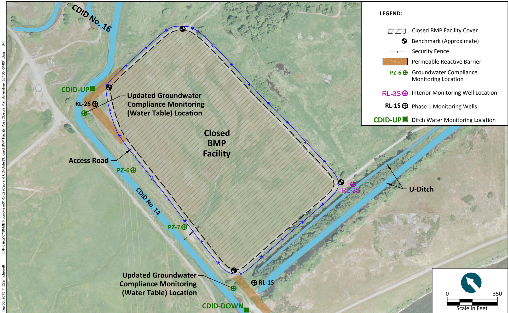
Figure B-4 Amended Closed BMP Facility Monitoring Elements Closed BMP Facility Post-Closure Plan Amendment Former Reynolds Metals Reduction Plant – Longview
