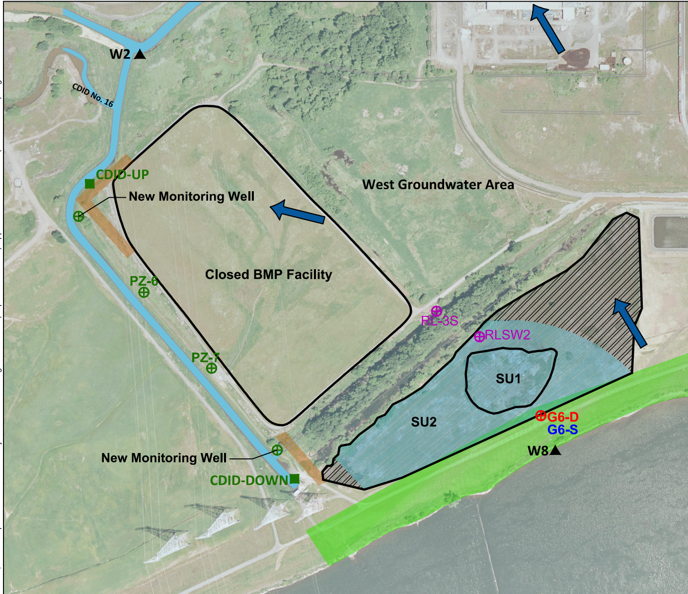
Figure 2-4a Groundwater Monitoring Locations - West Groundwater Area Cleanup Action Plan Former Reynolds Metals Reduction Plant – Longview
