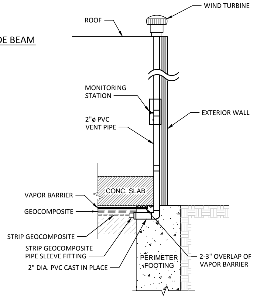
5 TYPICAL VENT PIPE PENETRATION N.T.S.
