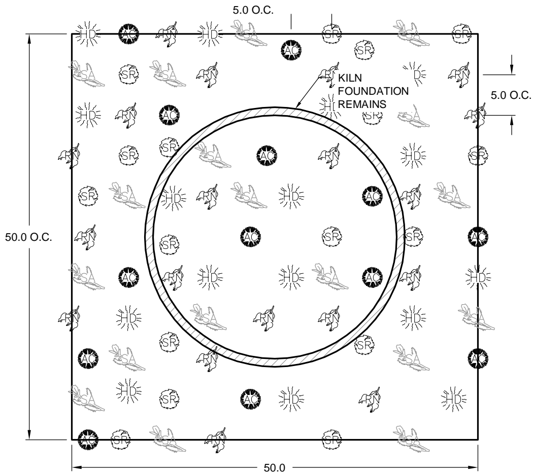
SHORELINE KILNS SHRUB PLANTING AREA TYPICAL LAYOUT SCALE: 1"=12'
