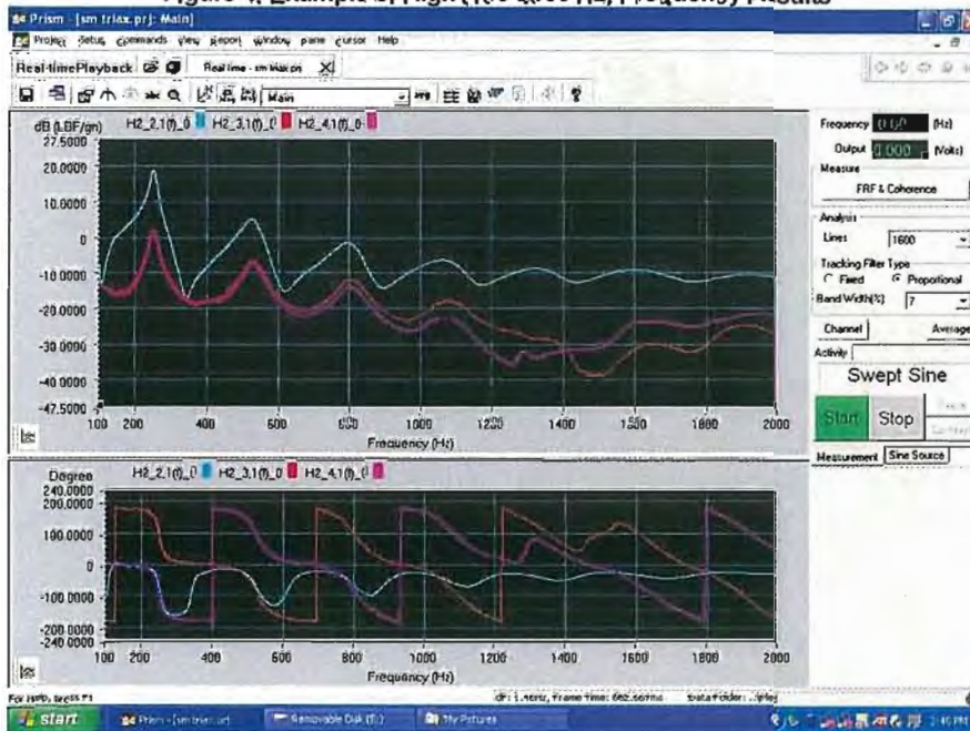
Figure 4: Example of High (100-2000 Hz) Frequency Results
