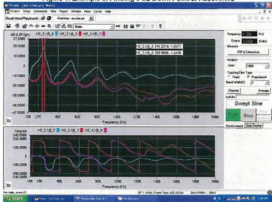
Figure 6: Example of Finding 3 dB Down Point of Resonance
