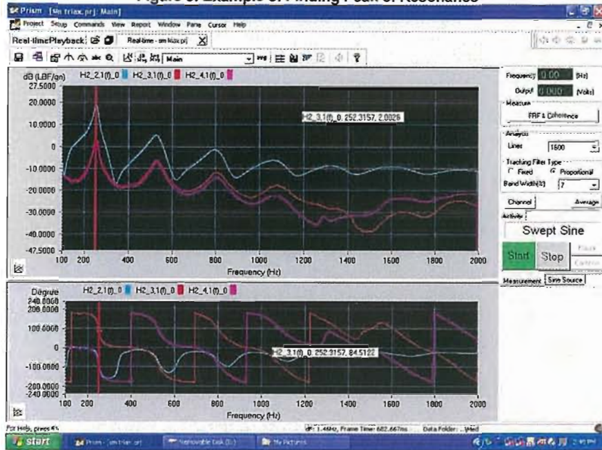
Figure 5: Example of Finding Peak of Resonance
