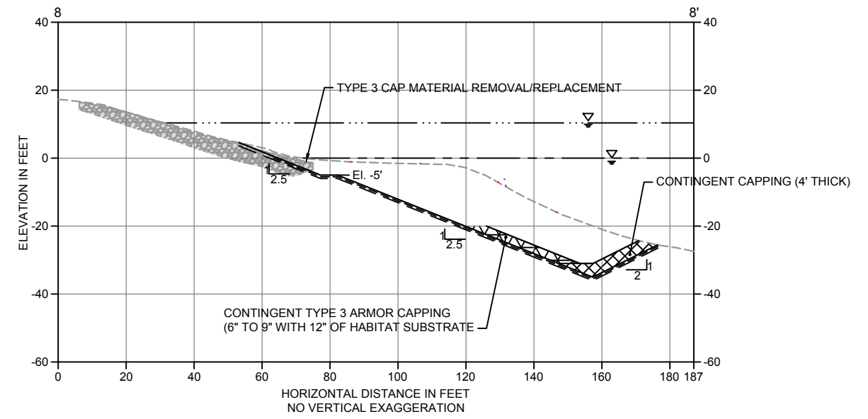
8 DREDGE/EXCAVATION SECTION C-01-A SCALE: 1" = 20'
