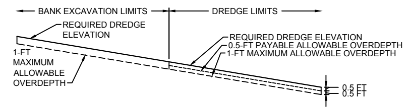
1 PAYABLE AND MAXIMUM ALLOWABLE OVERDEPTH DETAIL SCALE: NTS
