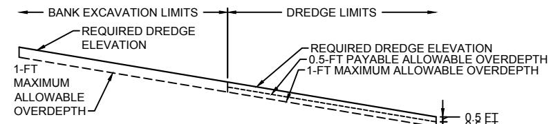
1 PAYABLE AND MAXIMUM ALLOWABLE OVERDEPTH DETAIL SCALE: 1" = 20'
