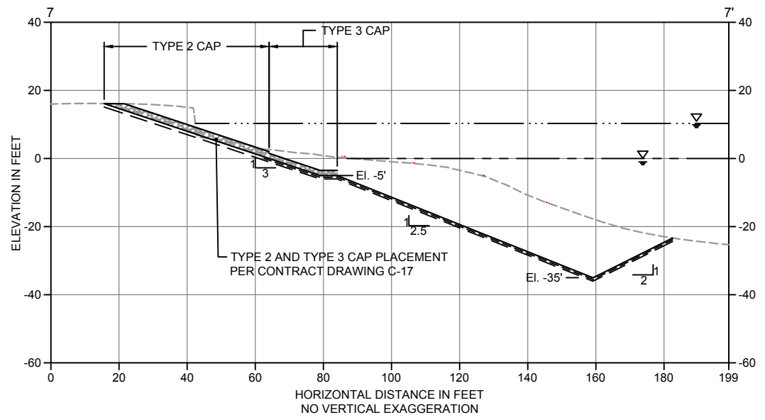
7 DREDGE/EXCAVATION SECTION C-01-A SCALE: 1" = 20'
