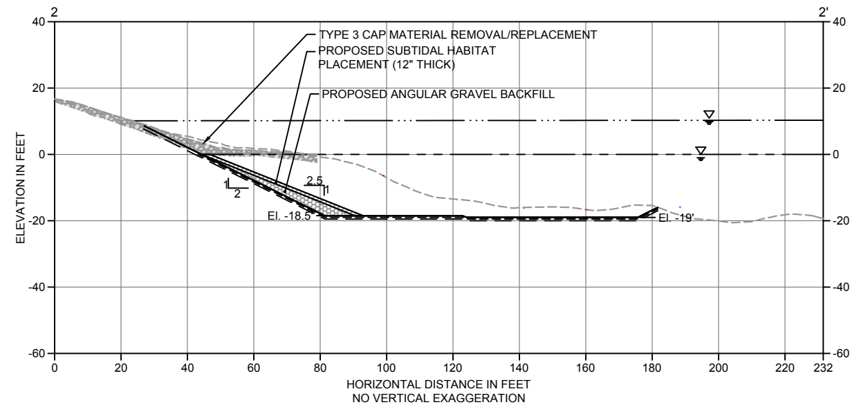
2 DREDGE/EXCAVATION SECTION C-01-A SCALE: 1" = 20'
