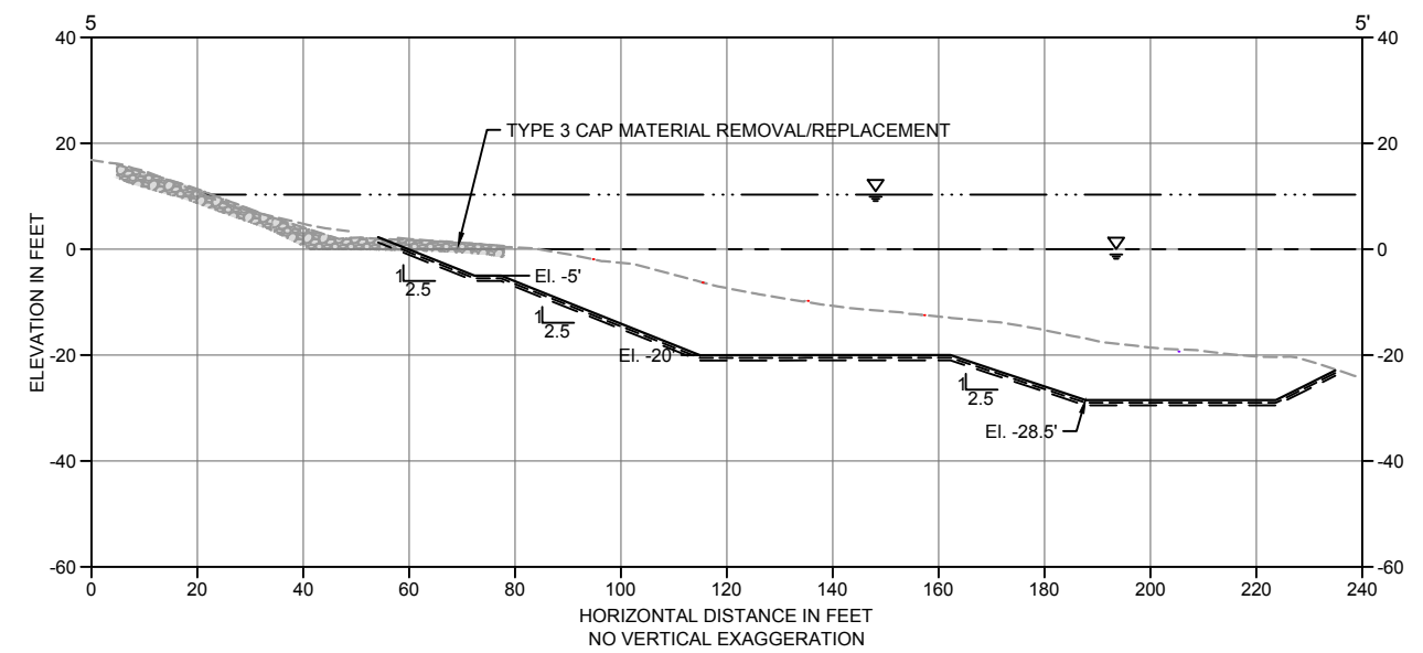
5 DREDGE/EXCAVATION SECTION C-01-A SCALE: 1" = 20'
