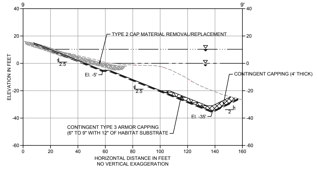
9 DREDGE/EXCAVATION SECTION C-01-A SCALE: 1" = 20'
