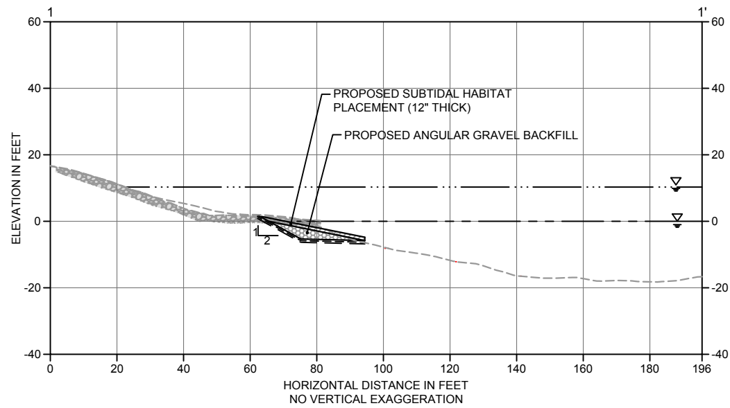
1 DREDGE/EXCAVATION SECTION C-01-A SCALE: 1" = 20'
