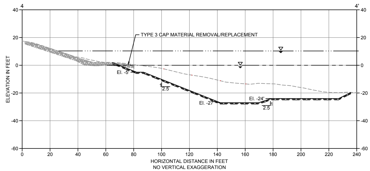
4 DREDGE/EXCAVATION SECTION C-01-A SCALE: 1" = 20'
