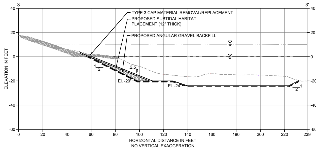
3 DREDGE/EXCAVATION SECTION C-01-A SCALE: 1" = 20'
