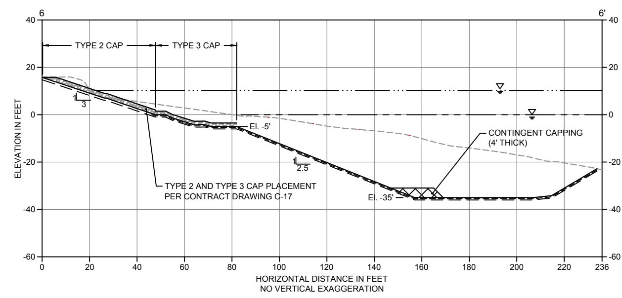
6 DREDGE/EXCAVATION SECTION C-01-A SCALE: 1" = 20'
