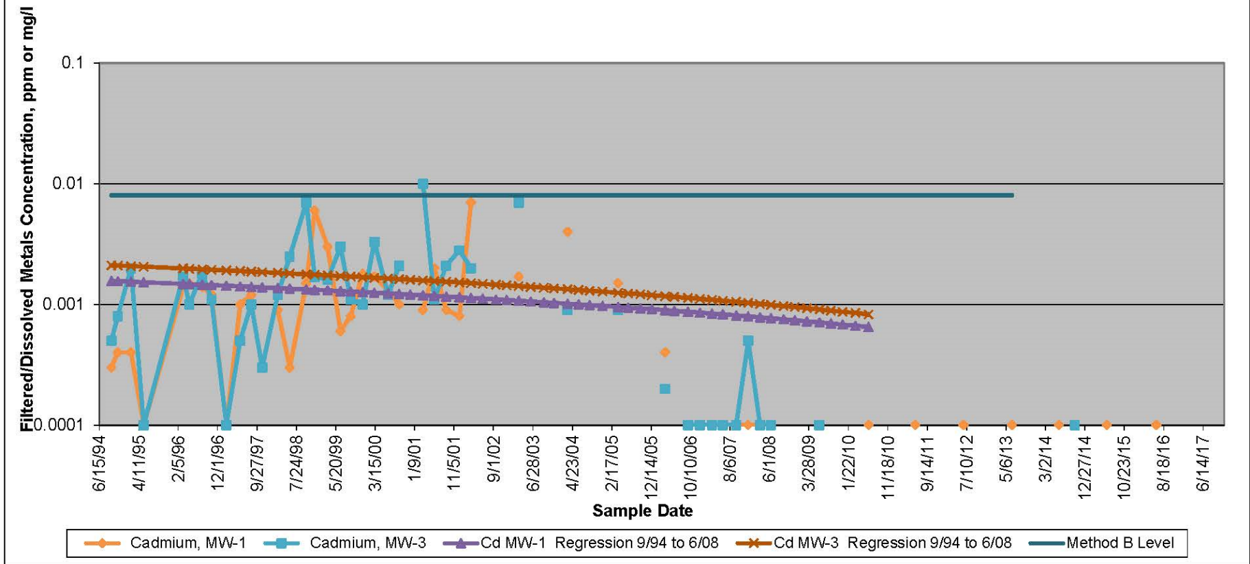
Figure 8. MW-1 and MW-3 Groundwater Cadmium Monitoring Results
