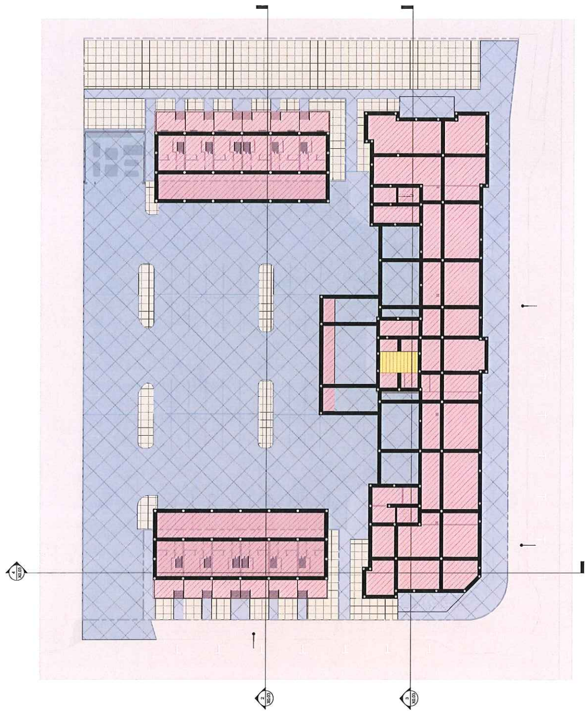
① EXCAVATION SITE PLAN 1/16" = 1'-0"
