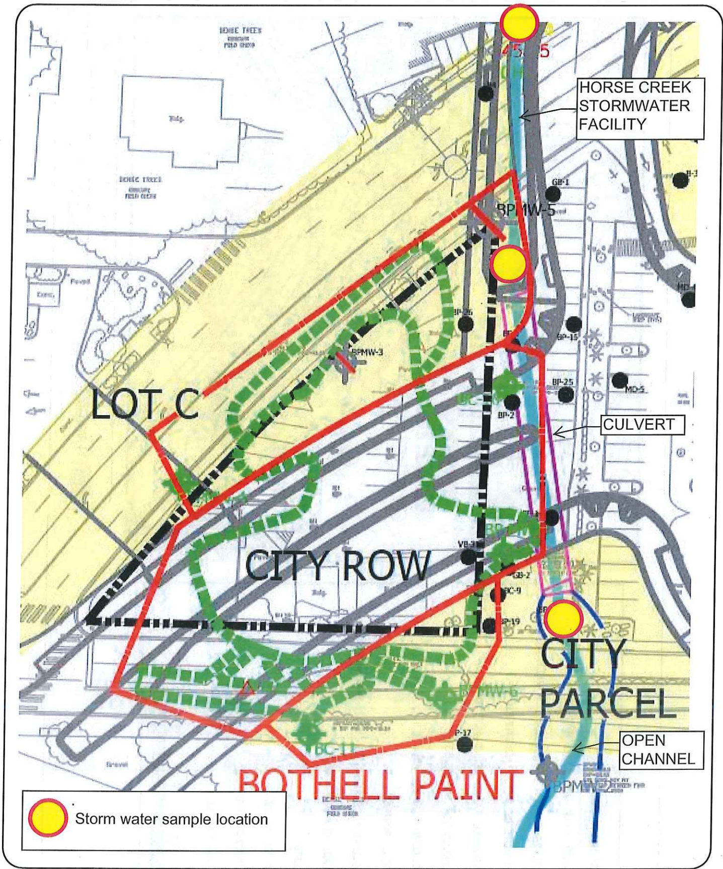
PROPOSED STORM WATER SAMPLING LOCATIONS
