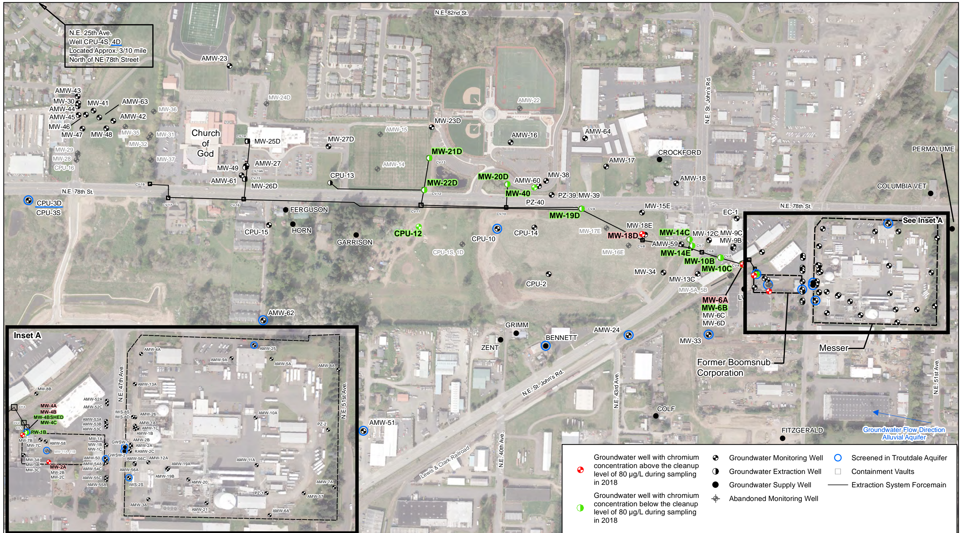
FIGURE 10 WELLS WITH CHROMIUM CONCENTRATIONS ABOVE THE CLEANUP LEVEL IN 2018
