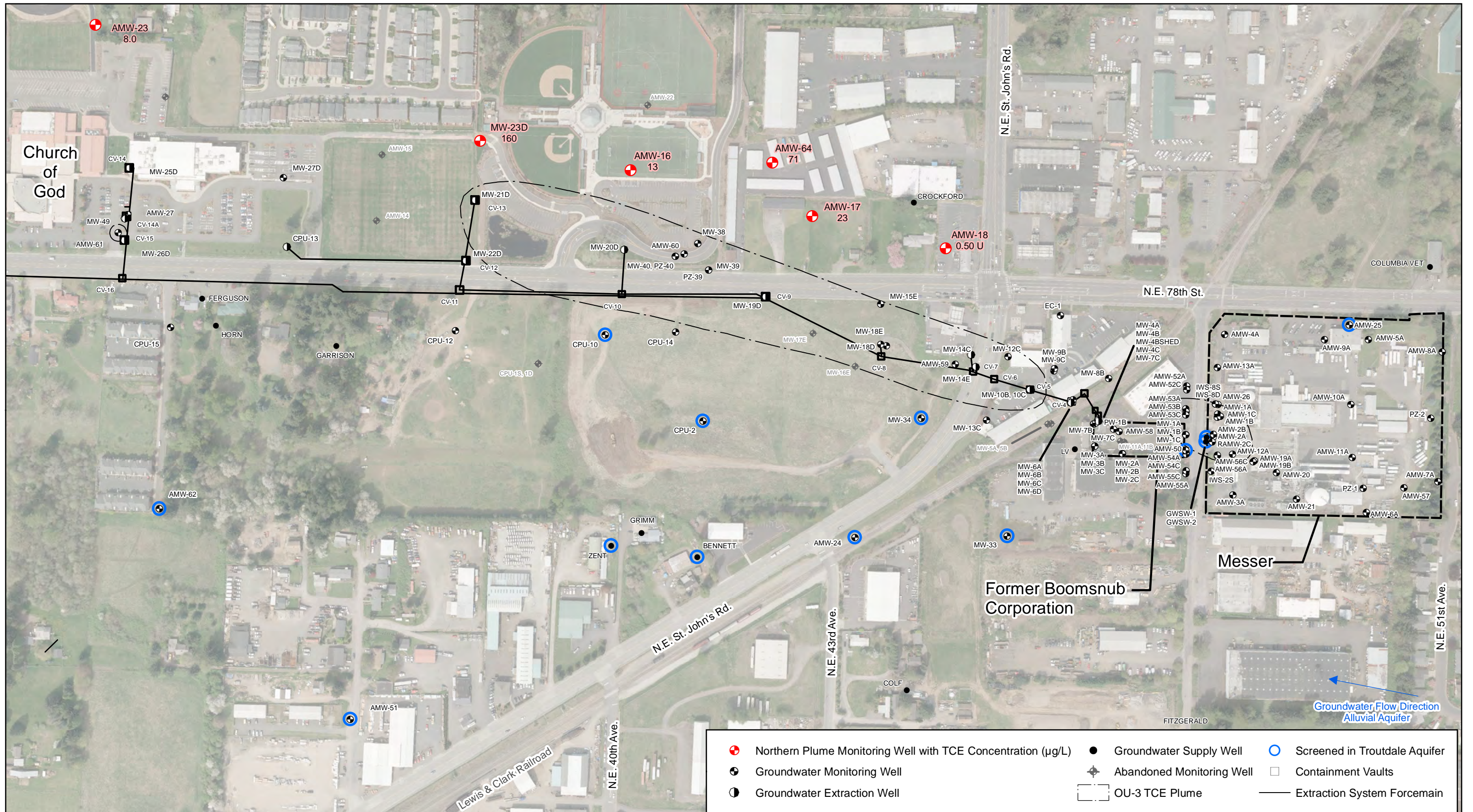
FIGURE D-1 NORTHERN PLUME MONITORING WELL LOCATIONS AND TRICHLOROETHENE CONCENTRATIONS, FALL 2018
