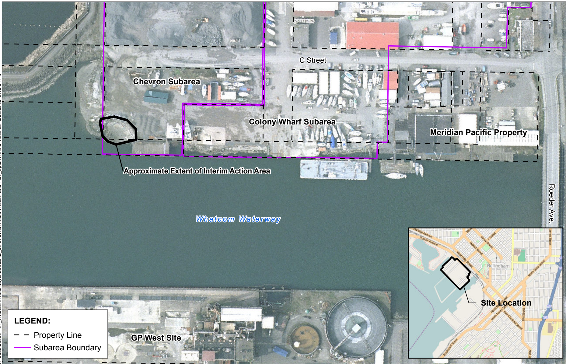
Figure 1 Site Plan Chevron Subarea Interim Action Central Waterfront Site Port of Bellingham
