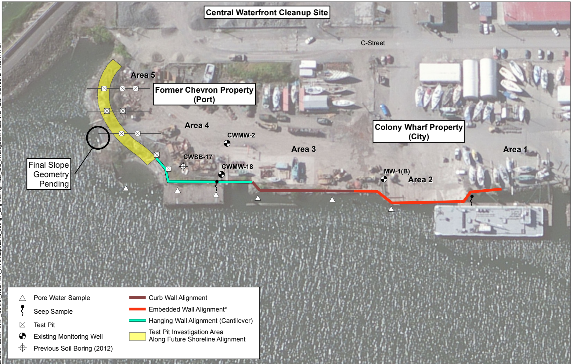
Figure 1 Supplemental Pre-Design Testing Locations and Central Waterfront Shoreline Features Whatcom Waterway Cleanup Project
