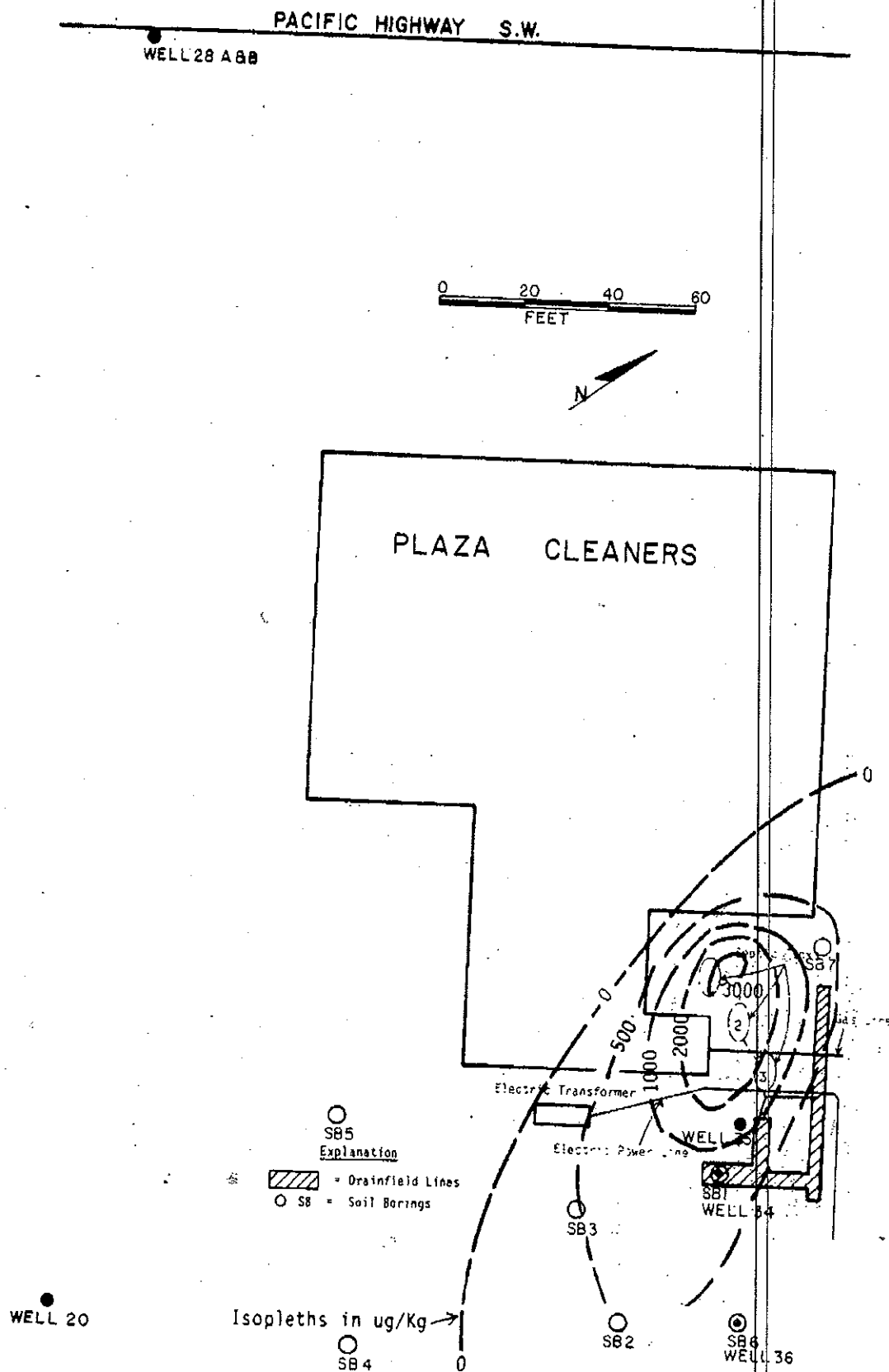
Figure 3.4. Concentration Distribution of PERC in the 0.0 to 5.0-ft Depth Interval on Plaza Cleaners' Property
