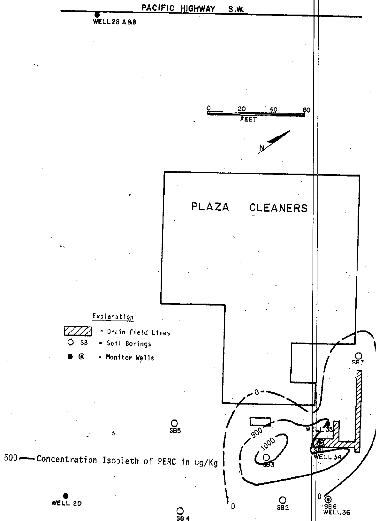
Figure 4. Extent of PERC Contamination in the Soil Under Plaza Cleaners at a Depth of 8.0 to 11.5 ft
