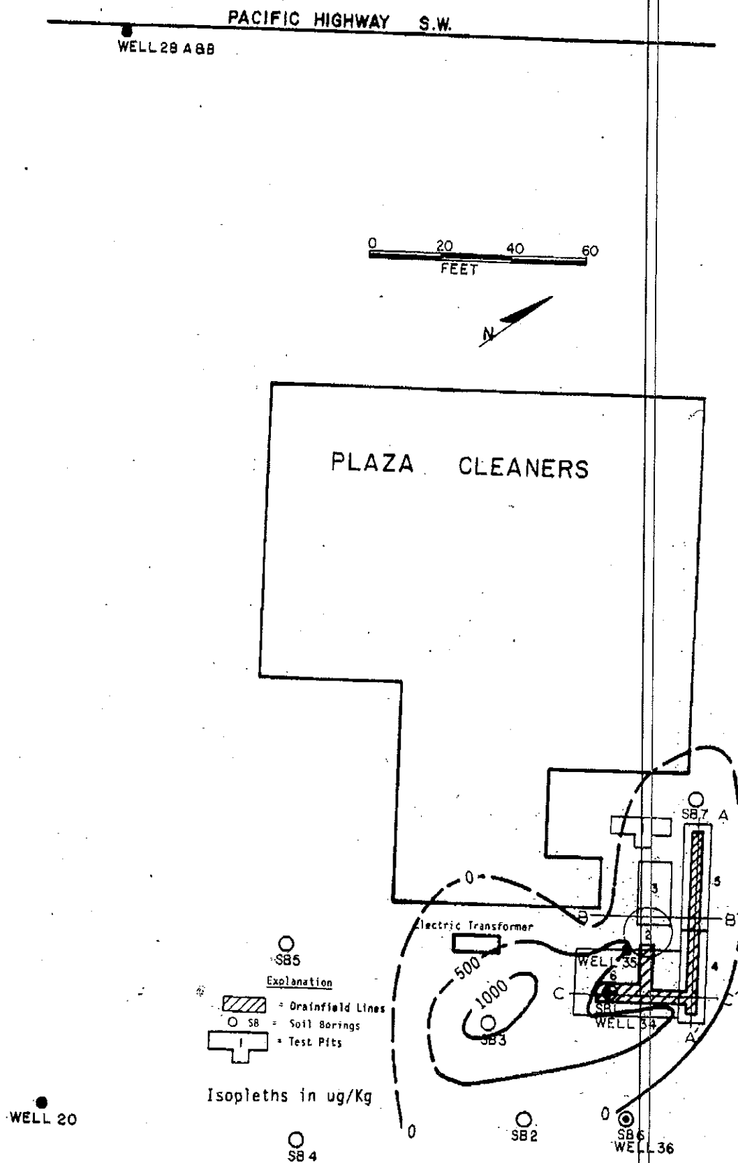
Figure 3.7. Concentration Distribution of PERC in the 8.5 to 11.5-ft Depth Interval on Plaza Cleaners' Property
