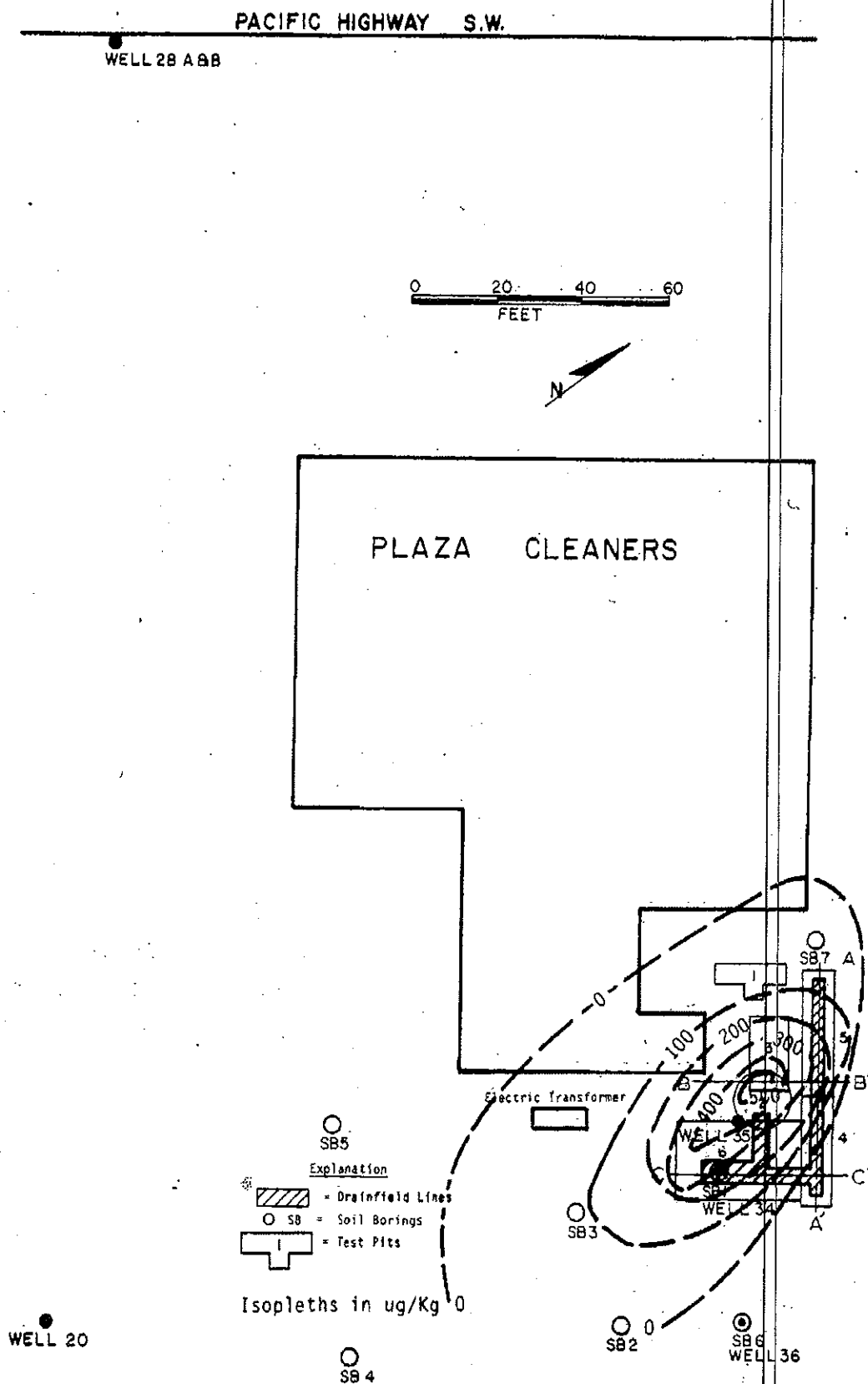
Figure 3.8. Concentration Distribution of PERC in the 11.5 to 12.5-ft Depth Interval on Plaza Cleaners' Property
