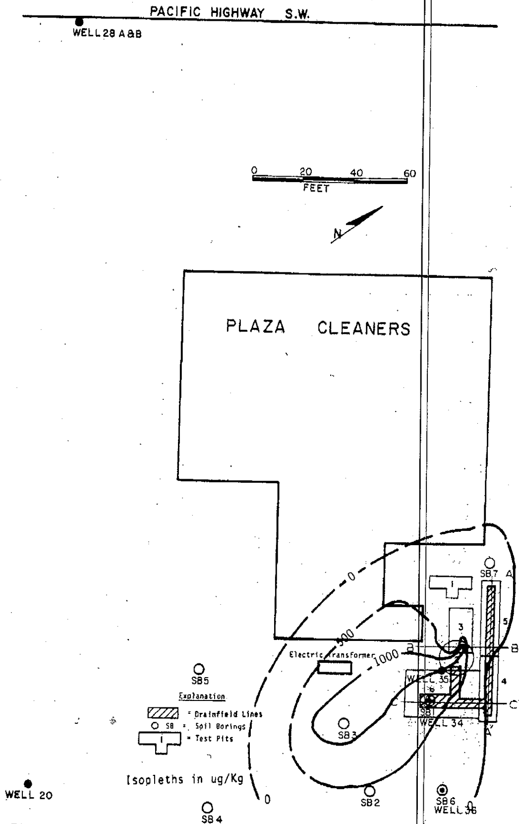
Figure 3.6. Concentration Distribution of PERC in the 7.0 to 8.5-ft Depth Interval on Plaza Cleaners' Property
