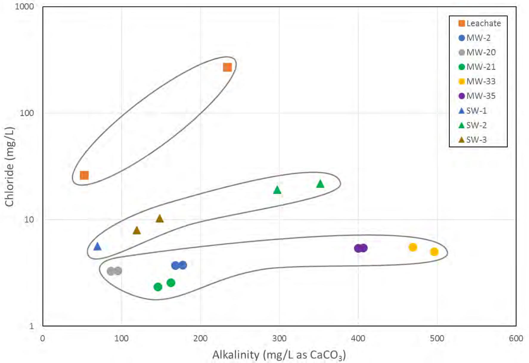
Figure 5 Cross-plot of Chloride Concentrations and Alkalinity
