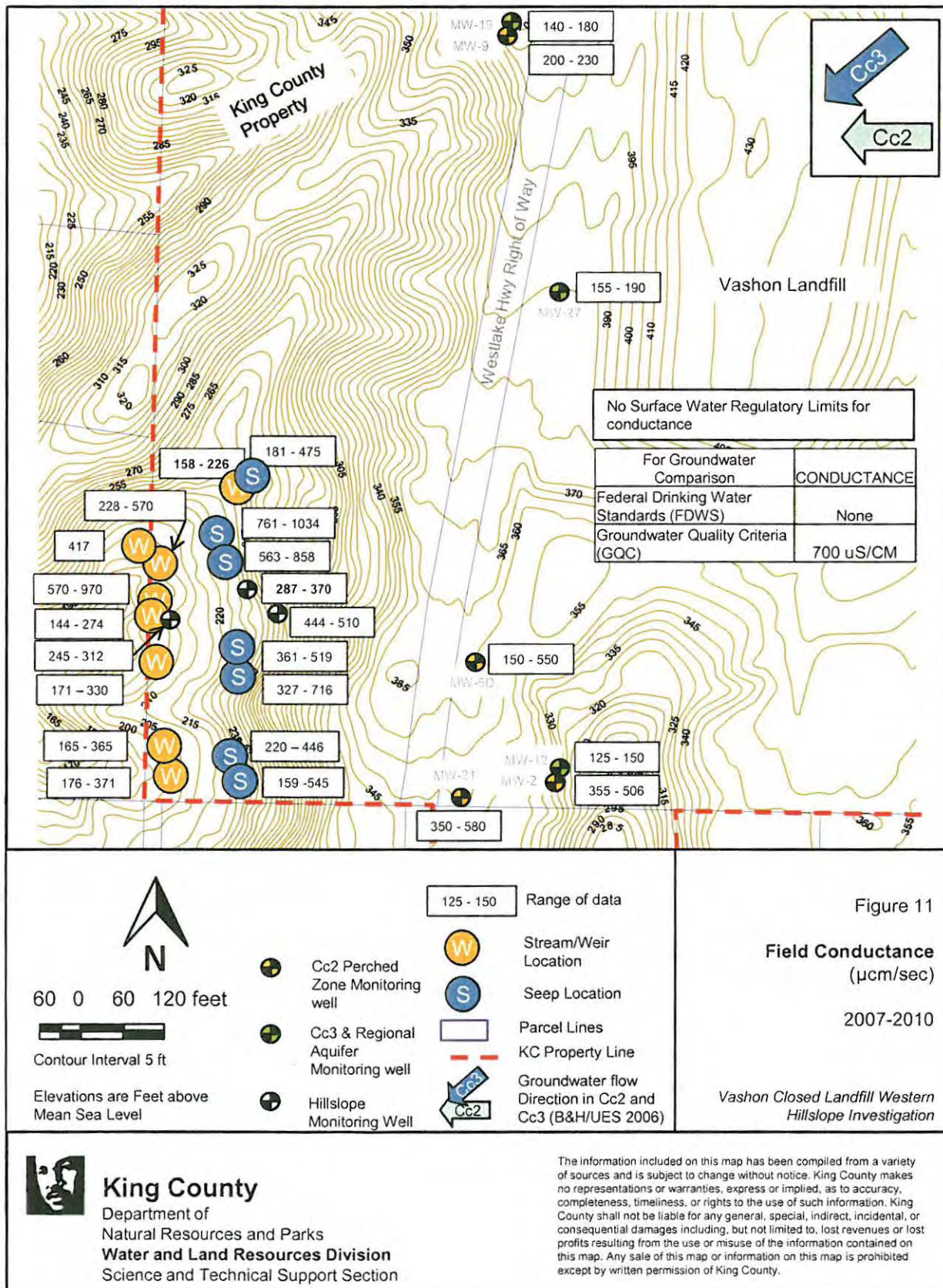
Figure 11. Field Conductance
