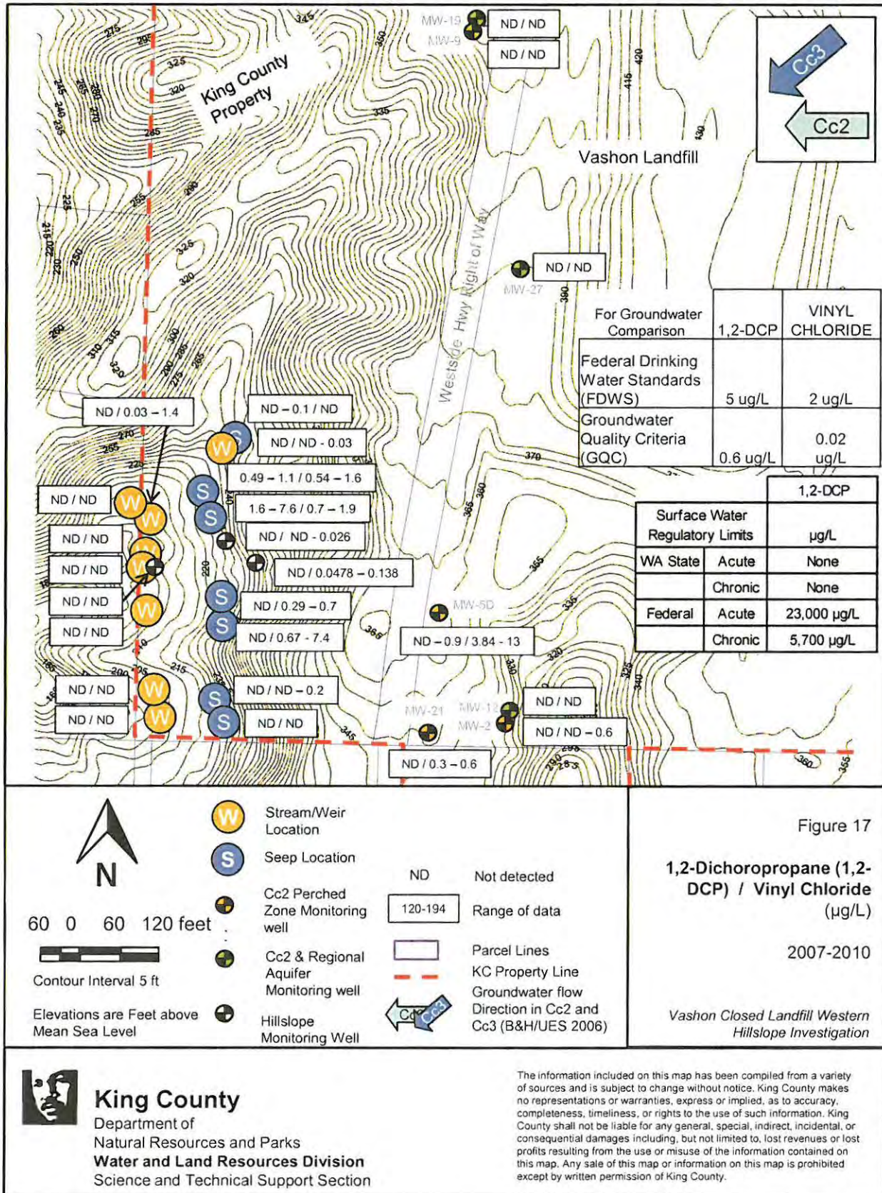
Figure 17. 1,2-Dichloropropane and Vinyl Chloride
