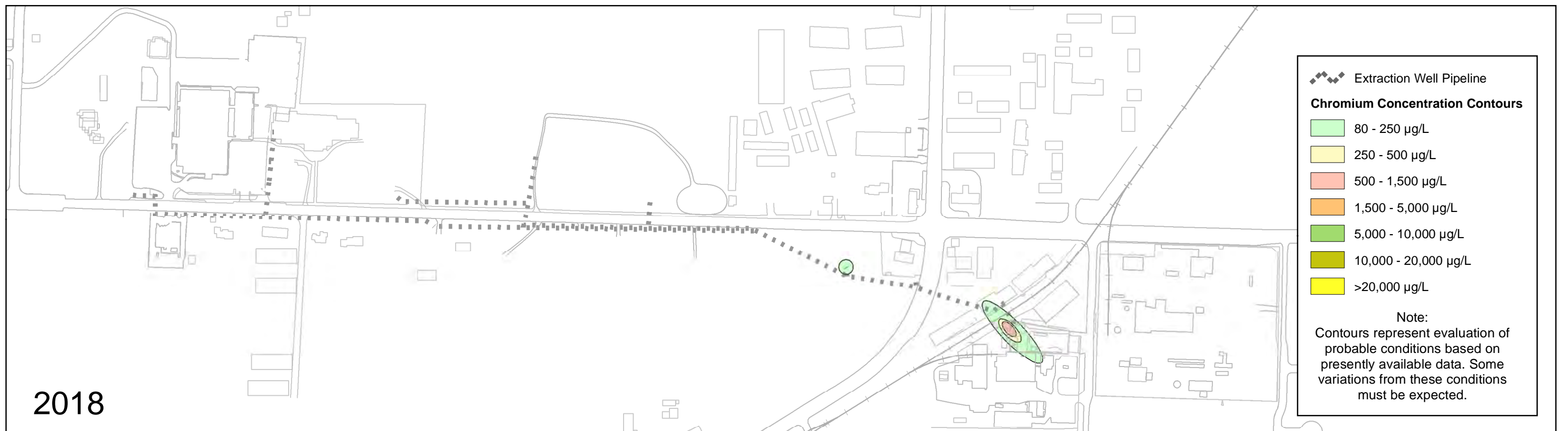
FIGURE 8 CHROMIUM PLUME COMPARISON 1995 VS. 2018
