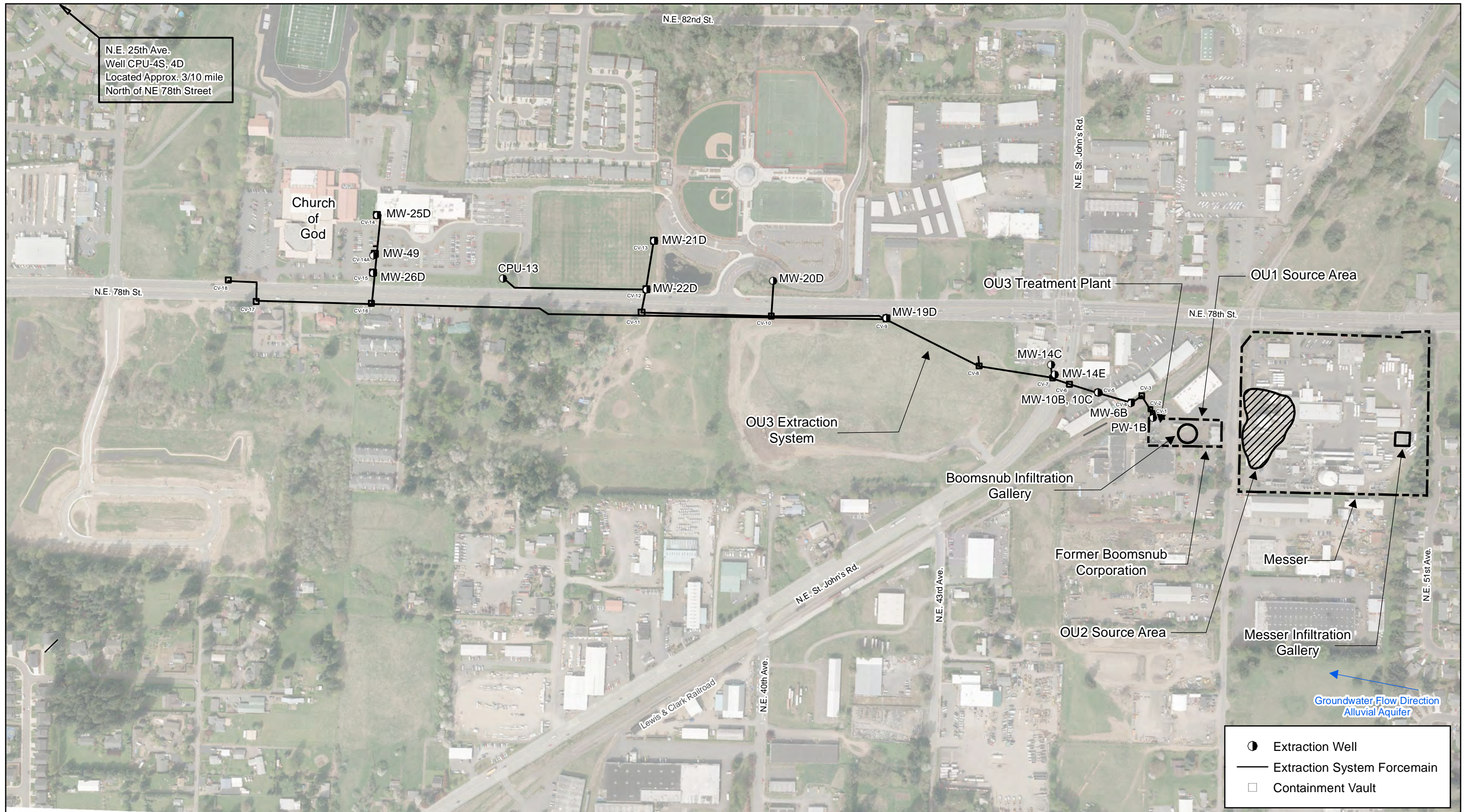
FIGURE 2 OPERABLE UNITS AND TREATMENT SYSTEM 2018
