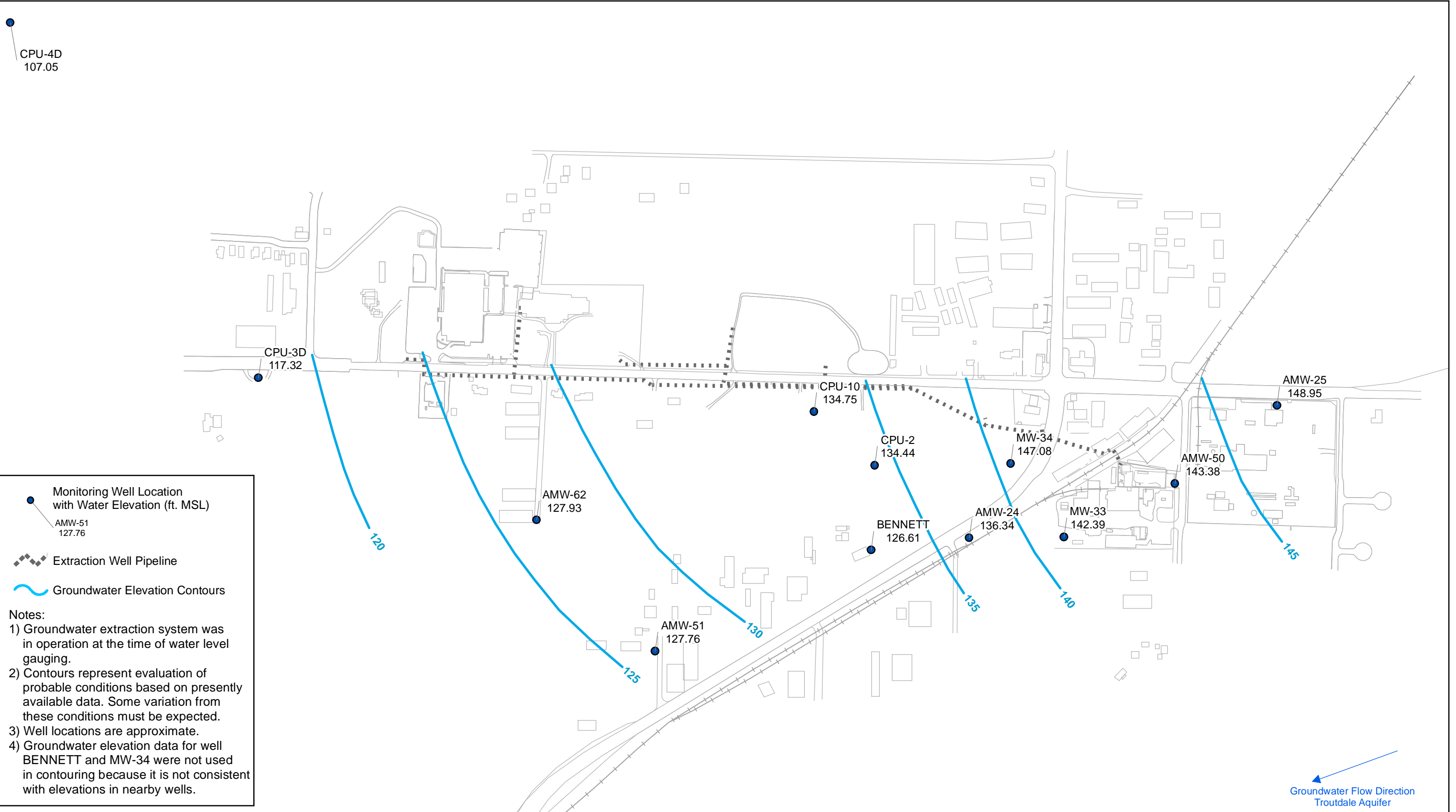
FIGURE 6 TROUTDALE AQUIFER GROUNDWATER CONTOURS FALL 2018
