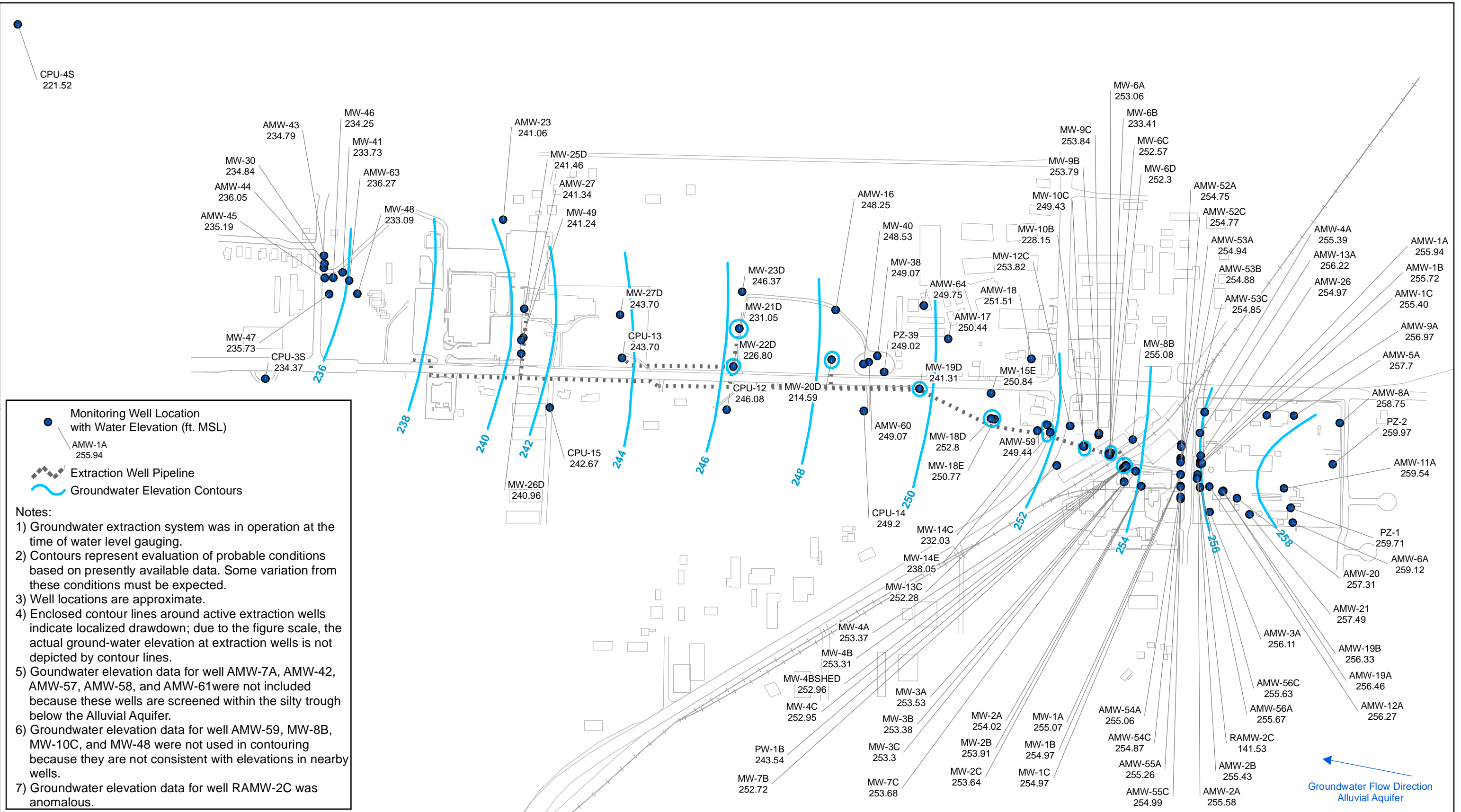
FIGURE 5 ALLUVIAL AQUIFER GROUNDWATER CONTOURS FALL 2018
