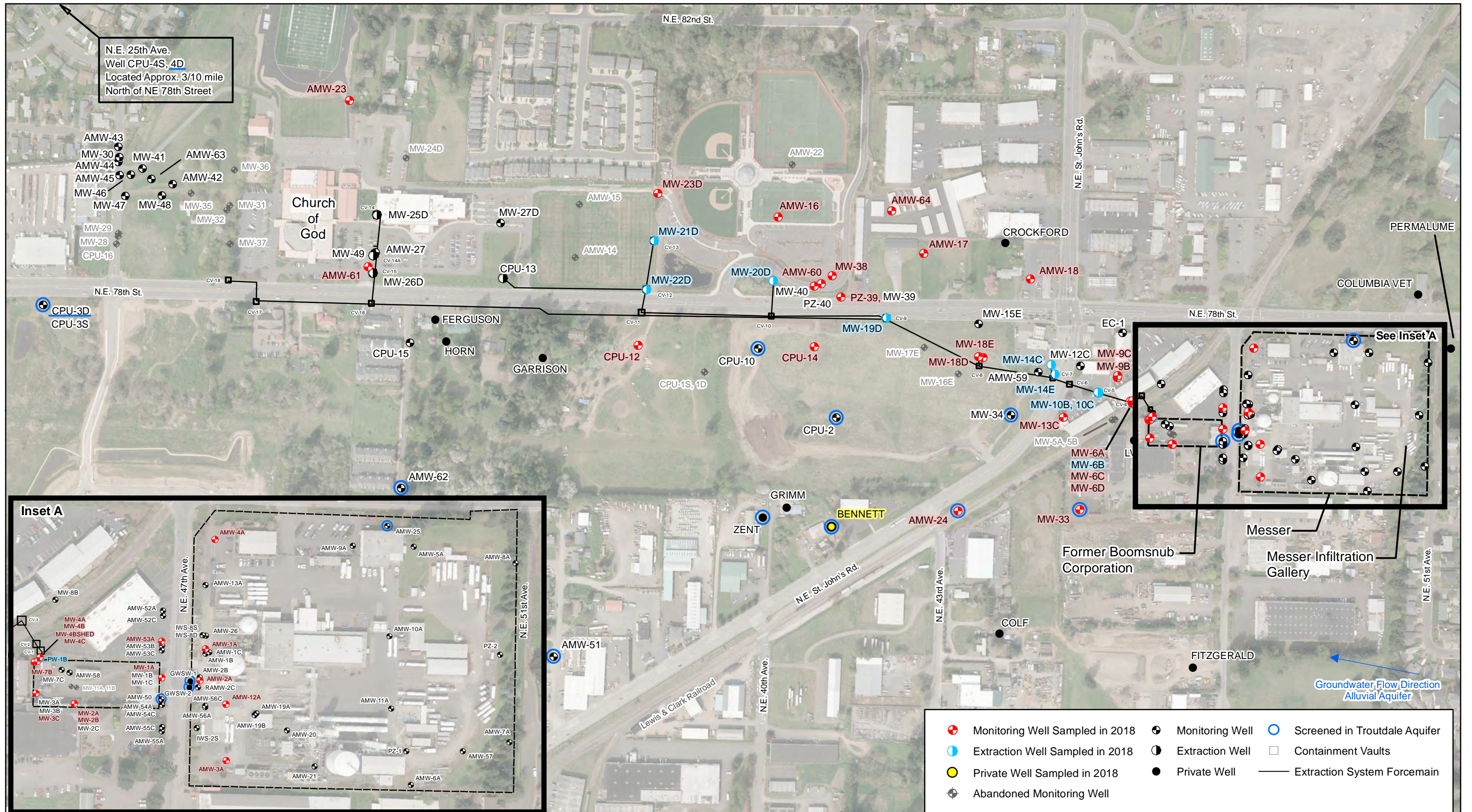
FIGURE 3 MONITORING AND EXTRACTION WELL NETWORK
