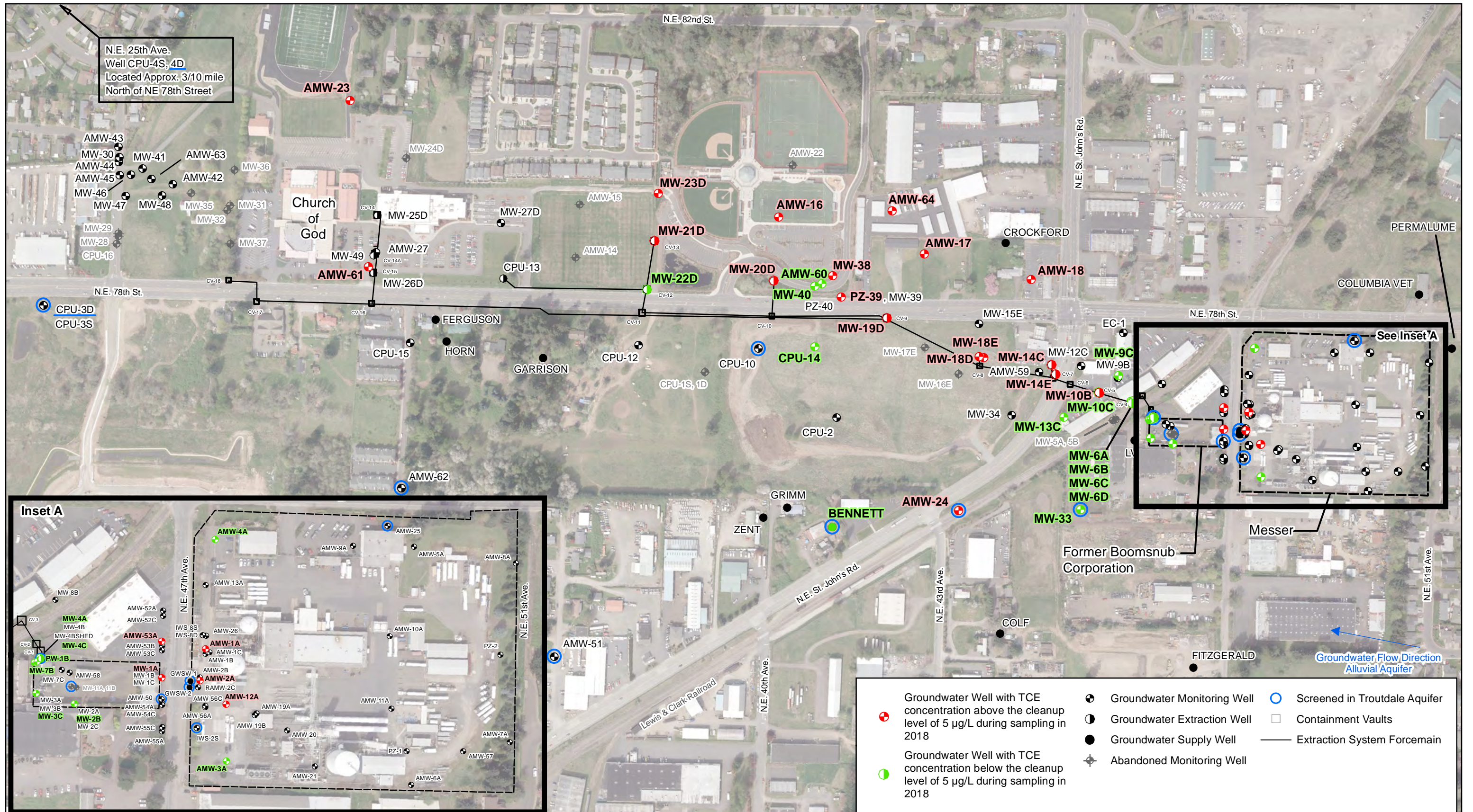
FIGURE 11 WELLS WITH TCE CONCENTRATIONS ABOVE THE CLEANUP LEVEL IN 2018
