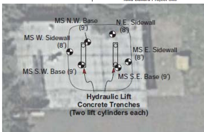
Figure 3 - Underground Storage Tank Excavation and Sampling Plan
