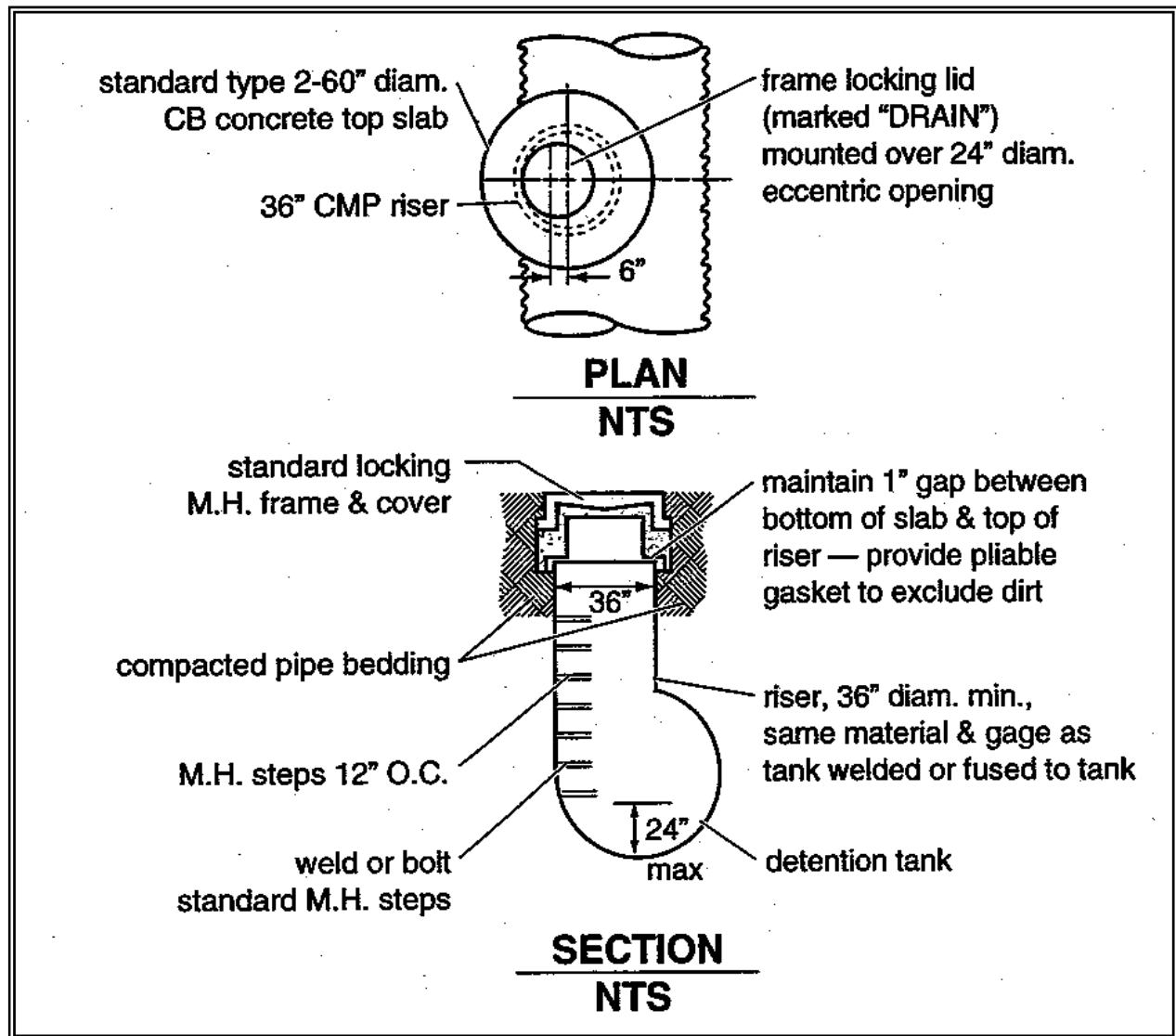
Figure 6.2.6 – Detention tank access detail
