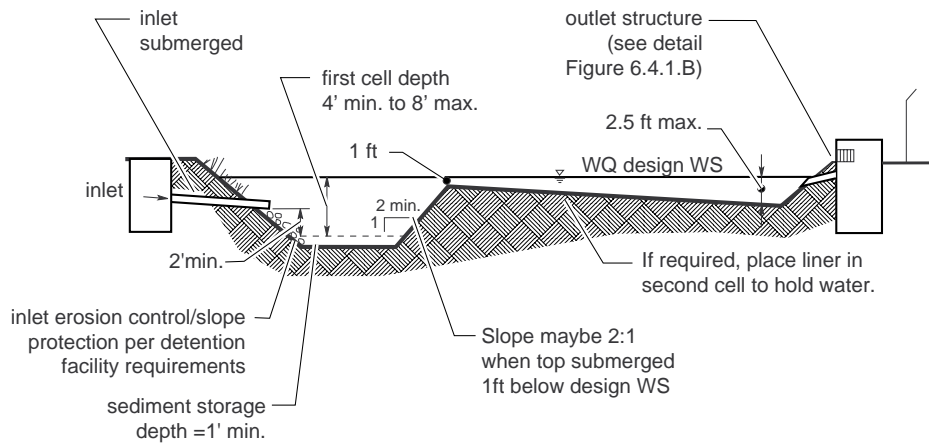
SECTION VIEW Option A NTS
