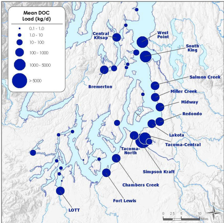
Figure G-15. Mean dissolved organic carbon loads from WWTPs during 2006-07.
