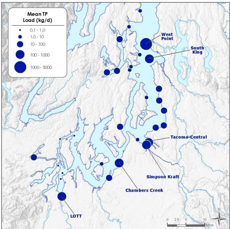
Figure G-12. Mean total phosphorus loads from WWTPs during 2006-07.
