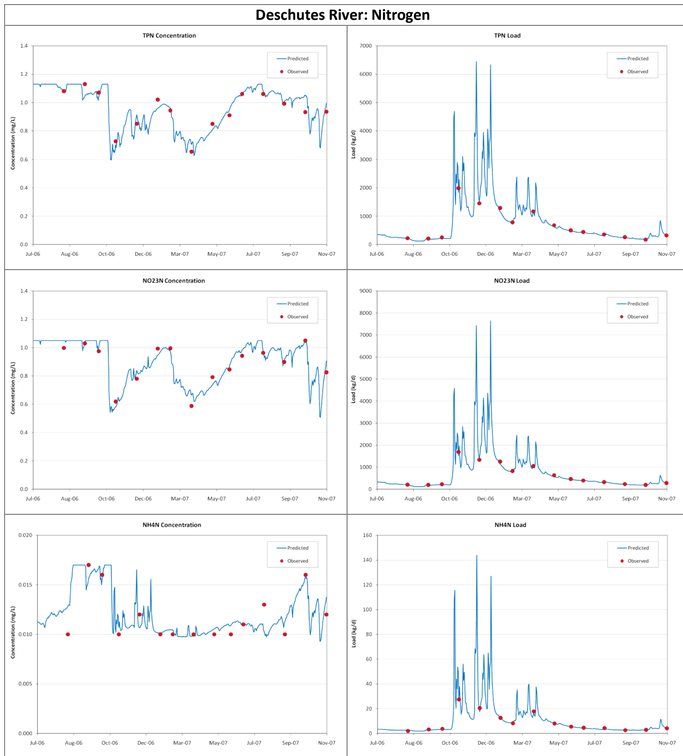
Figure D-1. Predicted and observed concentrations (left column) and loads (right column) of nitrogen for the Deschutes River.
