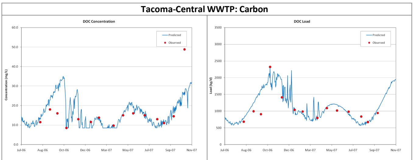
Figure E-11. Predicted and observed concentrations (left column) and loads (right column) of dissolved organic carbon (DOC) for the Tacoma-Central WWTP.
