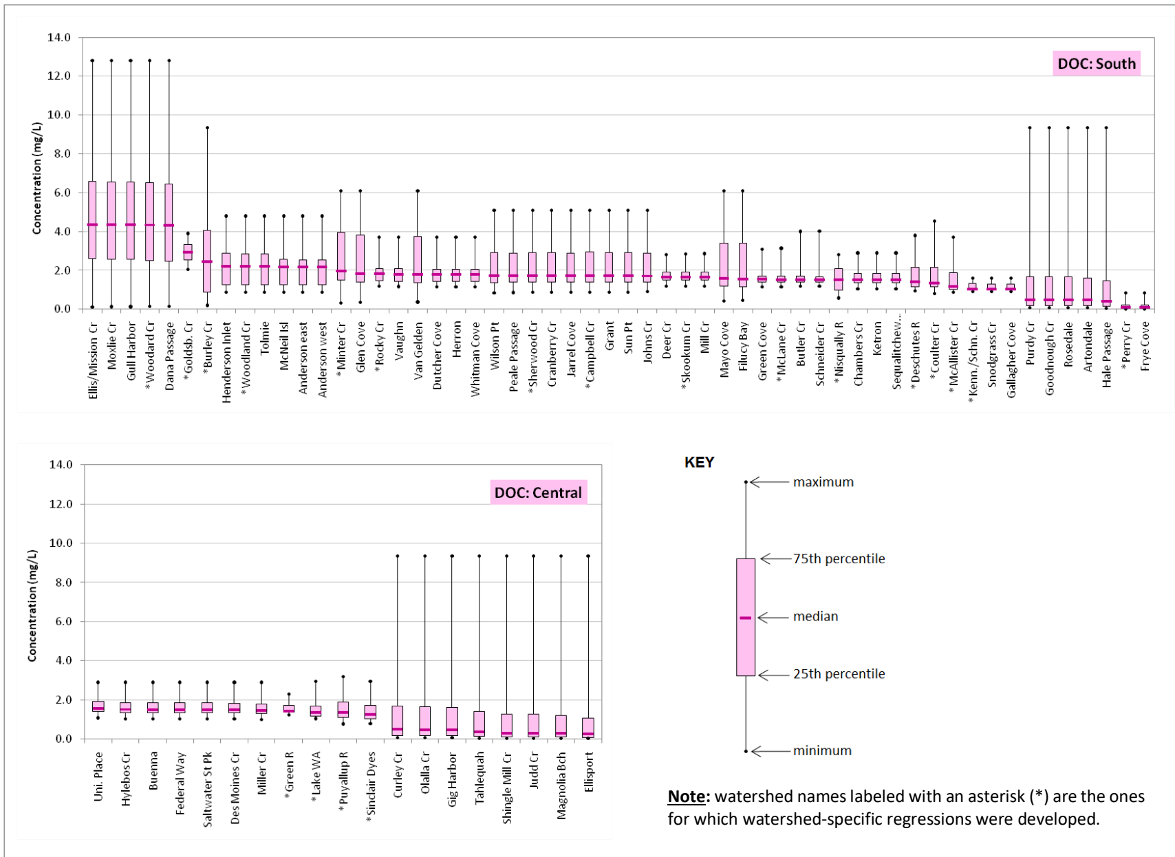
Figure F-7. Box plots of dissolved organic carbon concentrations for 2006-07 for watersheds in South (top) and Central (bottom) Puget Sound.
