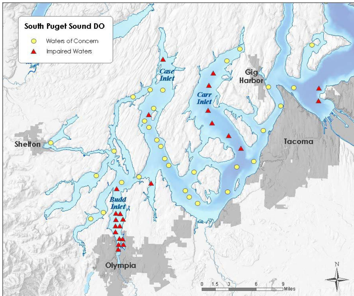
Figure 1. Results from the 2008 Water Quality Assessment for dissolved oxygen in South Puget Sound.
