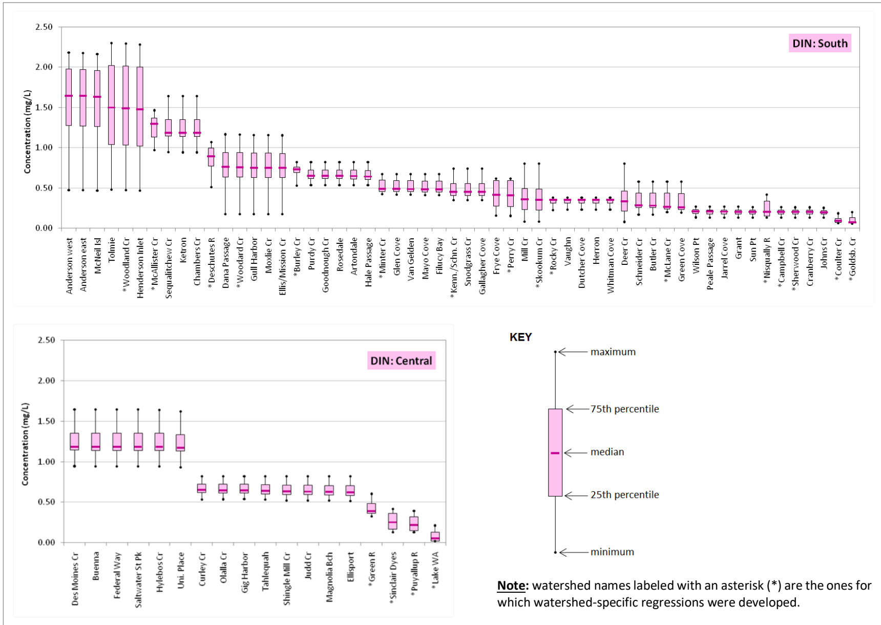
Figure 9. Box plots of dissolved inorganic nitrogen (DIN) concentrations for watersheds in South (top) and Central (bottom) Puget Sound, 2006-07.
