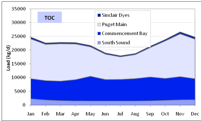
Figure G-18. Mean 2006-07 monthly organic carbon loads from WWTPs totaled according to the regions in South and Central Puget Sound into which they drain.
