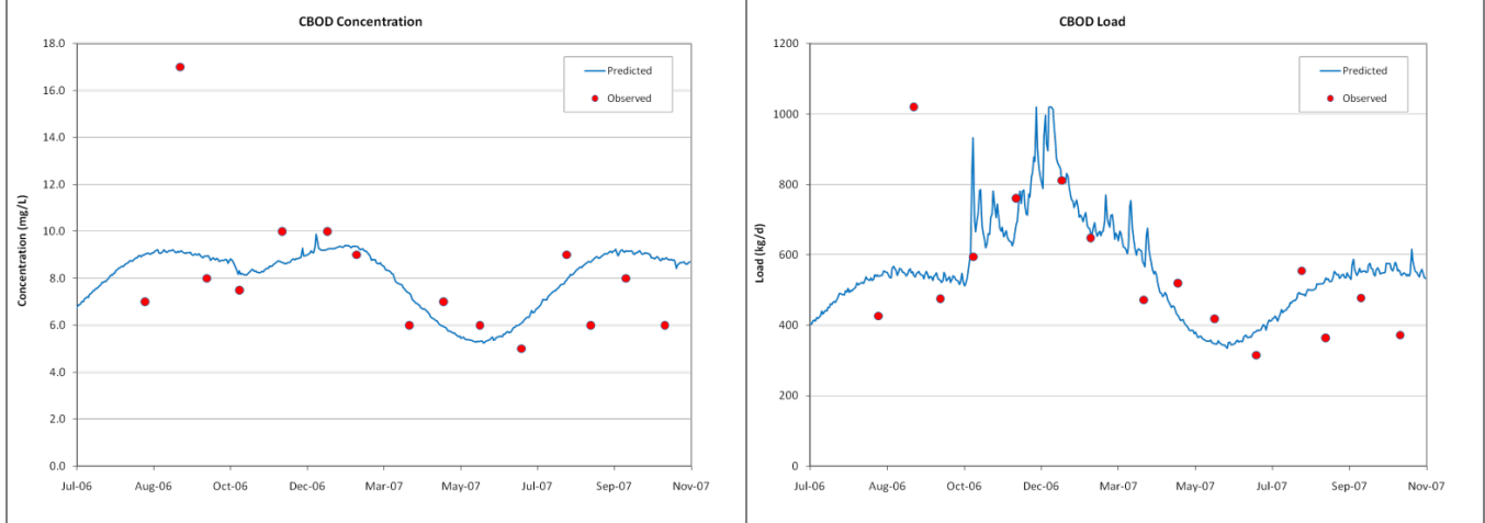
Figure E-4. Predicted and observed concentrations (left column) and loads (right column) of CBOD for the Chambers Creek WWTP.
