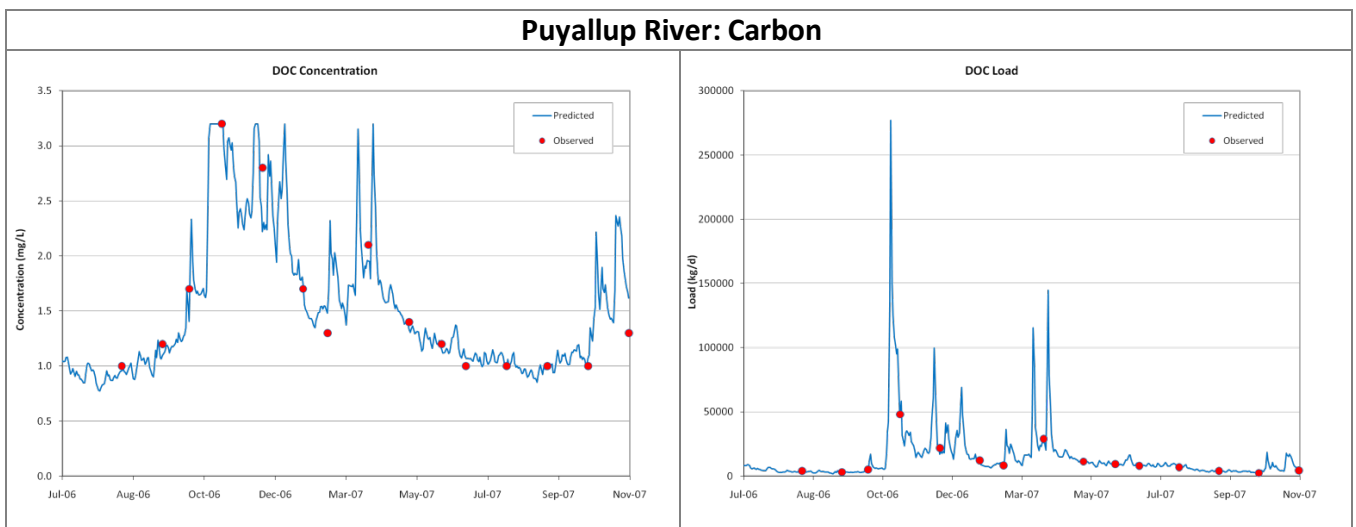
Figure D-12. Predicted and observed concentrations (left column) and loads (right column) of dissolved organic carbon (DOC) for the Puyallup River.
