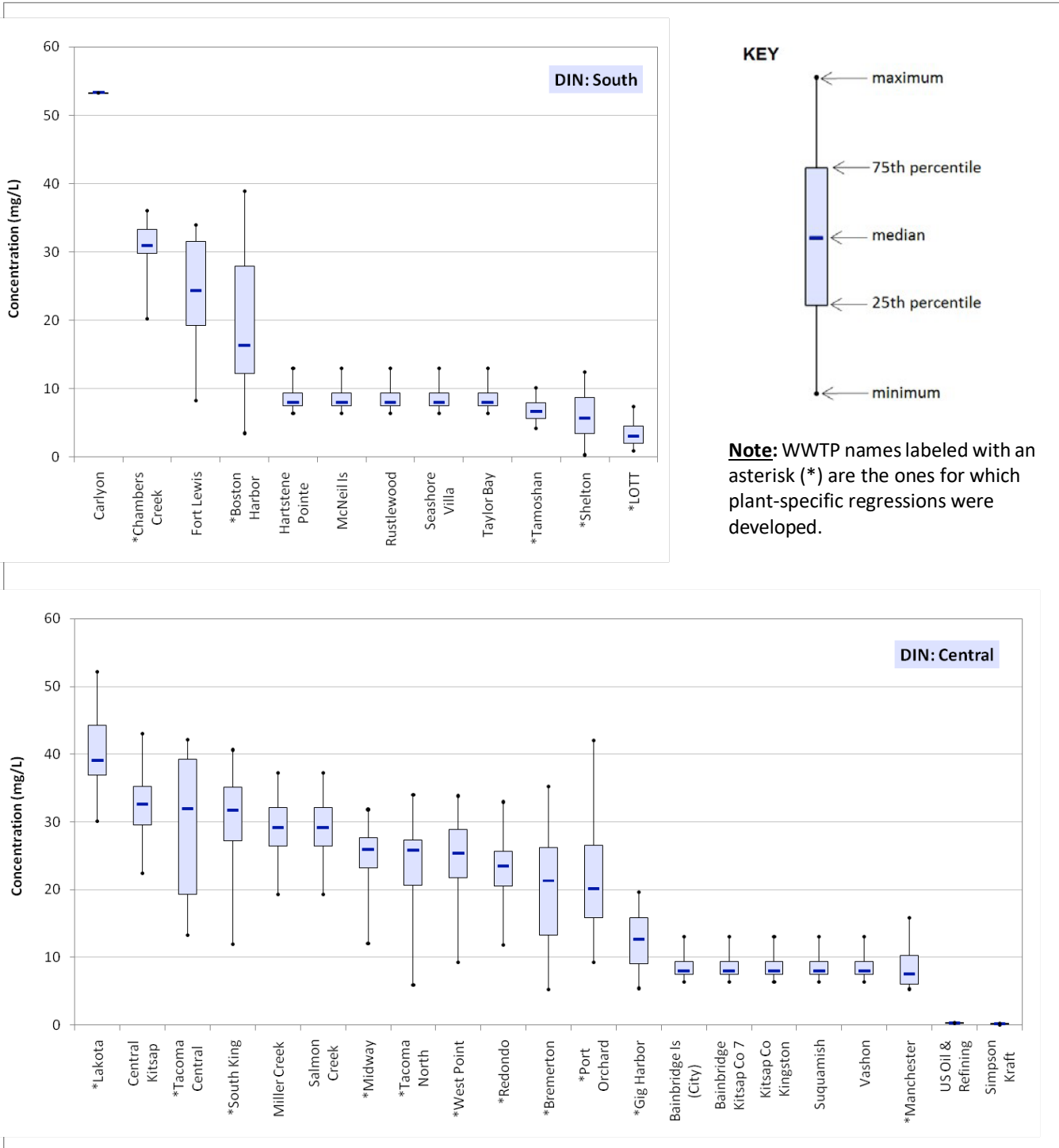
Figure 16. Box plots of dissolved inorganic nitrogen (DIN) concentrations for WWTPs in South (top) and Central (bottom) Puget Sound, 2006-07.
