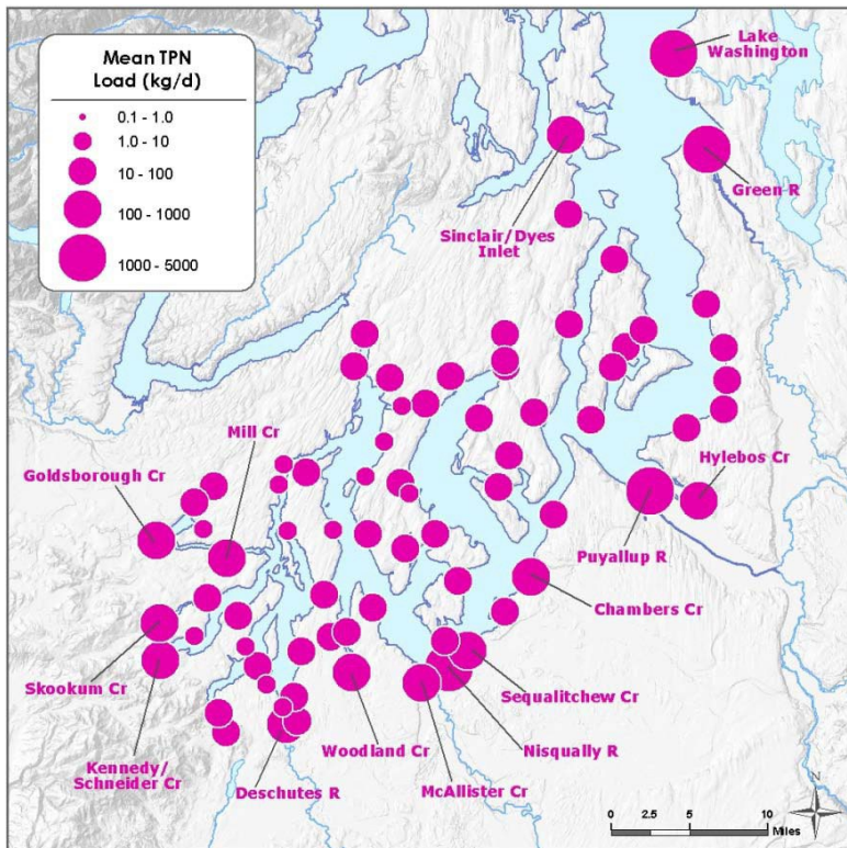
Figure F-8. Mean total persulfate nitrogen loads from watersheds during 2006-07.
