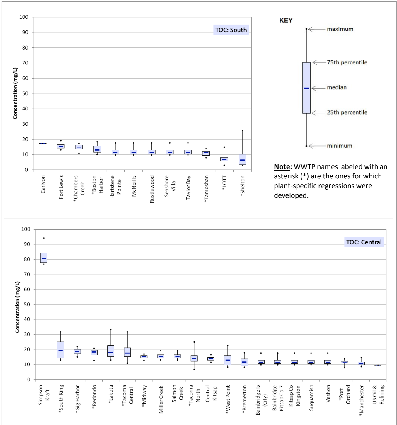
Figure G-6. Box plots of total organic carbon concentrations for 2006-07 for WWTPs in South (top) and Central (bottom) Puget Sound.
