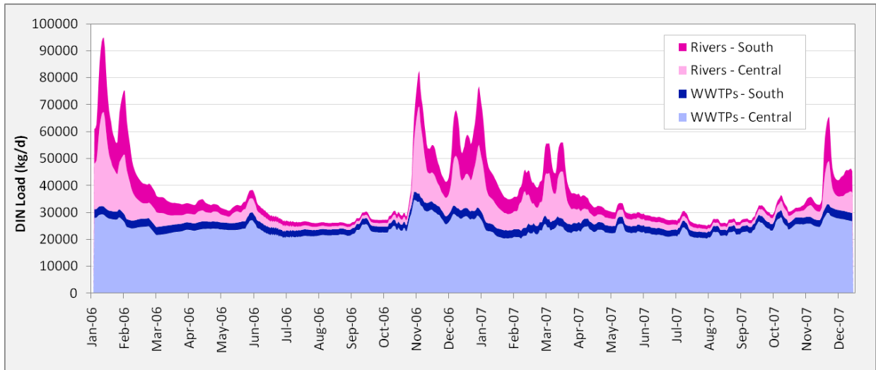
Figure ES-5. Seven-day average of daily dissolved inorganic nitrogen (DIN) loads from rivers and WWTPs into South and Central Puget Sound during 2006-07.
