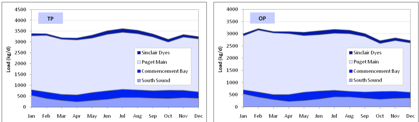
Figure G-17. Mean 2006-07 monthly phosphorus loads from WWTPs totaled according to the regions in South and Central Puget Sound into which they drain.
