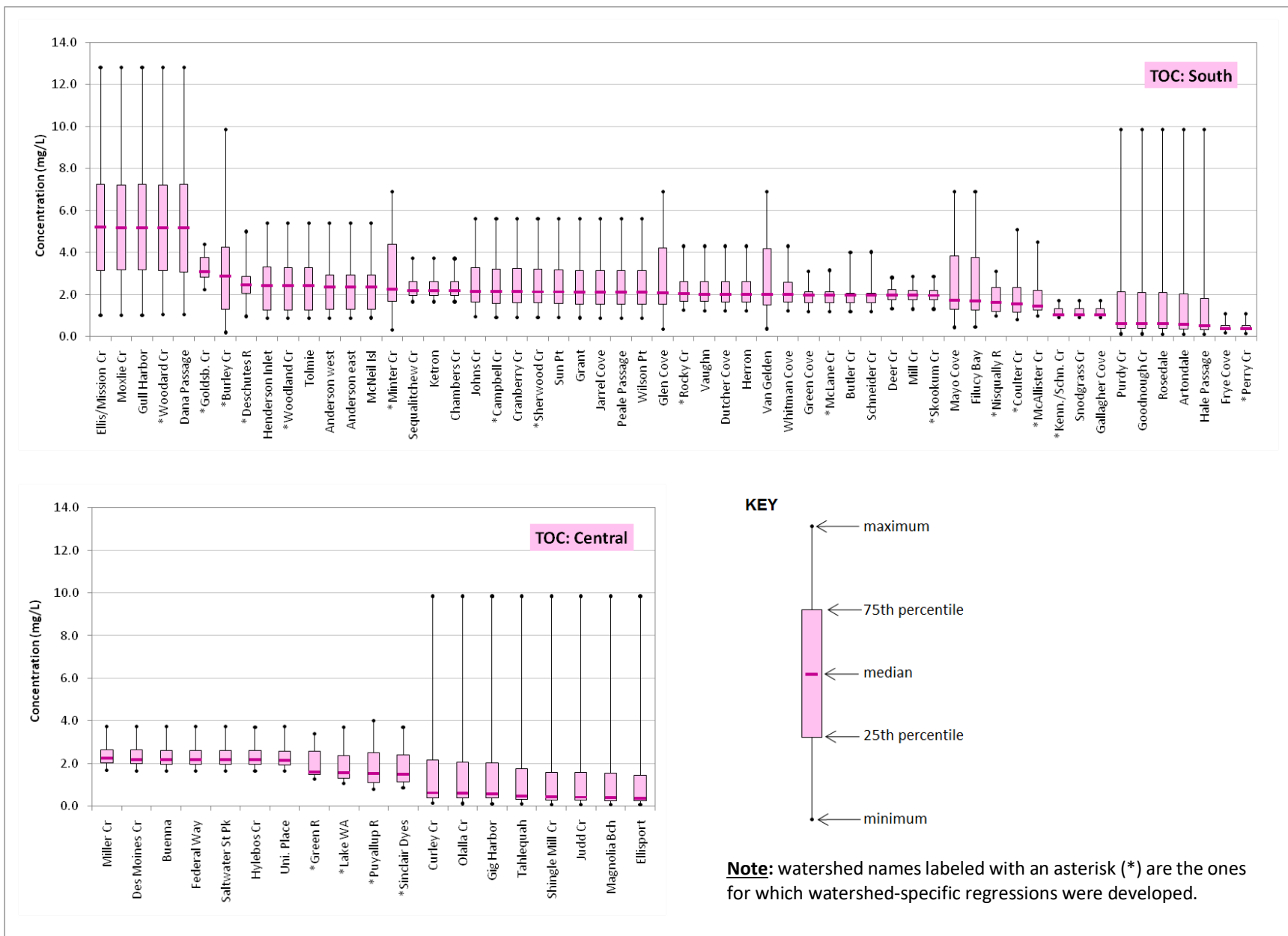
Figure F-6. Box plots of total organic carbon concentrations for 2006-07 for watersheds in South (top) and Central (bottom) Puget Sound.
