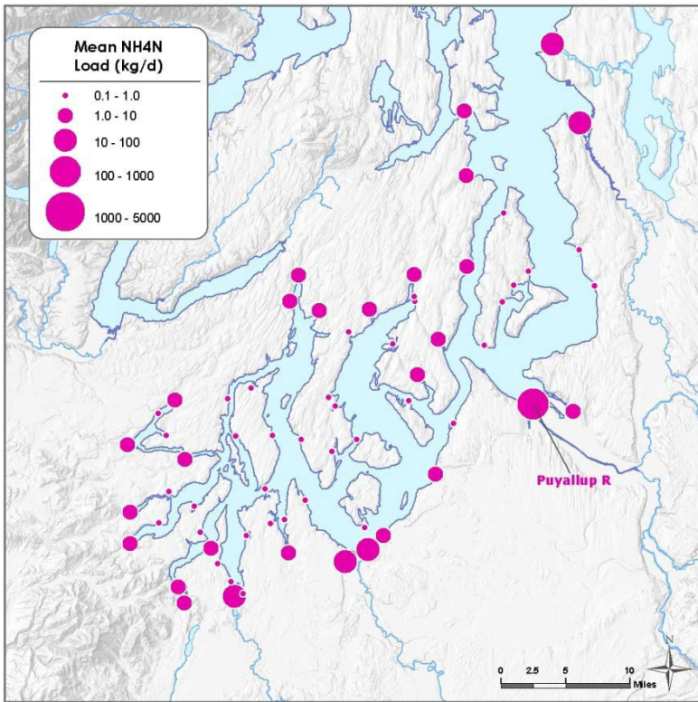
Figure F-10. Mean ammonium loads from watersheds during 2006-07.
