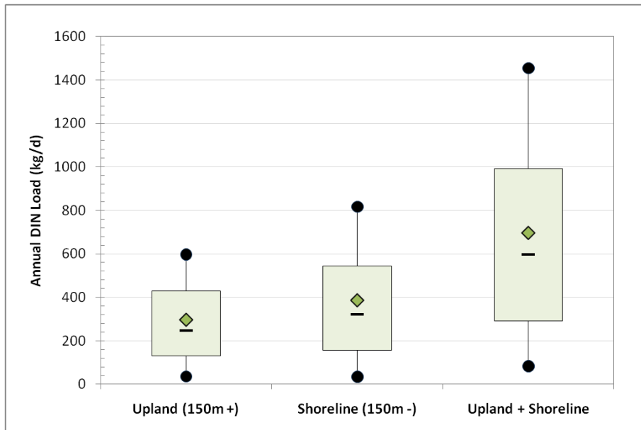
Figure 14. On-site septic systems dissolved inorganic nitrogen (DIN) loading estimates from upland regions, shoreline regions, and both regions combined for water year 2007.
