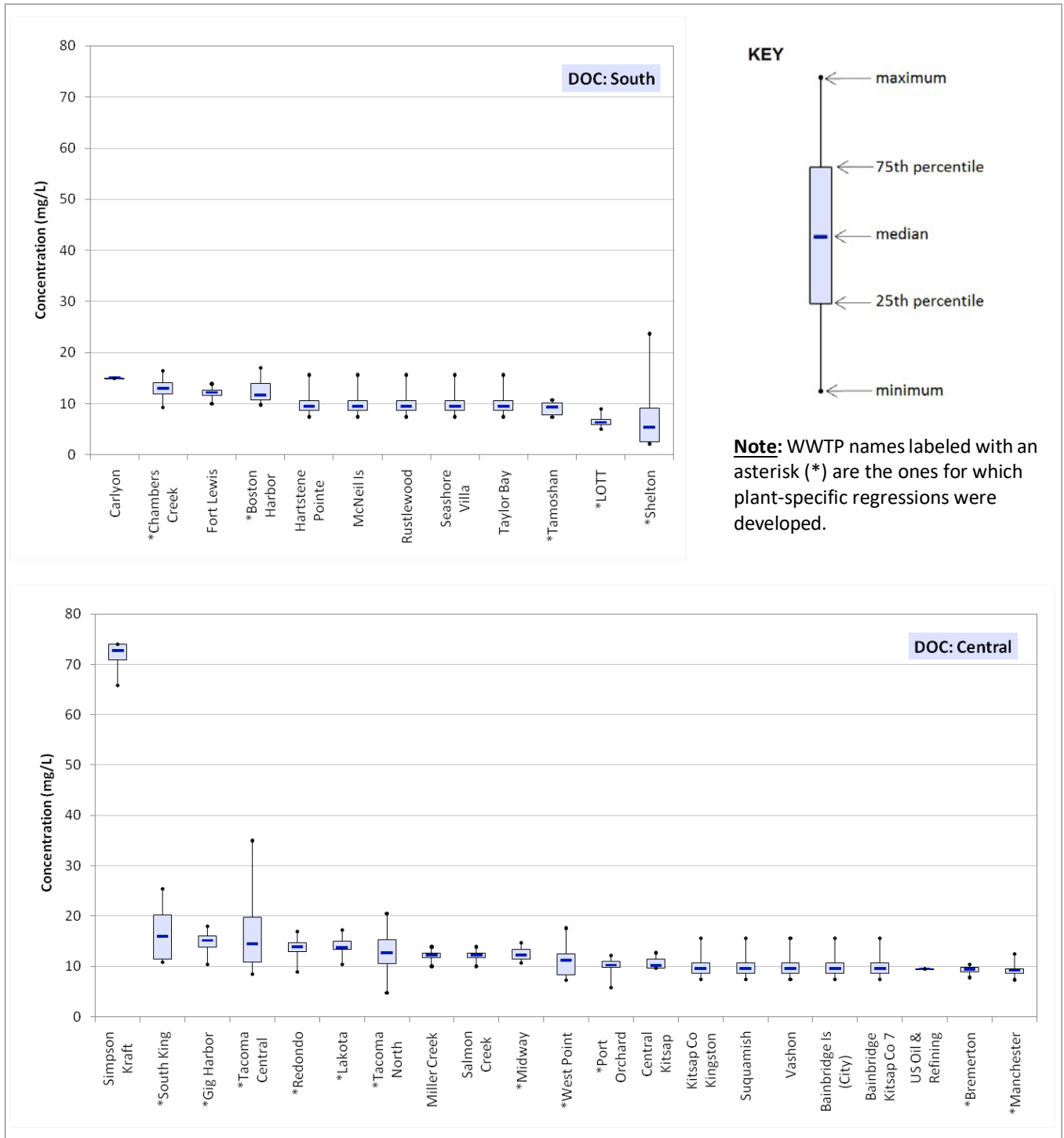
Figure G-7. Box plots of dissolved organic carbon concentrations for 2006-07 for WWTPs in South (top) and Central (bottom) Puget Sound.
