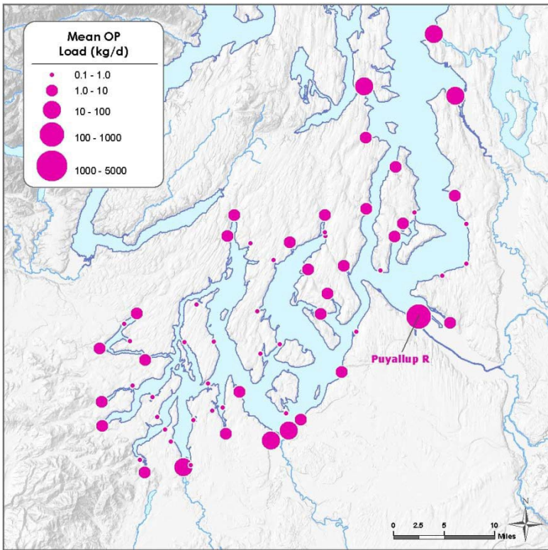
Figure F-12. Mean ortho-phosphate loads from watersheds during 2006-07.
