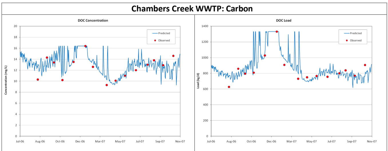
Figure E-3. Predicted and observed concentrations (left column) and loads (right column) of dissolved organic carbon (DOC) for the Chambers Creek WWTP.
