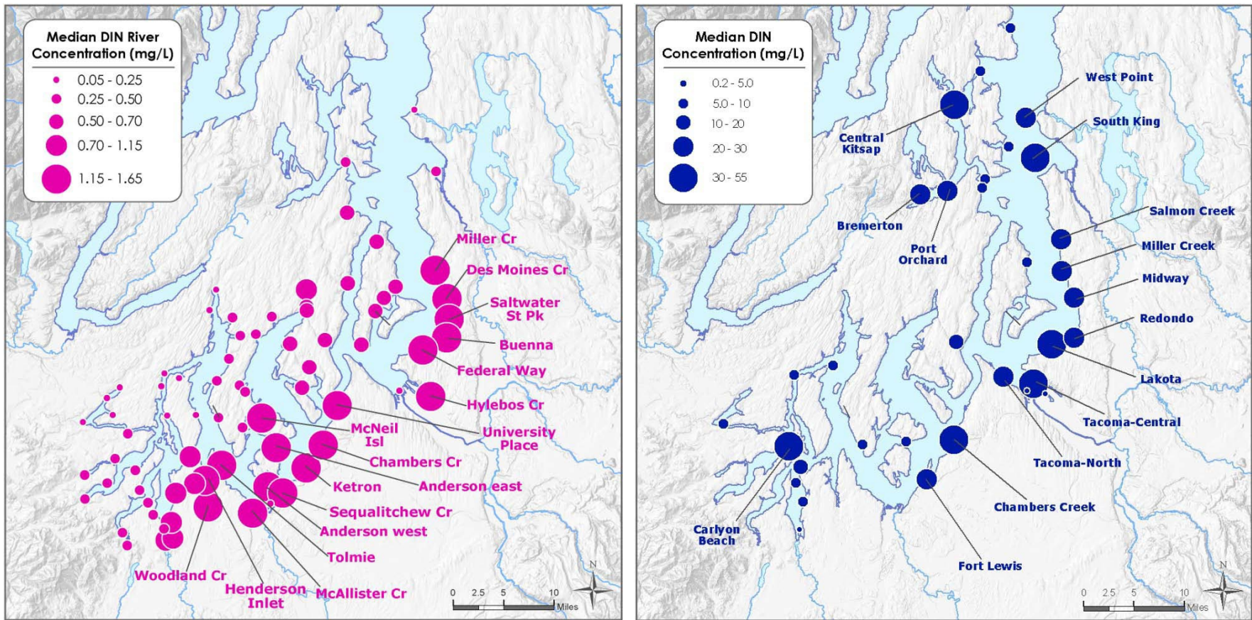
Figure ES-2. Median river (left) and WWTP (right) dissolved inorganic nitrogen (DIN) concentrations for 2006-07.
