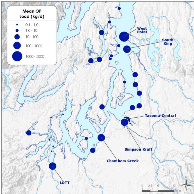
Figure G-13. Mean ortho-phosphate loads from WWTPs during 2006-07.
