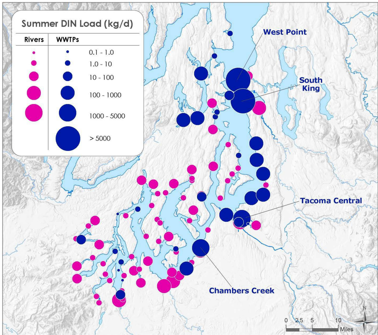
Figure ES-4. Mean summer dissolved inorganic nitrogen (DIN) loads from rivers and WWTPs into South and Central Puget Sound from 2006-07.
