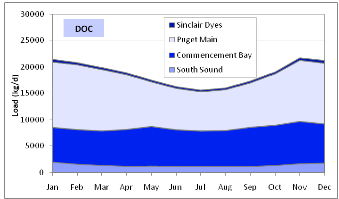
Figure G-18. Mean 2006-07 monthly organic carbon loads from WWTPs totaled according to the regions in South and Central Puget Sound into which they drain.
