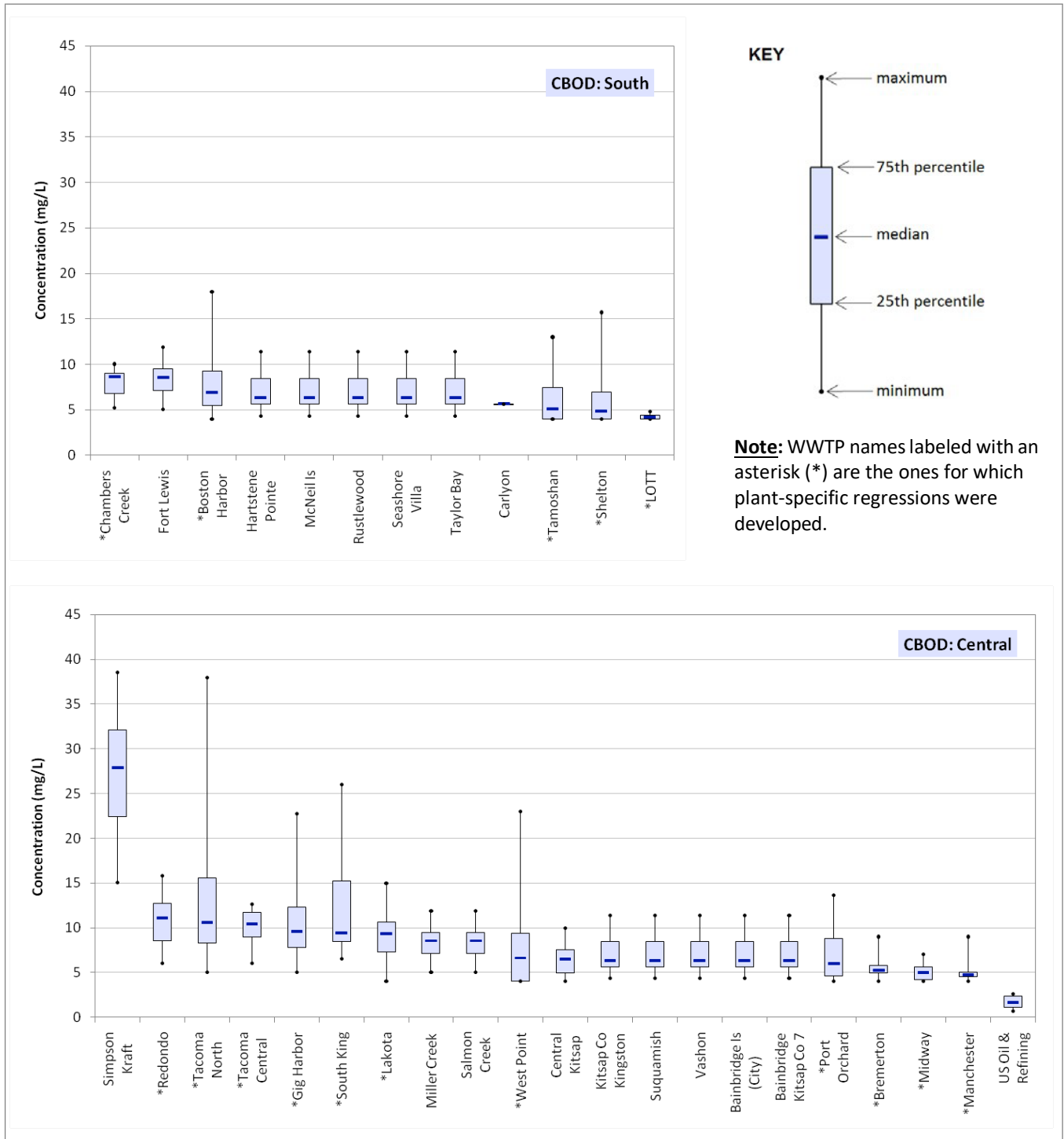
Figure G-8. Box plots of carbonaceous biochemical oxygen demand concentrations for 2006-07 for WWTPs in South (top) and Central (bottom) Puget Sound.
