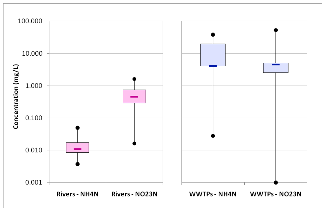
Figure 19. Box plots comparing the range of median concentrations of NH 4 N and NO 2 3N across all rivers and WWTPs in the study area, 2006-07.
