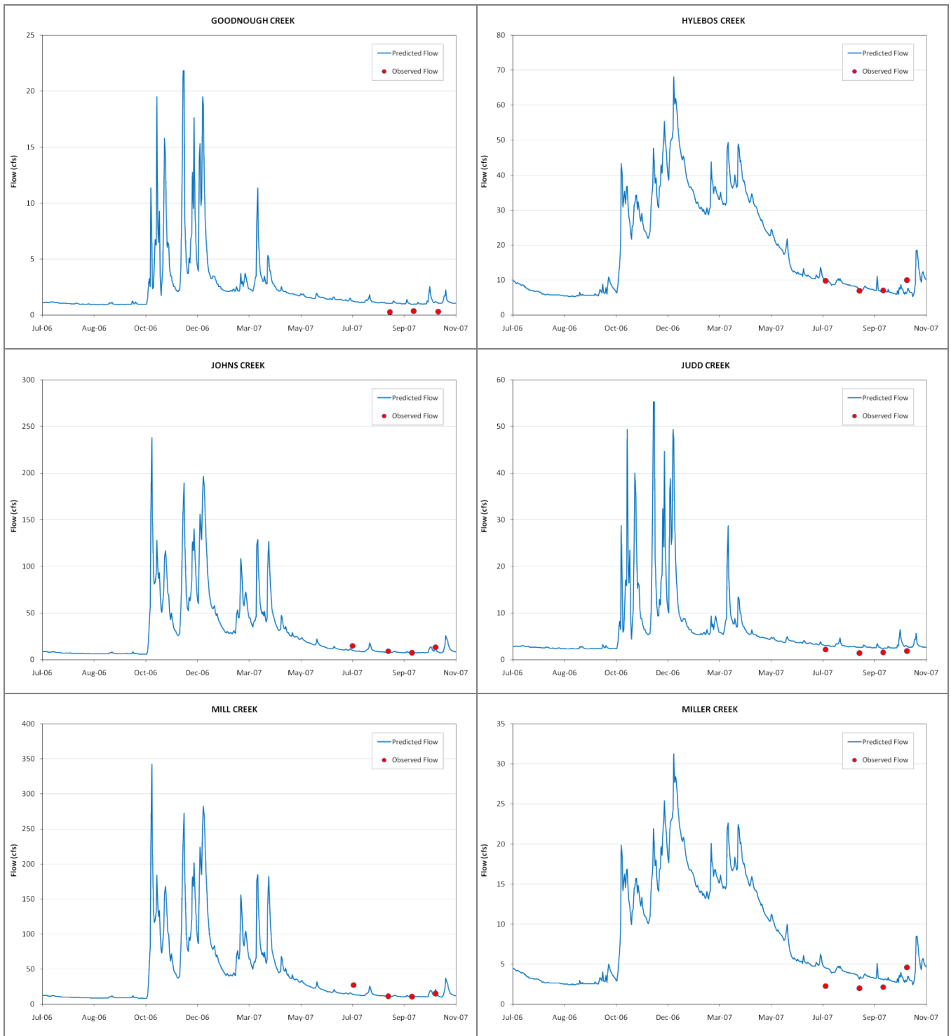
Figure B-4. Predicted and observed flows on creeks where four months of data were collected between July 2006 and October 2007.
