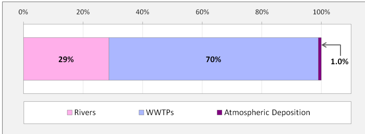
Figure 26. Annual dissolved inorganic nitrogen (DIN) loads from rivers, WWTPs, and the atmosphere.
