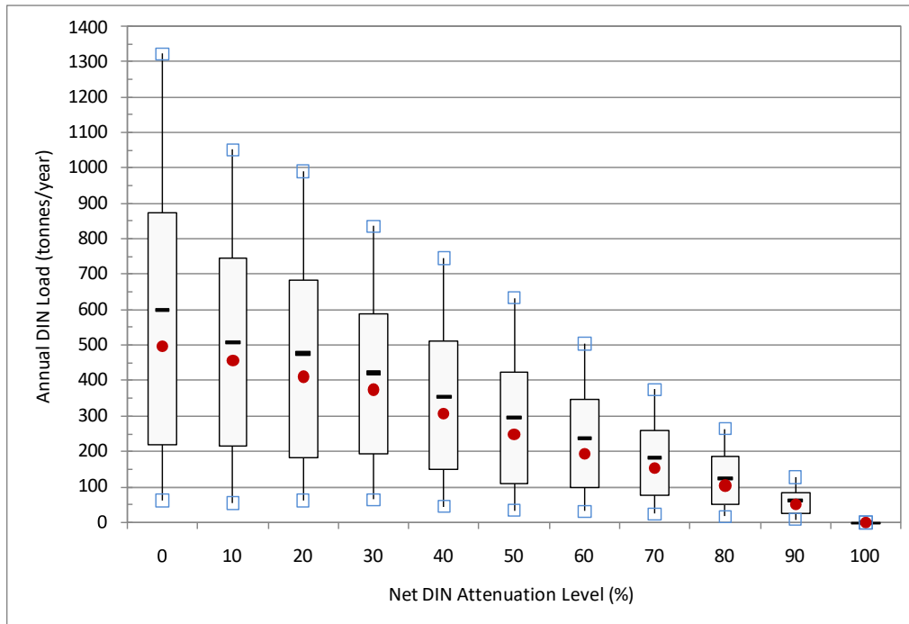
Figure 1. Box plots of predicted DIN loading for entire exclusive area provided varying attenuation levels.
