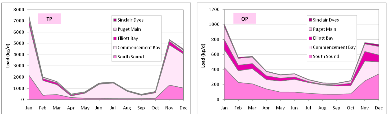
Figure F-16. Mean 2006-07 monthly phosphorus loads from watersheds totaled according to the regions in South and Central Puget Sound into which they drain.
