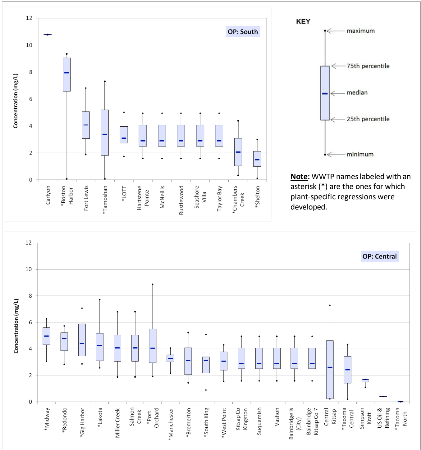
Figure G-5. Box plots of ortho-phosphate concentrations for 2006-07 for WWTPs in South (top) and Central (bottom) Puget Sound.
