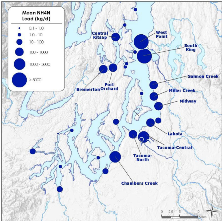
Figure G-11. Mean ammonium loads from WWTPs during 2006-07.
