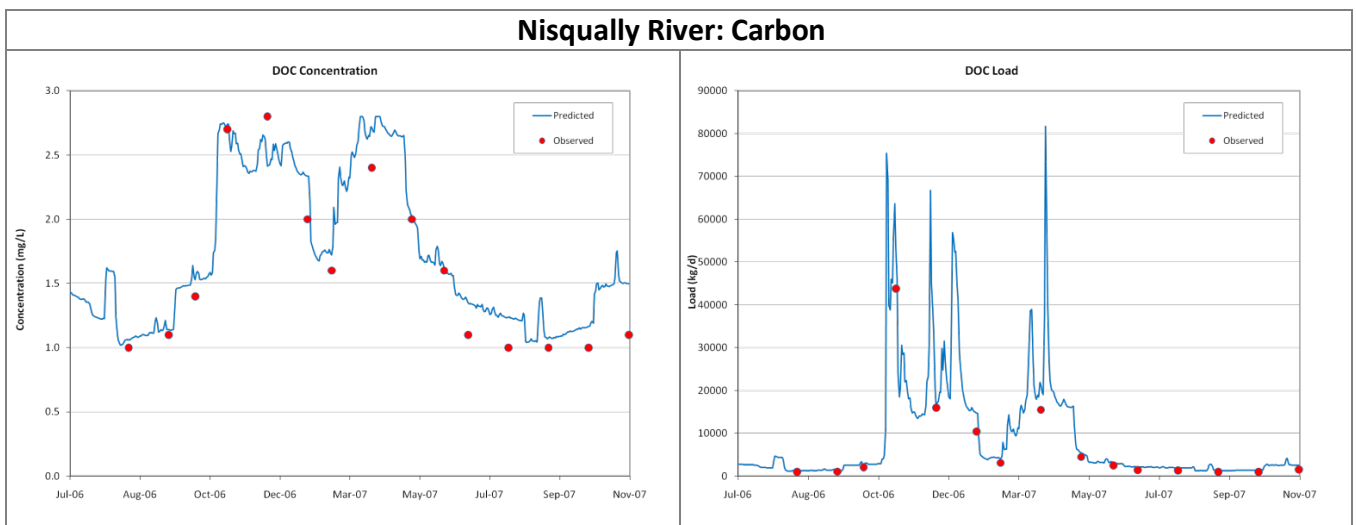
Figure D-9. Predicted and observed concentrations (left column) and loads (right column) of dissolved organic carbon (DOC) for the Nisqually River.
