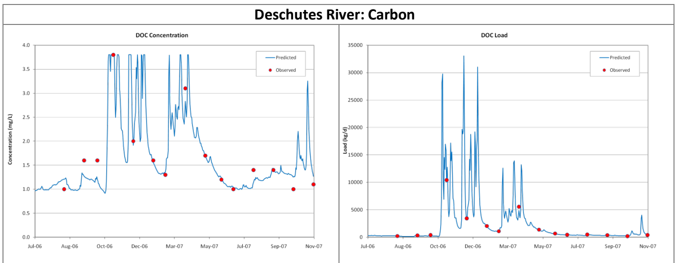
Figure D-3. Predicted and observed concentrations (left column) and loads (right column) of dissolved organic carbon (DOC) for the Deschutes River.
