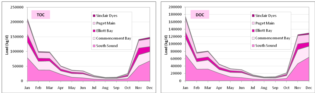
Figure F-17. Mean 2006-07 monthly organic carbon loads from watersheds totaled according to the regions in South and Central Puget Sound into which they drain.
