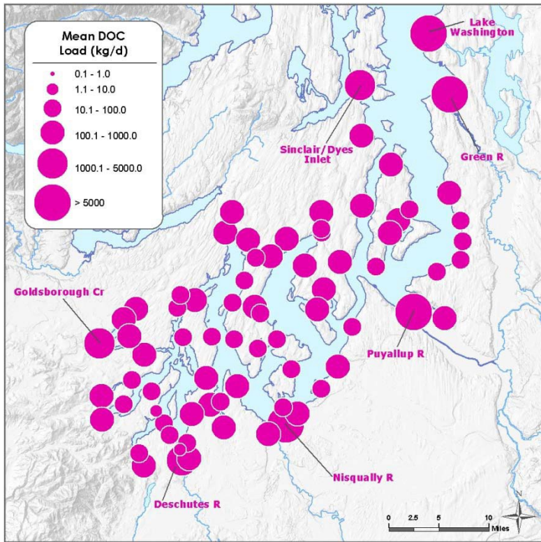
Figure F-14. Mean dissolved organic carbon loads from watersheds during 2006-07.
