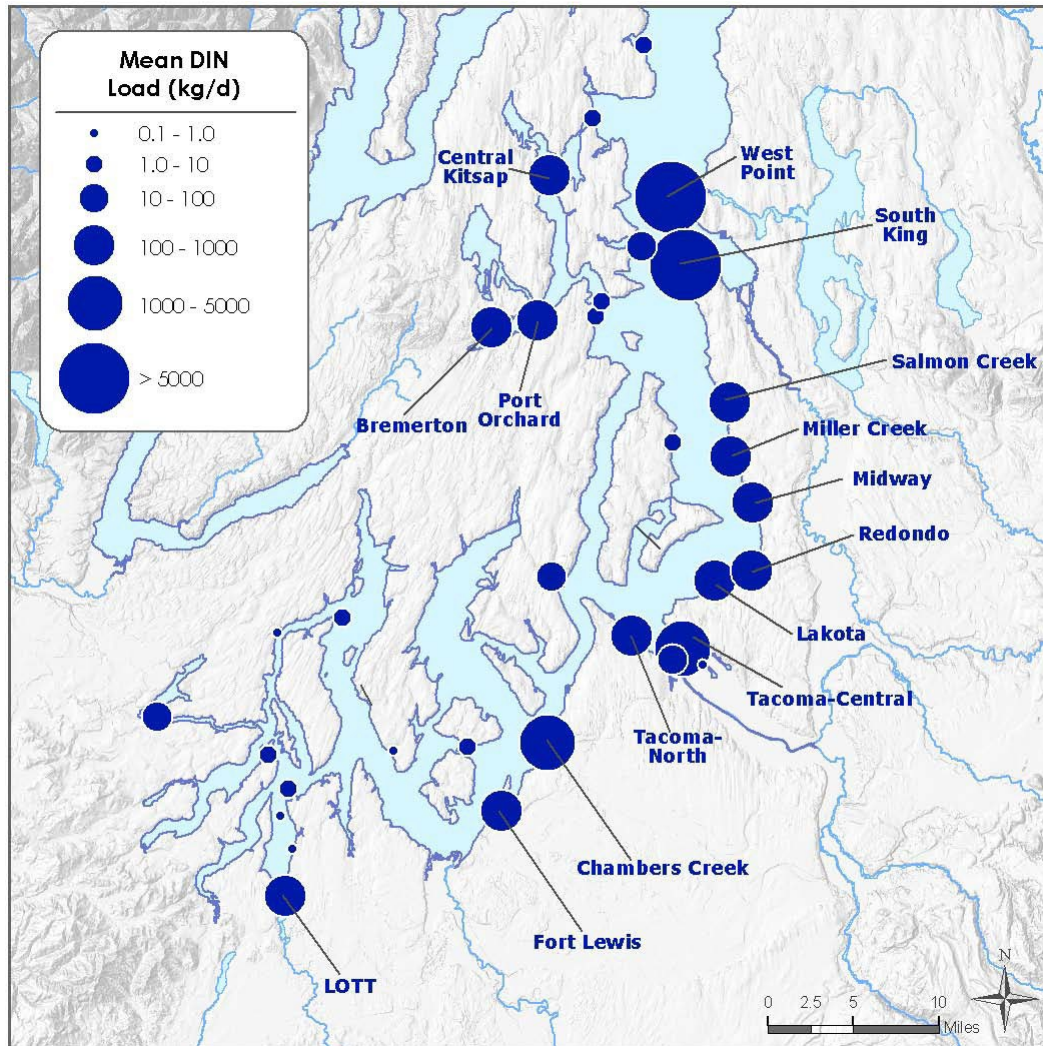
Figure 17. Mean dissolved inorganic nitrogen (DIN) loads from WWTPs from watersheds into South and Central Puget Sound during 2006-07.
