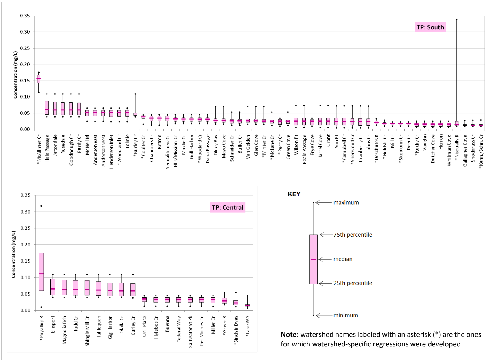
Figure F-4. Box plots of total phosphorus concentrations for 2006-07 for watersheds in South (top) and Central (bottom) Puget Sound.
