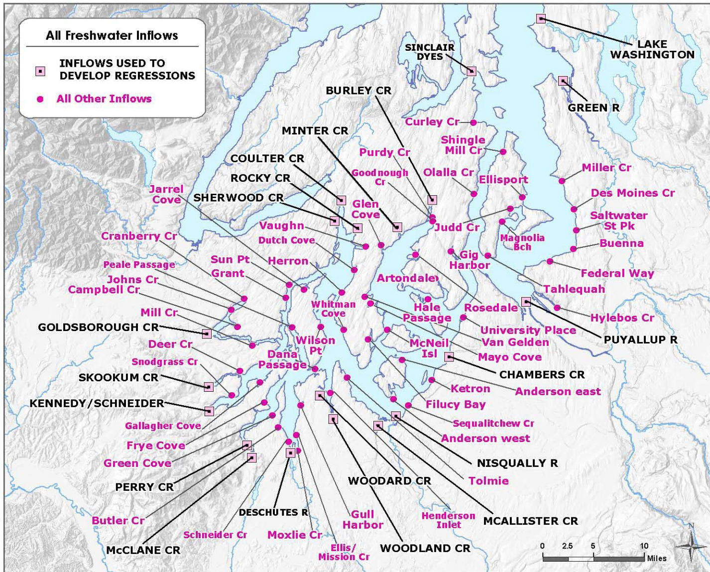
Figure 5. All 75 freshwater inflows included in the GEMSS water quality and hydrodynamics model of South and Central Puget Sound for which daily nutrient concentrations were developed for the 2006-07 calendar years.
