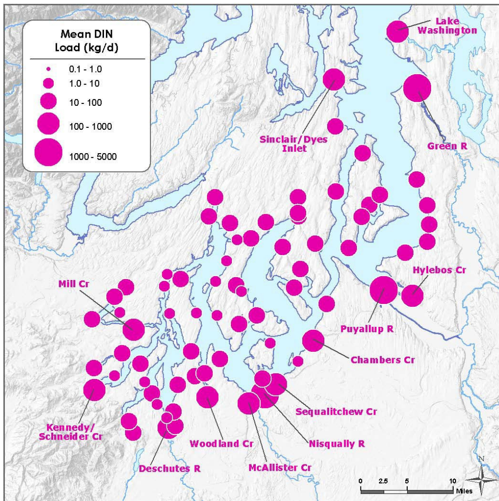
Figure 10. Mean dissolved inorganic nitrogen (DIN) loads from watersheds into South and Central Puget Sound during 2006-07.
