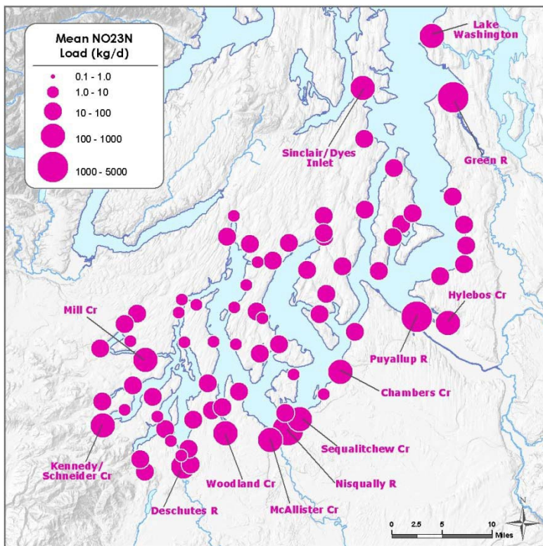
Figure F-9. Mean nitrate + nitrite loads from watersheds during 2006-07.
