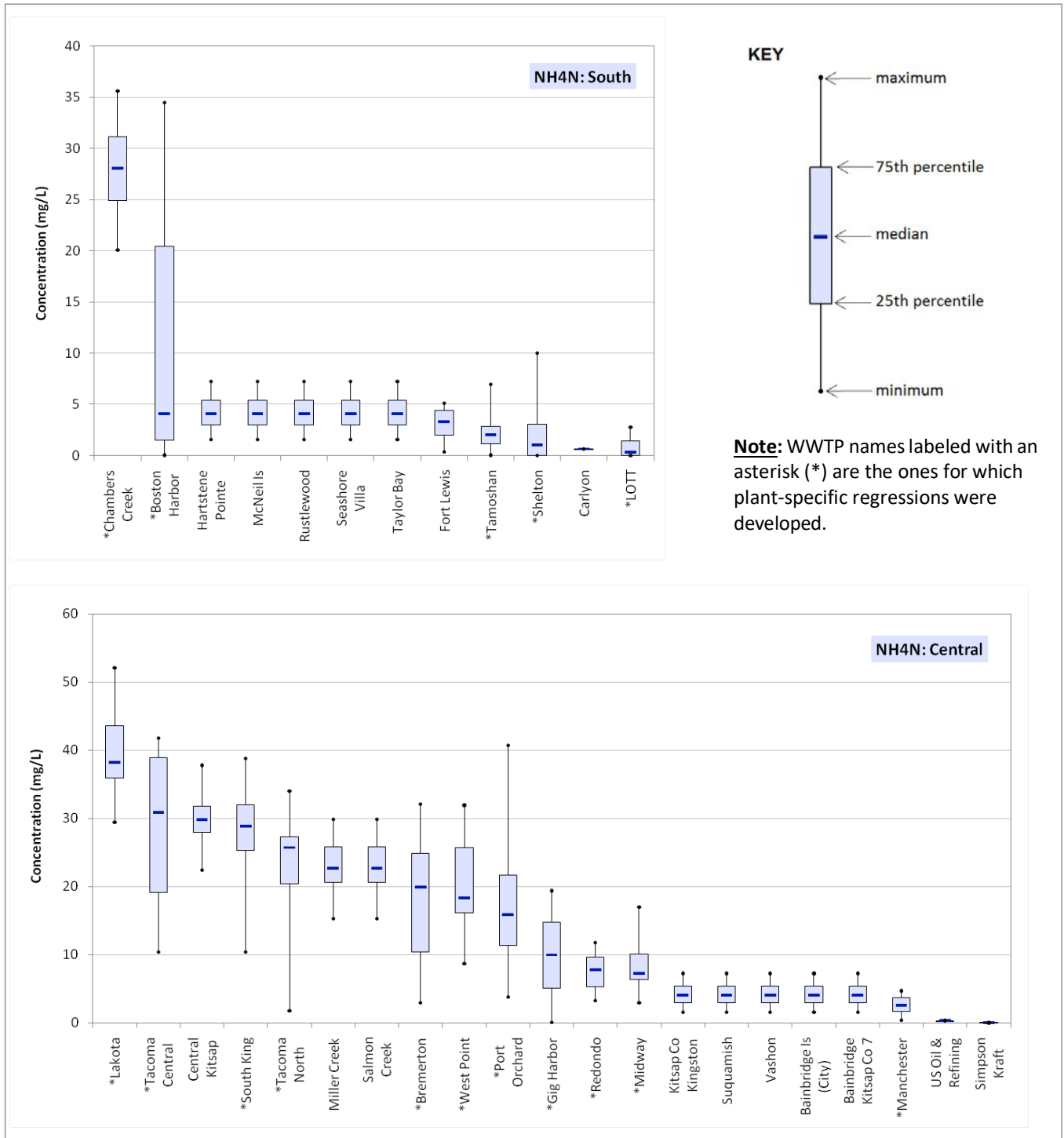
Figure G-3. Box plots of ammonium concentrations for 2006-07 for WWTPs in South (top) and Central (bottom) Puget Sound.
