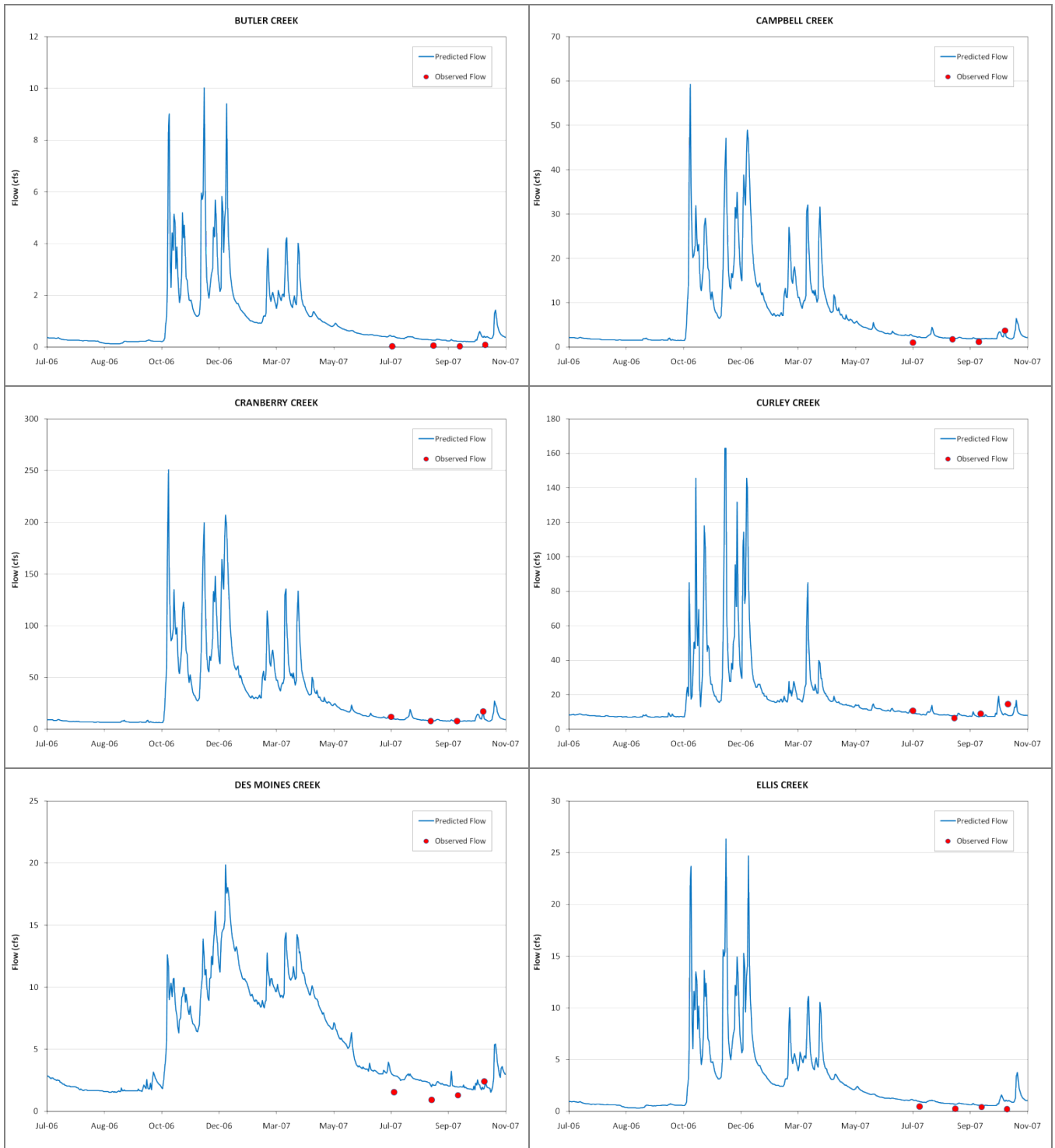
Figure B-3. Predicted and observed flows on creeks where four months of data were collected between July 2006 and October 2007.
