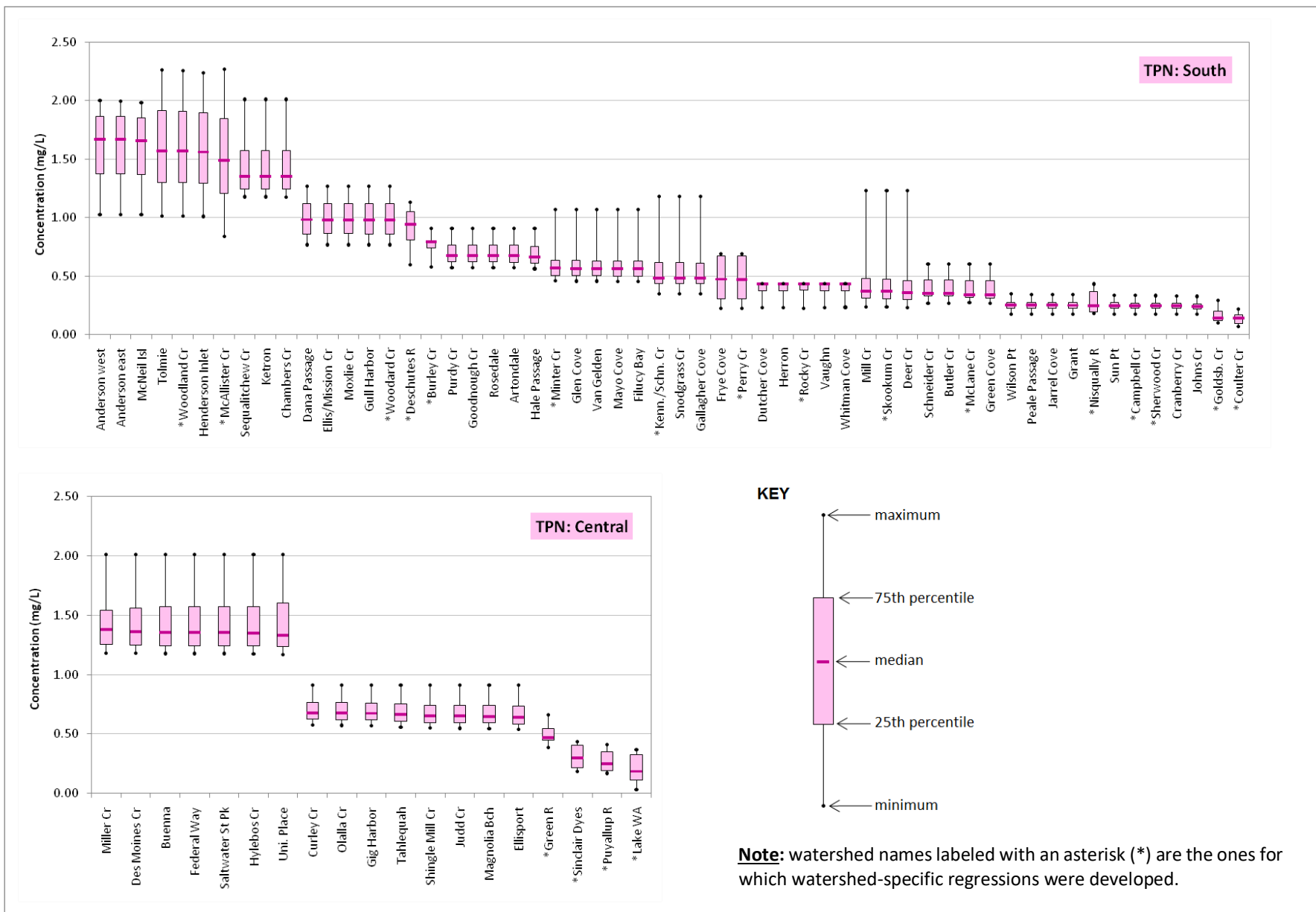
Figure F-1. Box plots of total persulfate nitrogen concentrations for 2006-07 for watersheds in South (top) and Central (bottom) Puget Sound.
