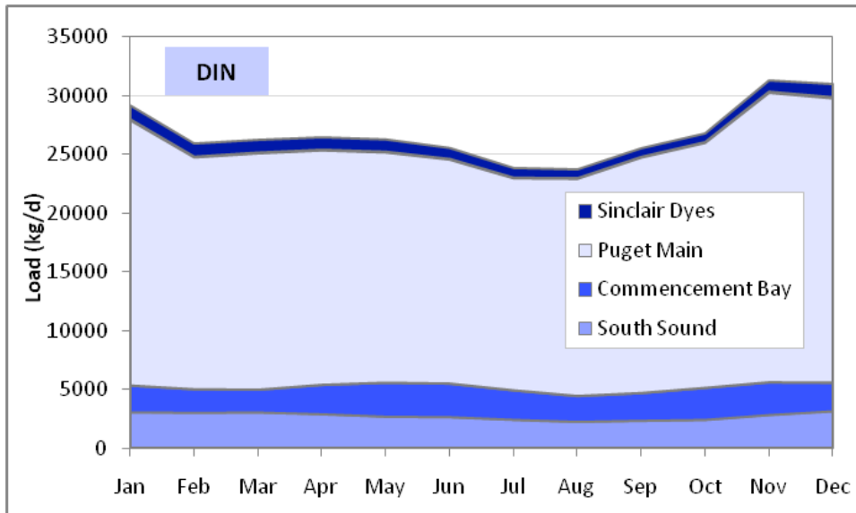
Figure 18. Mean 2006-07 monthly dissolved inorganic nitrogen (DIN) loads from WWTPs totaled according to the regions in South and Central Puget Sound into which they discharge effluent.
