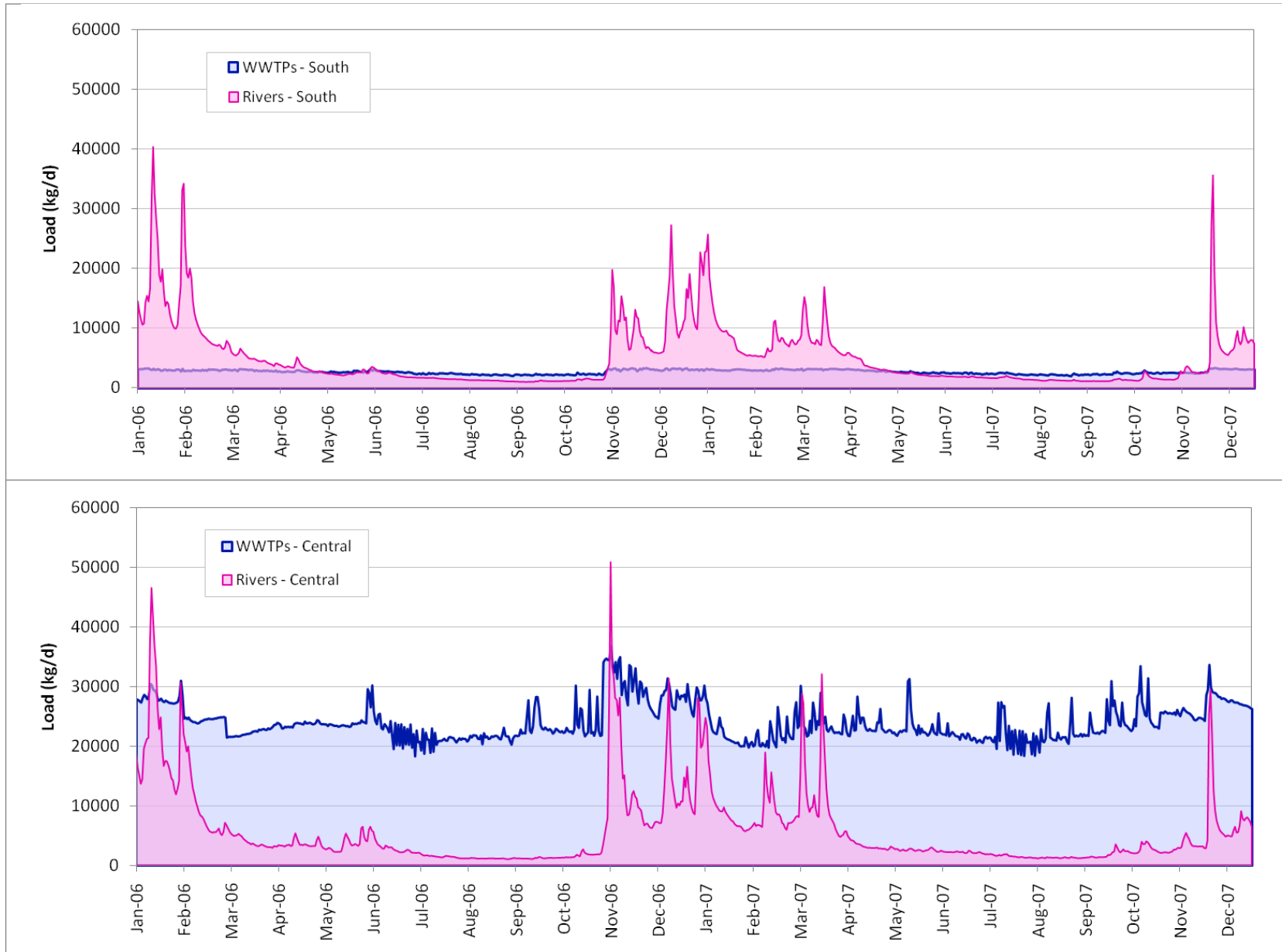
Figure 22. Daily dissolved inorganic nitrogen (DIN) loads from rivers and WWTPs into South (top) and Central (bottom) Puget Sound, 2006-07.
