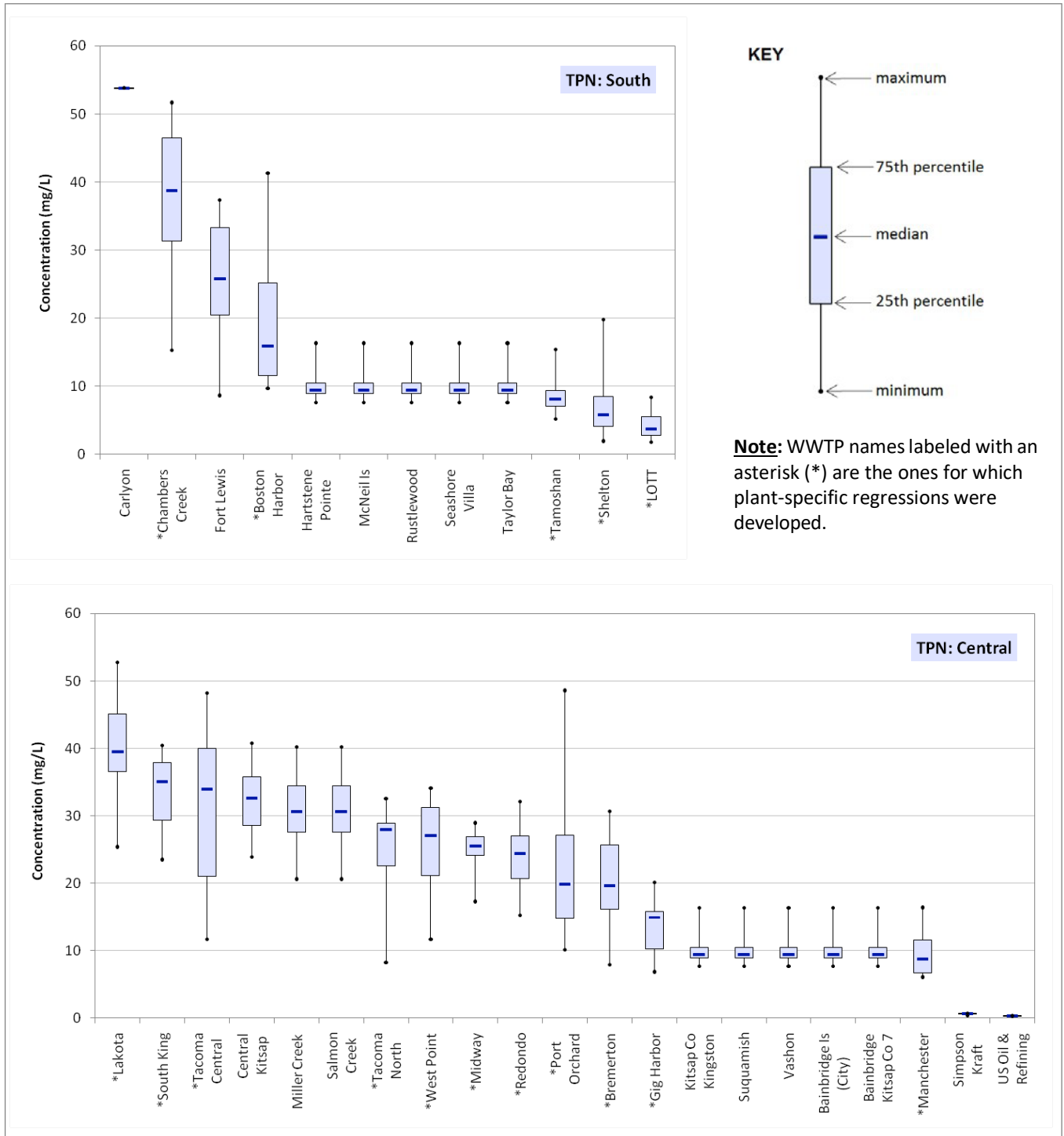
Figure G-1. Box plots of total persulfate nitrogen concentrations for 2006-07 for WWTPs in South (top) and Central (bottom) Puget Sound.
