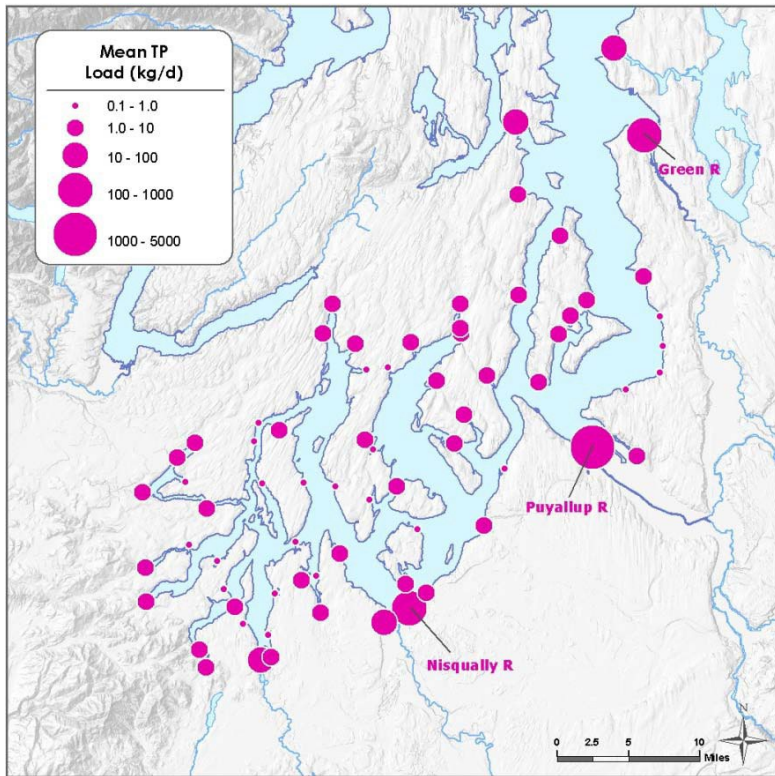
Figure F-11. Mean total phosphorus loads from watersheds during 2006-07.
