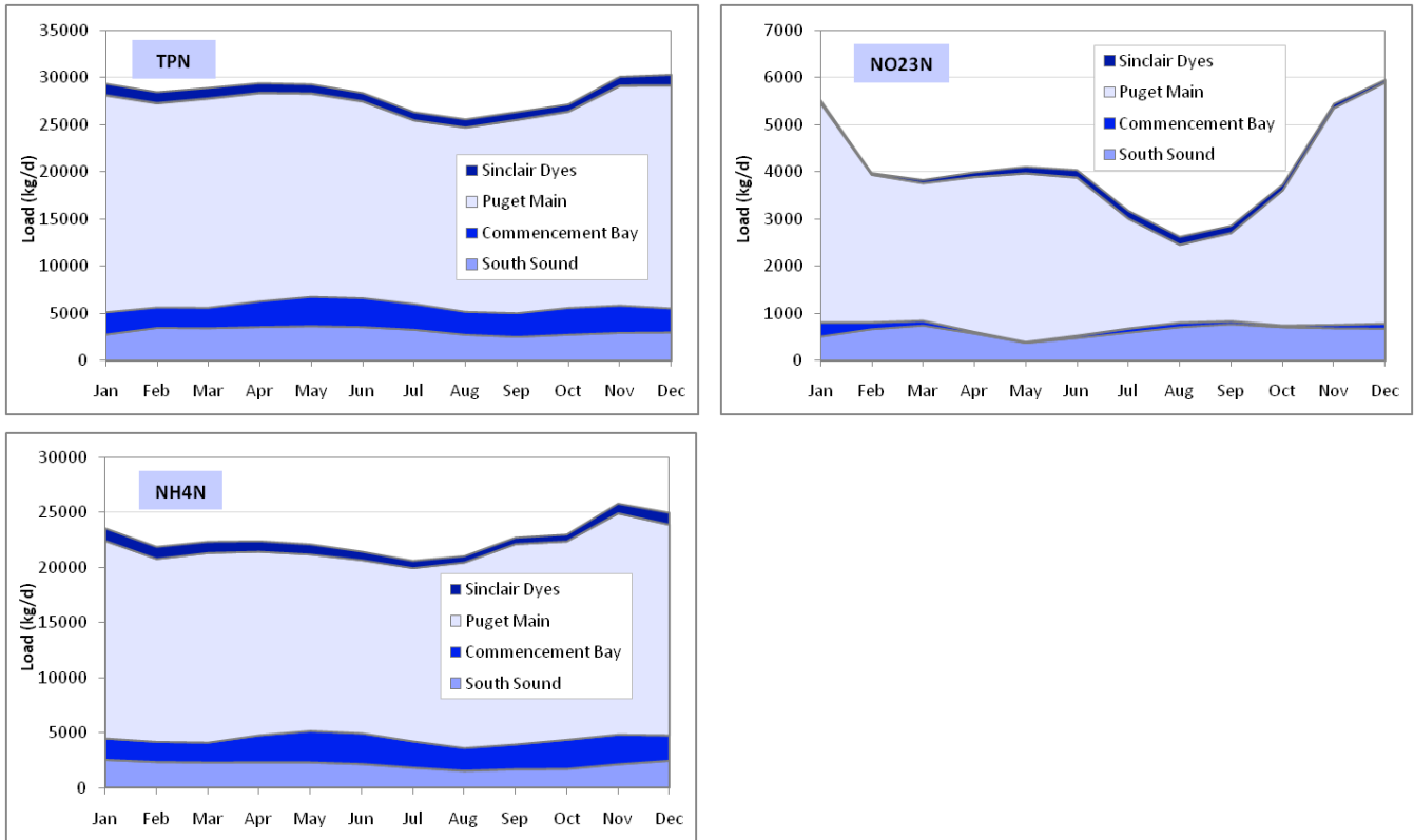
Figure G-16. Mean 2006-07 monthly nitrogen loads from WWTPs totaled according to the regions in South and Central Puget Sound into which they drain.
