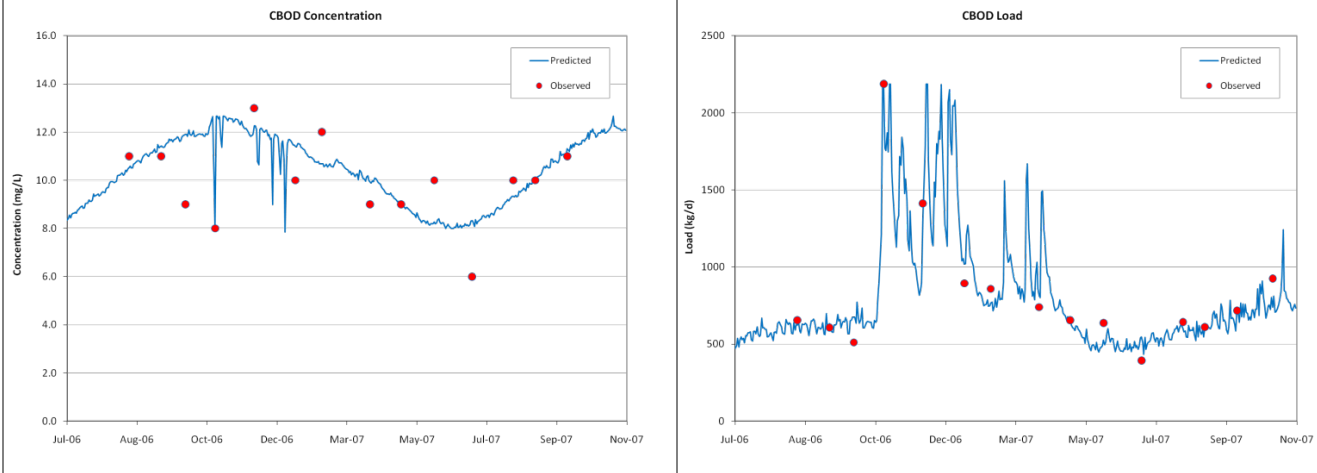
Figure E-12. Predicted and observed concentrations (left column) and loads (right column) of CBOD for the Tacoma-Central WWTP.
