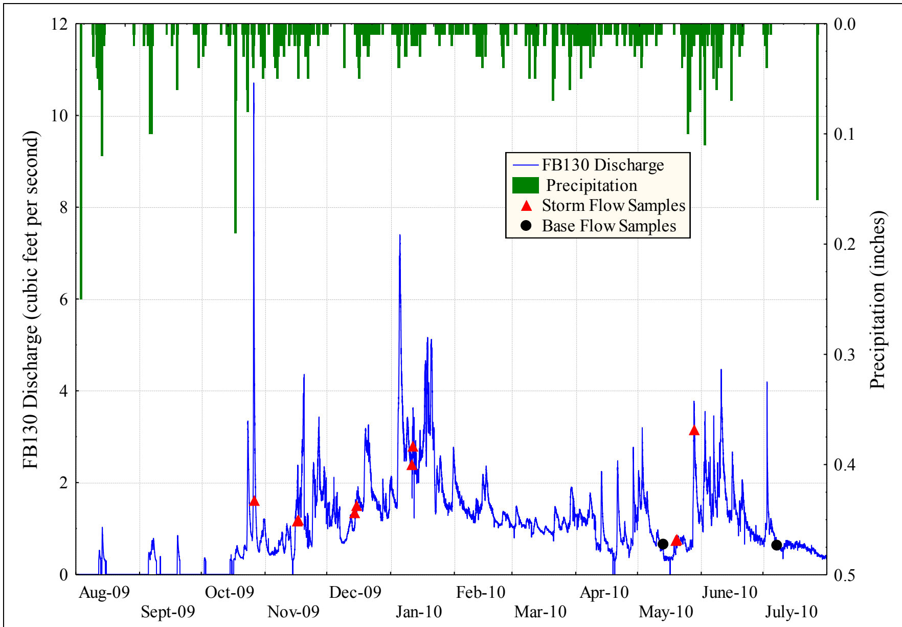
Figure D-15. FB130 hydrograph, hyetograph, and sample collection times.
