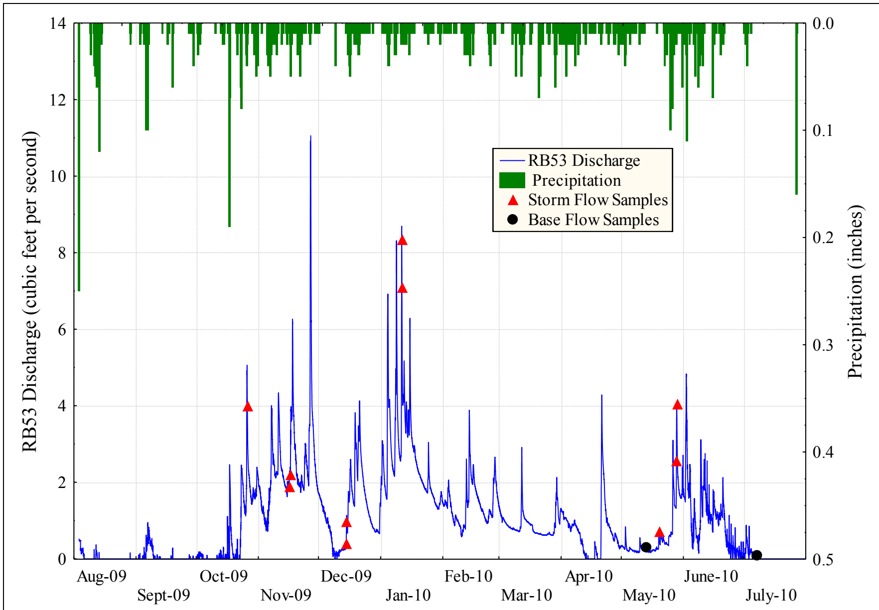
Figure D-11. RB53 hydrograph, hyetograph, and sample collection times.
