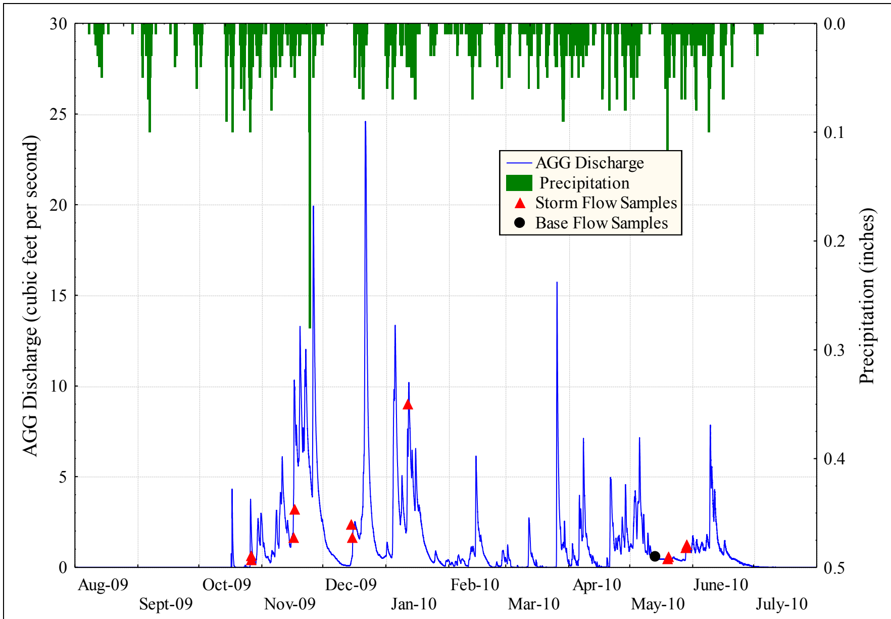
Figure D-6. AGG hydrograph, hietograph, and sample collection times.
