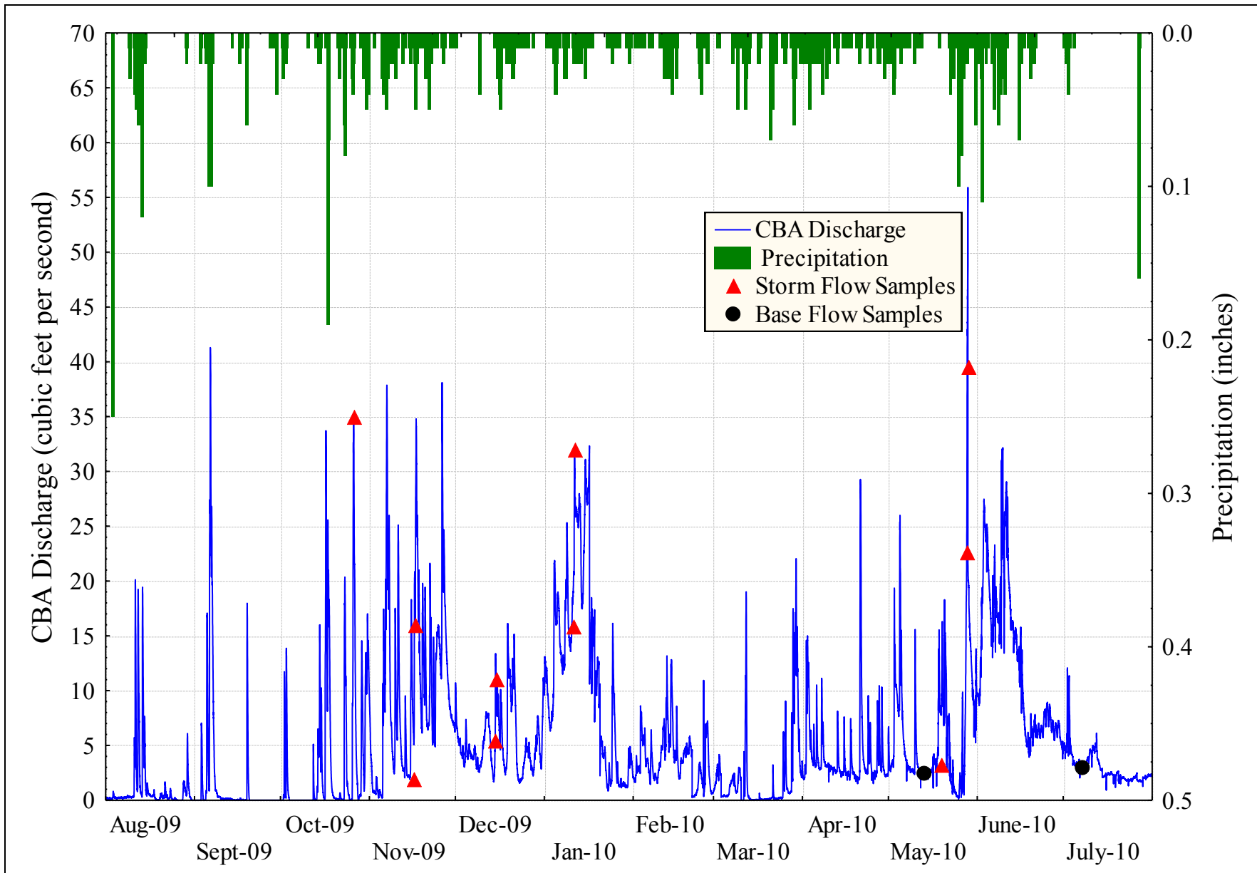
Figure D-9. CBA hydrograph, hyetograph, and sample collection times.
