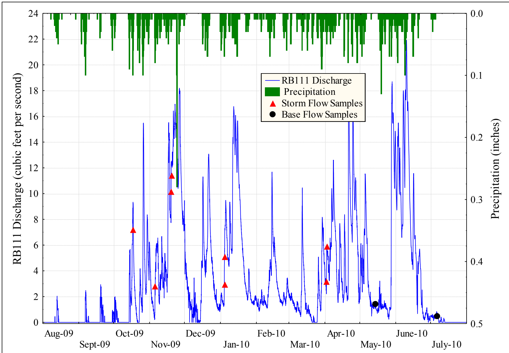
Figure D-3. RB111 hydrograph, hyetograph, and sample collection times.
