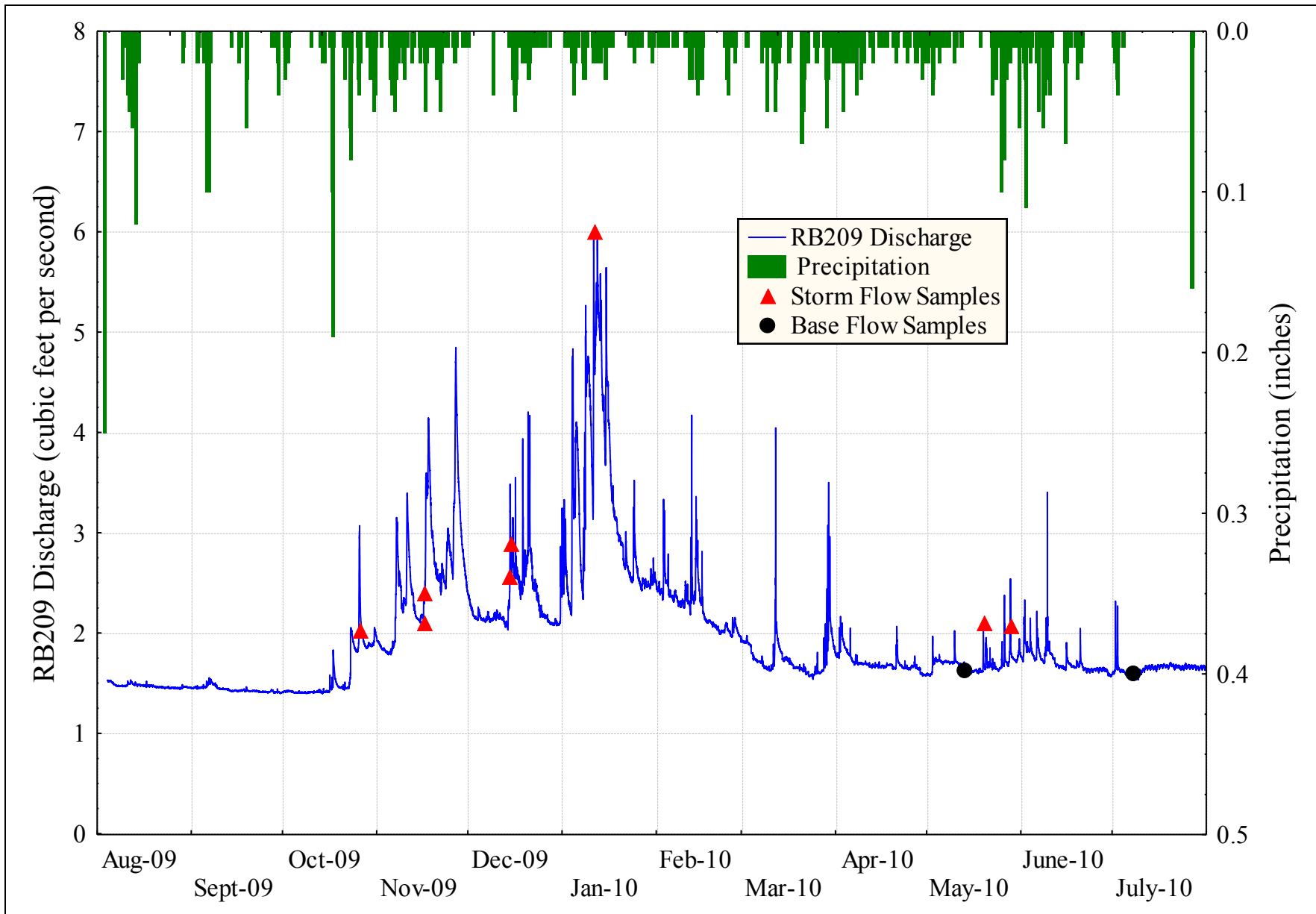
Figure D-12. RB209 hydrograph, hyetograph, and sample collection times.
