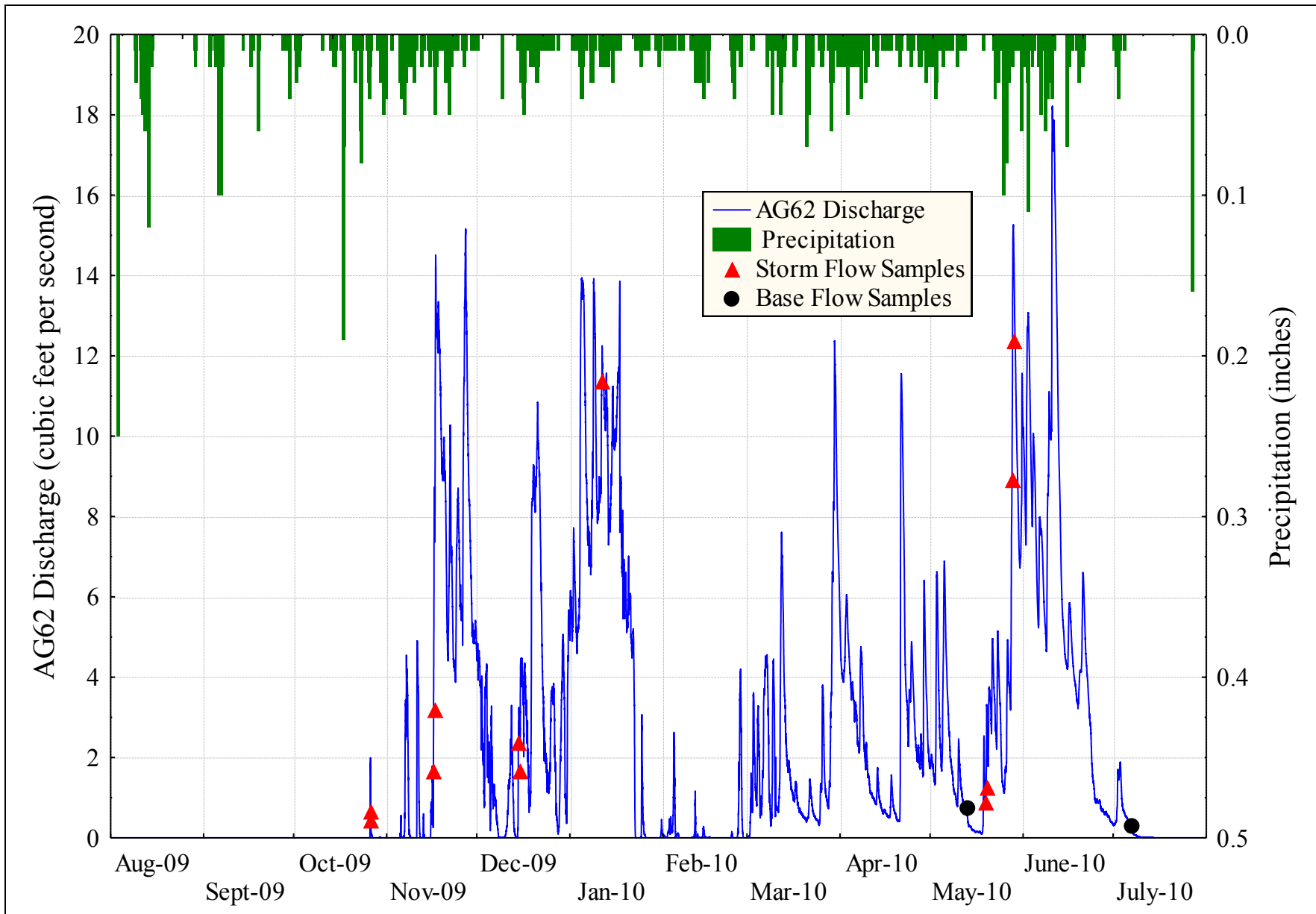
Figure D-14. AG62 hydrograph, hyetograph, and sample collection times.
