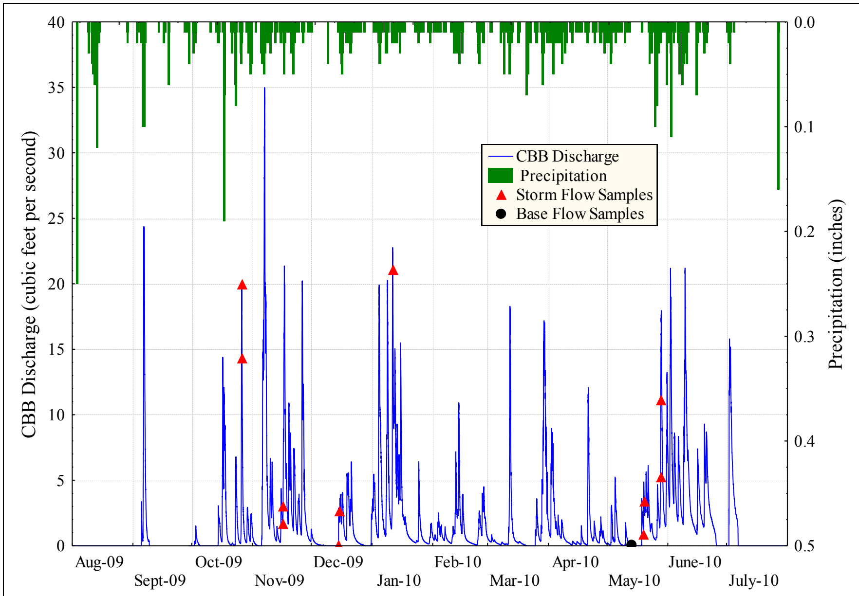
Figure D-10. CBB hydrograph, hyetograph, and sample collection times.
