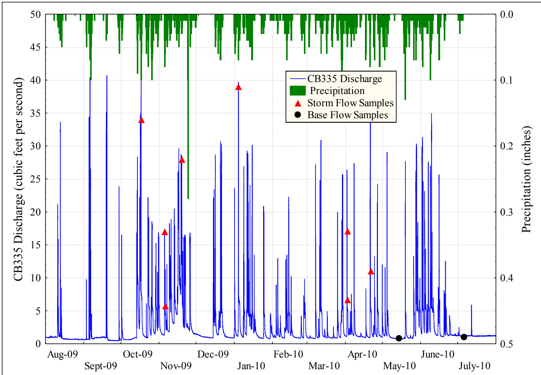
Figure D-1. CB335 hydrograph, hyetograph, and sample collection times.
