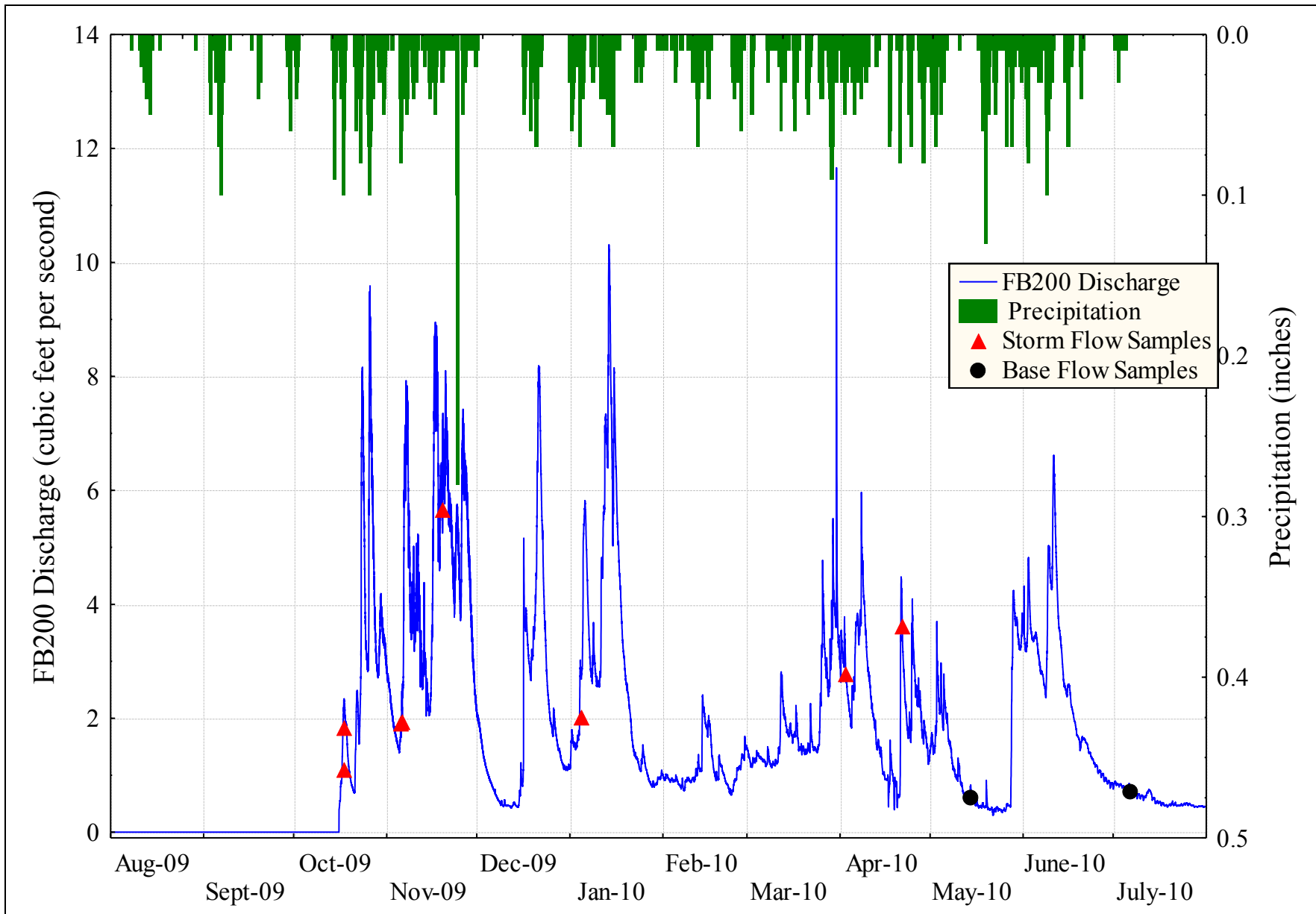
Figure D-7. FB200 hydrograph, hyetograph, and sample collection times.
