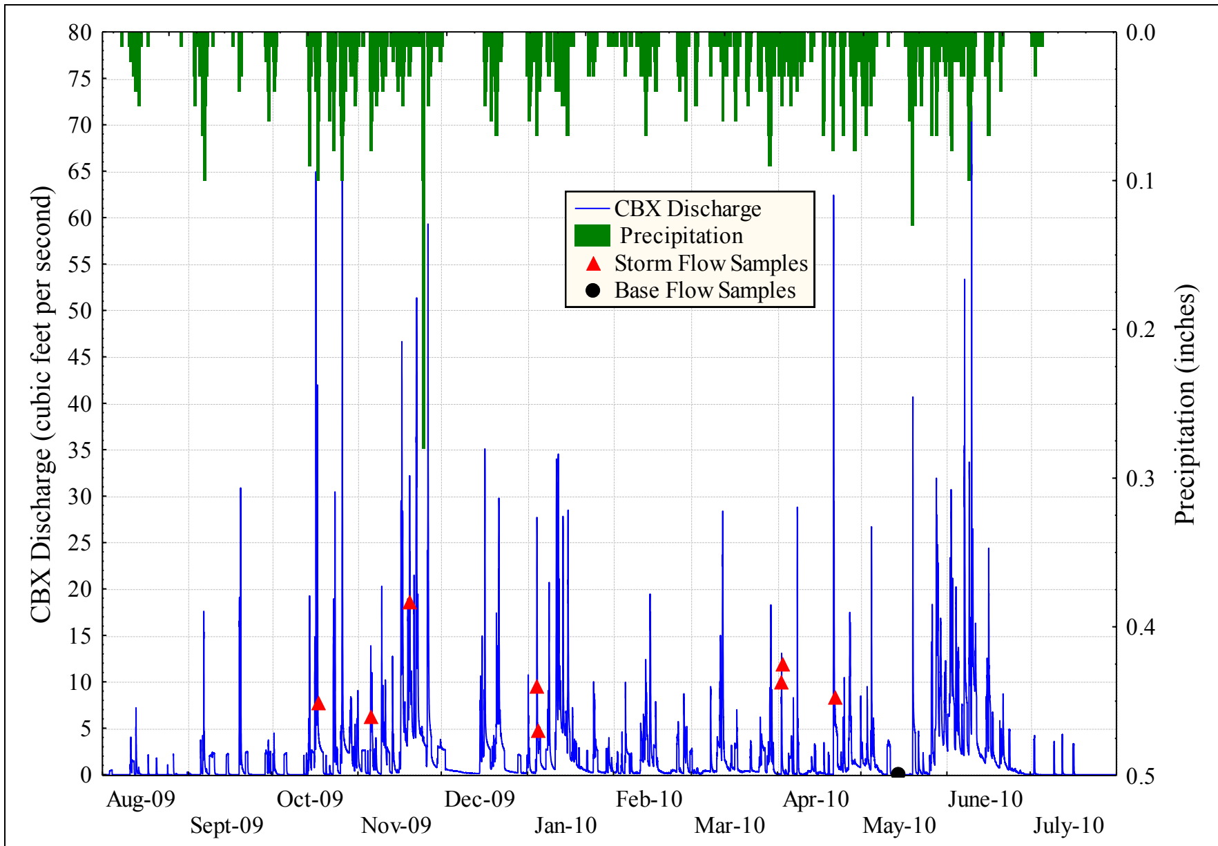
Figure D-2. CBX hydrograph, hyetograph, and sample collection times.
