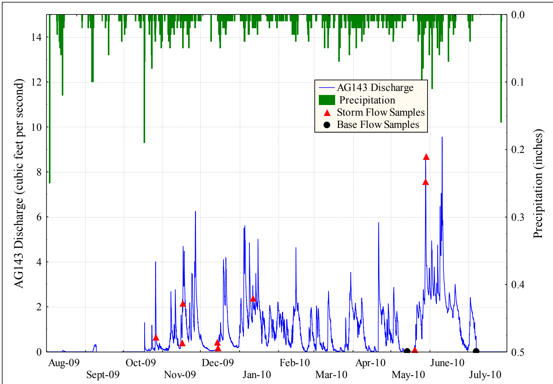
Figure D-13. AG143 hydrograph, hyetograph, and sample collection times.
