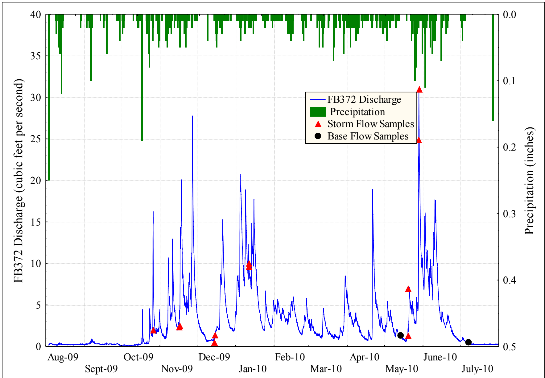
Figure D-16. FB372 hydrograph, hyetograph, and sample collection times.
