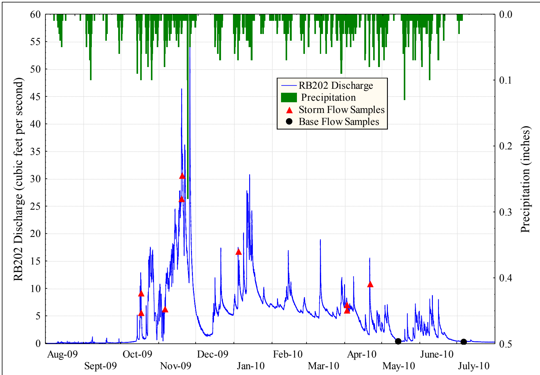
Figure D-4. RB202 hydrograph, hyetograph, and sample collection times.
