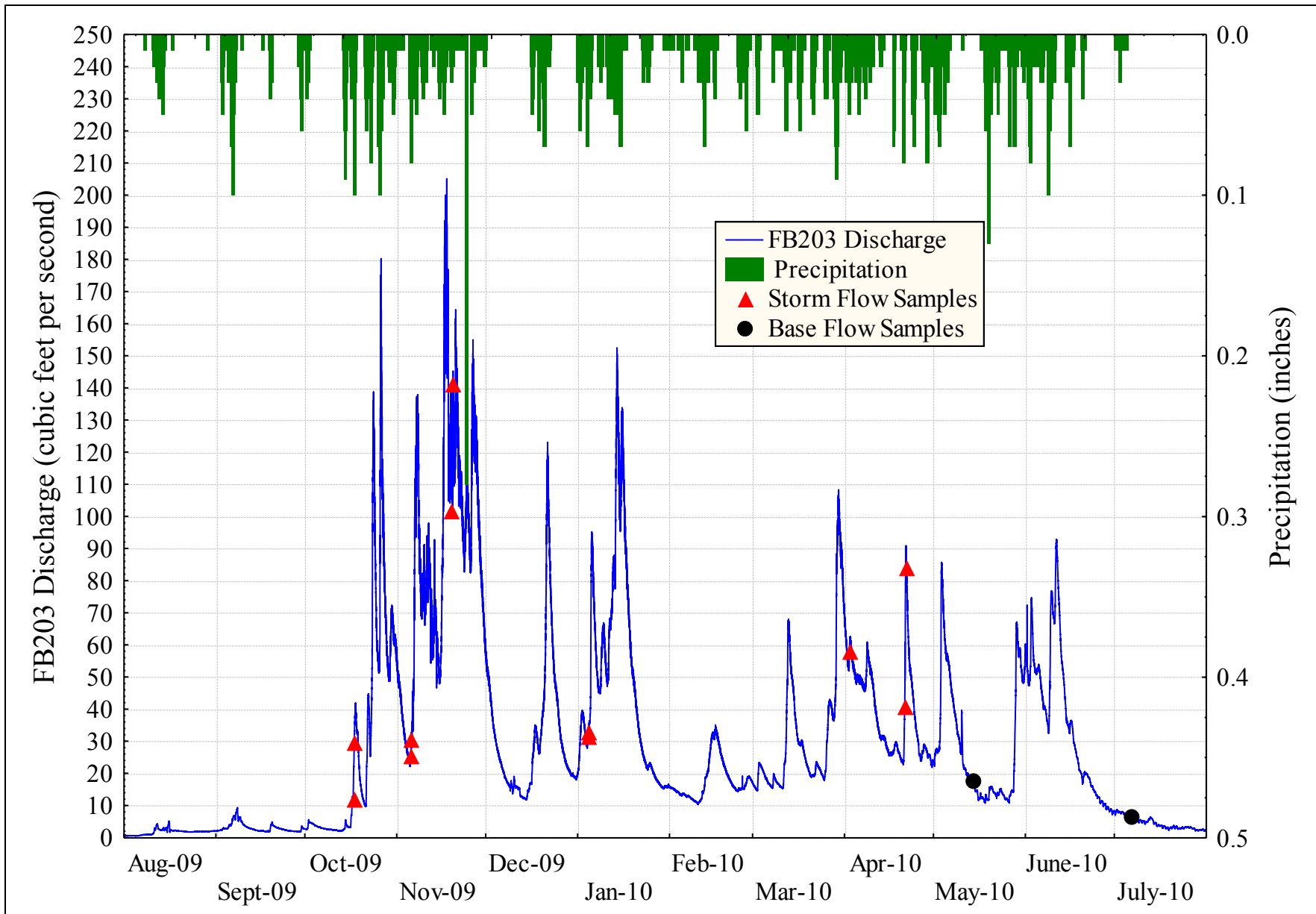
Figure D-8. FB203 hydrograph, hyetograph, and sample collection times.
