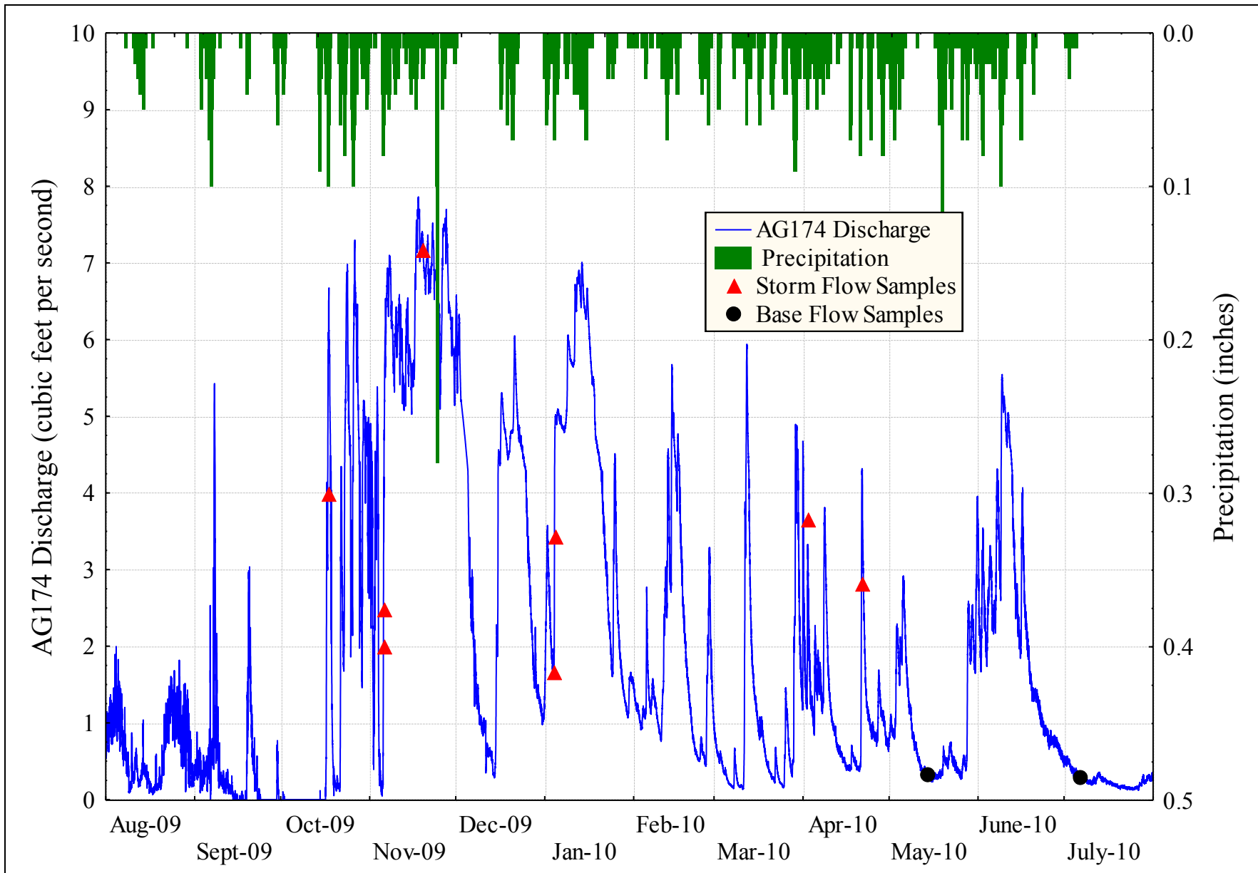
Figure D-5. AG174 hydrograph, hyetograph, and sample collection times.
