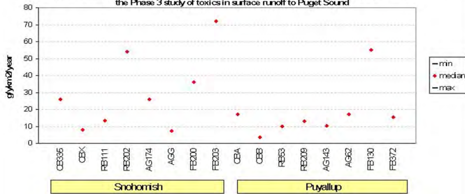
Figure O-117. Base flow unit area toxic chemical loading estimates for 1,2-dichlorobenzene for the Phase 3 study of toxics in surface runoff to Puget Sound
