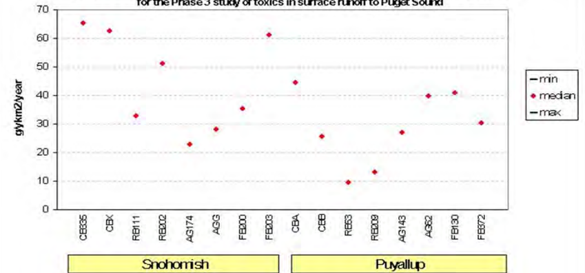
Figure O-118. Storm event unit area toxic chemical loading estimates for 1,2-dichlorobenzene for the Phase 3 study of toxics in surface runoff to Puget Sound
