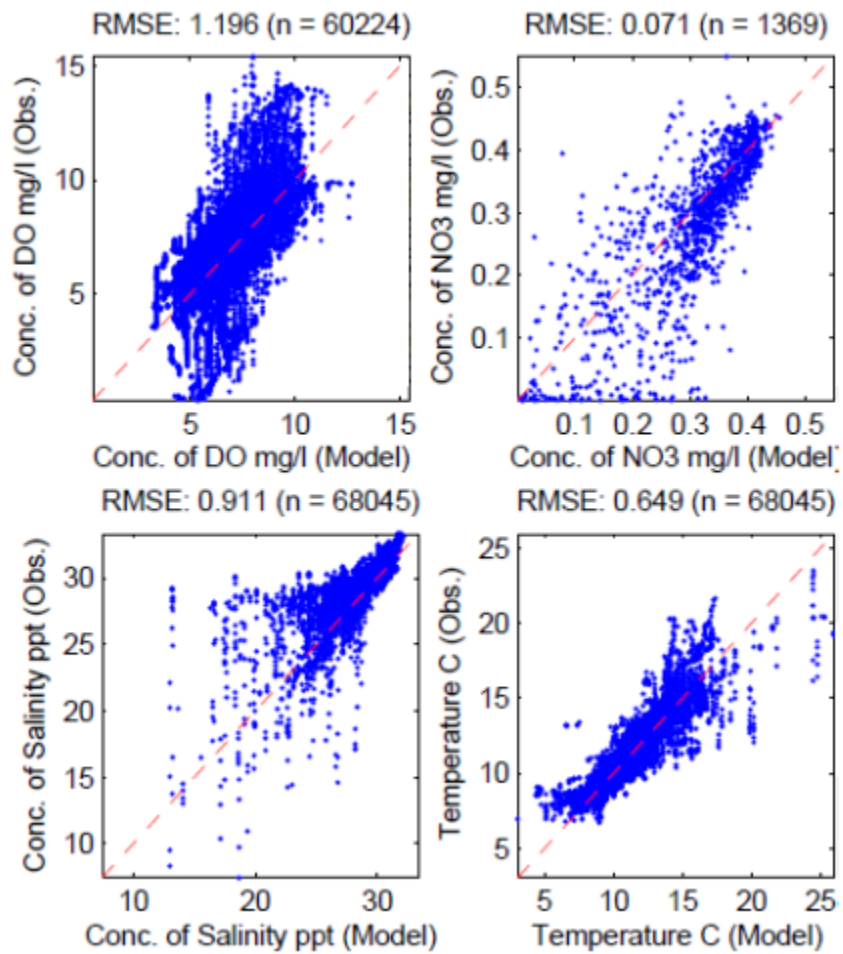
Figure 3.13. Aggregated goodness-of-fit statistics for Dissolved Oxygen (DO, mg/L), Nitrate+Nitrite (NO 3 , mg/L), Salinity (PPT), and Temperature (deg C) for 36 stations distributed throughout model domain.
