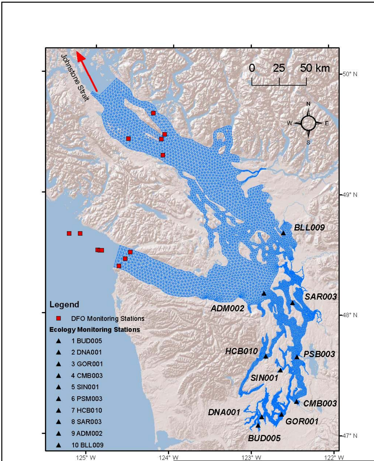
Figure 2.3. Computational Grid – Puget Sound Water Quality Model
