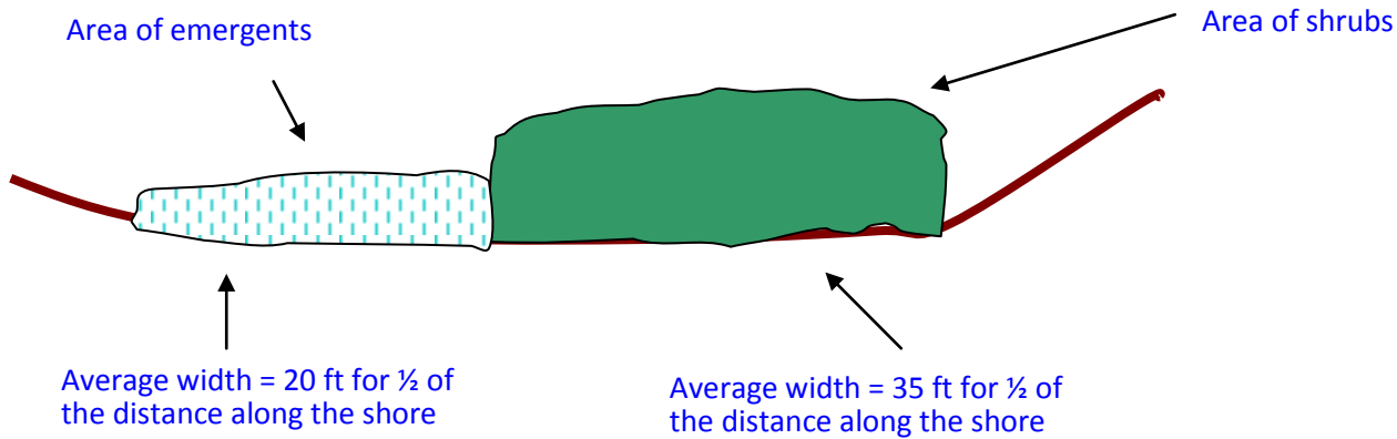
Figure 39. Estimating width of plant types along the shores of a lake. The average width of shrubs is 35 ft for \frac{1}{2} the length along the shore and the width of emergents is 20 ft for \frac{1}{2} of the length. This wetland would score 4 points because more than \frac{1}{4} of the length consists of a zone of shrubs wider than 33 ft.
