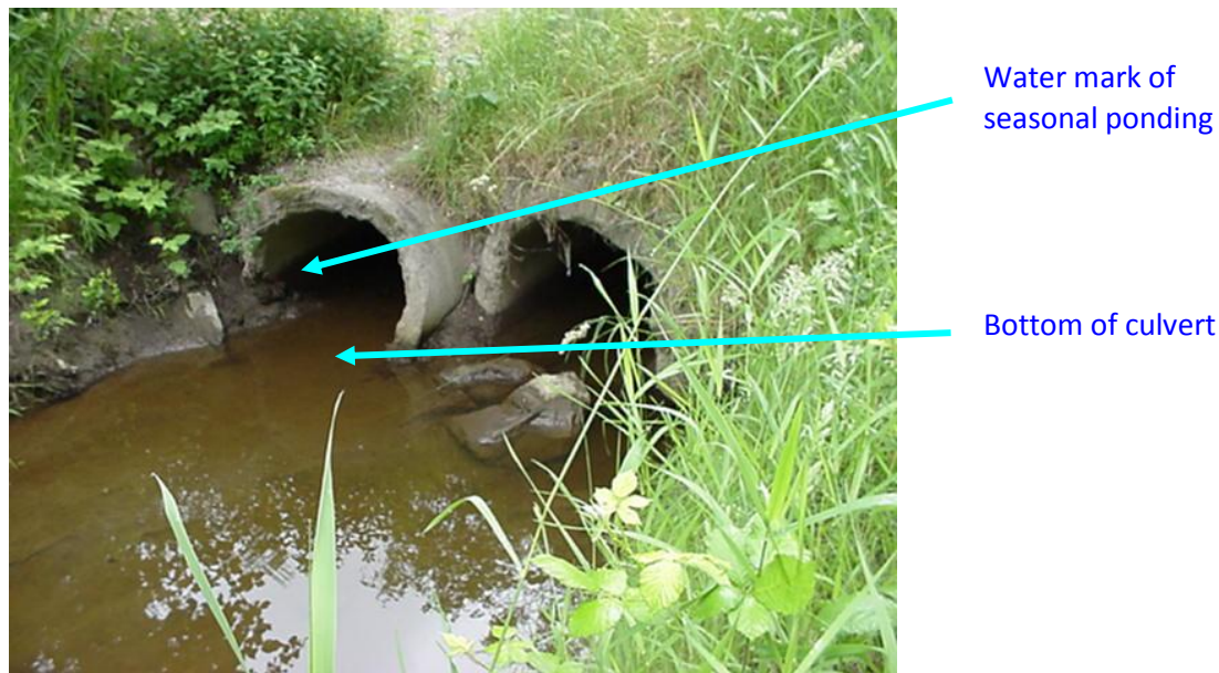
Figure 25. A round culvert with water still present. Live storage is measured from the bottom of the culvert, not the present water level. The depth of storage is approximately 7 in.
