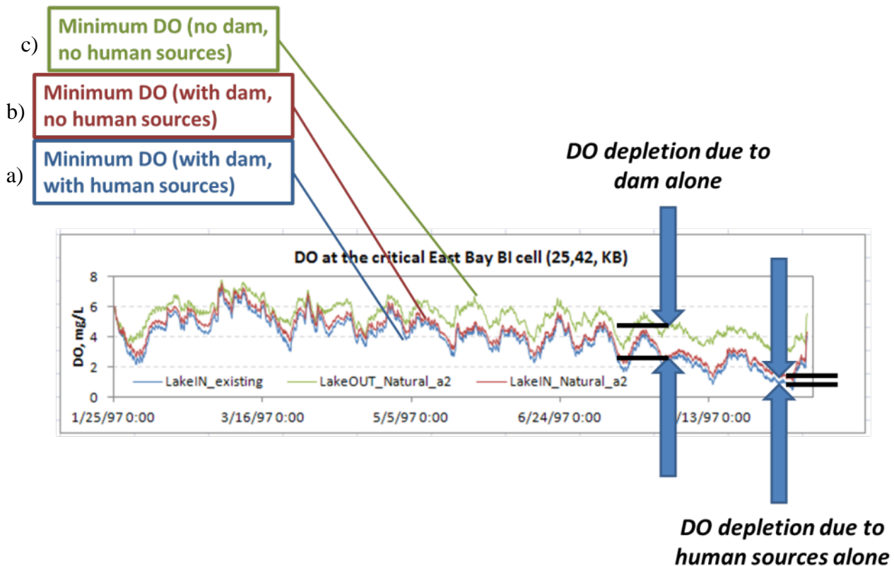
Figure 33. DO in the bottom layer at the critical cell in East Bay (a) at the existing condition with the Capitol Lake dam and current anthropogenic sources, (b) with the Capitol Lake dam and no anthropogenic sources, and (c) without the Capitol Lake dam and without anthropogenic sources.
