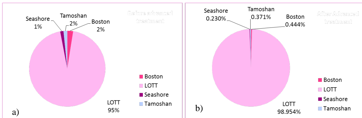
Figure 21. The proportion of point source loading of nitrogen from the various local point sources (a) under the existing condition, and (b) with advanced treatment at the three small WWTPs (Seashore Villa, Tamoshan, and Boston Harbor).
