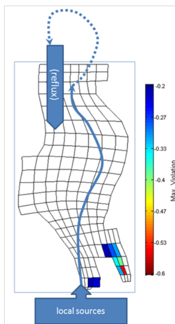
Figure 26. Conceptual diagram of reflux, which is the fraction of local anthropogenic loading that re-enters back across the open boundary of Budd Inlet after leaving.
