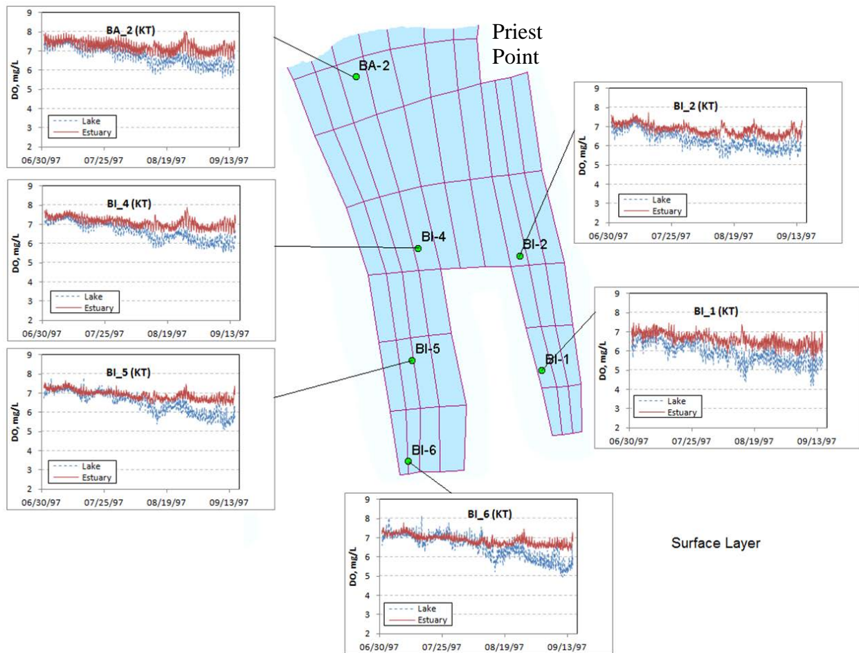
Figure 16. Predicted DO in the surface layer at selected locations in Budd Inlet with current anthropogenic loading with the Capitol Lake dam (blue-dashed lines labeled “Lake”) and without the Capitol Lake dam (red line labeled “Estuary”).
