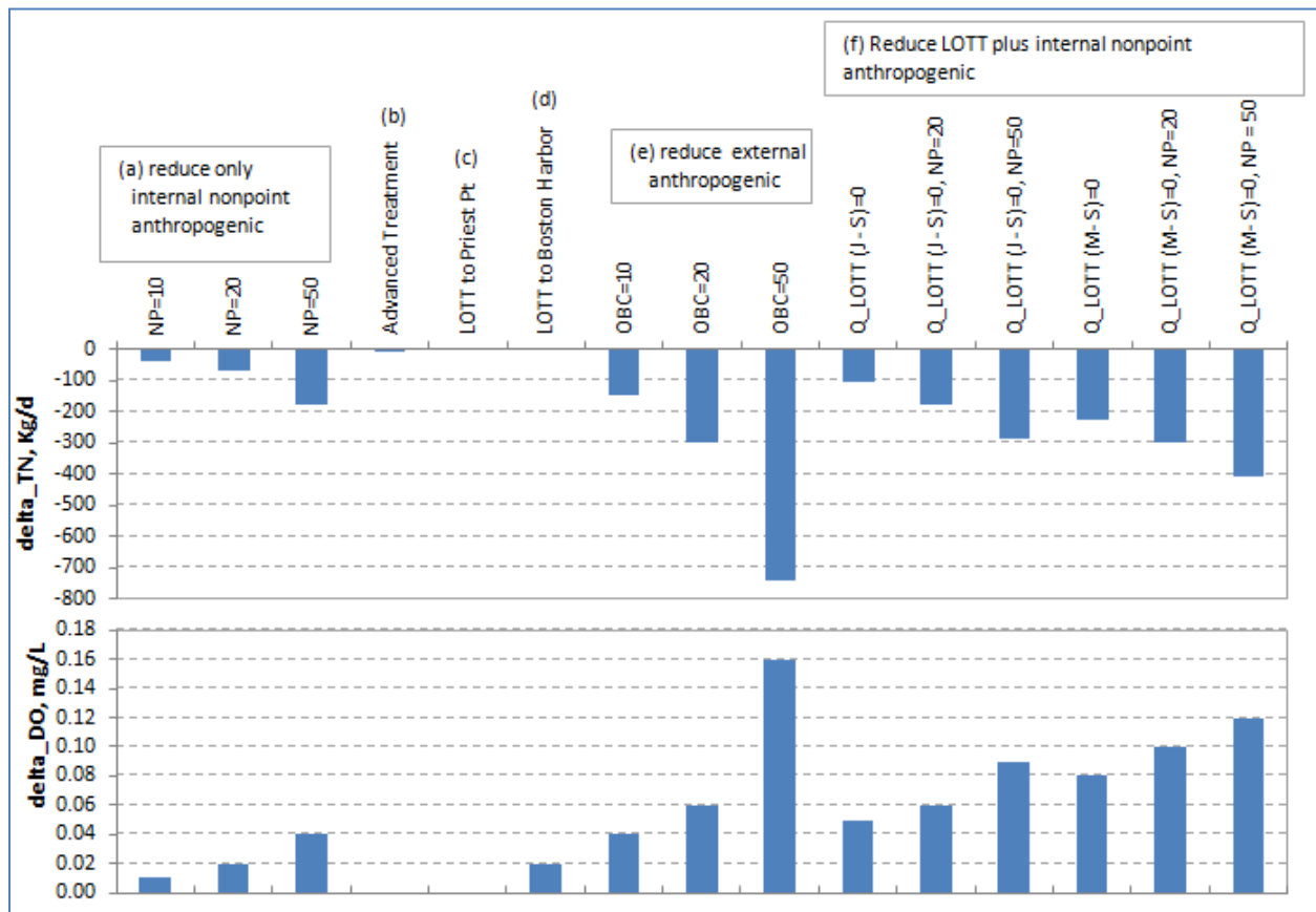
Figure 32. The estimated total nitrogen (TN) loading reduction and DO improvement at the critical East Bay cell for the various model scenarios including (a) reduction of local nonpoint anthropogenic load by 10%, 20%, or 50%, (b) advanced treatment by local small WWTPs, (c) moving the LOTT outfall to north of Priest Point, (d) moving the LOTT outfall to Boston Harbor, (e) reducing external anthropogenic loading by 10%, 20%, or 50%, and (f) reducing LOTT and local nonpoint anthropogenic loading.
