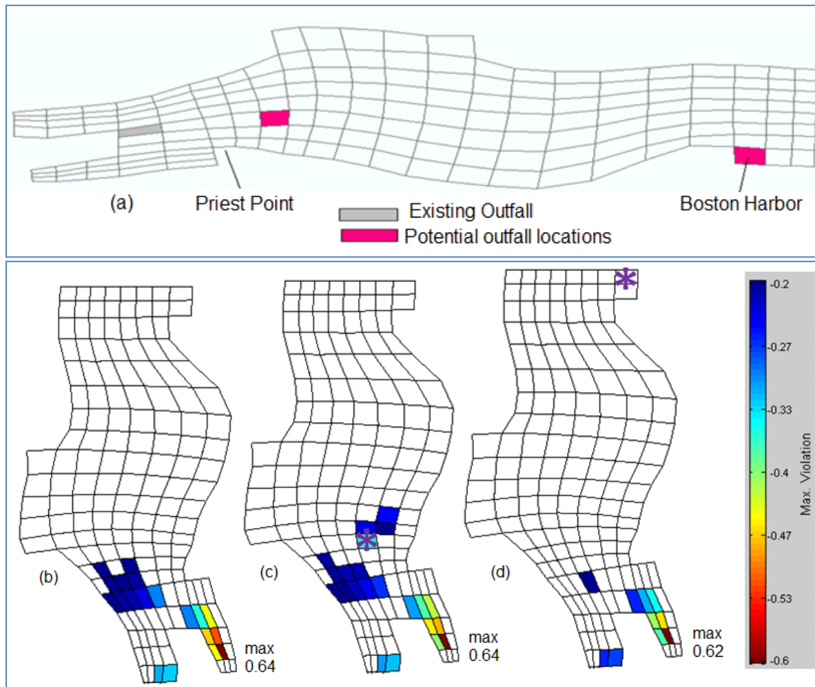
Figure 22. DO depletion (mg/L) for alternative potential outfall locations (a) without the Capitol Lake dam, (b) with existing anthropogenic nutrient sources (same as Figure 17), (c) with the LOTT outfall moved to north of Priest Point Park, and (d) with the LOTT outfall moved to Boston Harbor.
