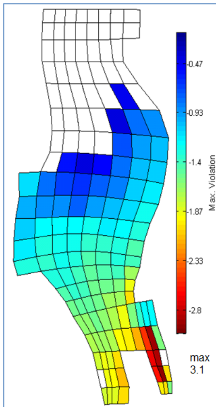
Figure 8. DO depletion (mg/L) caused by the cumulative effect of all anthropogenic influences including Capitol Lake dam and current anthropogenic loading sources.
