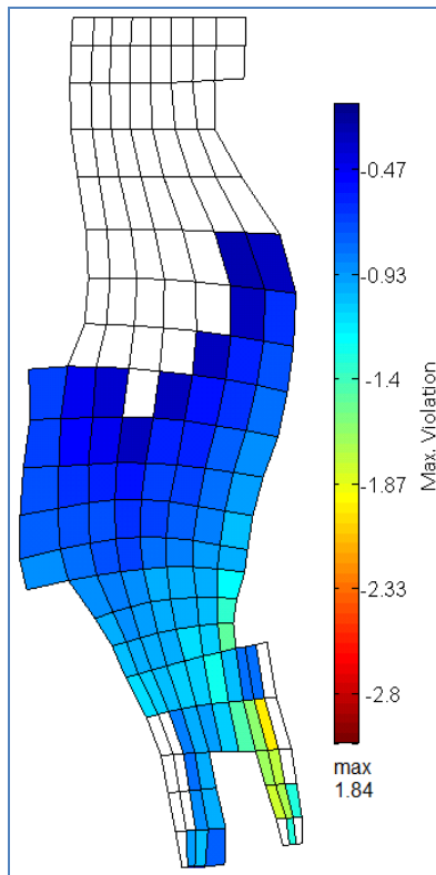
Figure 9. DO depletion (mg/L) caused solely by the Capitol Lake dam.
