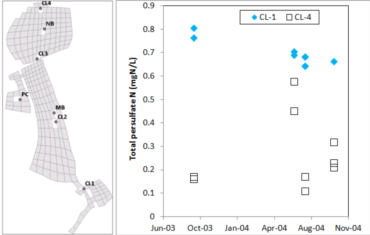
Figure 14. Total persulfate nitrogen (TPN) at two locations in Capitol Lake during 2003-2004.
