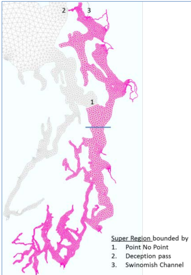
Figure A-1. Salish Sea model super-region.
