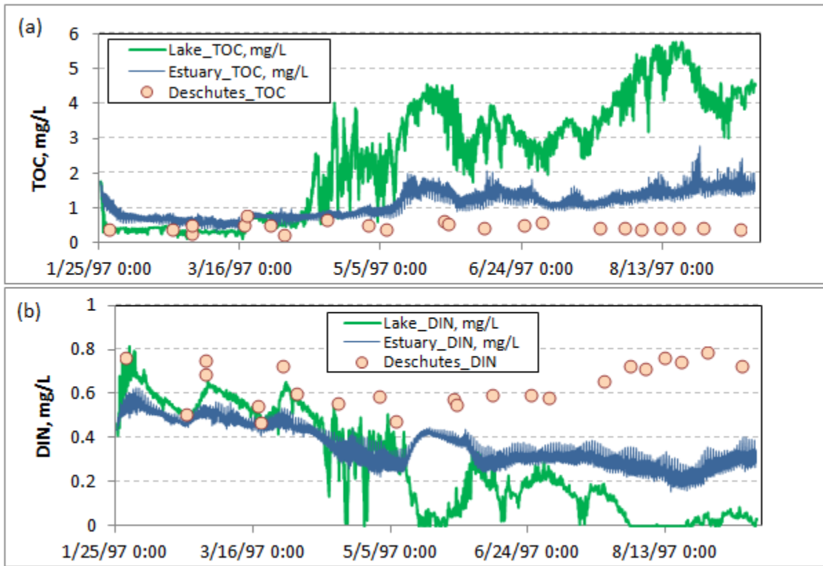
Figure 11. a) Total organic carbon (TOC) and b) dissolved inorganic nitrogen (DIN) concentrations at the location of the Capitol Lake dam under Lake (with the dam) and Estuary (without the dam) scenarios compared with concentrations in the Deschutes River at E Street.
