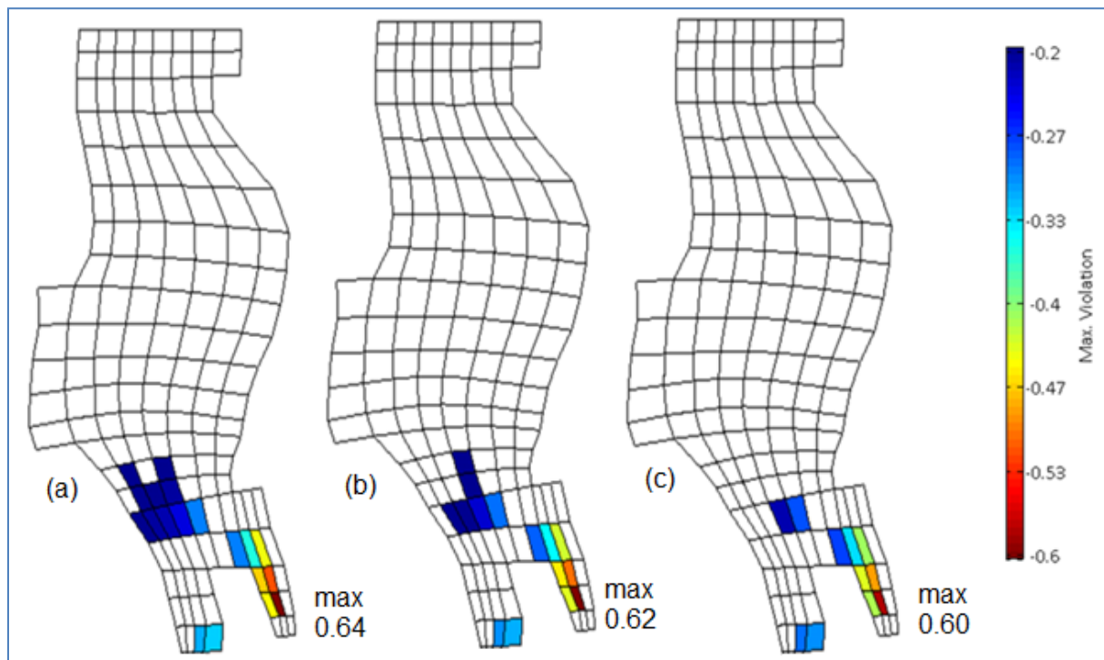
Figure 19. DO depletion (mg/L) without the Capitol Lake dam (a) with the existing anthropogenic nitrogen sources (same as Figure 17), (b) with 20% reduction in local anthropogenic watershed sources, and (c) with 50% reduction in local anthropogenic sources.
