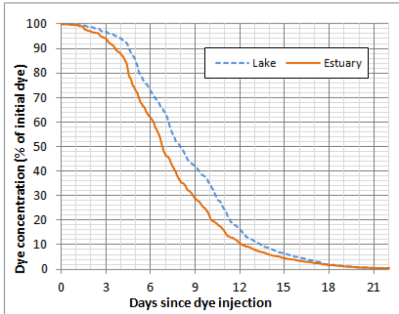
Figure 10. Time-series dye concentration at the critical East Bay grid cell under two scenarios: Lake (dashed blue line with the dam) and Estuary (solid orange line without the dam).
