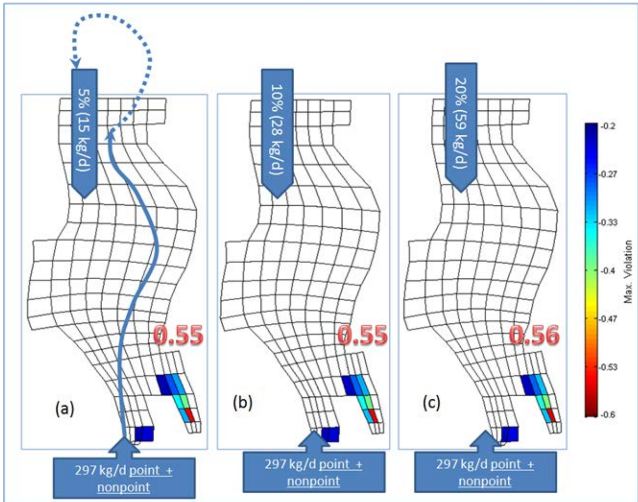
Figure 27. DO depletion (mg/L) with no Capitol Lake dam with (a) reflux of 5% of the local nonpoint anthropogenic load, (b) reflux of 10% of the local nonpoint anthropogenic load, and (c) reflux of 20% of the local nonpoint anthropogenic load.
