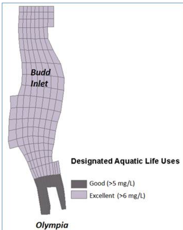
Figure 3. Water quality standards for oxygen in Budd Inlet and Capitol Lake.
