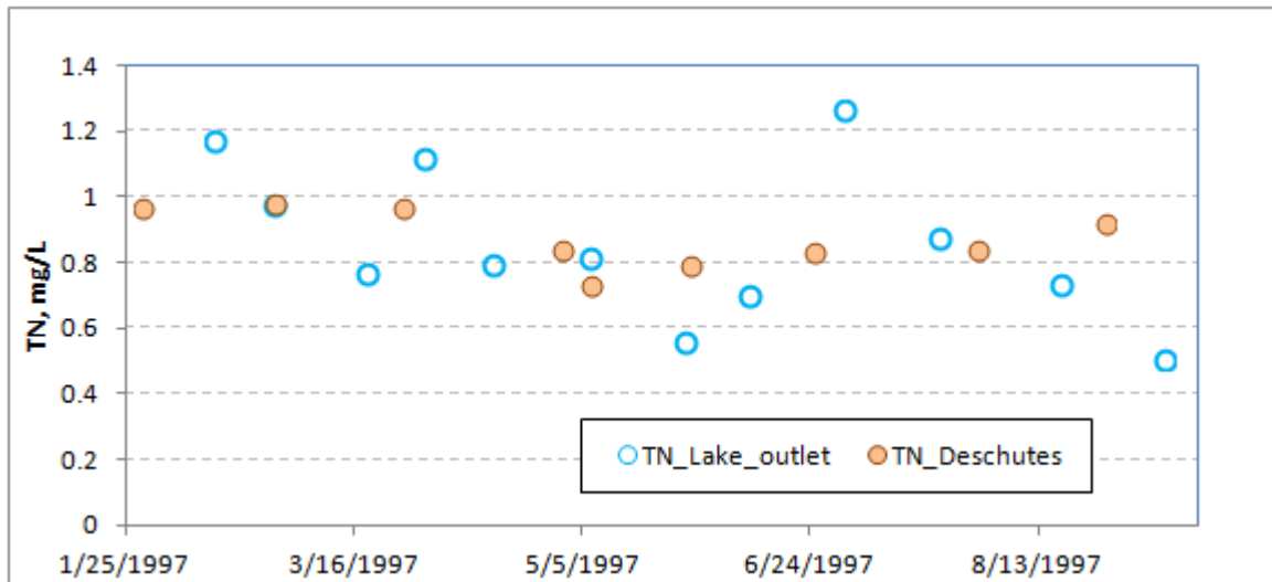
Figure 12. Total nitrogen concentration in the Deschutes River and at the location of the Capitol Lake outlet near dam during 1997.
