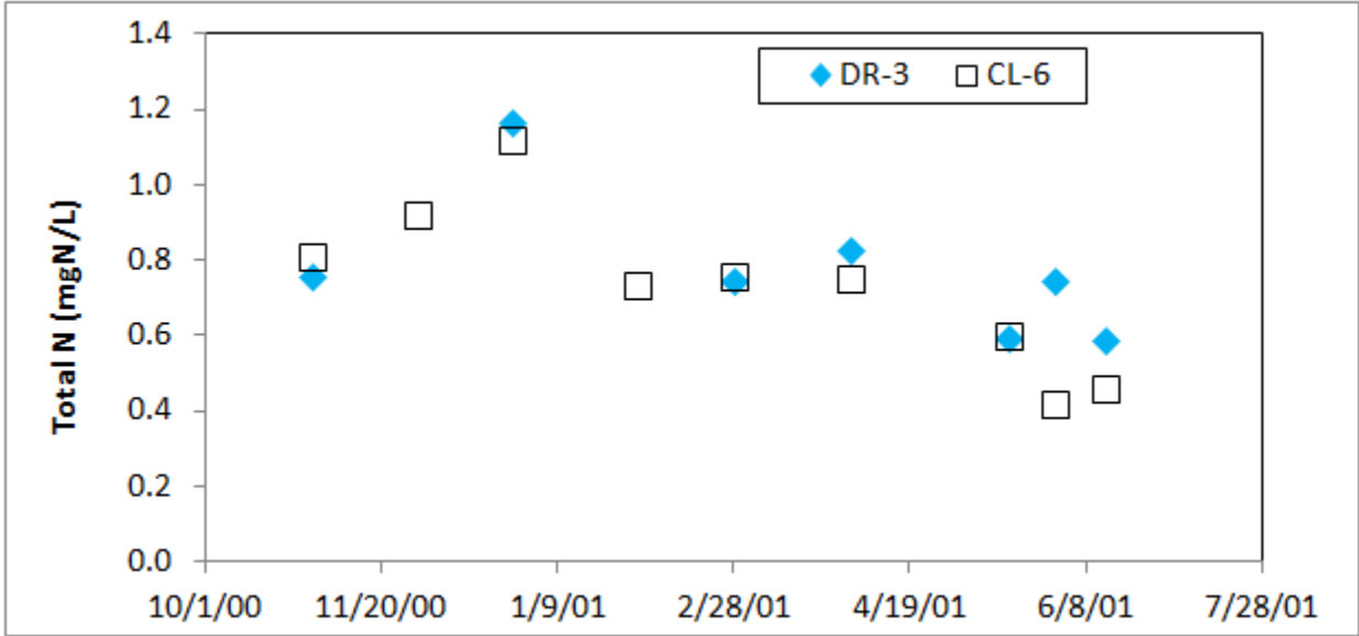
Figure 13. Total nitrogen concentrations in the Deschutes River (DR-3) and Capitol Lake near the dam (CL-6) during 2000-2001.
