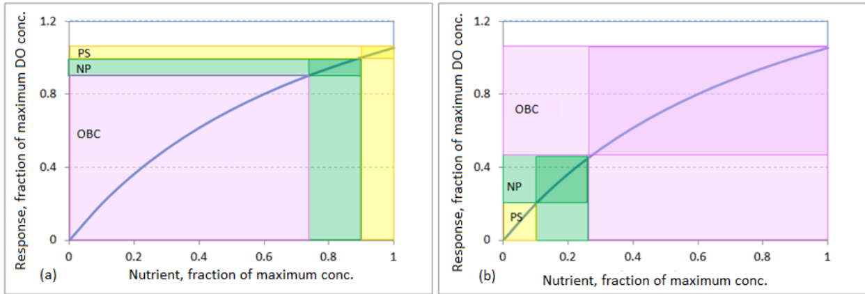
Figure 29. Decrease in DO depletion (response) as a function of the order of management activities implemented for point sources (PS), nonpoint sources (NPS) or sources outside of Budd Inlet (OBC). (a) Smaller response by point sources if they are subtracted first from the combined anthropogenic loading, and (b) larger response contribution to depletion of DO by point sources if they are subtracted last from the combined anthropogenic loading.
