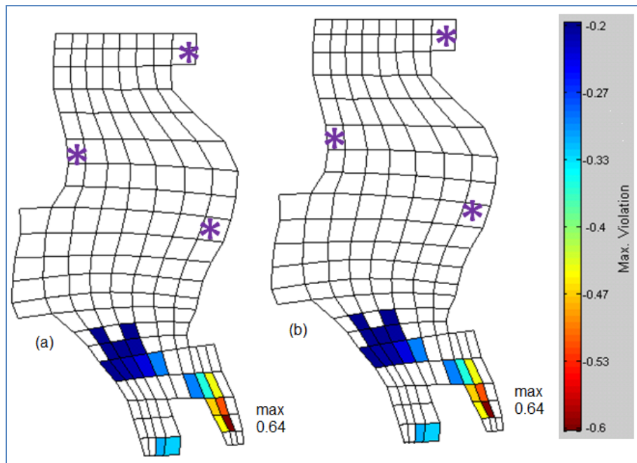
Figure 20. DO (mg/L) depletion without the Capitol Lake dam (a) with existing anthropogenic nitrogen sources (same as Figure 17), and (b) with advanced treatment for nitrogen removal at the three small WWTPs (Seashore Villa, Tamoshan, and Boston Harbor) discharging to Budd Inlet.
