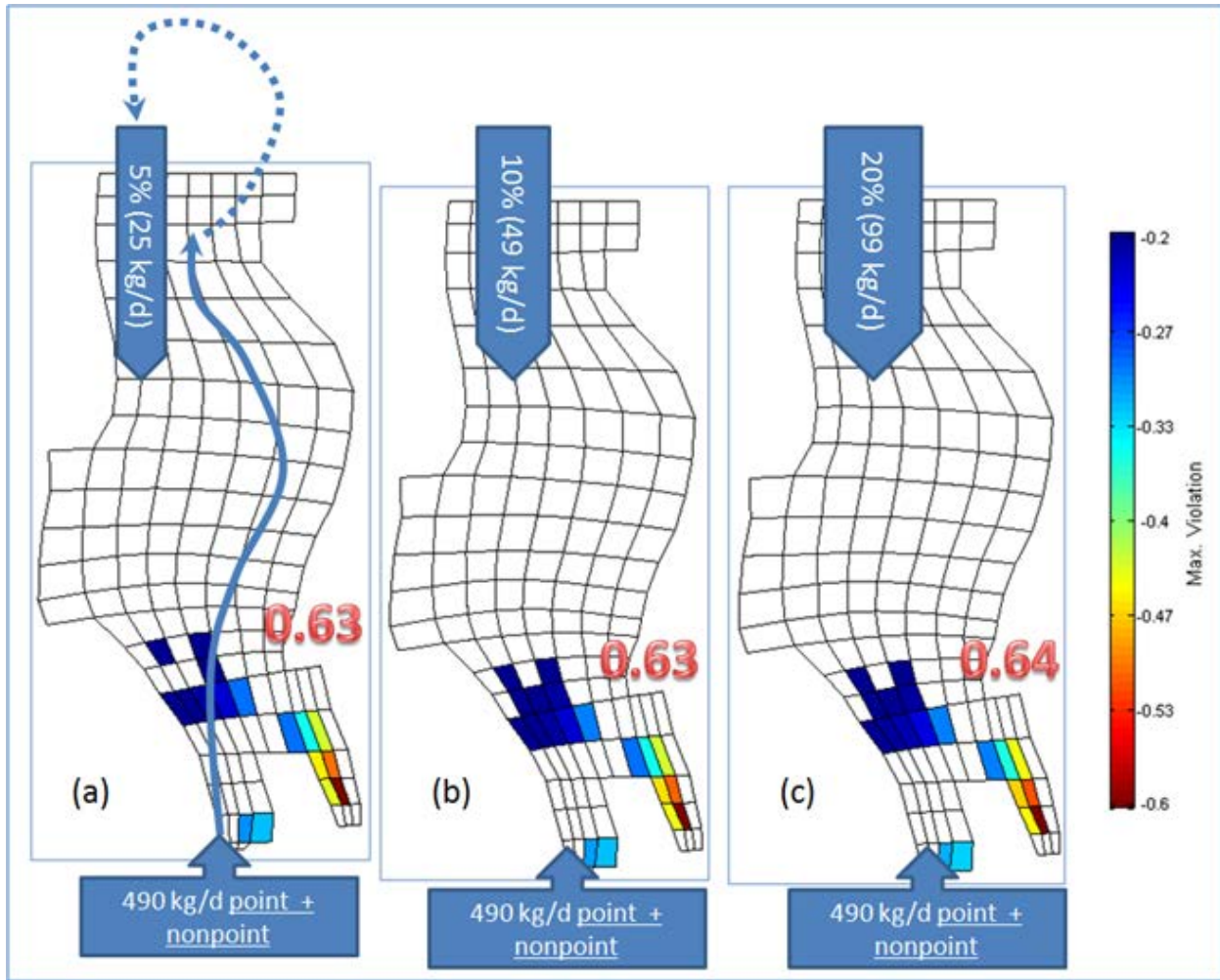
Figure 28. DO depletion (mg/L) with no Capitol Lake dam with (a) reflux of 5% of the total local anthropogenic load, (b) reflux of 10% of the total local anthropogenic load, and (c) reflux of 20% of the total local anthropogenic load.
