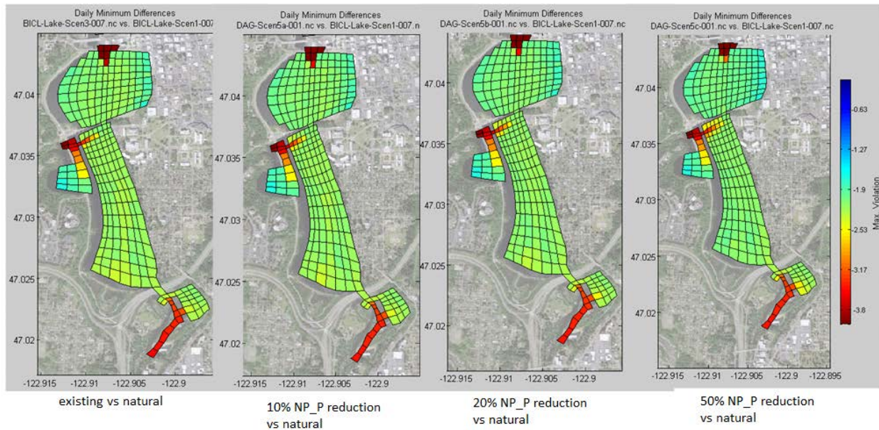
Figure 34. Predicted DO depletion (mg/L) from various assumed reductions in nonpoint phosphorus loading to Capitol Lake.
