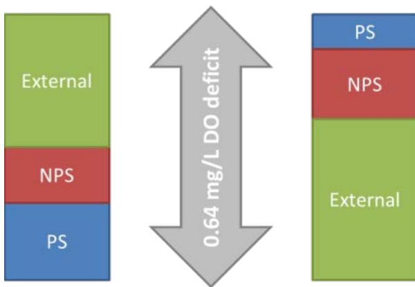
Figure 30. Example of how the order of management activities (top to bottom) implemented affects the DO depletion (vertical extent of the boxes) in the critical cell in East Bay. DO depletion is not linearly related to loading.
