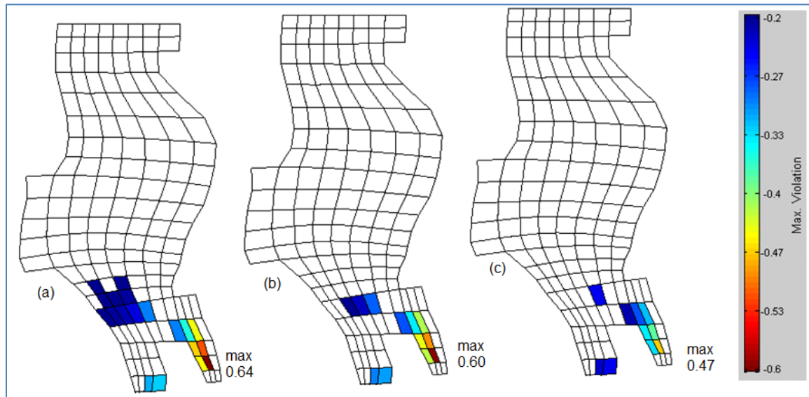
Figure 23. DO depletion (mg/L) without the Capitol Lake dam (a) with existing local anthropogenic nutrient sources (same as Figure 17), (b) with 10% reduction (149 kg/d) in external anthropogenic nutrient sources, and (c) with 50% reduction (744 kg/d) in external anthropogenic nutrient sources.
