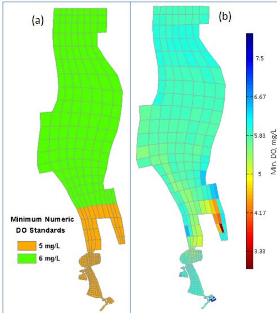
Figure 7. a) Water quality standards for DO in Budd Inlet and a natural estuary, and b) predicted minimum DO (mg/L) under natural conditions without the Capitol Lake dam.
