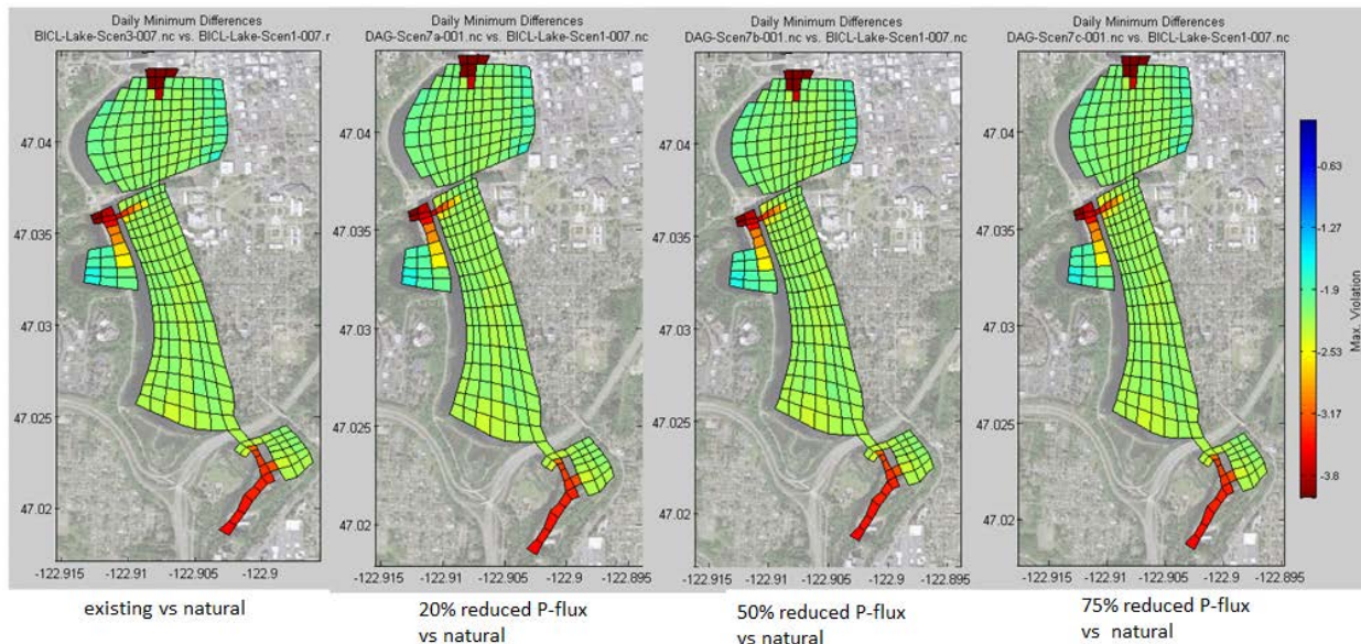
Figure 36. Predicted DO depletion (mg/L) in Capitol Lake with reduced sediment/water flux of phosphorus.
