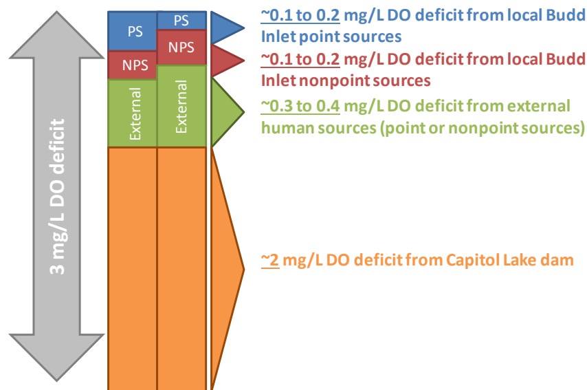
Figure 31. The estimated range of contributions to DO depletion at the critical cell in East Bay from anthropogenic activities due to various alternatives for the order of addition to, or subtraction from, other sources.
