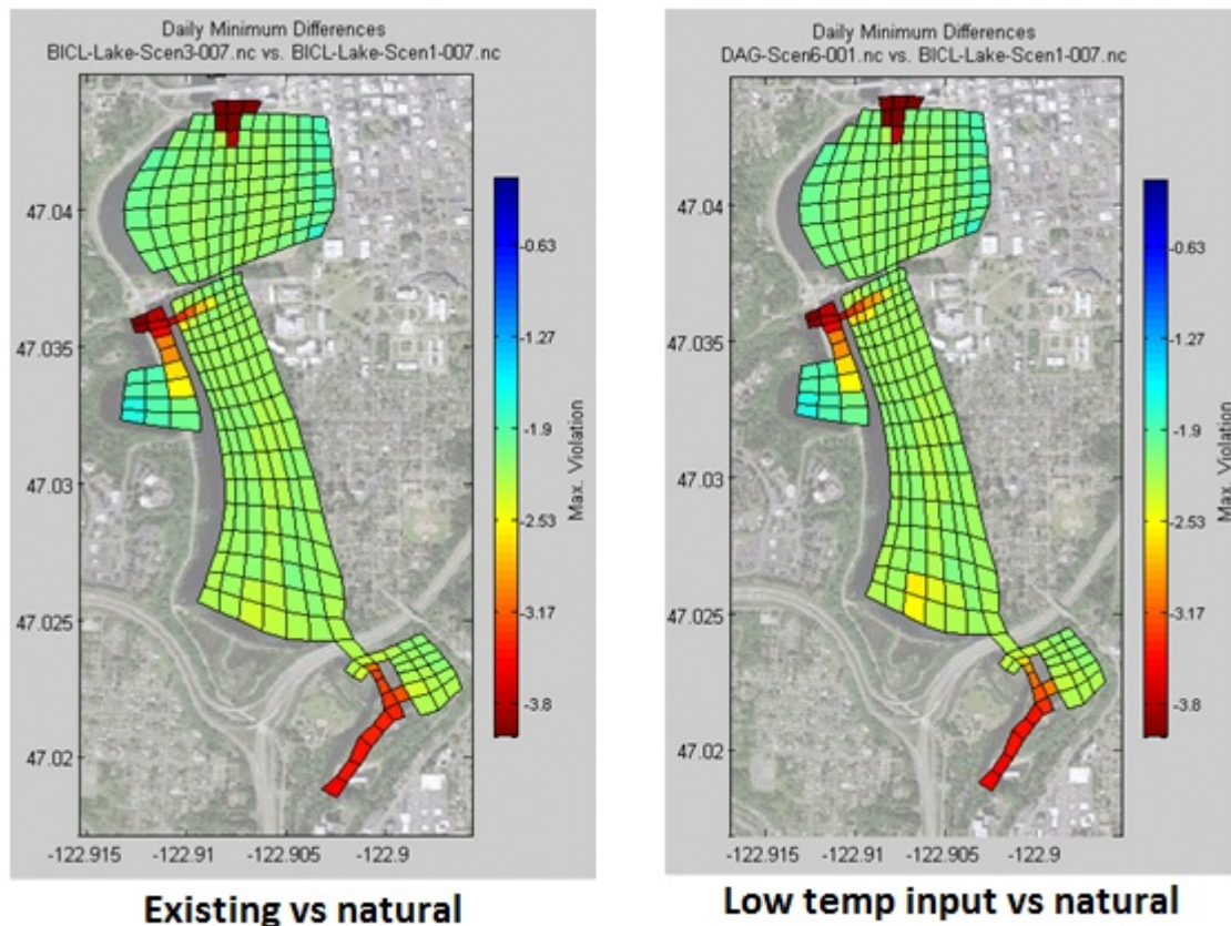
Figure 35. Predicted DO depletion (mg/L) in Capitol Lake with decreased water temperature in the Deschutes River.
