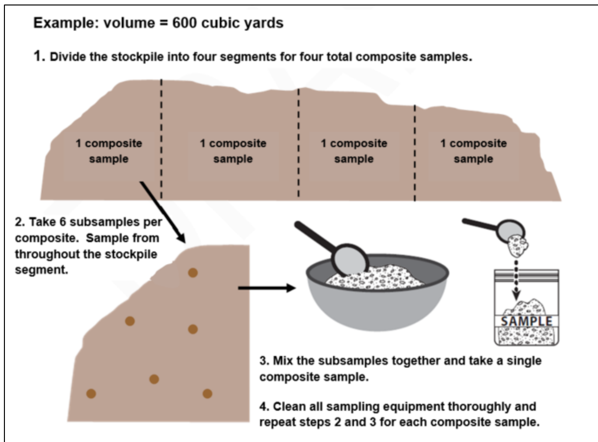
Figure 7: Stockpile sampling process.
