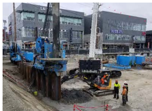
A sealed metal sheet-pile wall being installed.
